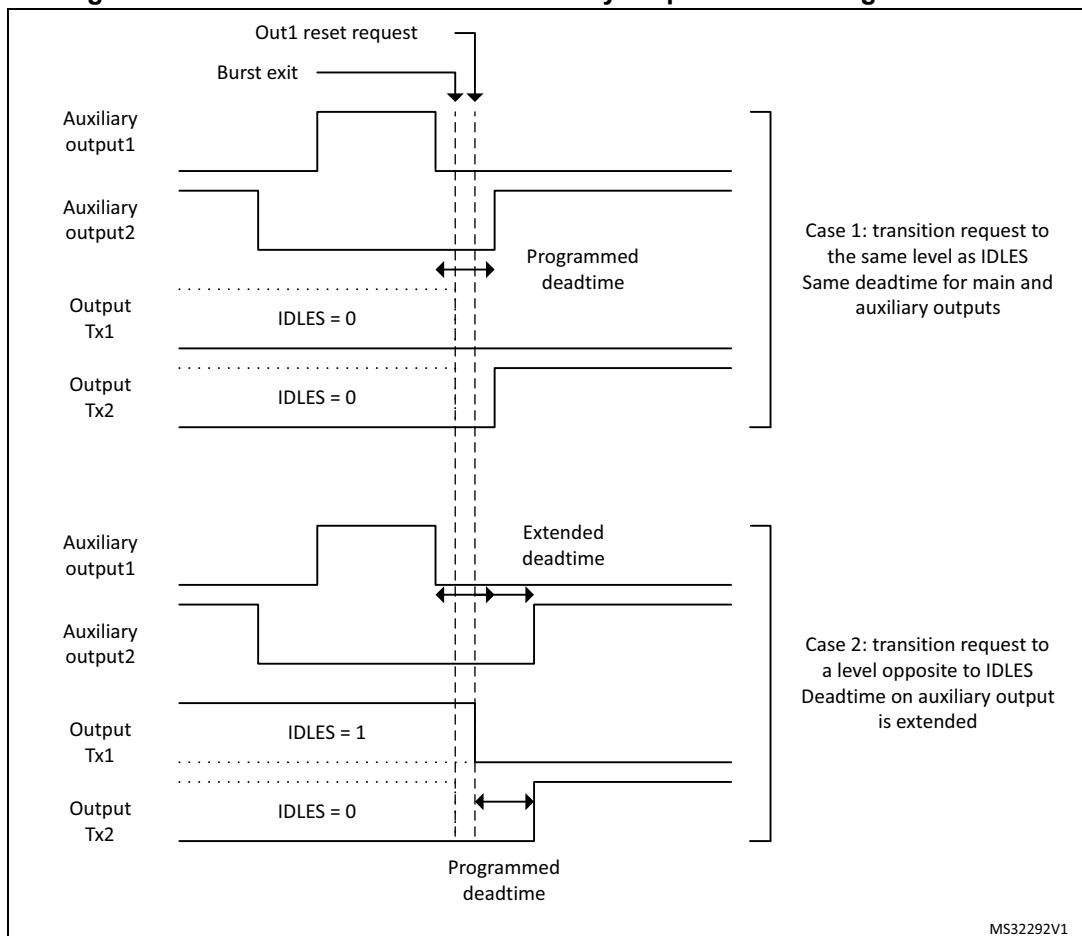
Figure 374. Deadtime distortion on auxiliary output when exiting burst mode
