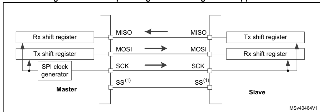
Figure 656. Full-duplex single master/ single slave application
