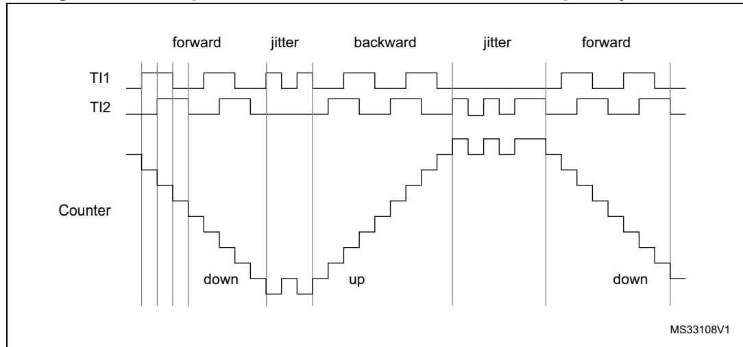
Figure 442. Example of encoder interface mode with TI1FP1 polarity inverted.
