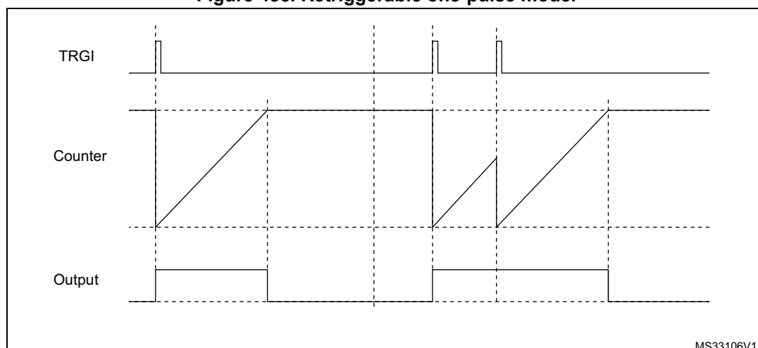
Figure 485. Retriggerable one-pulse mode.
