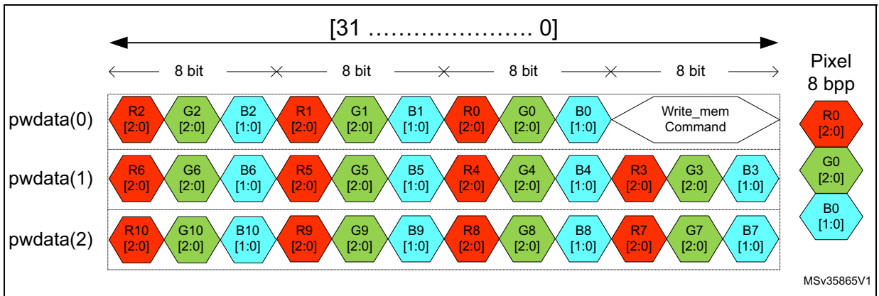
Figure 264. 8 bpp APB pixel to byte organization
