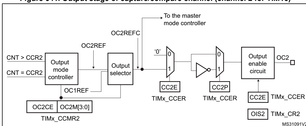
Figure 541. Output stage of capture/compare channel (channel 2 for TIM15)
