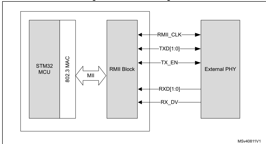
Figure 840. RMII block diagram
