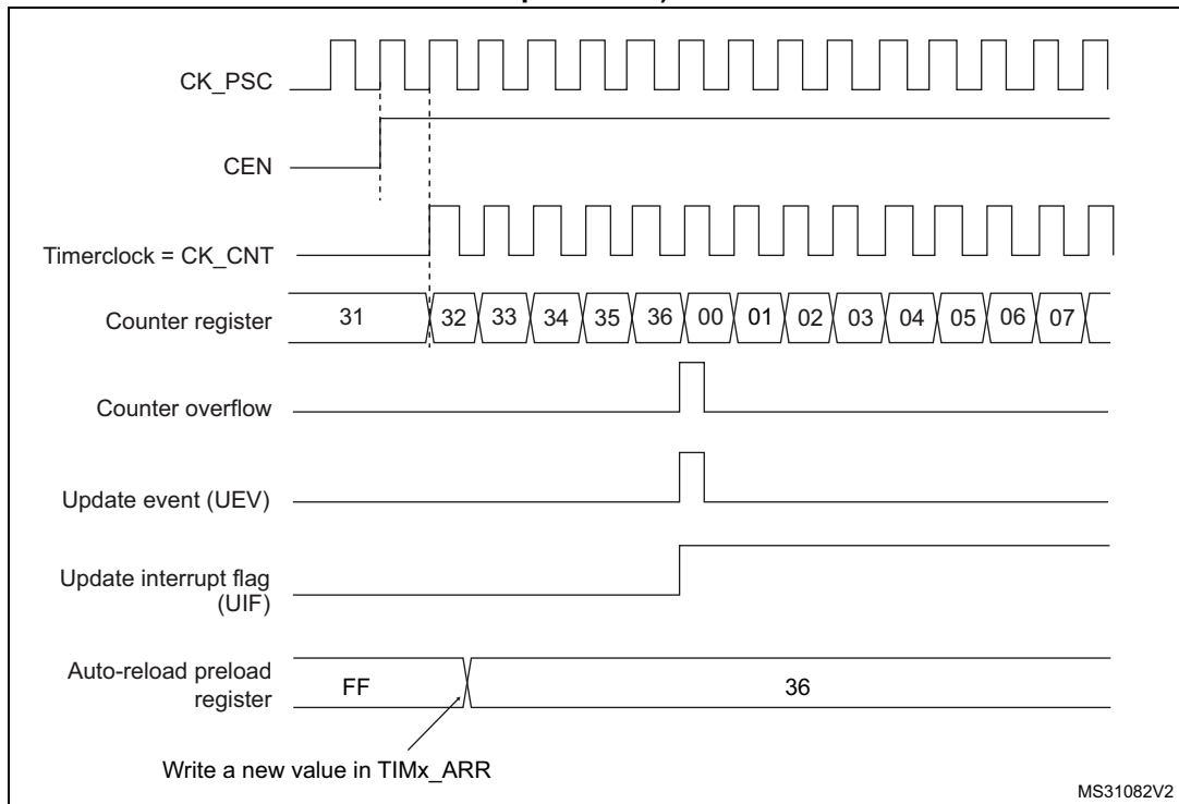
Figure 564. Counter timing diagram, update event when ARPE = 0 (TIMx_ARR not preloaded)
