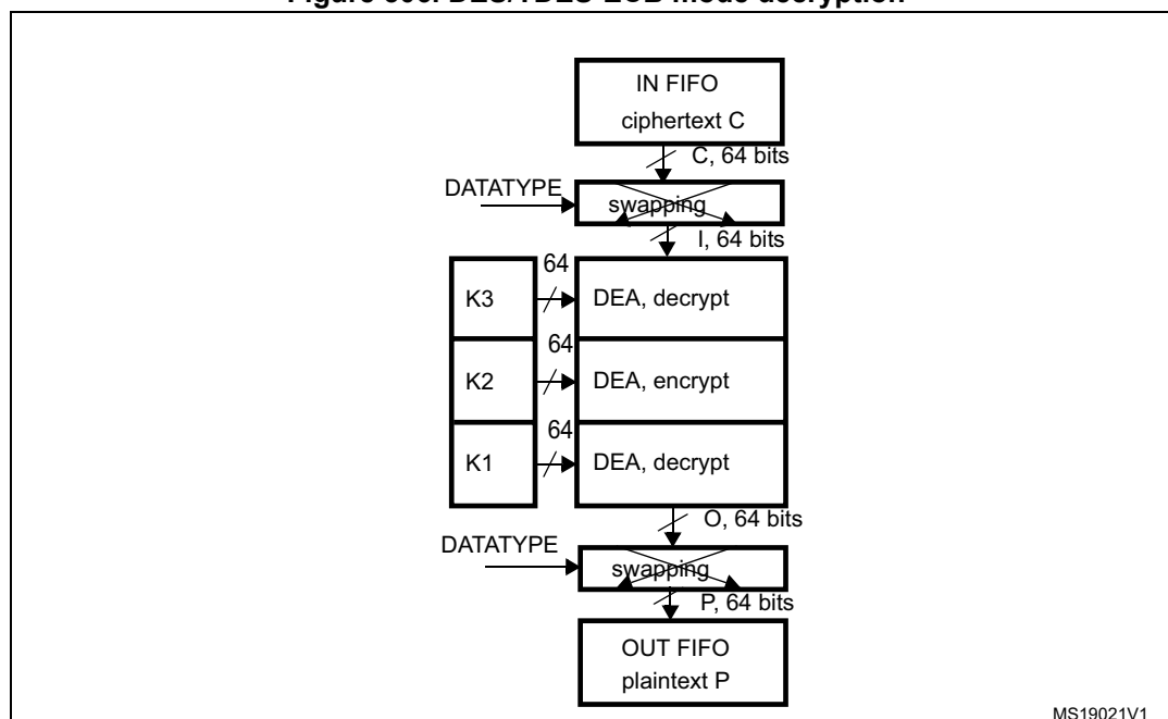
Figure 306. DES/TDES-ECB mode decryption
