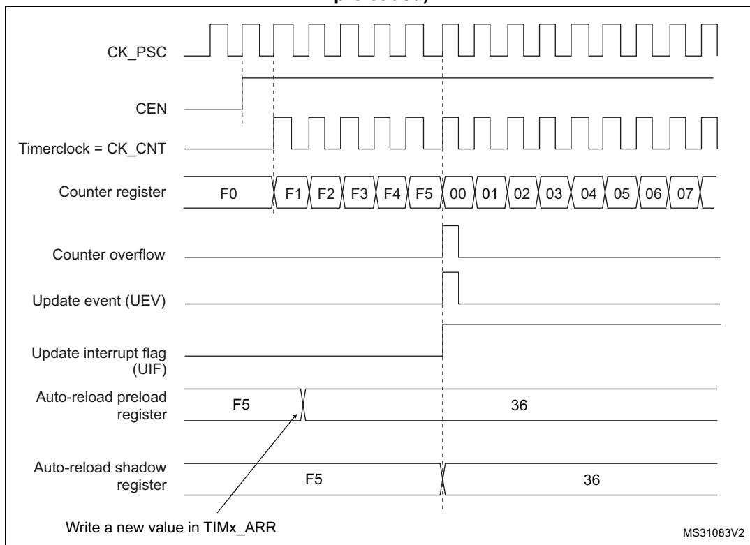
Figure 533. Counter timing diagram, update event when ARPE=1 (TIMx_ARR preloaded)
