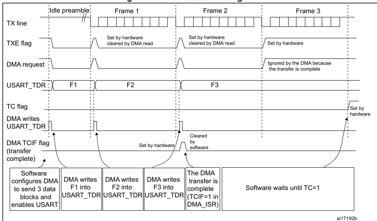
Figure 648. Transmission using DMA
