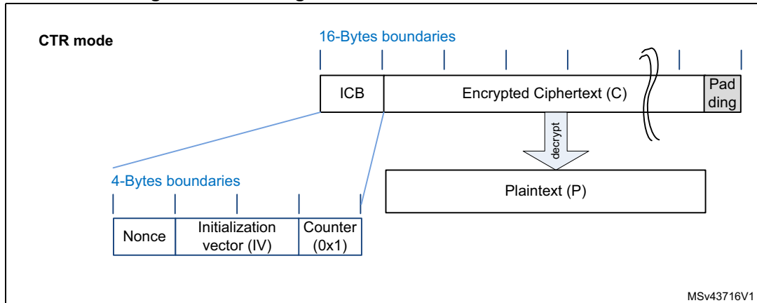
Figure 313. Message construction for the Counter mode
