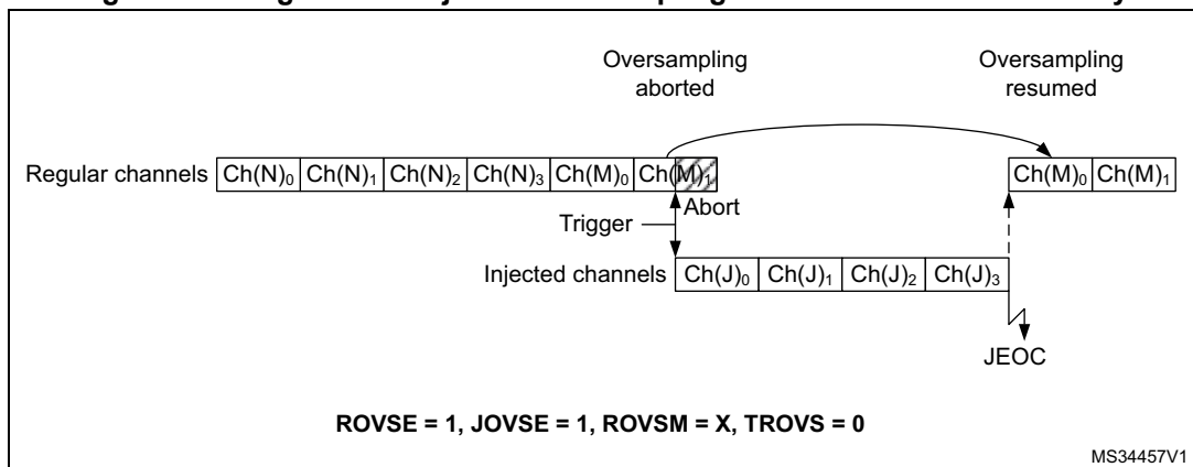
Figure 188. Regular and injected oversampling modes used simultaneously
