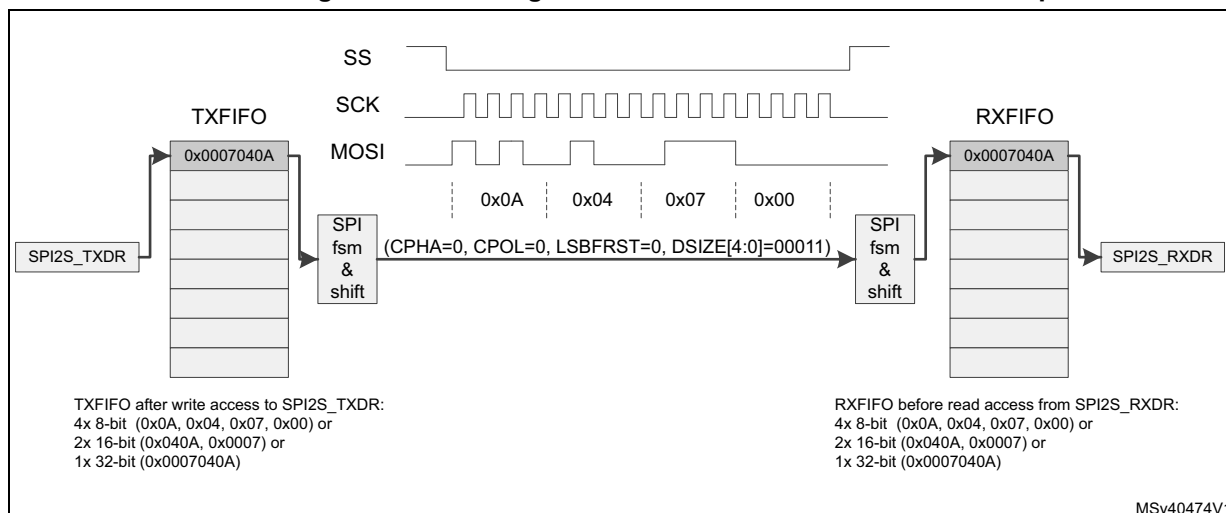
Figure 667. Packing data in FIFO for transmission and reception
