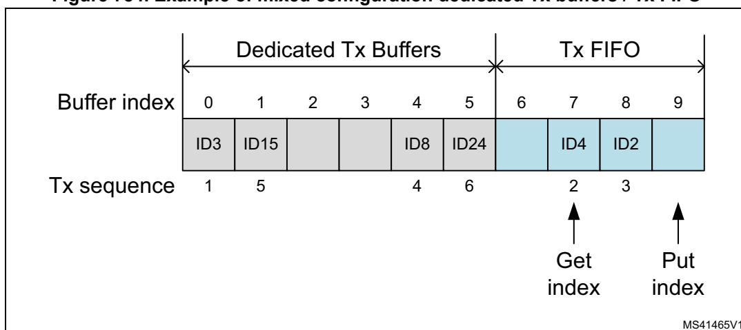
Figure 784. Example of mixed configuration dedicated Tx buffers / Tx FIFO
