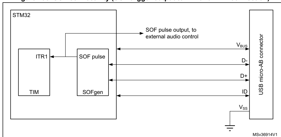
Figure 795. SOF connectivity (SOF trigger output to TIM and ITR1 connection)
