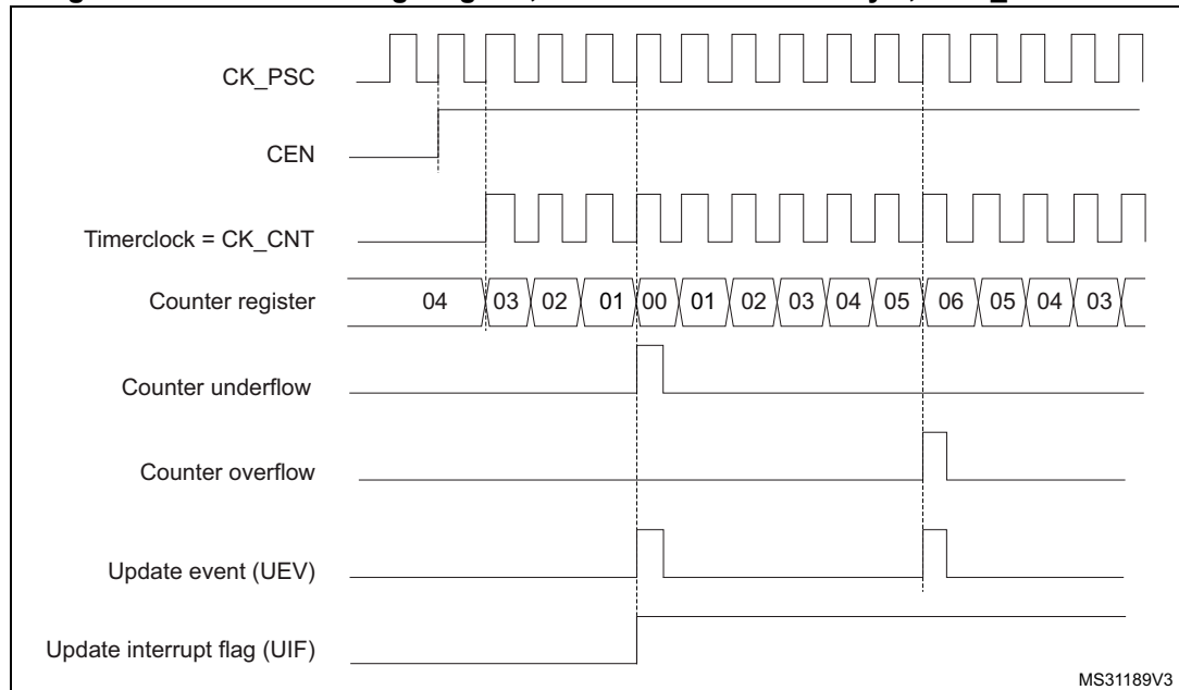
Figure 403. Counter timing diagram, internal clock divided by 1, TIMx_ARR = 0x6
