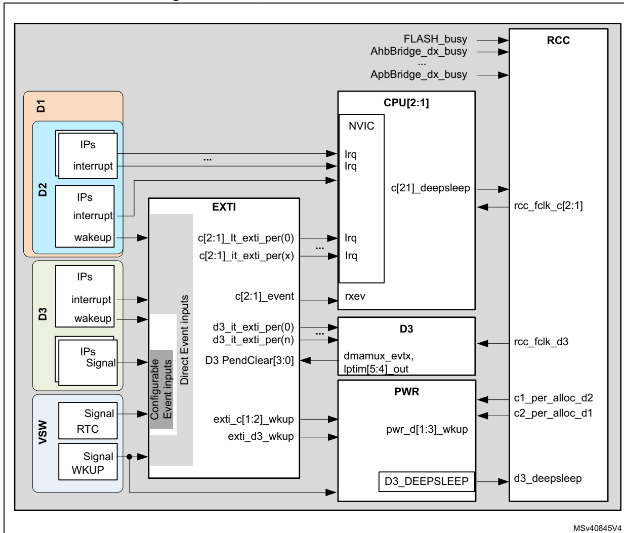
Figure 43. EXTI, RCC and PWR interconnections
