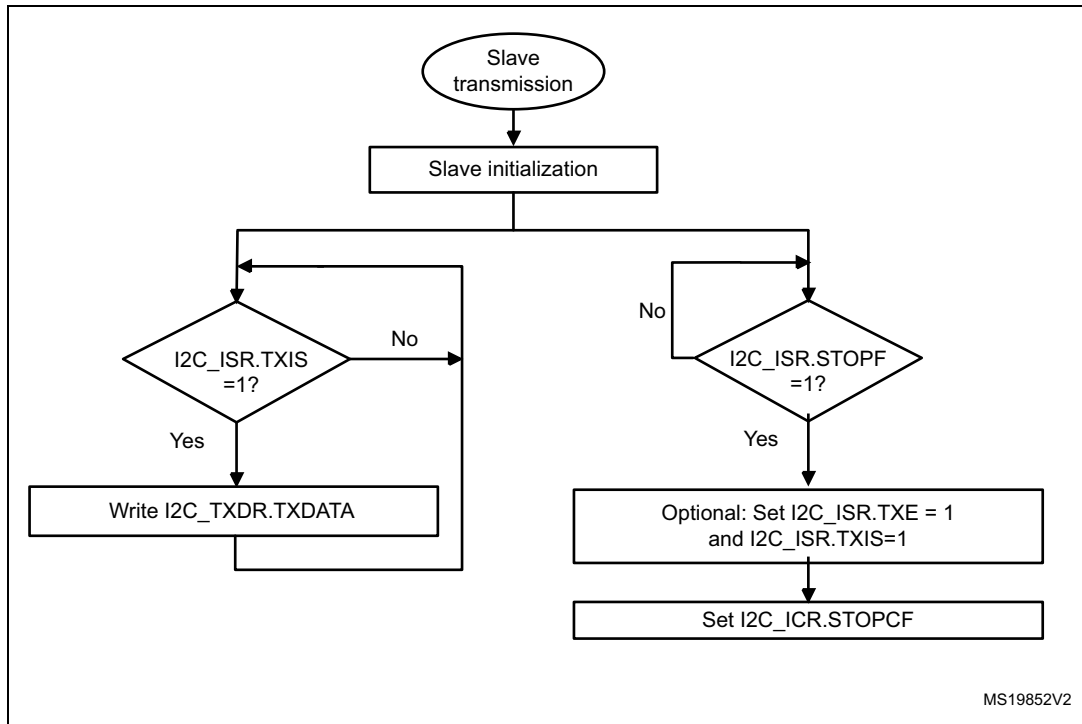
Figure 591. Transfer sequence flowchart for I2C slave transmitter, NOSTRETCH= 1
