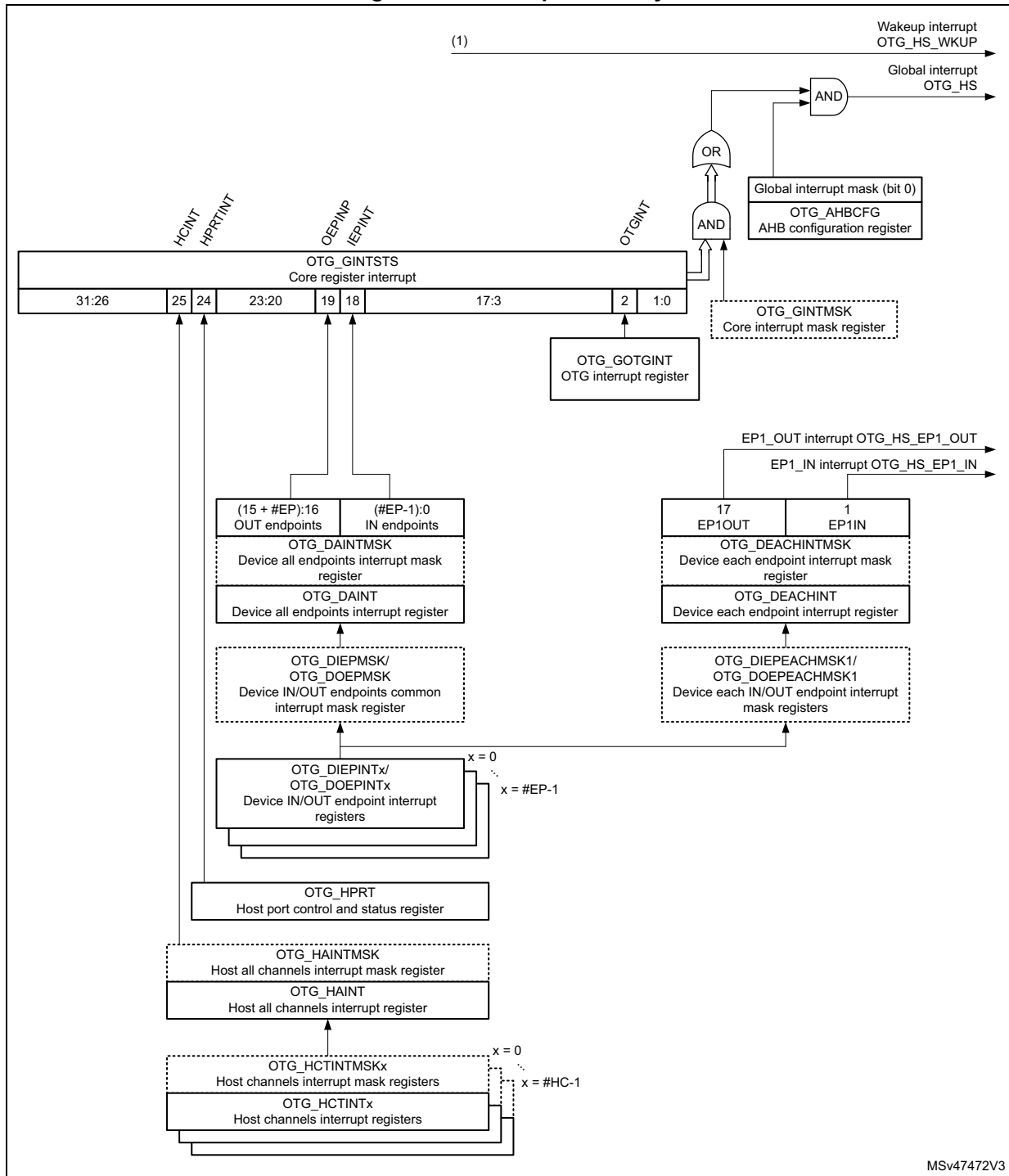
Figure 799. Interrupt hierarchy
