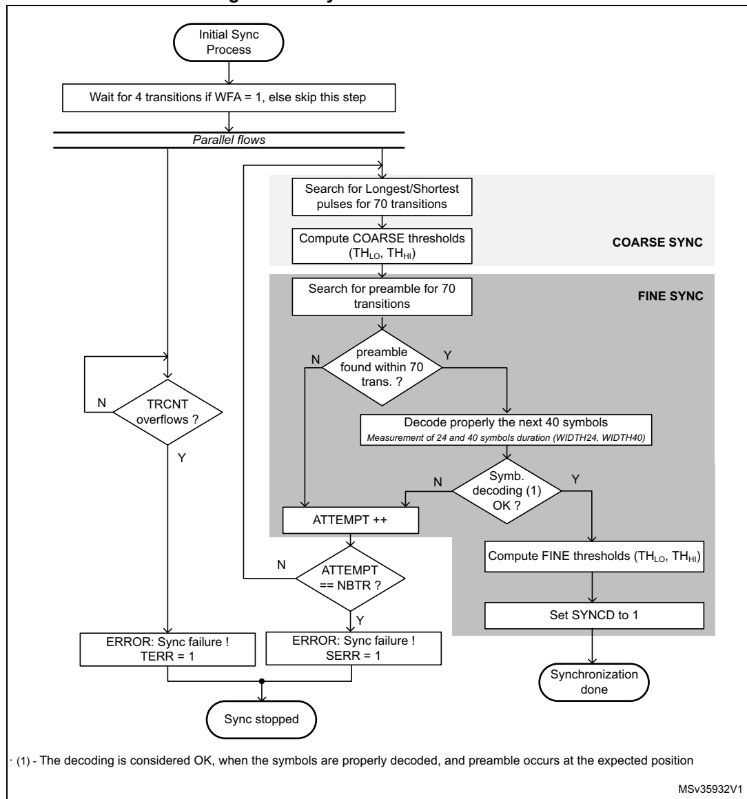
Figure 719. Synchronization flowchart
