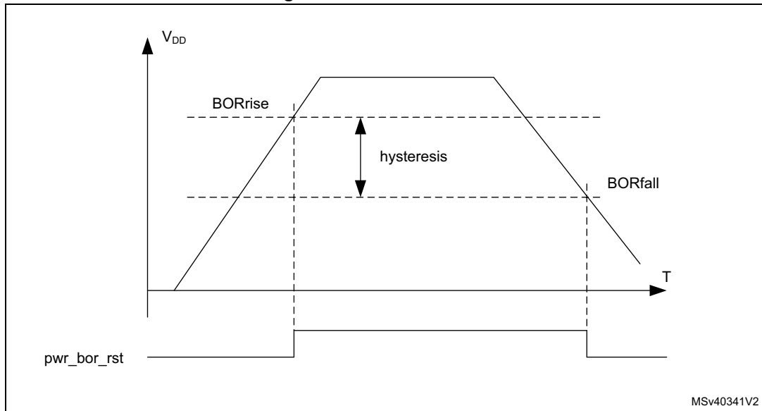
Figure 30. BOR thresholds
