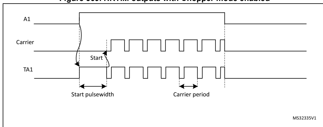
Figure 369. HRTIM outputs with Chopper mode enabled
