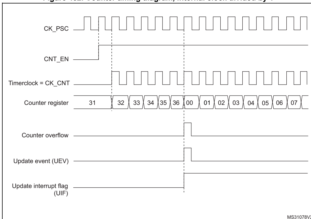
Figure 452. Counter timing diagram, internal clock divided by 1
