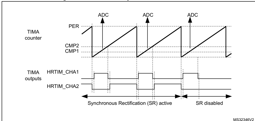
Figure 384. Buck with synchronous rectification
