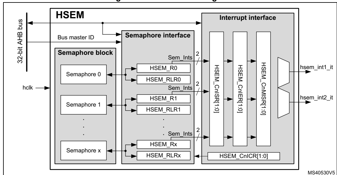
Figure 72. HSEM block diagram
