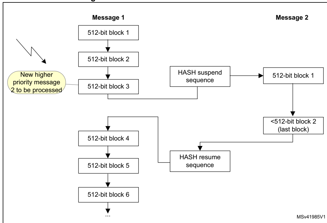
Figure 324. HASH save/restore mechanism
