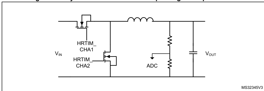
Figure 383. Synchronous rectification depending on output current
