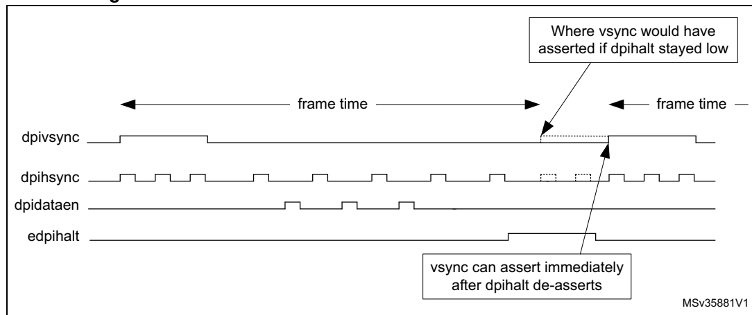
Figure 270. Transmission of commands on the last line of a frame
