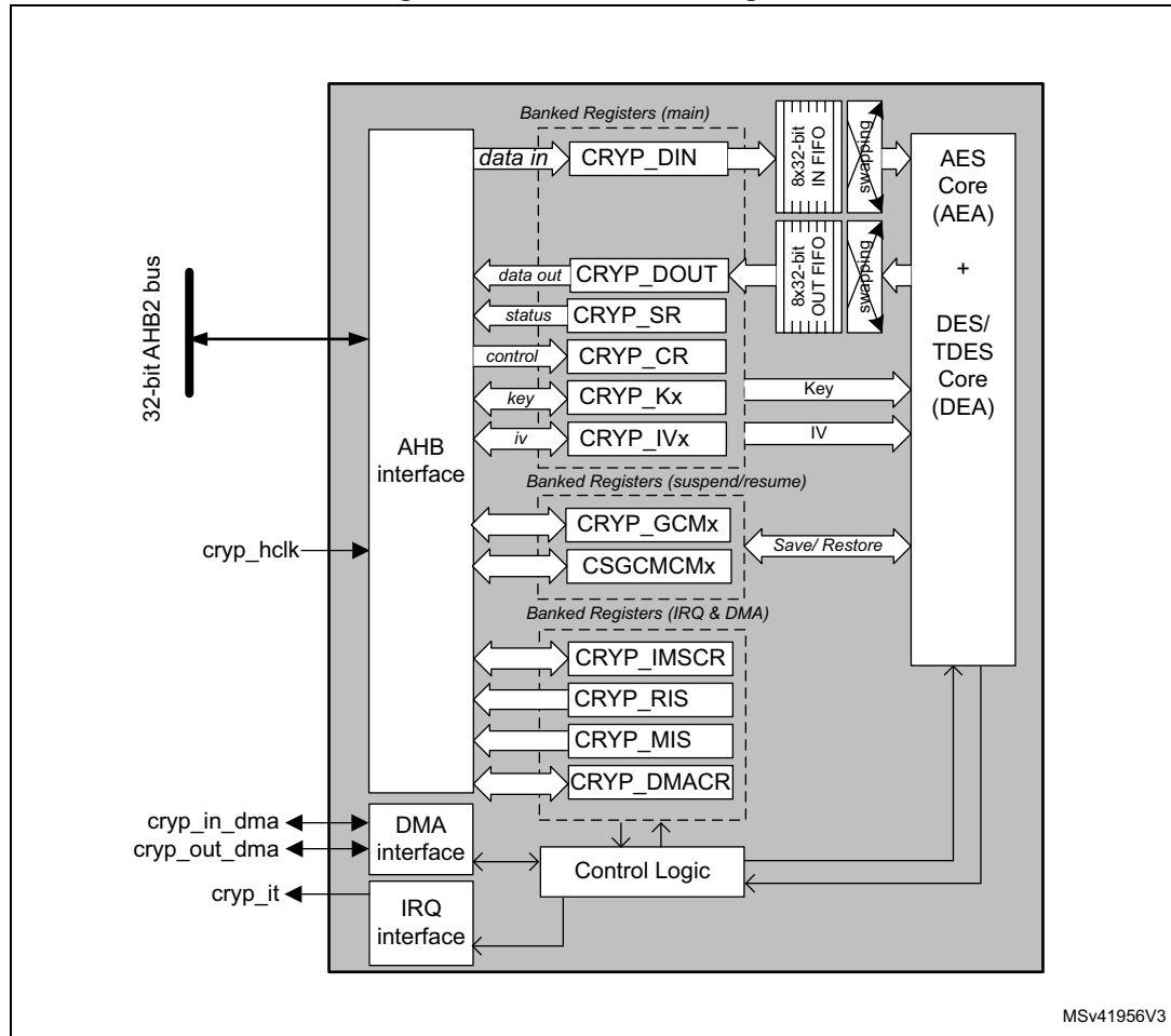
Figure 295. CRYP block diagram
