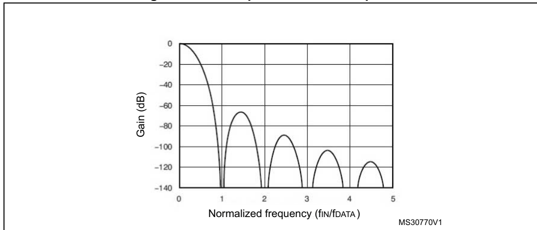
Figure 239. Example: Sinc 3 filter response
