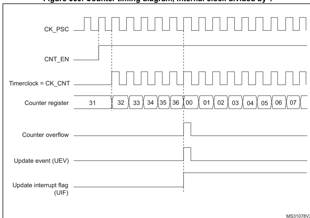
Figure 560. Counter timing diagram, internal clock divided by 1
