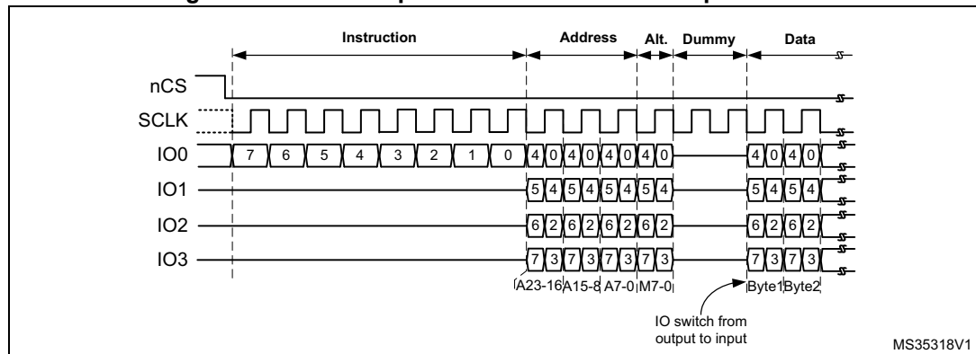
Figure 134. An example of a DDR command in quad mode
