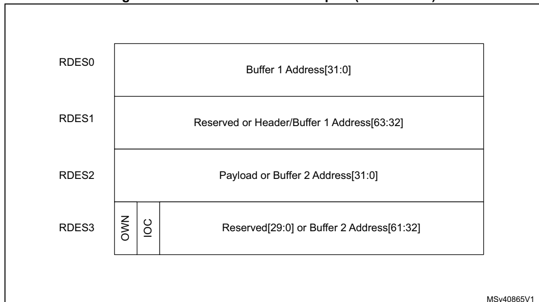
Figure 848. Receive normal descriptor (read format)
