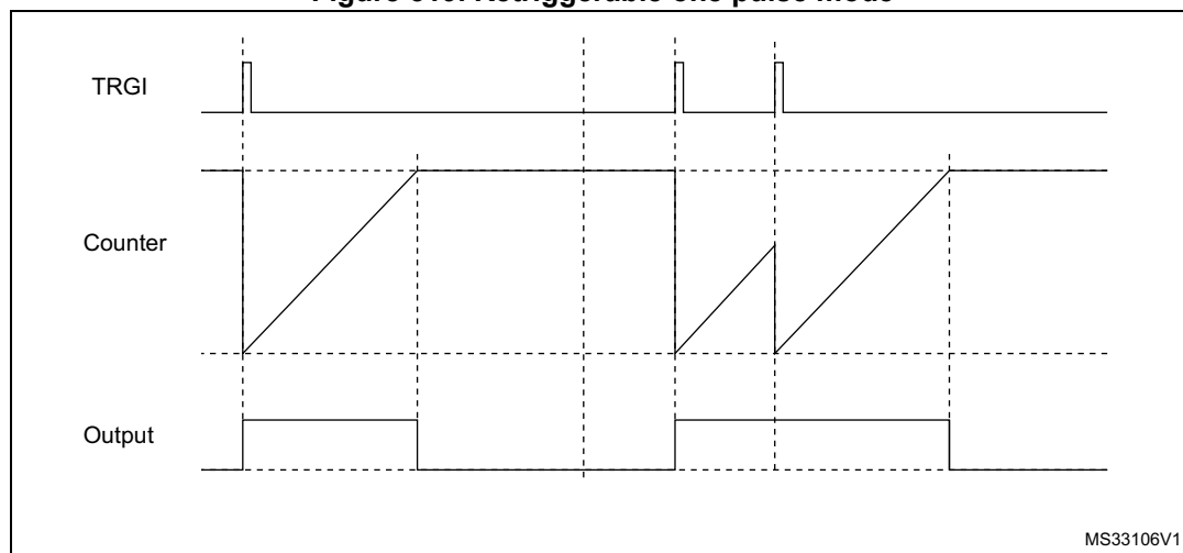
Figure 519. Retriggerable one pulse mode
