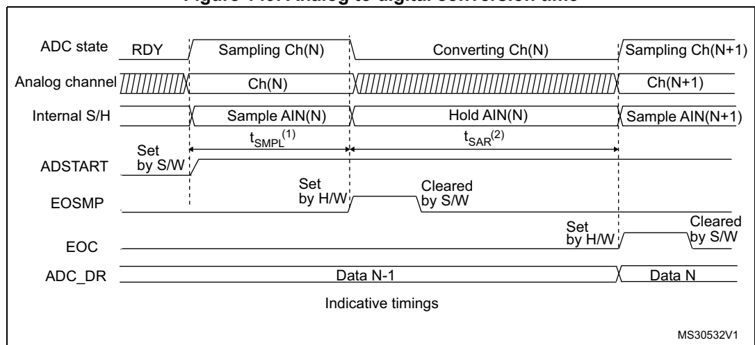
Figure 149. Analog to digital conversion time
