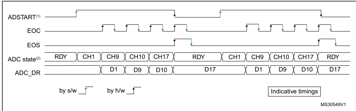
Figure 166. Single conversions of a sequence, software trigger
