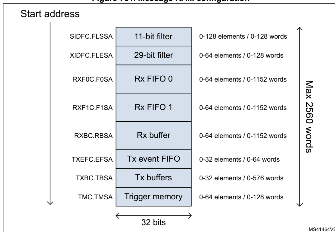
Figure 781. Message RAM configuration
