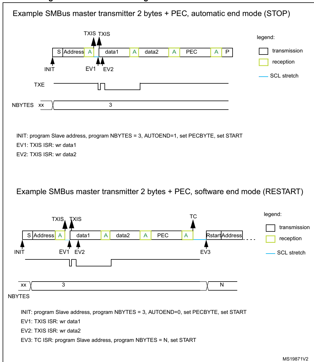
Figure 611. Bus transfer diagrams for SMBus master transmitter
