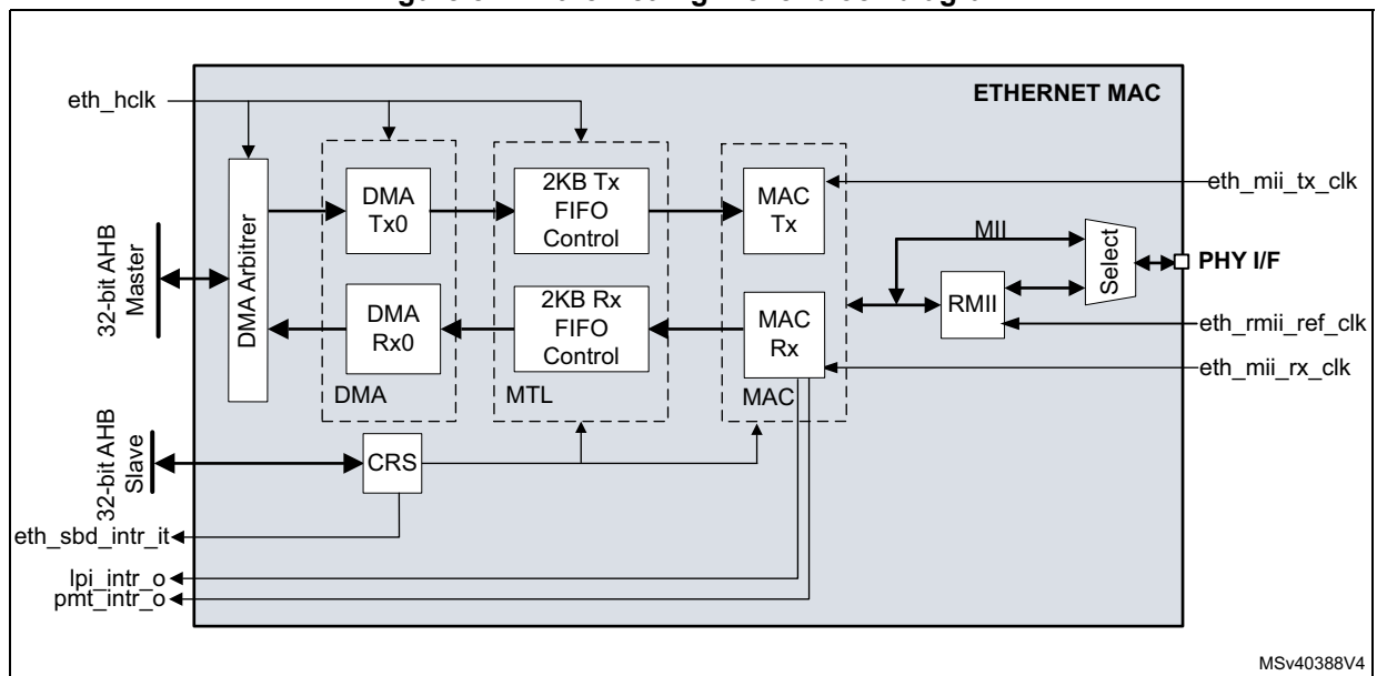
Figure 822. Ethernet high-level block diagram
