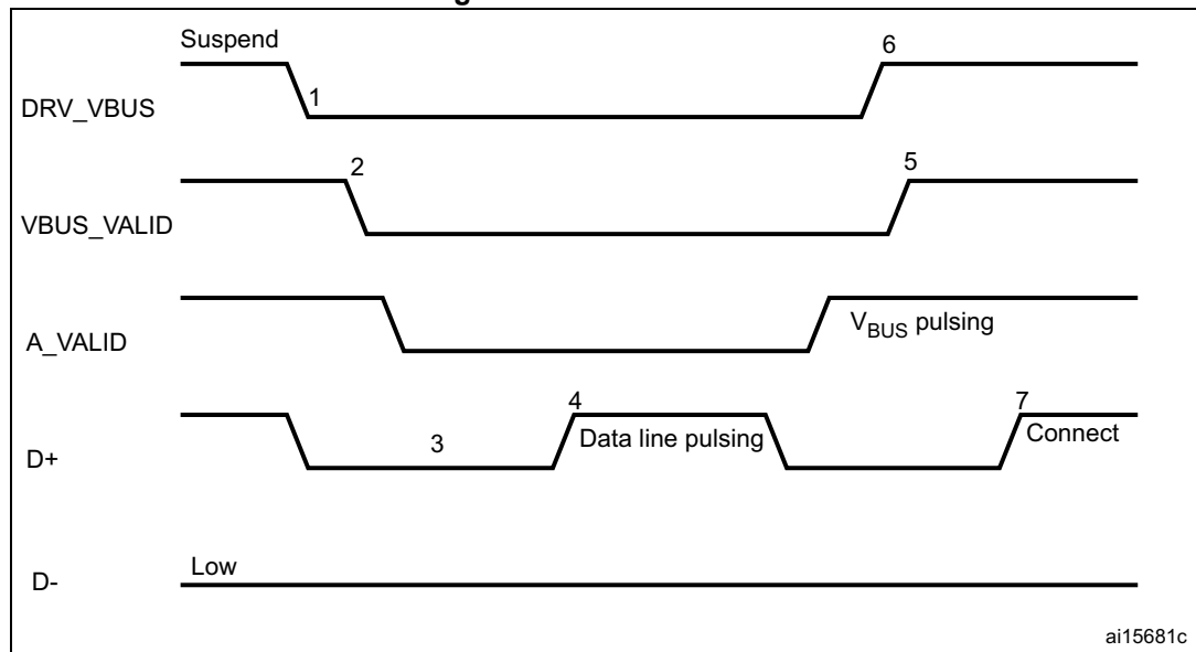
Figure 818. A-device SRP
