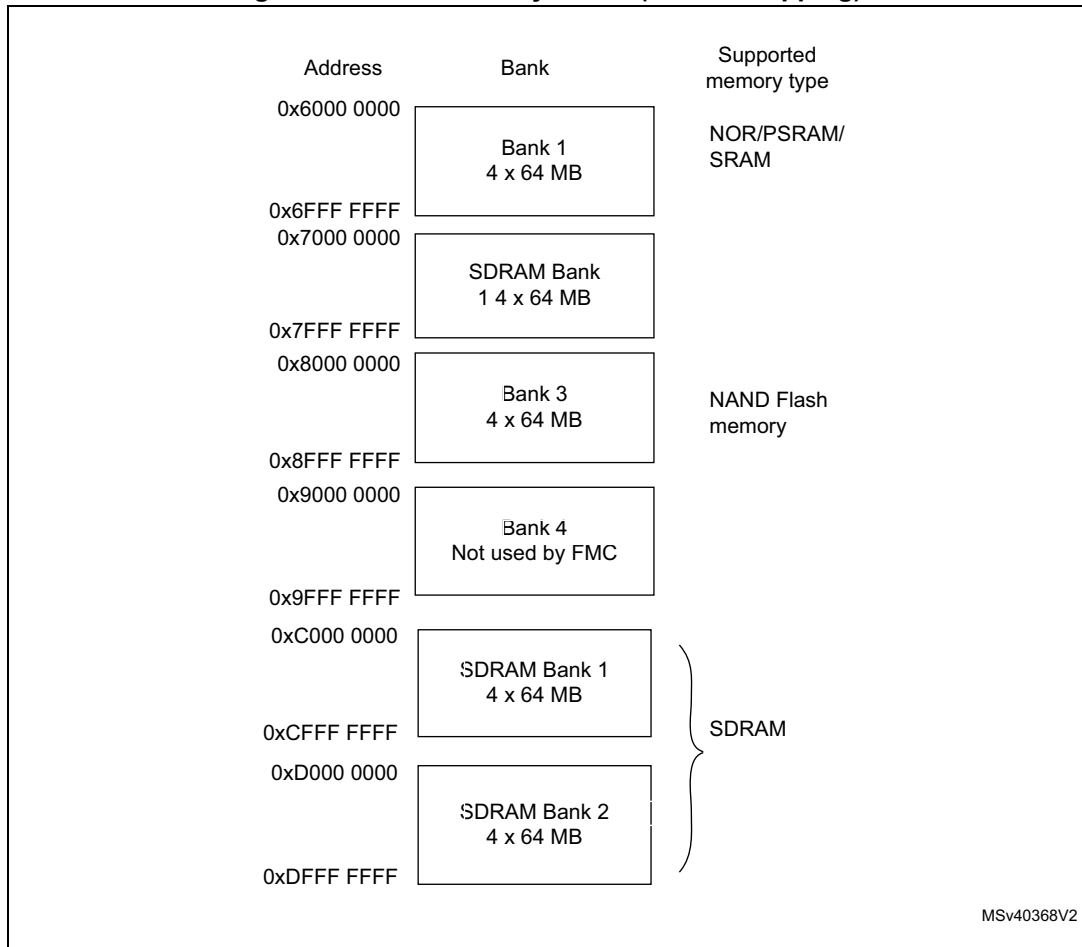
Figure 103. FMC memory banks (default mapping)
