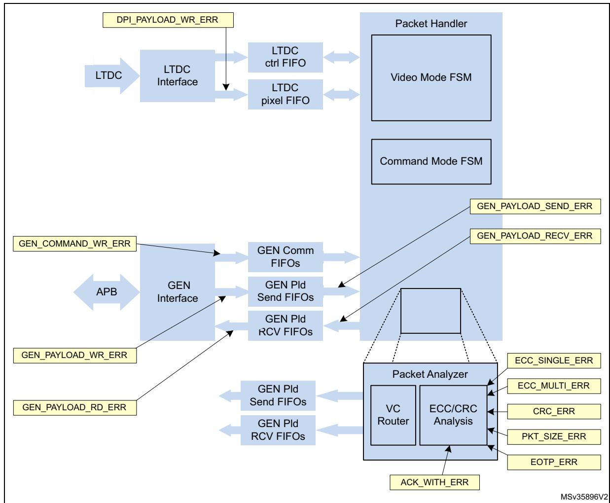
Figure 287. Error sources
