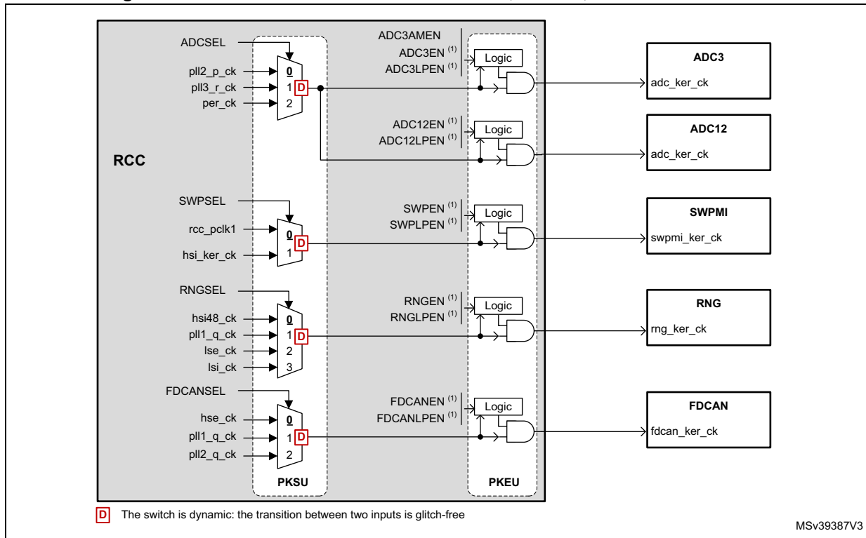
Figure 63. Kernel clock distribution For ADCs, SWPMI, RNG and FDCAN (2)
