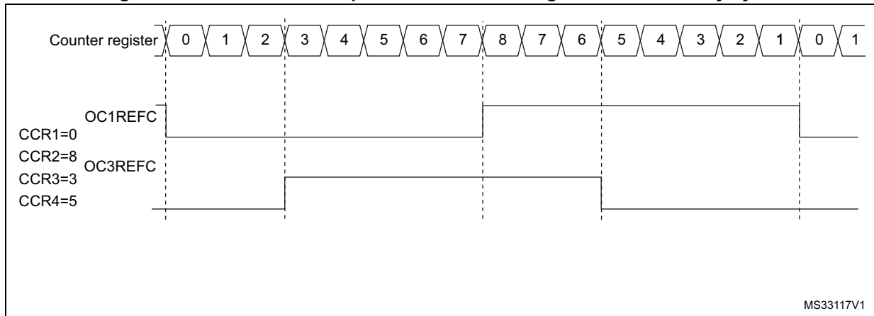
Figure 426. Generation of 2 phase-shifted PWM signals with 50% duty cycle
