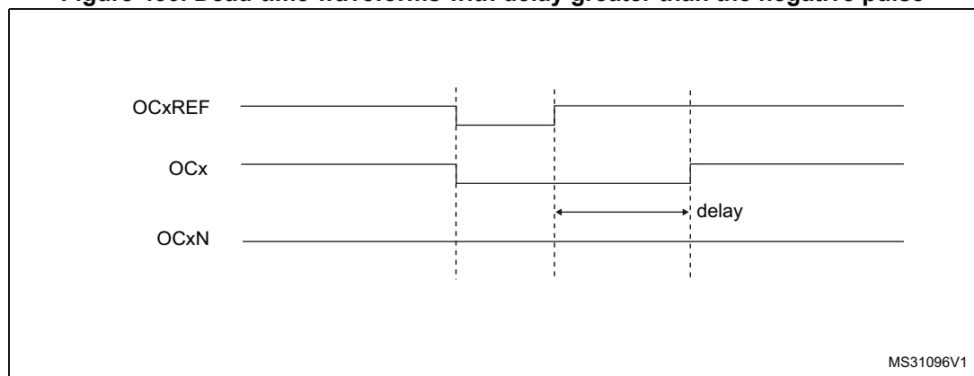
Figure 430. Dead-time waveforms with delay greater than the negative pulse
