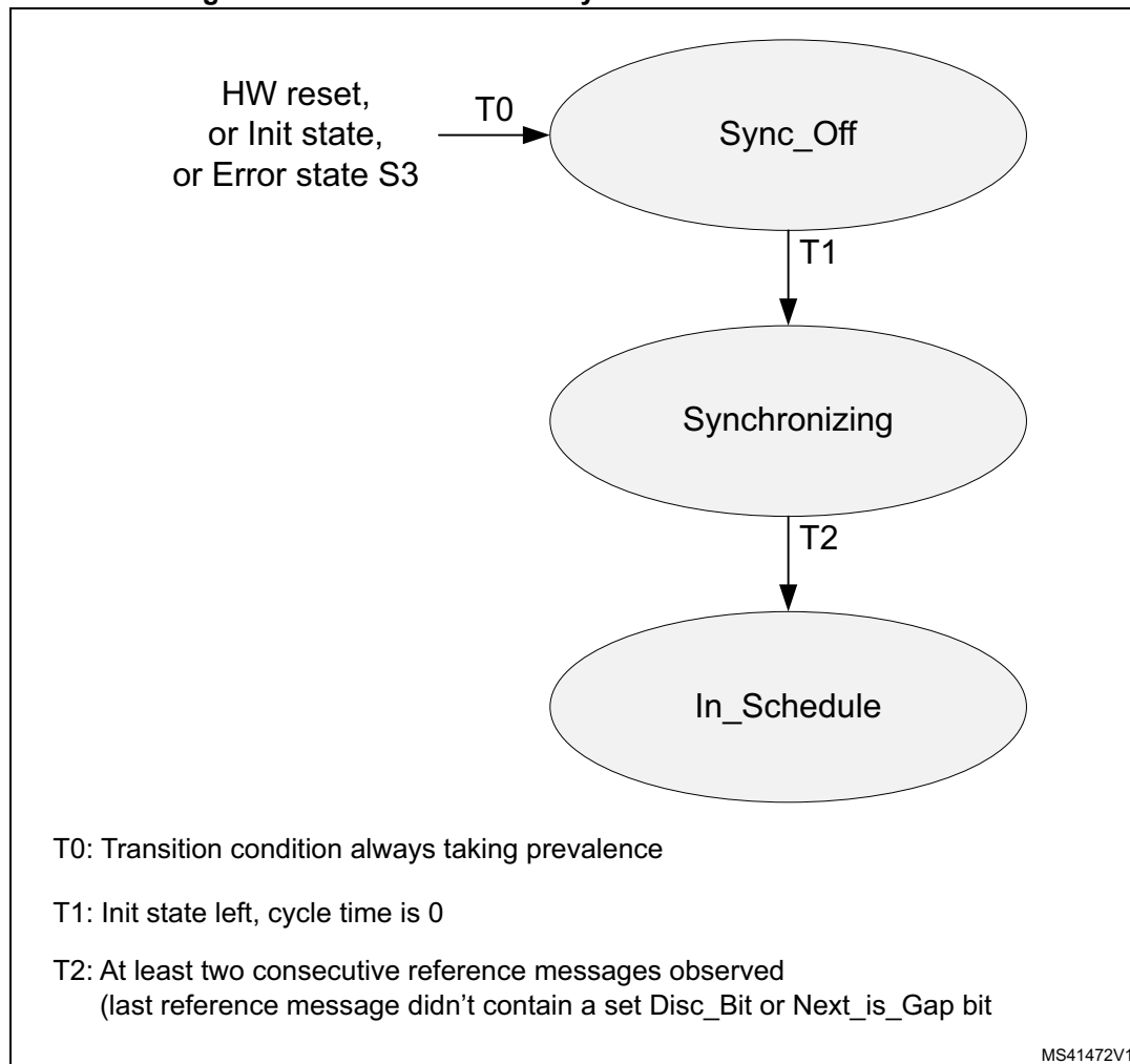
Figure 791. Level 0 schedule synchronization state machine
