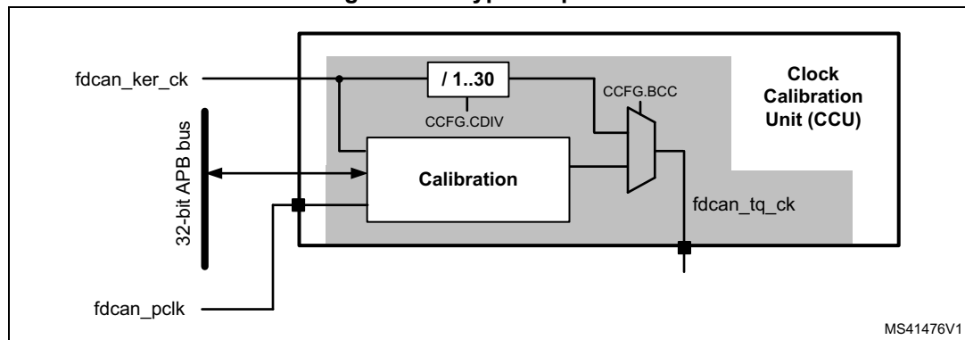
Figure 787. Bypass operation
