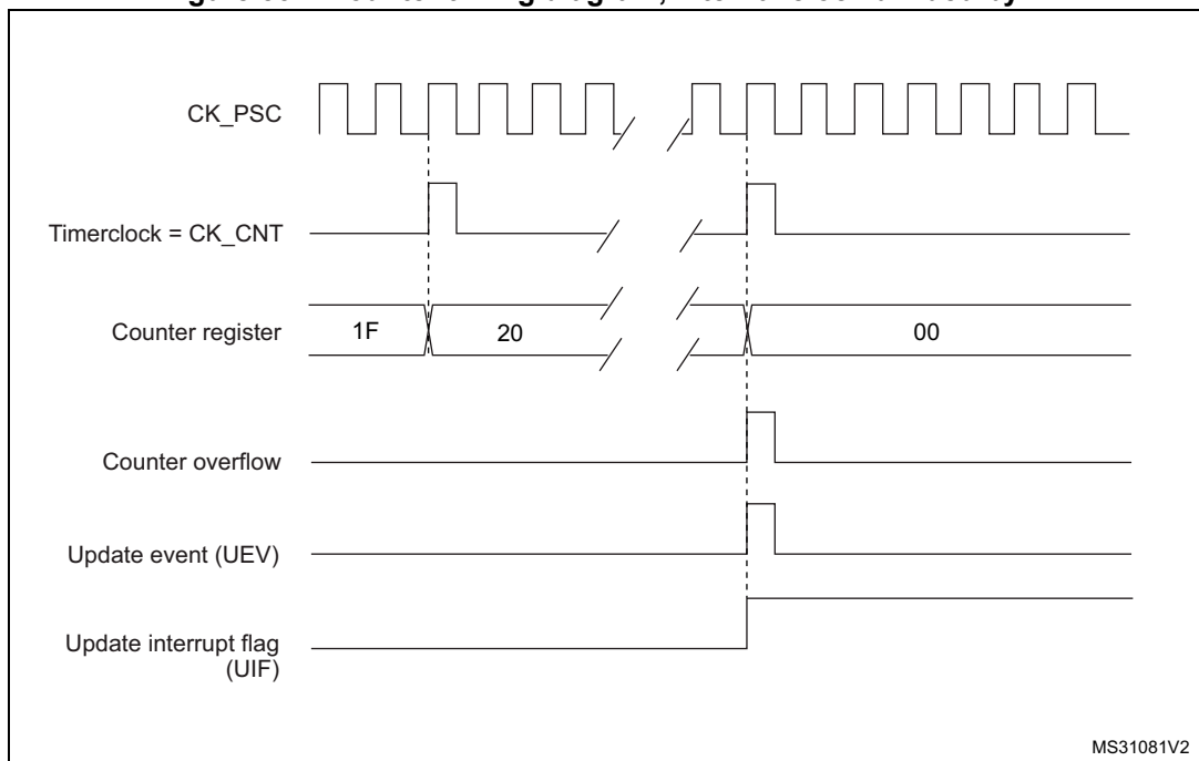
Figure 531. Counter timing diagram, internal clock divided by N
