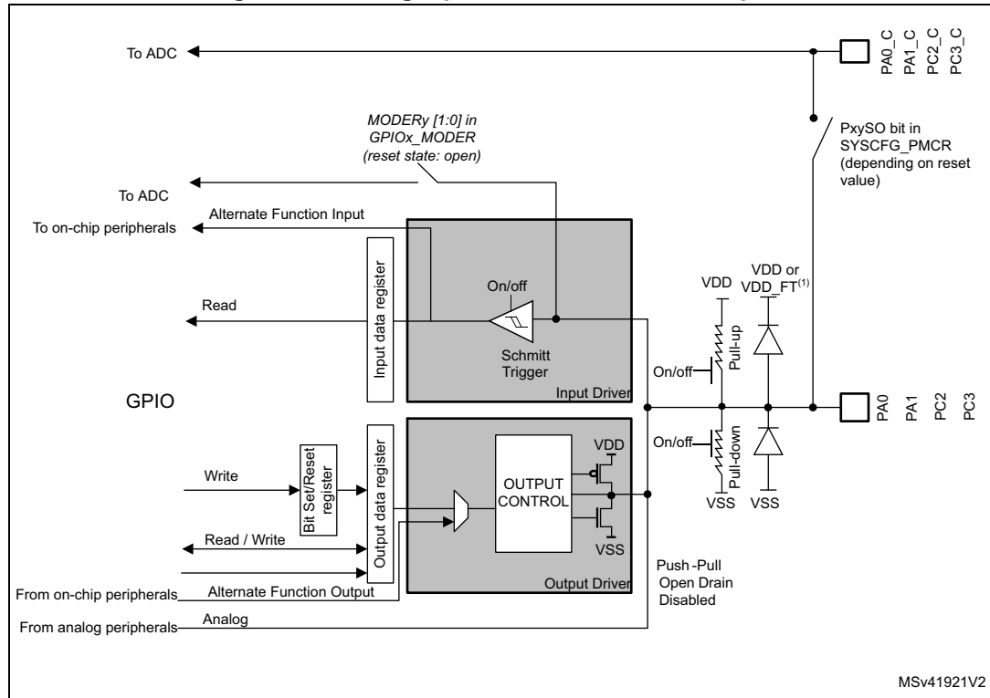
Figure 81. Analog inputs connected to ADC inputs
