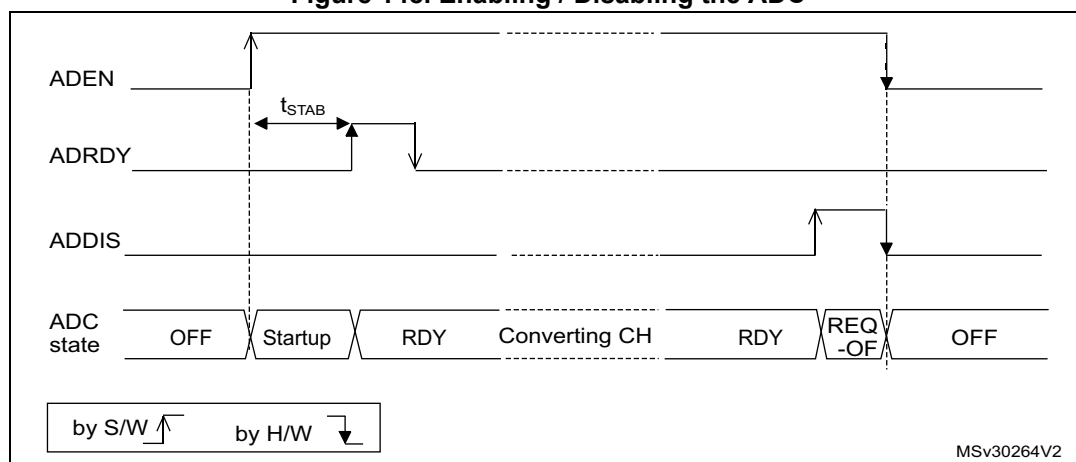
Figure 148. Enabling / Disabling the ADC
