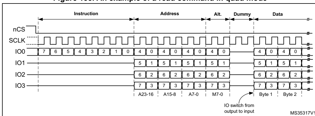
Figure 133. An example of a read command in quad mode
