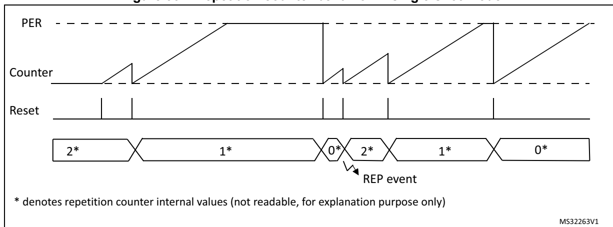
Figure 332. Repetition counter behavior in single-shot mode
