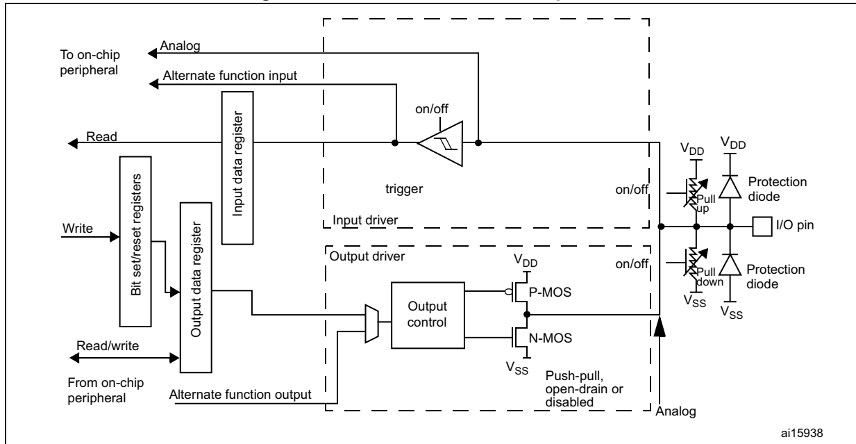
Figure 75. Basic structure of an I/O port bit
