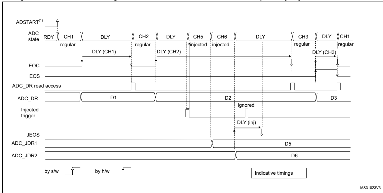
Figure 178. AUTDLY=1, regular continuous conversions interrupted by injected conversions
