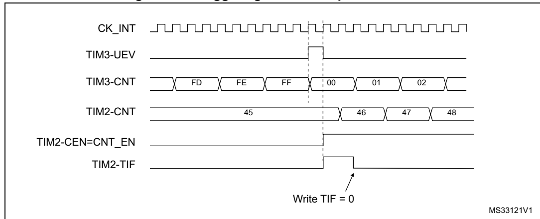
Figure 495. Triggering TIM2 with update of TIM3
