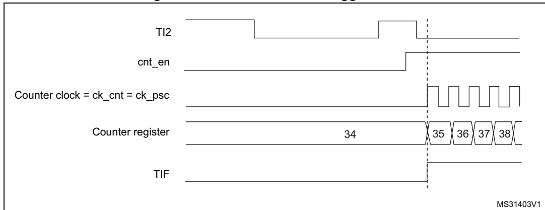
Figure 523. Control circuit in trigger mode
