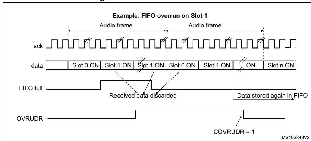
Figure 709. Overrun detection error
