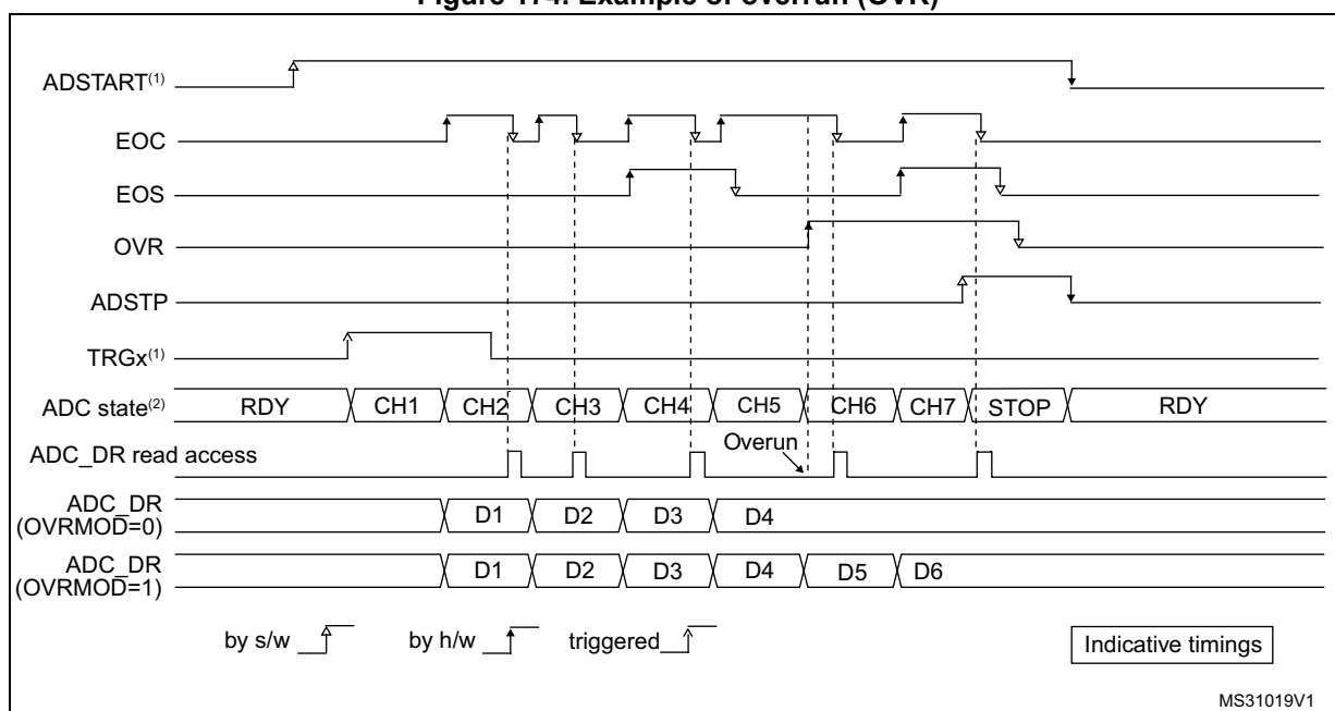
Figure 174. Example of overrun (OVR)
