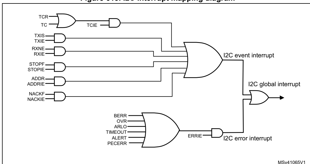
Figure 613. I2C interrupt mapping diagram
