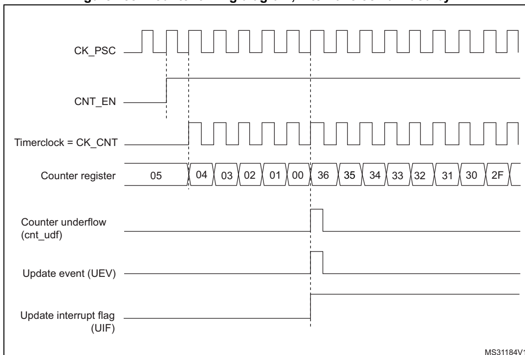
Figure 458. Counter timing diagram, internal clock divided by 1
