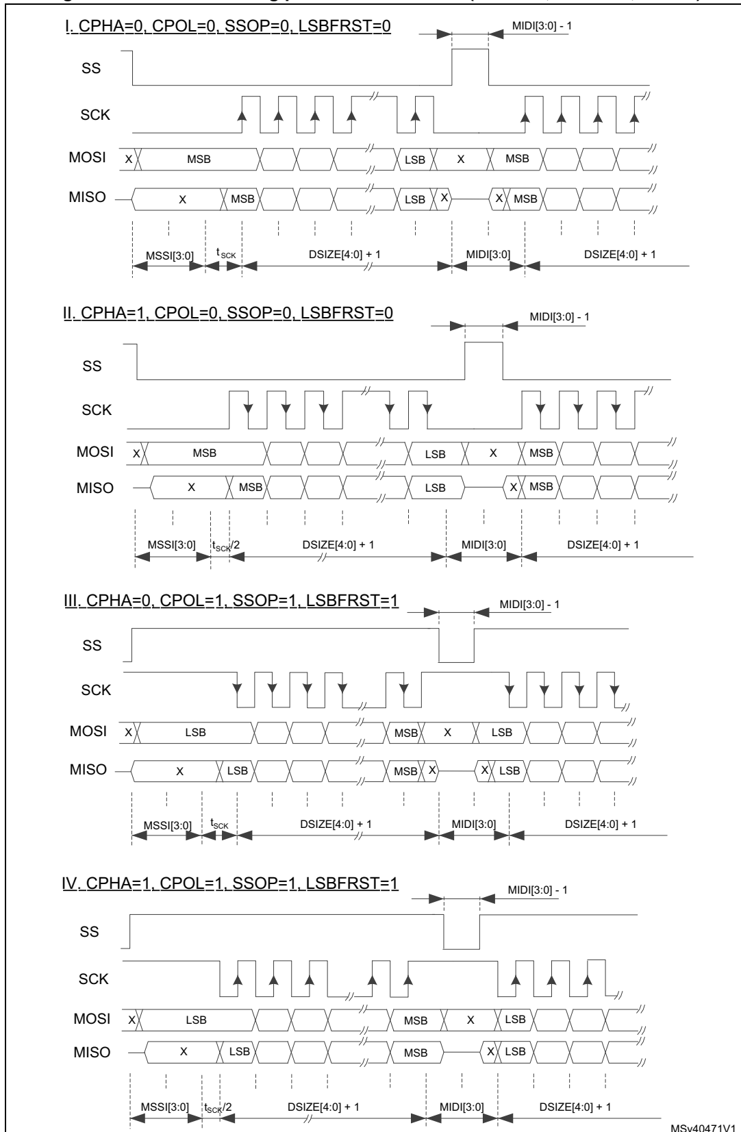
Figure 664. SS interleaving pulses between data (SSOE=1, SSOM=1,SSM=0)
