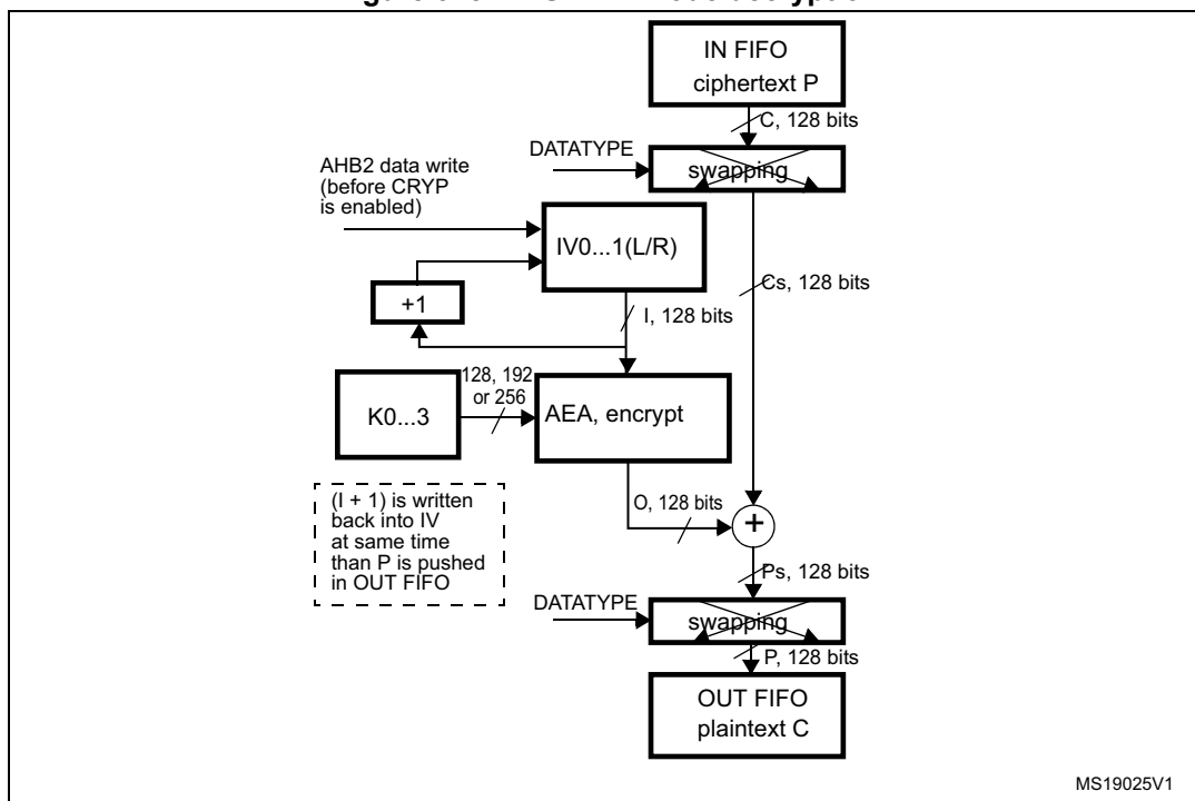
Figure 315. AES-CTR mode decryption
