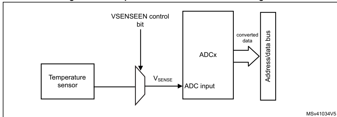
Figure 207. Temperature sensor channel block diagram
