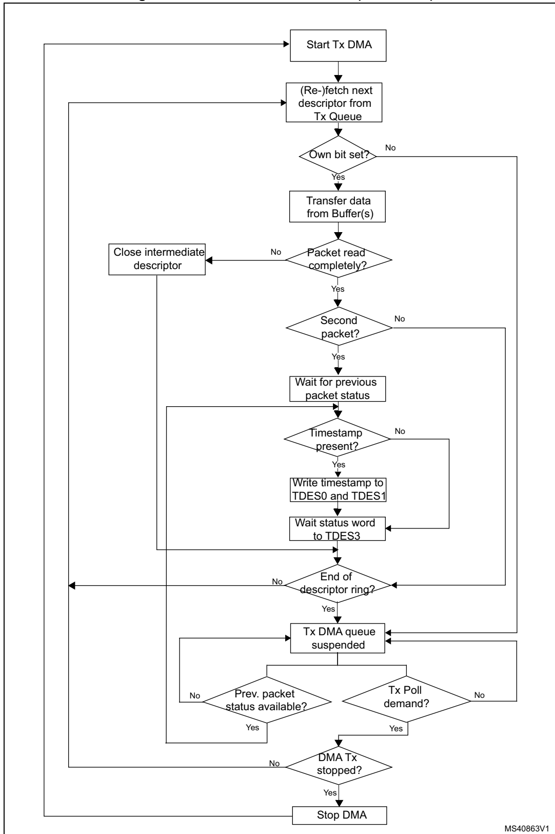
Figure 824. DMA transmission flow (OSP mode)
