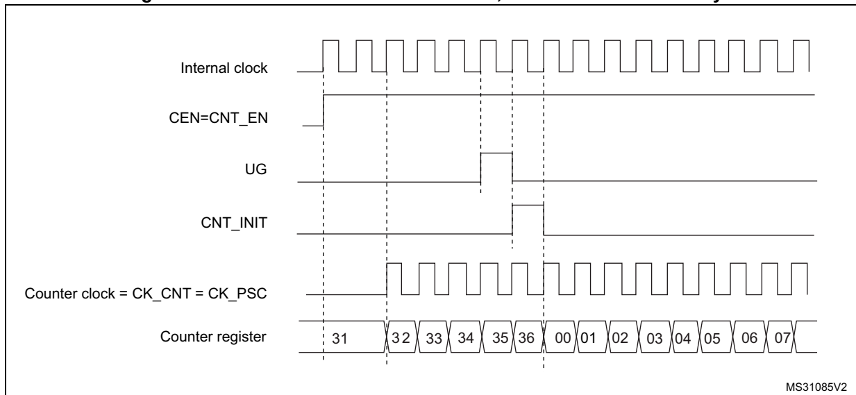
Figure 412. Control circuit in normal mode, internal clock divided by 1
