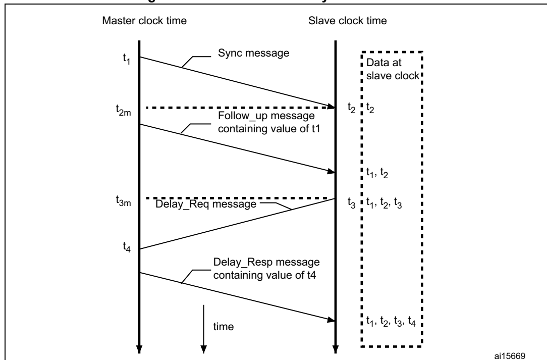
Figure 829. Networked time synchronization
