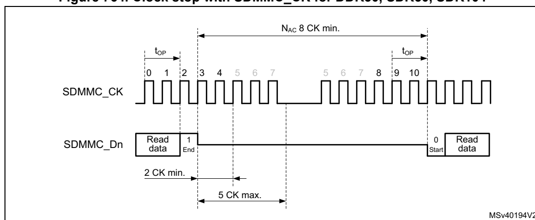
Figure 764. Clock stop with SDMMC_CK for DDR50, SDR50, SDR104
