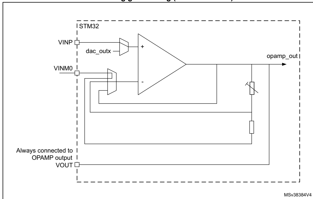
Figure 229. Example configuration
