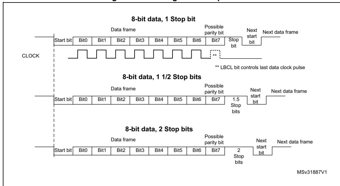
Figure 616. Configurable stop bits
