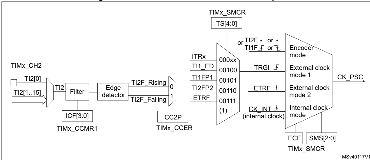
Figure 470. TI2 external clock connection example
