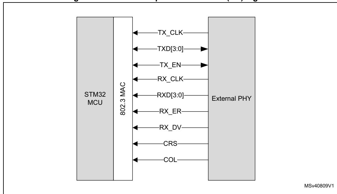
Figure 839. Media independent interface (MII) signals
