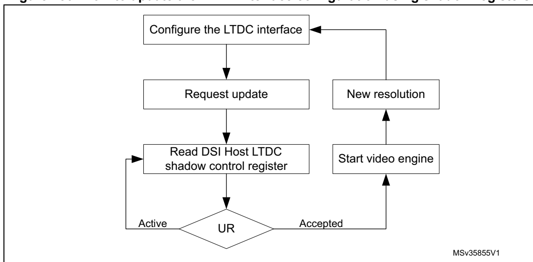
Figure 256. Flow to update the LTDC interface configuration using shadow registers
