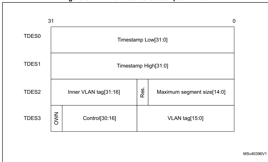
Figure 847. Transmit context descriptor format
