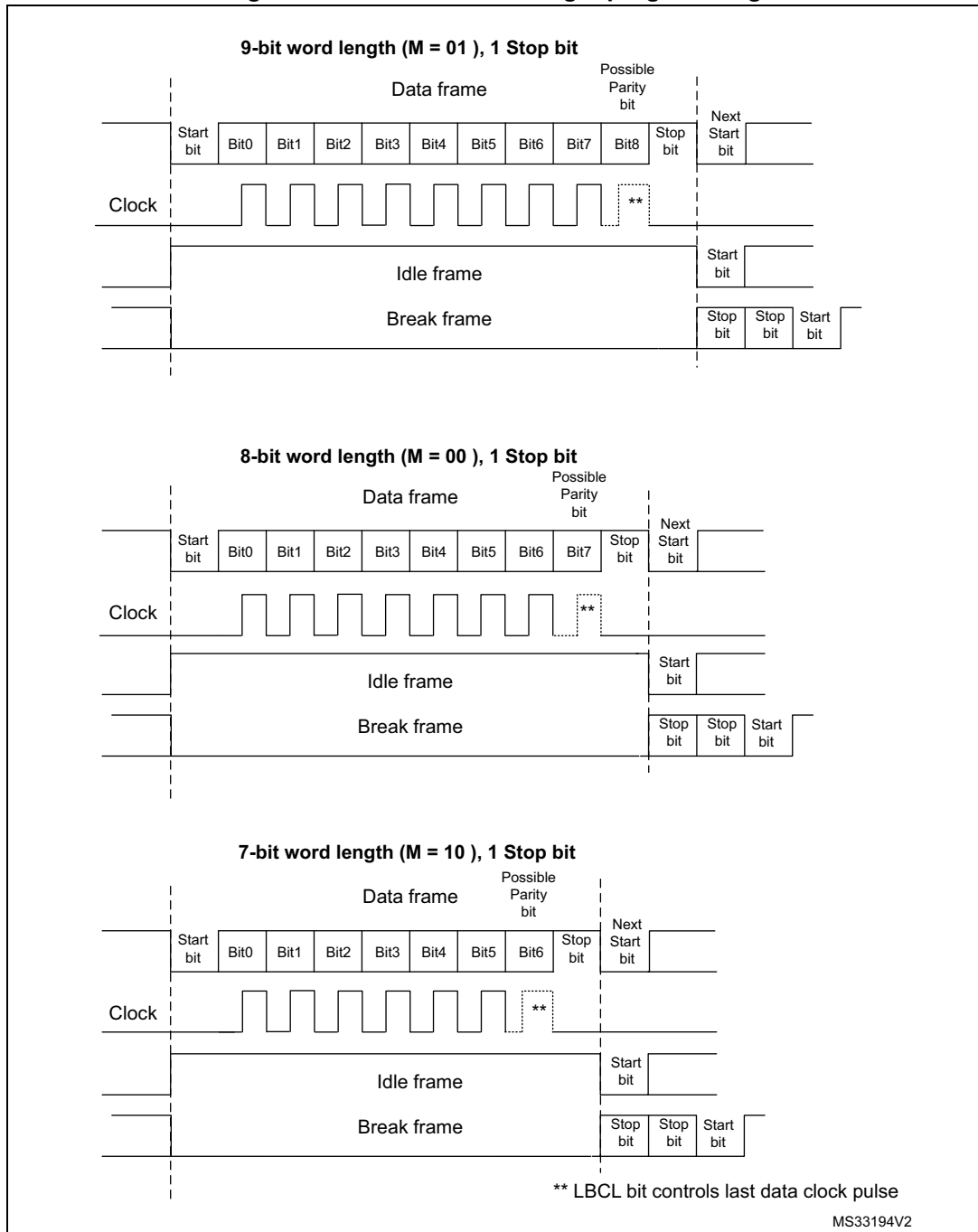
Figure 642. LPUART word length programming
