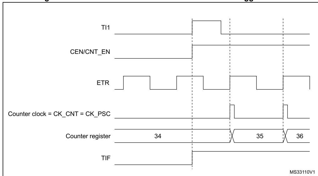
Figure 448. Control circuit in external clock mode 2 + trigger mode
