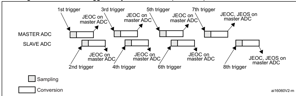
Figure 198. Alternate trigger: 4 injected channels (each ADC) in discontinuous mode
