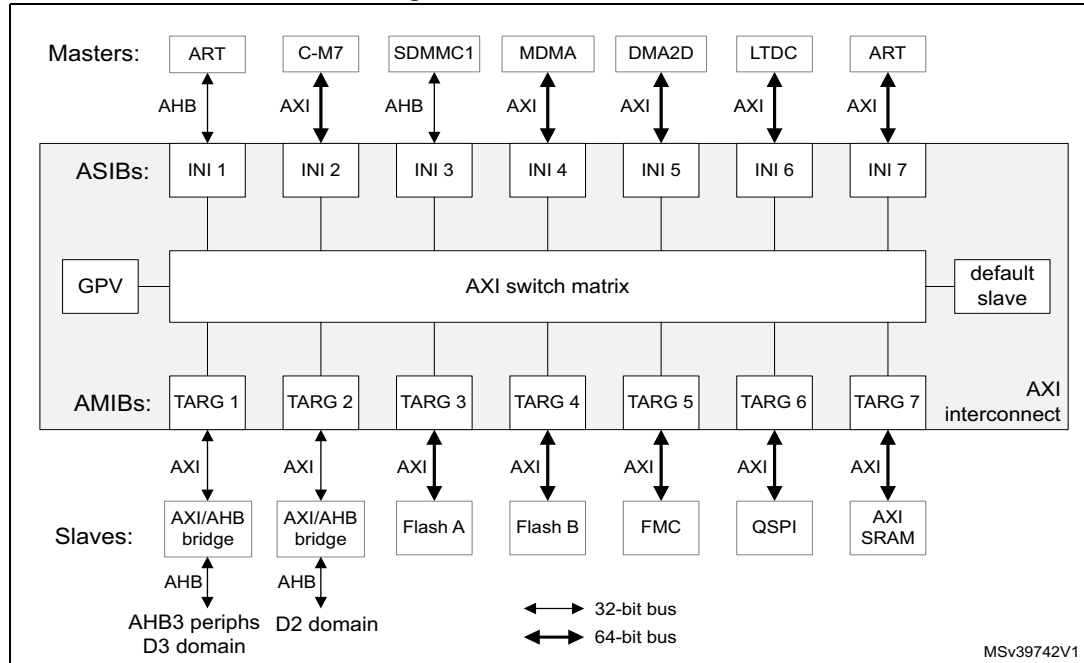
Figure 2. AXI interconnect
