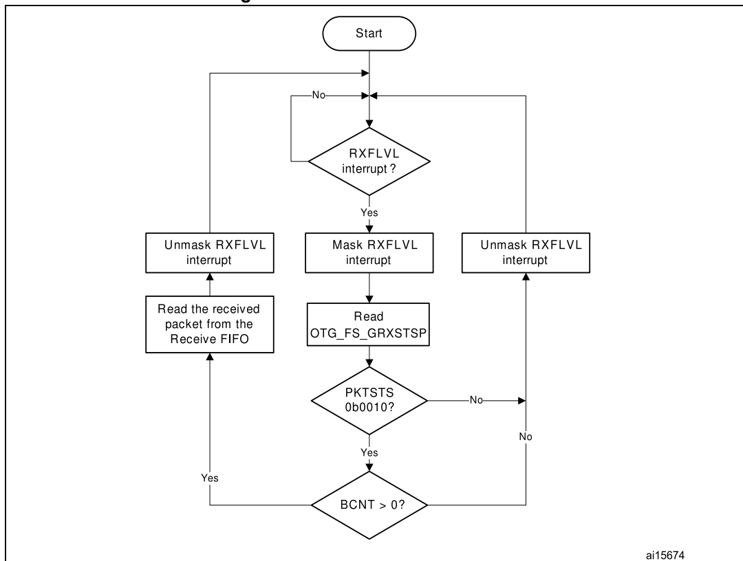
Figure 801. Receive FIFO read task
