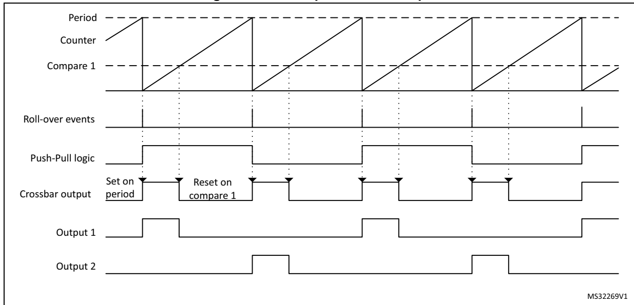
Figure 338. Push-pull mode example
