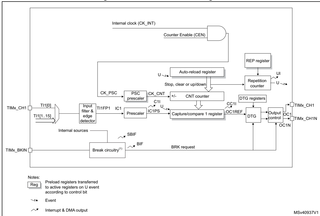
Figure 525. TIM16/TIM17 block diagram
