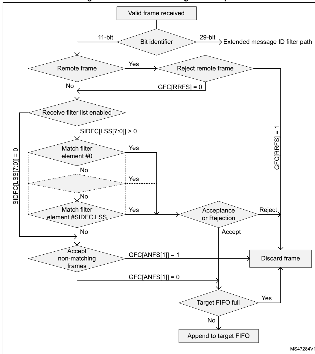
Figure 782. Standard message ID filter path
