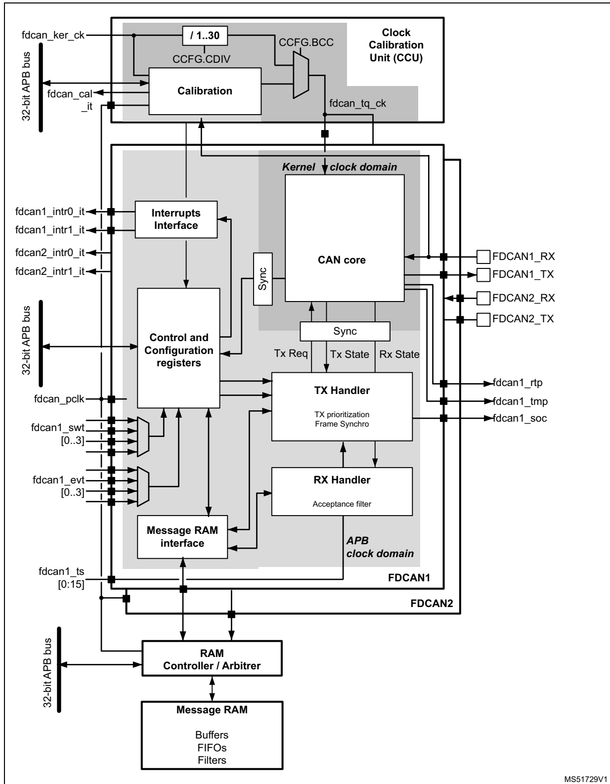
Figure 776. CAN subsystem
