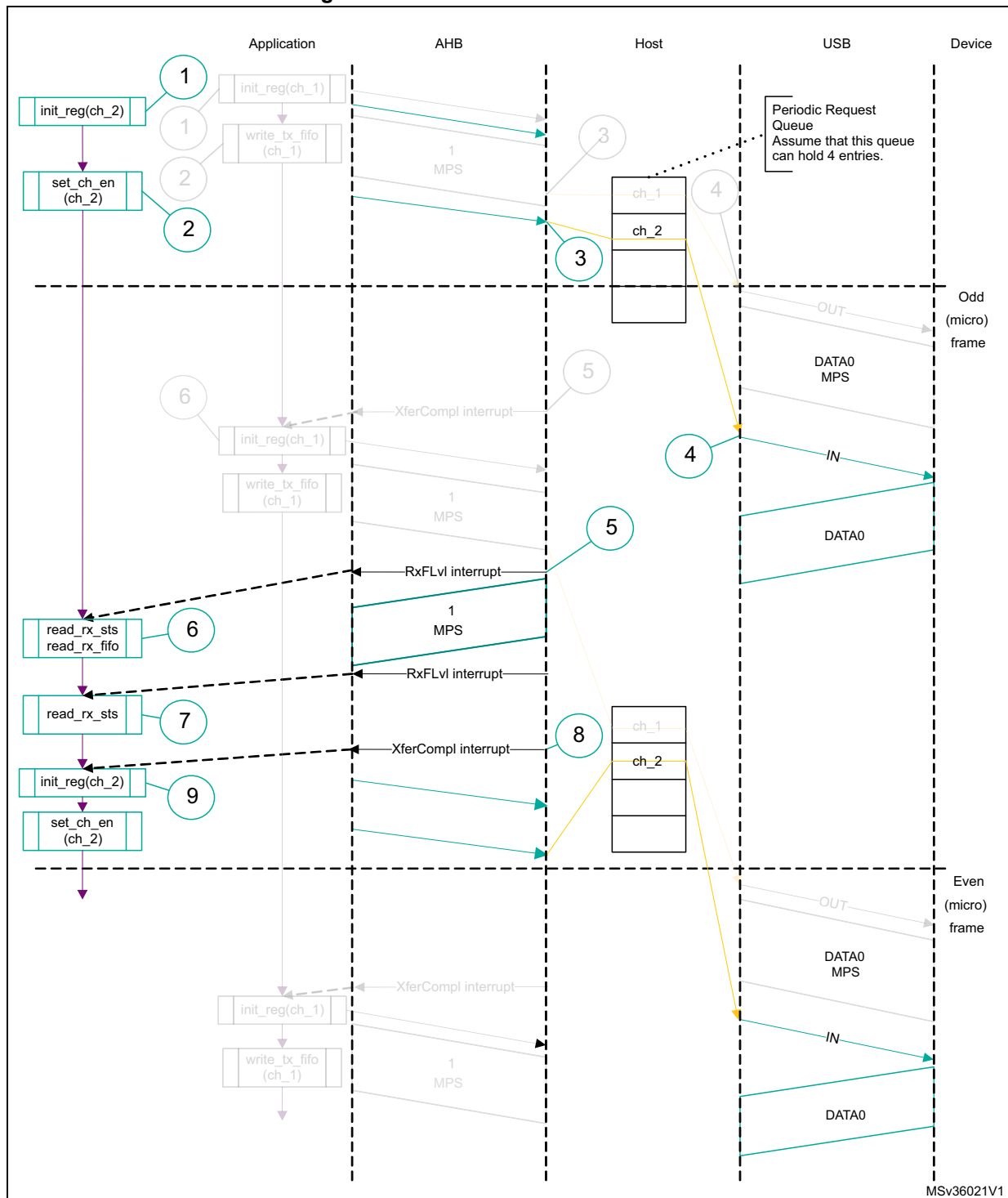
Figure 807. Isochronous IN transactions
