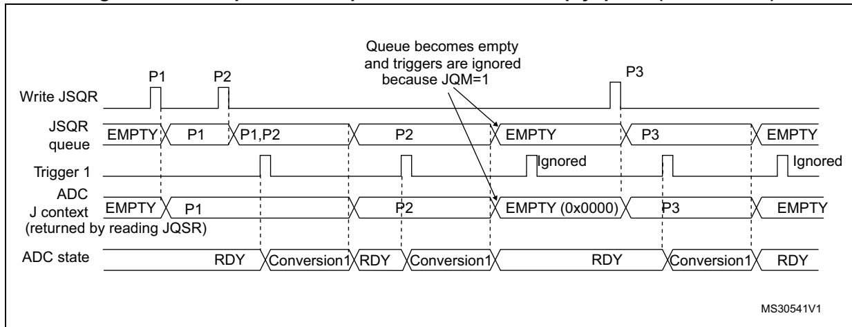
Figure 159. Example of JSQR queue of context with empty queue (case JQM=1)
