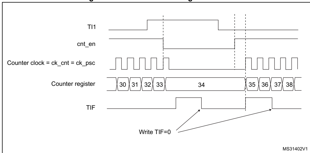
Figure 489. Control circuit in gated mode
