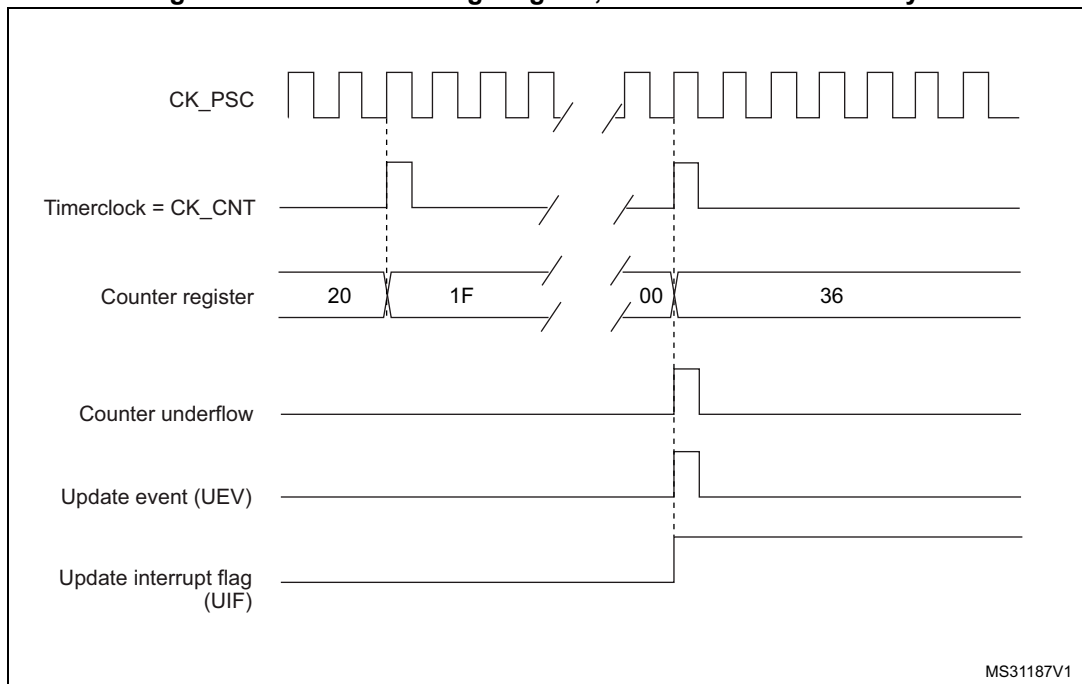
Figure 401. Counter timing diagram, internal clock divided by N
