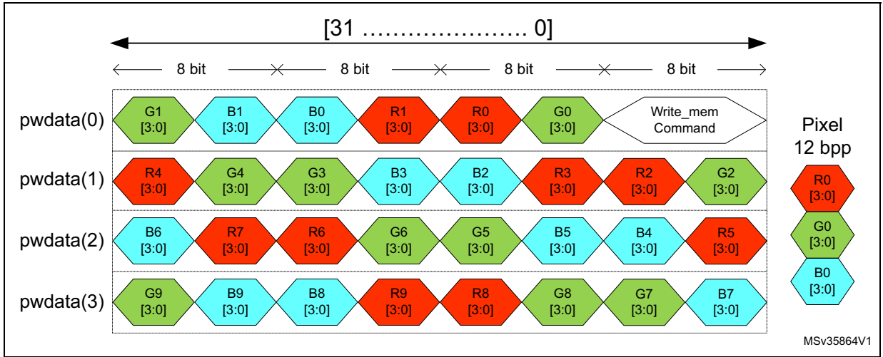
Figure 263. 12 bpp APB pixel to byte organization
