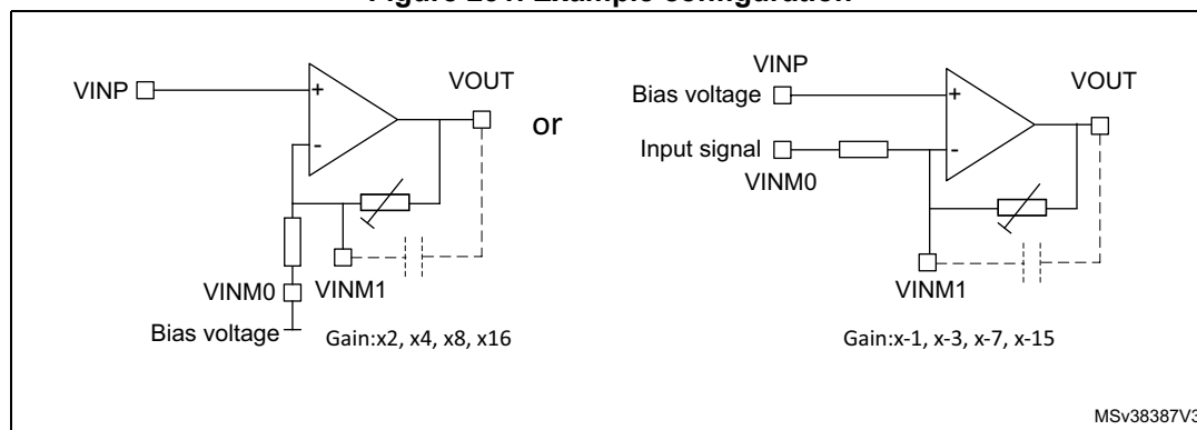
Figure 231. Example configuration
