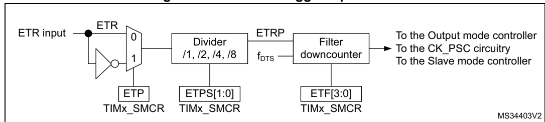
Figure 410. External trigger input block
