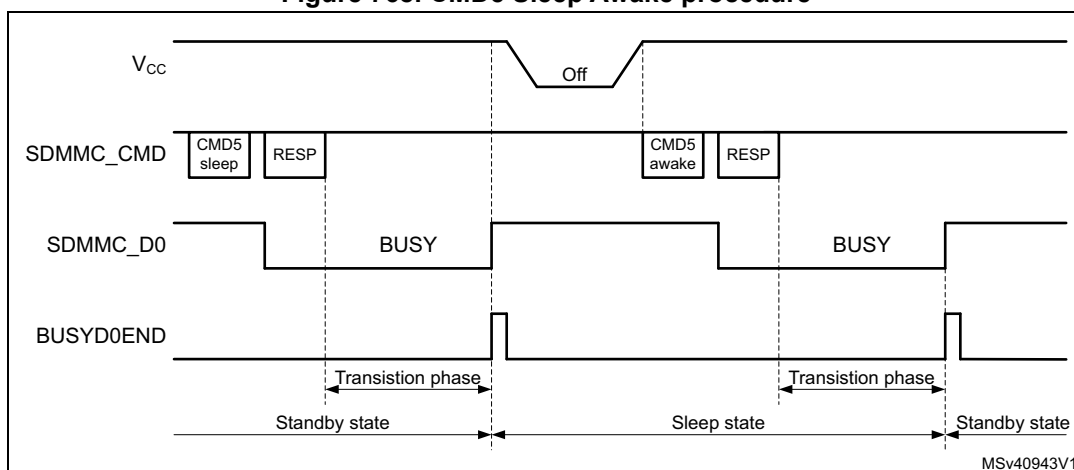
Figure 768. CMD5 Sleep Awake procedure
