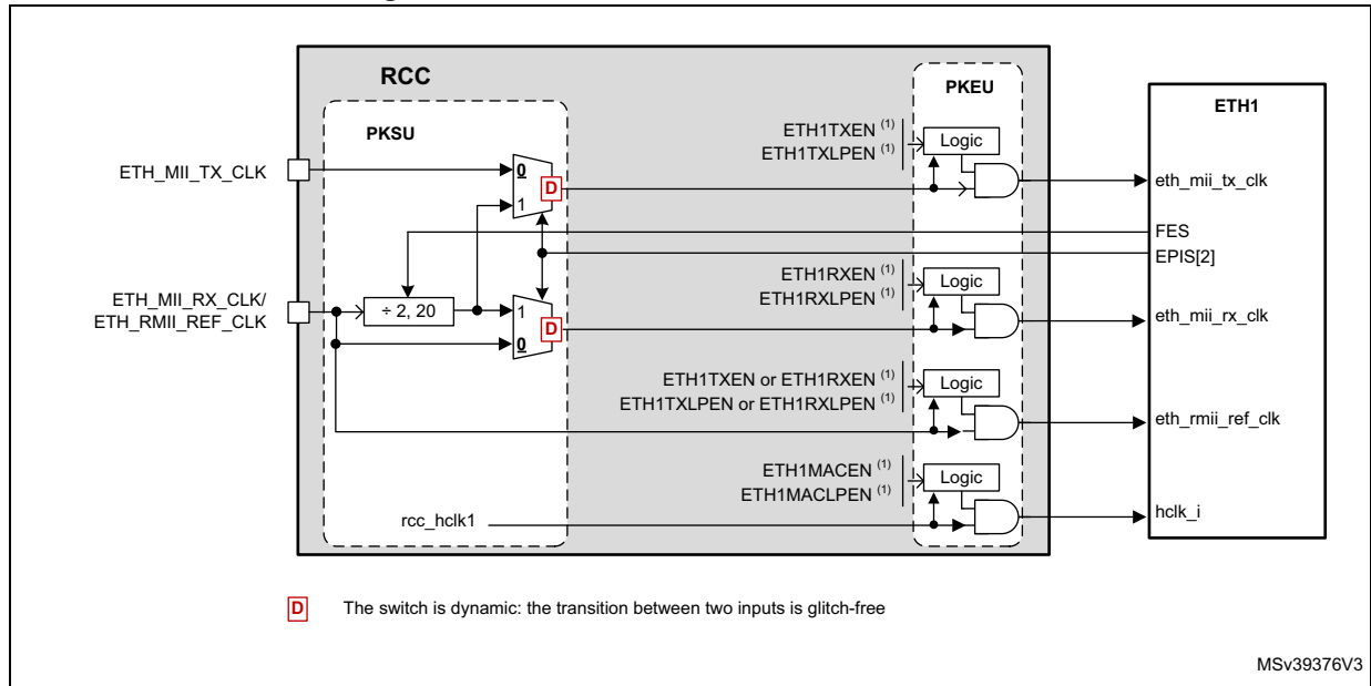
Figure 62. Kernel clock distribution for Ethernet
