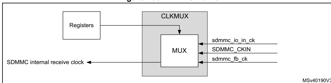
Figure 756. CLKMUX unit
