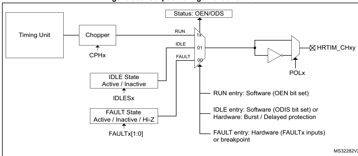
Figure 360. Output management overview
