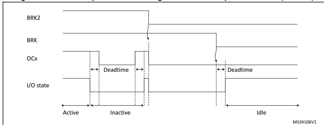
Figure 434. PWM output state following BRK and BRK2 pins assertion ( OSSI=1 )
