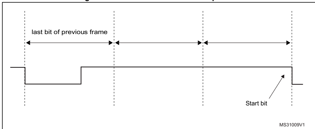
Figure 858. SFT of three nominal bit periods
