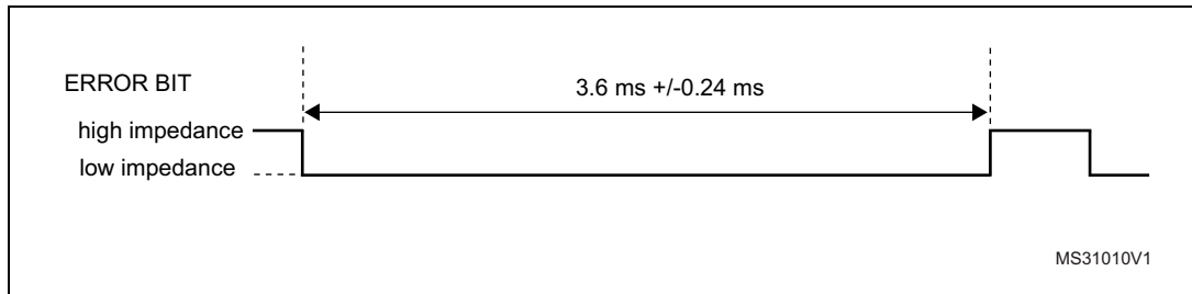
Figure 859. Error bit timing
