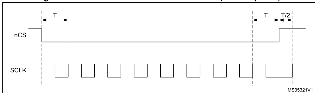
Figure 137. nCS when CKMODE = 1 in DDR mode (T = CLK period)
