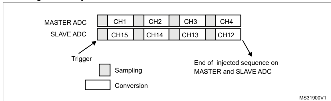
Figure 192. Injected simultaneous mode on 4 channels: dual ADC mode
