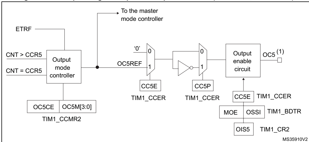
Figure 421. Output stage of capture/compare channel (channel 5, idem ch. 6)
