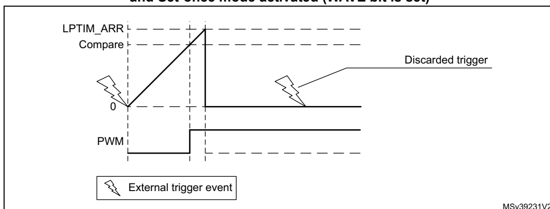
Figure 572. LPTIM output waveform, Single counting mode configuration and Set-once mode activated (WAVE bit is set)
