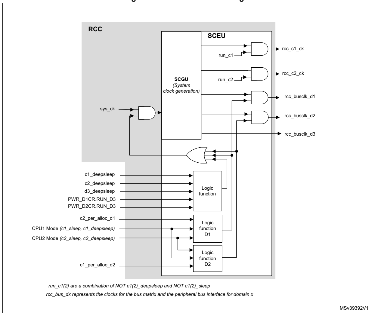
Figure 68. Bus clock enable logic
