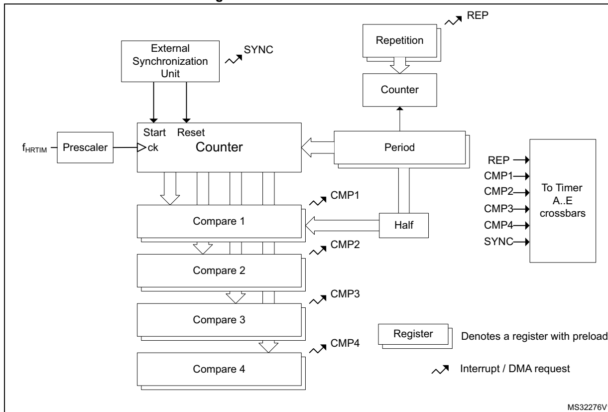
Figure 345. Master timer overview
