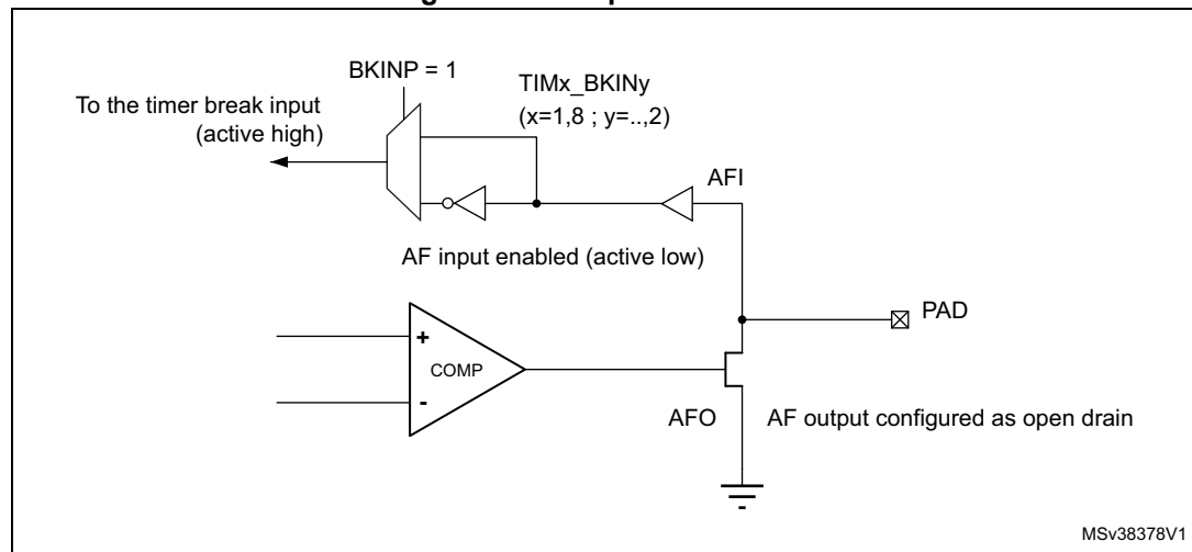
Figure 222. Output redirection
