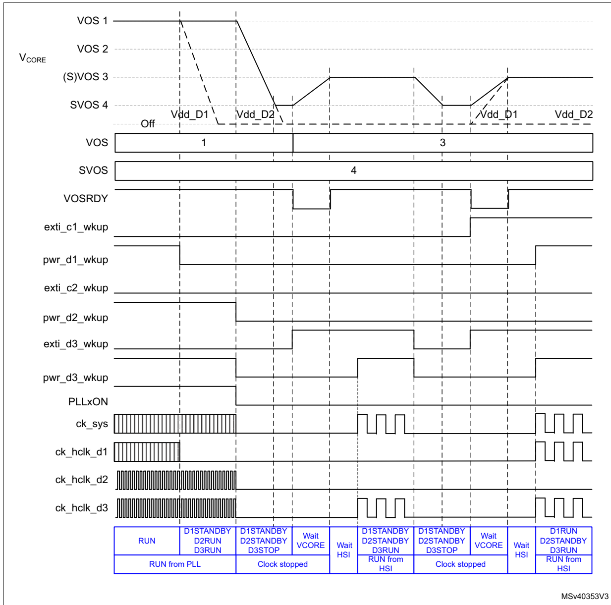
Figure 41. Dynamic voltage scaling behavior with D1 and D2 in DStandby mode and D3 in autonomous mode
