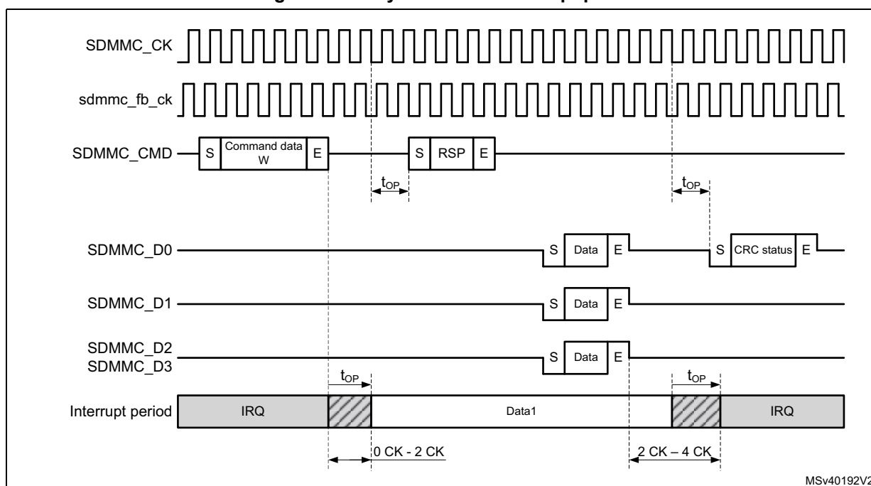
Figure 762. Asynchronous interrupt period data write
