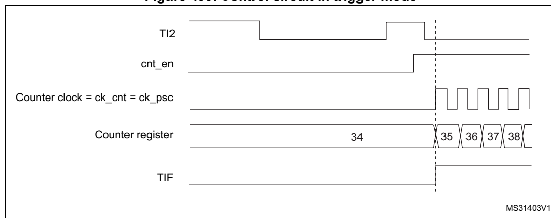
Figure 490. Control circuit in trigger mode
