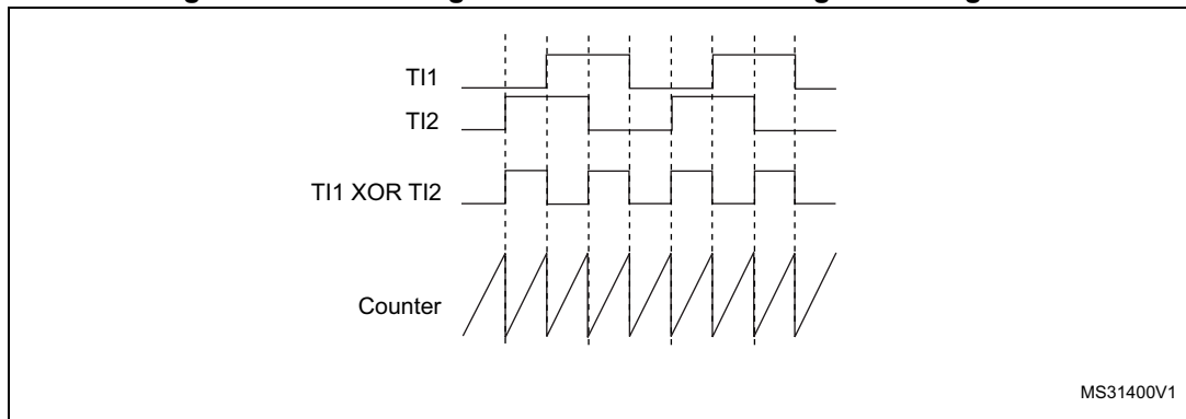
Figure 553. Measuring time interval between edges on 2 signals
