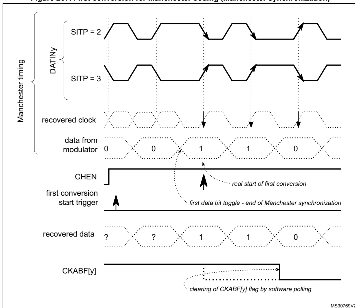
Figure 237. First conversion for Manchester coding (Manchester synchronization)
