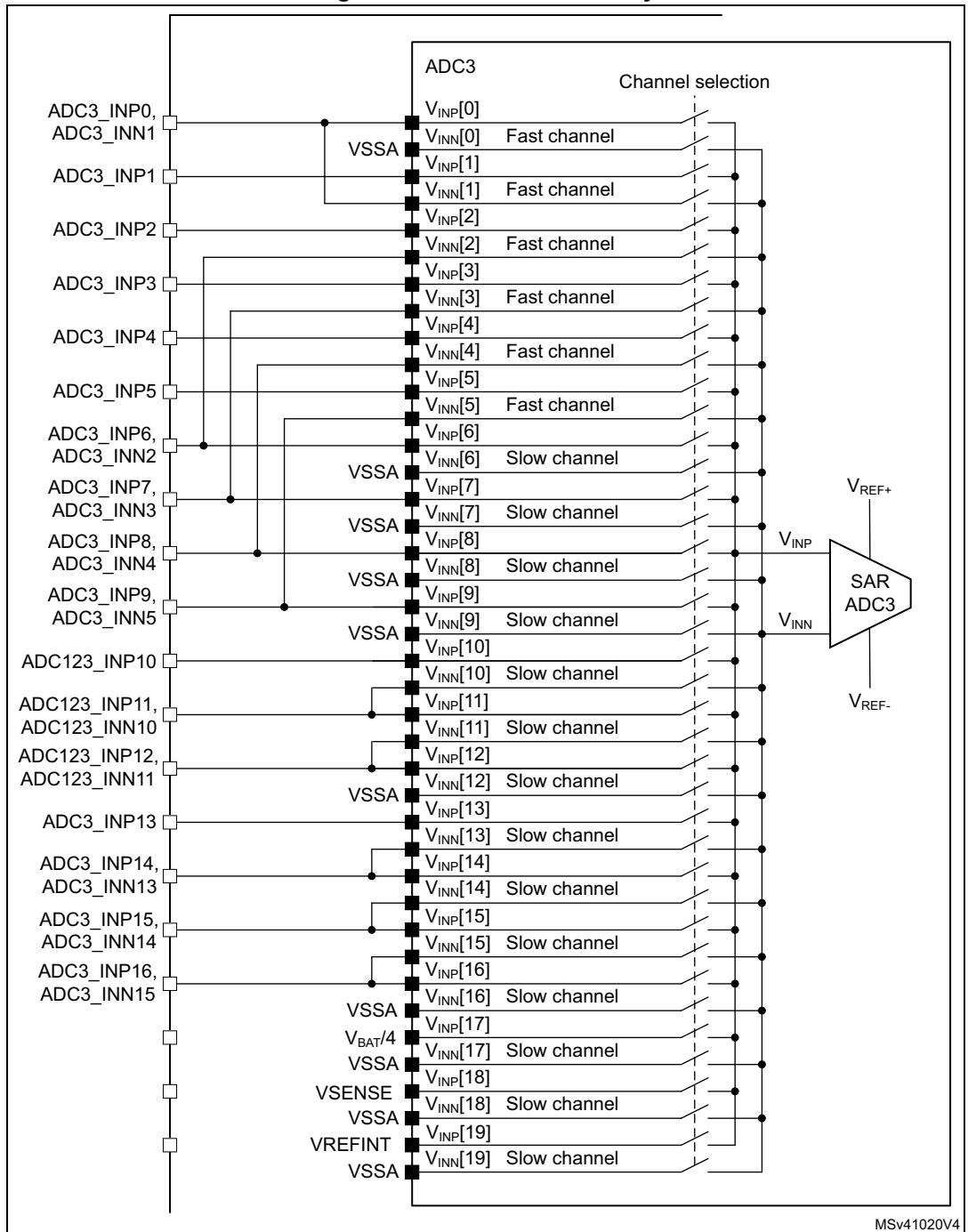
Figure 144. ADC3 connectivity
