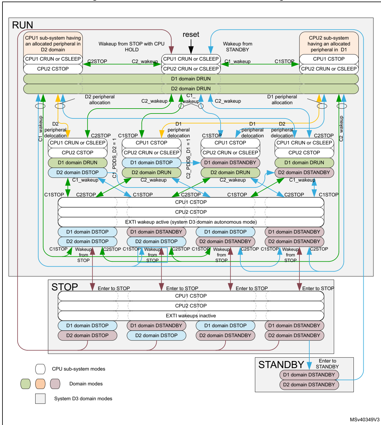
Figure 37. Power control modes detailed state diagram
