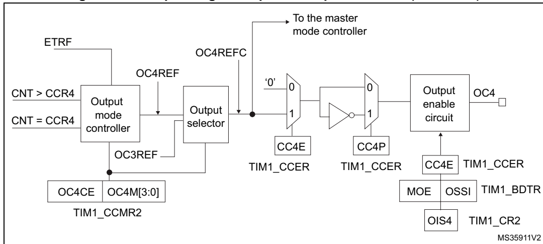
Figure 420. Output stage of capture/compare channel (channel 4)
