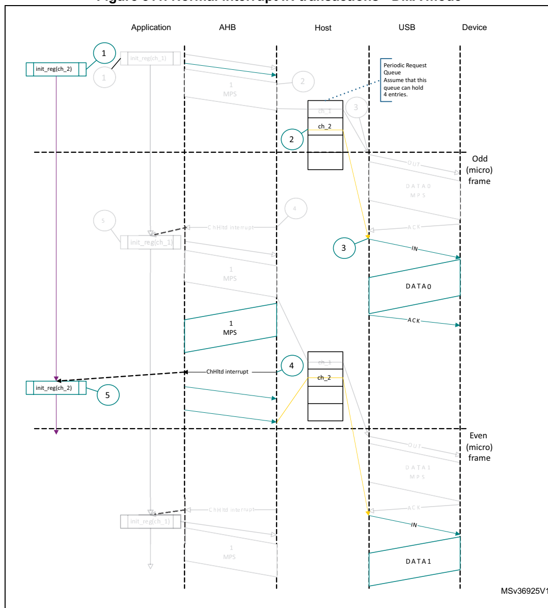
Figure 811. Normal interrupt IN transactions - DMA mode
