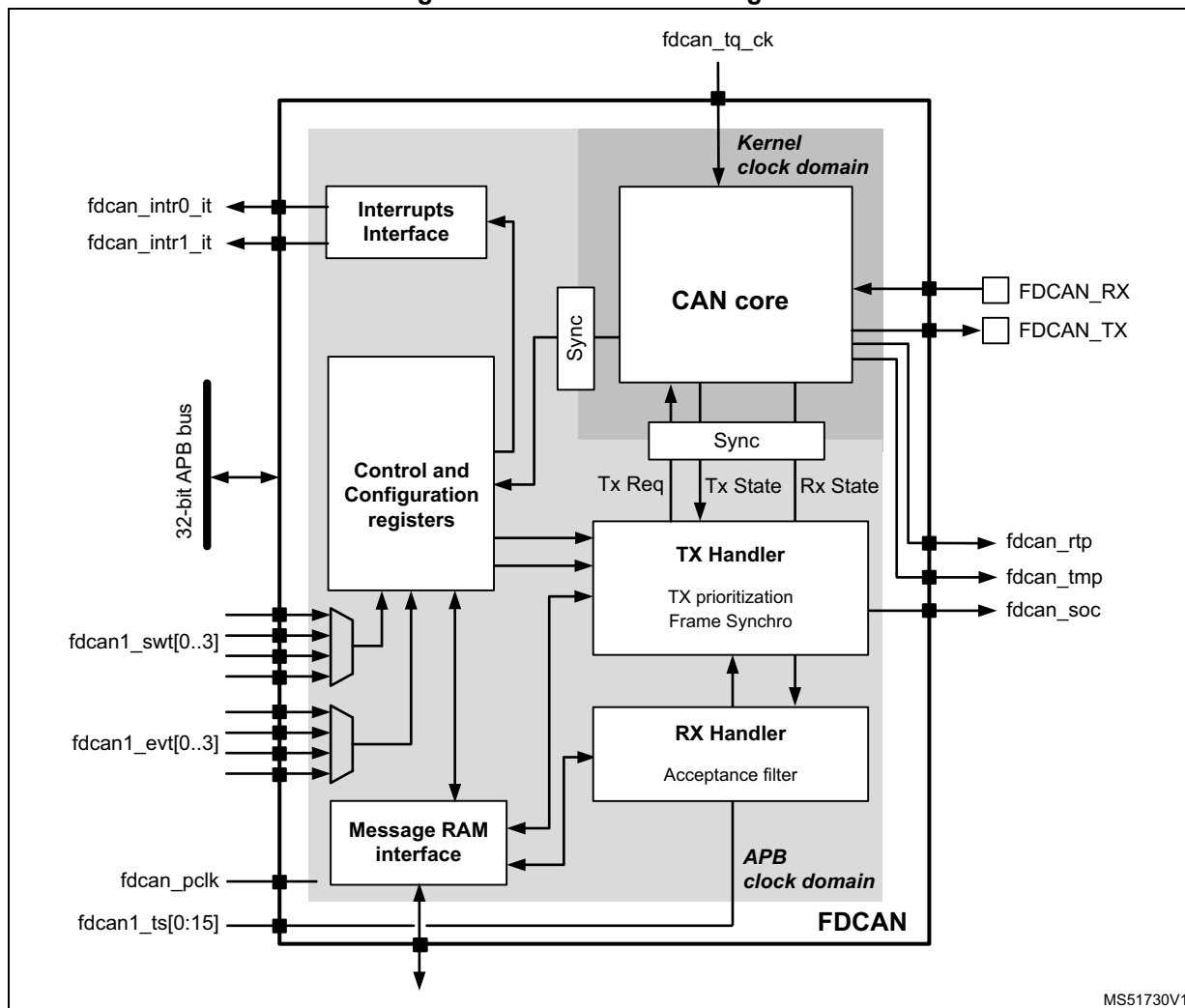
Figure 777. FDCAN block diagram
