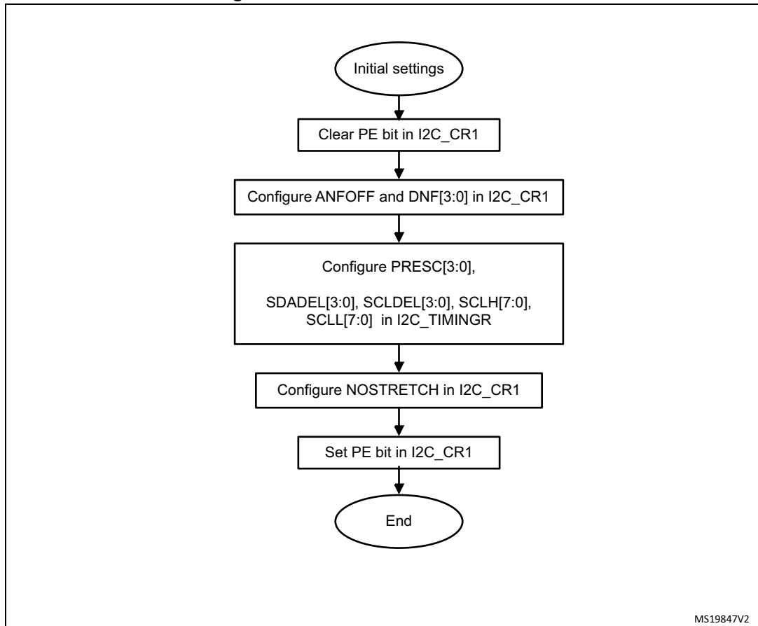
Figure 586. I2C initialization flowchart
