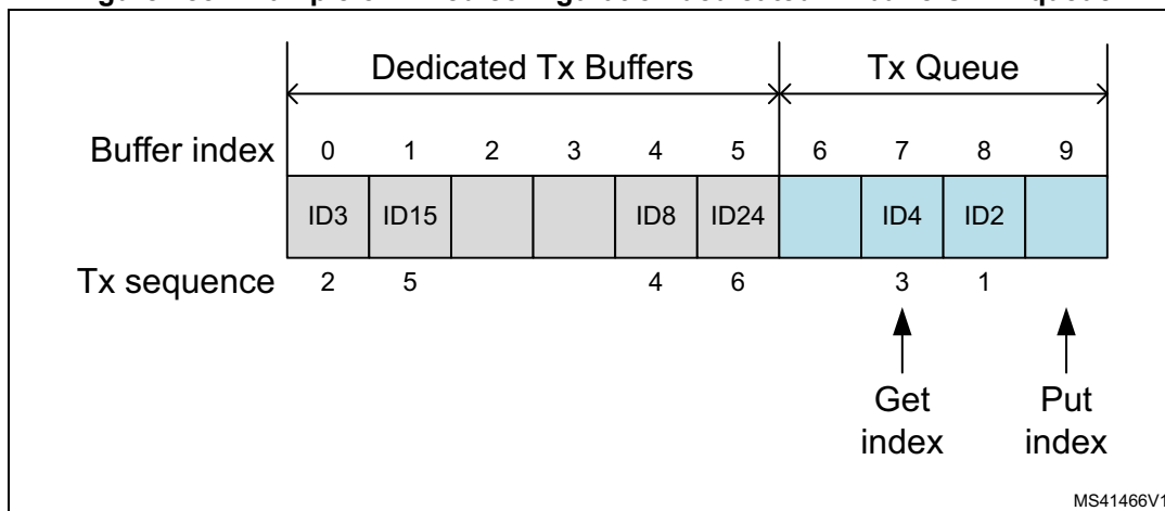
Figure 785. Example of mixed configuration dedicated Tx buffers / Tx queue
