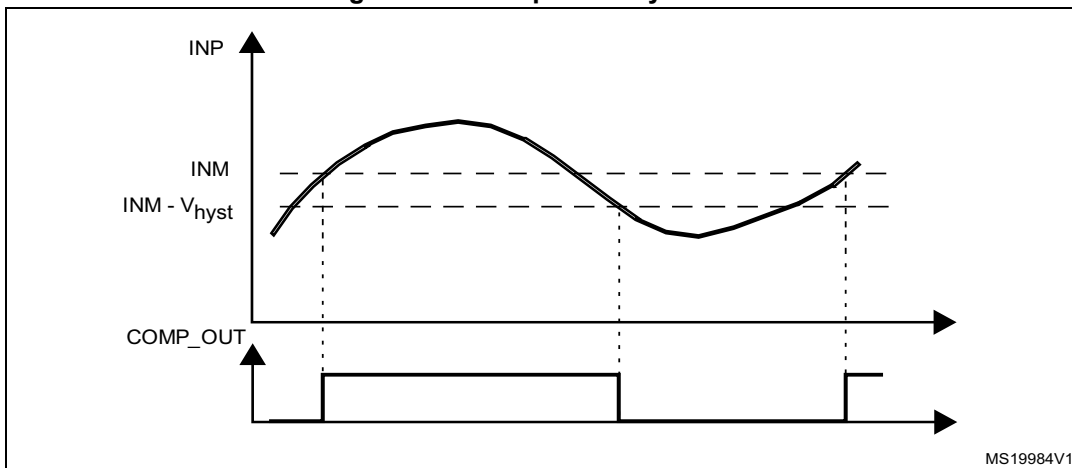
Figure 220. Comparator hysteresis
