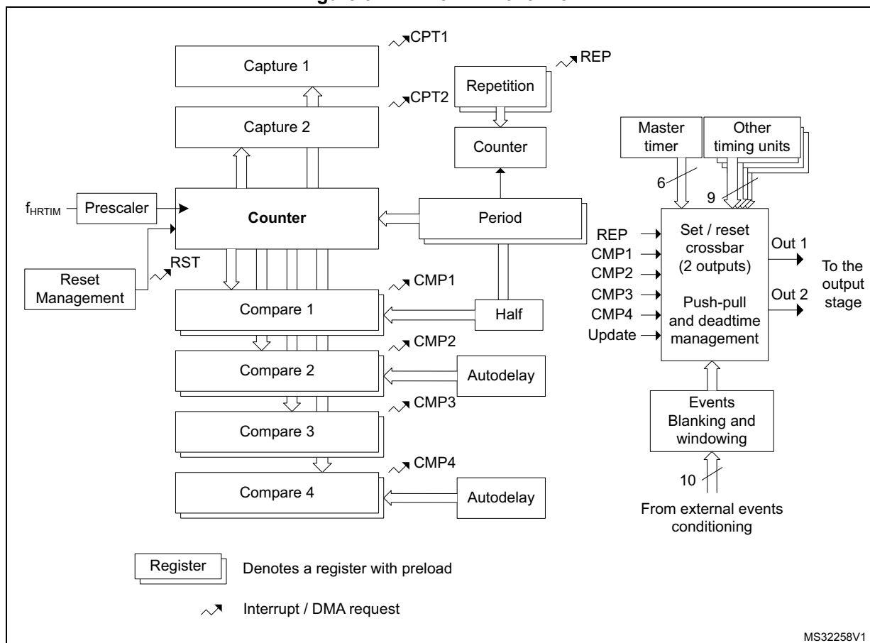
Figure 327. Timer A..E overview
