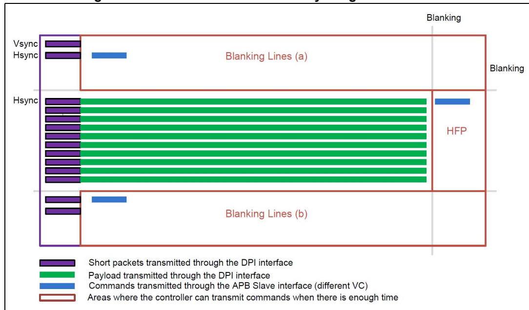
Figure 280. Command transmission by the generic interface
