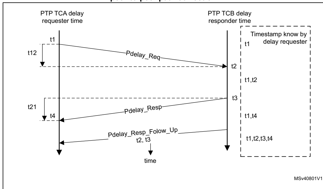
Figure 830. Propagation delay calculation in clocks supporting peer-to-peer path correction
