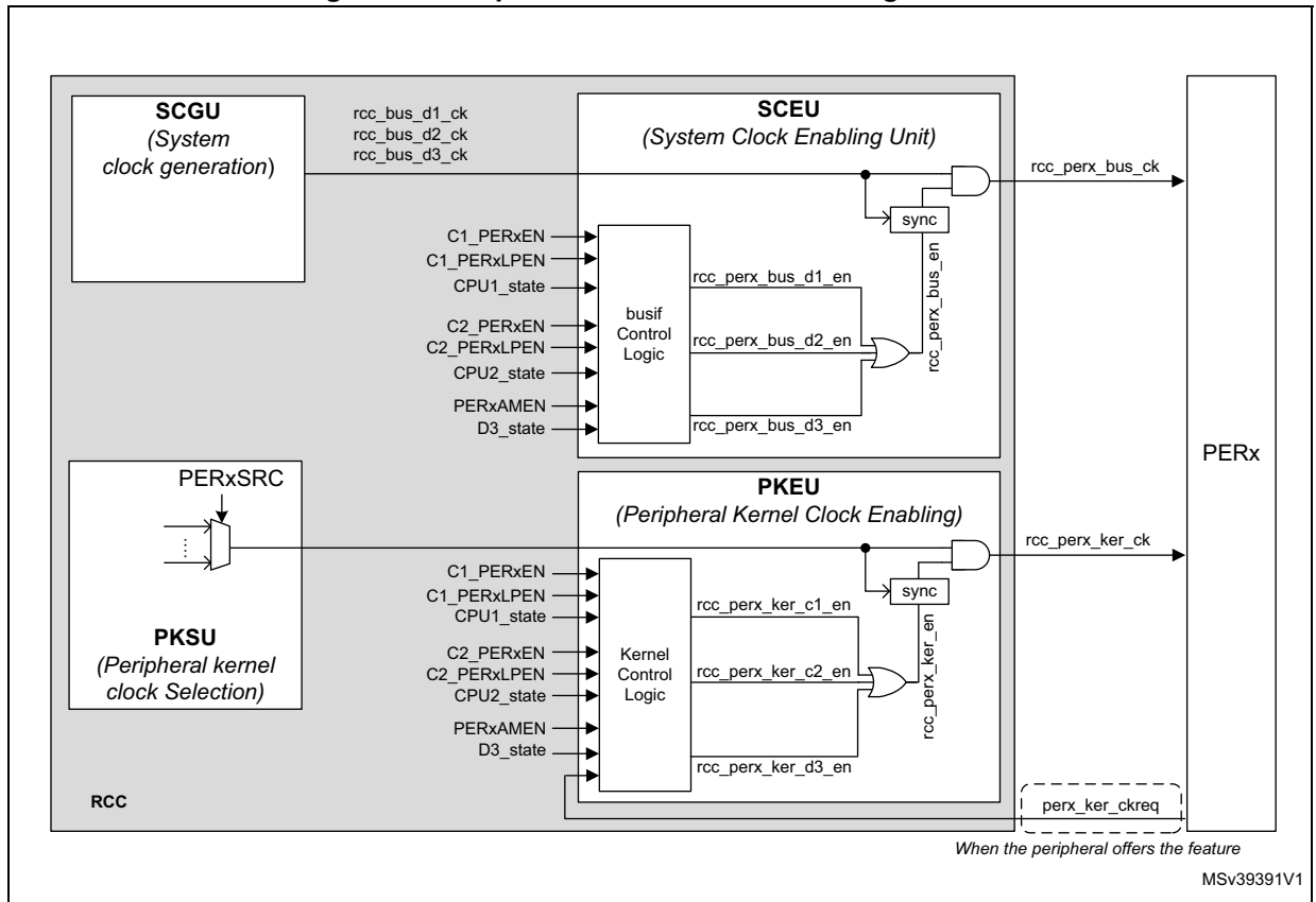
Figure 67. Peripheral kernel clock enable logic details
