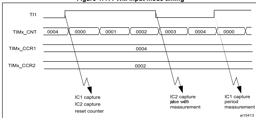
Figure 477. PWM input mode timing
