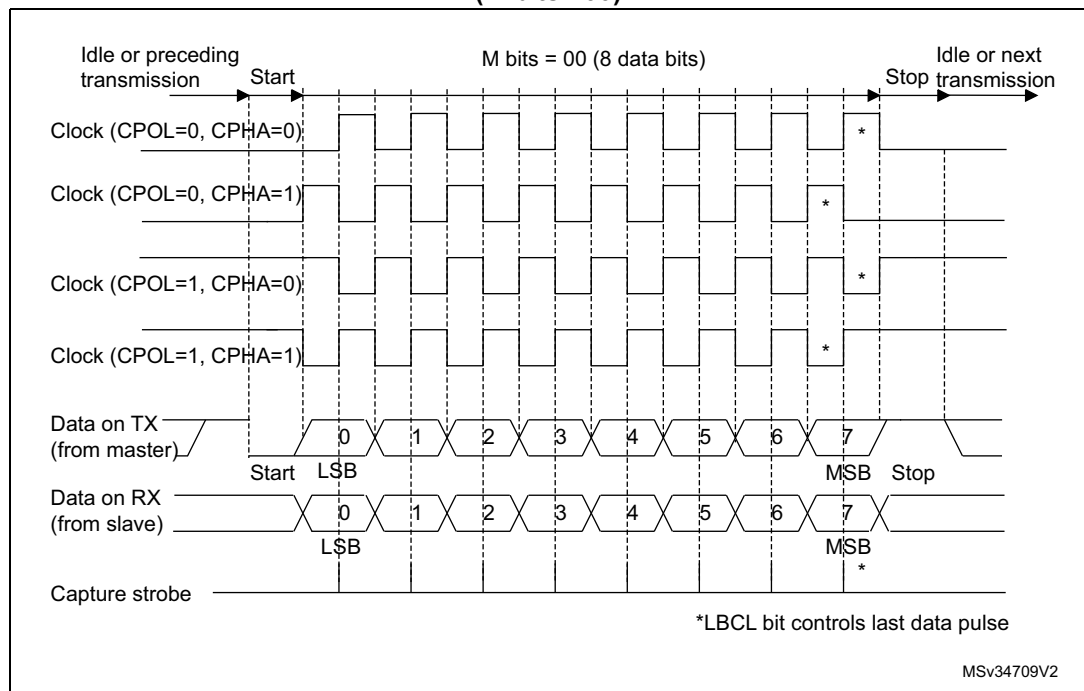
Figure 627. USART data clock timing diagram in synchronous master mode (M bits =00)
