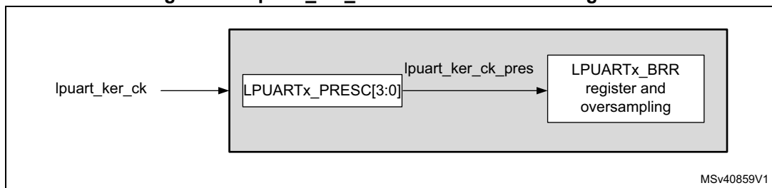
Figure 645. lpuart_ker_ck clock divider block diagram
