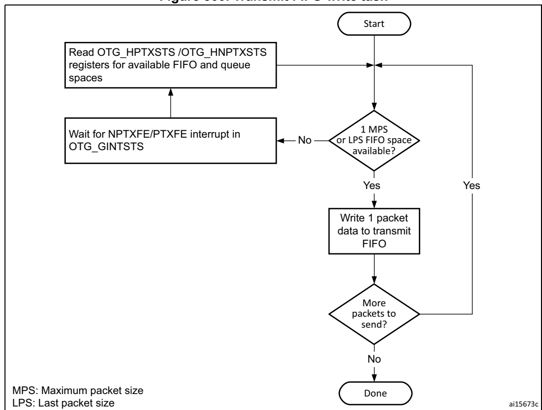
Figure 800. Transmit FIFO write task
