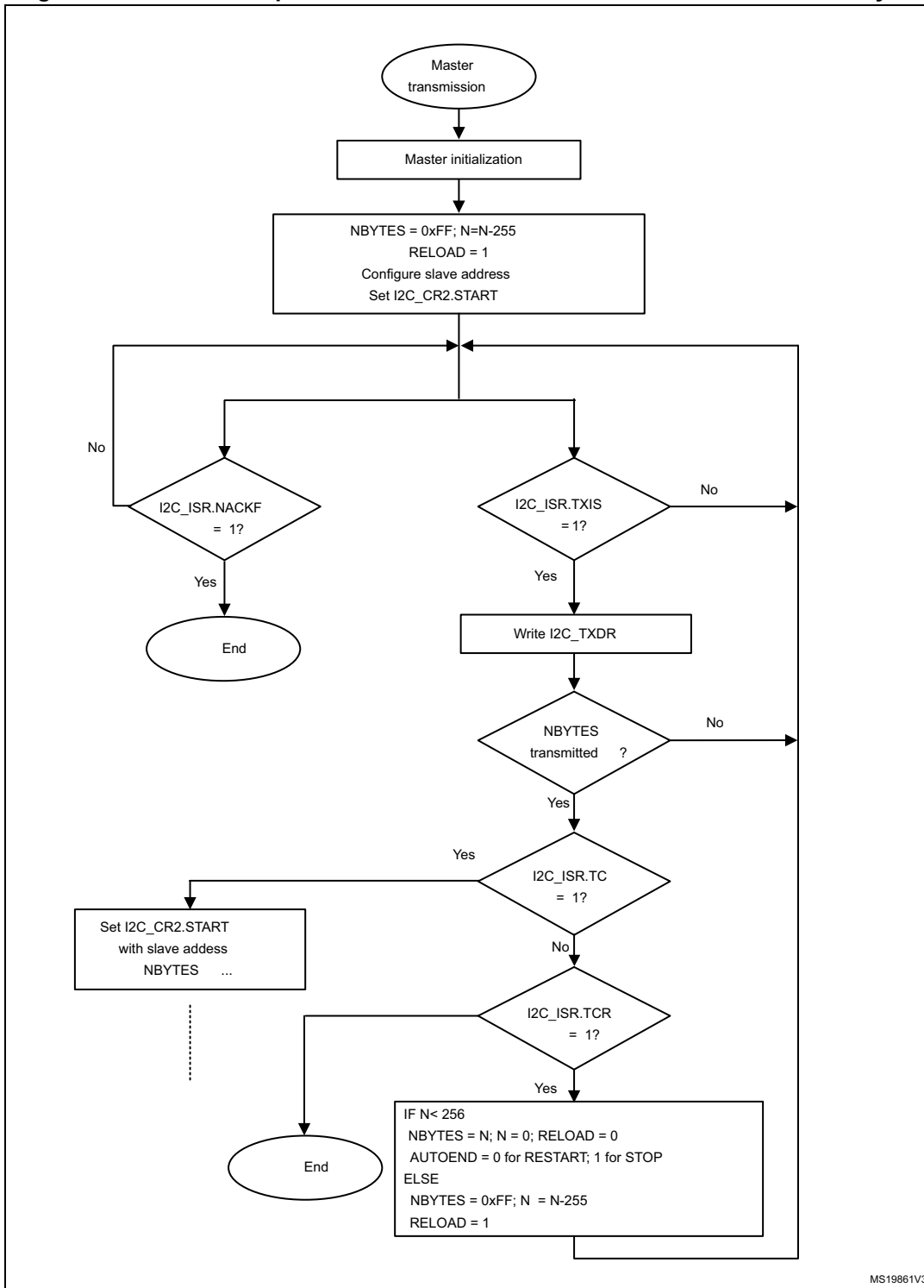
Figure 601. Transfer sequence flowchart for I2C master transmitter for N>255 bytes
