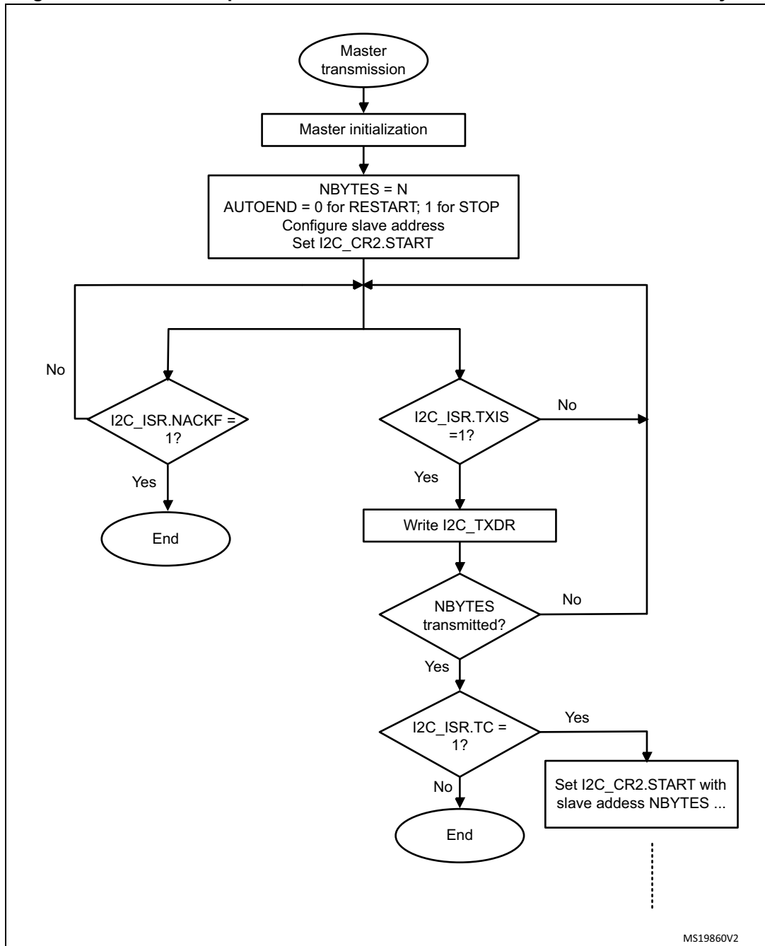
Figure 600. Transfer sequence flowchart for I2C master transmitter for N≤255 bytes
