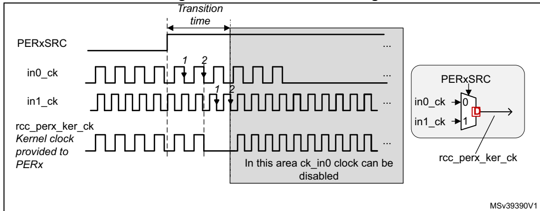
Figure 66. Kernel Clock switching
