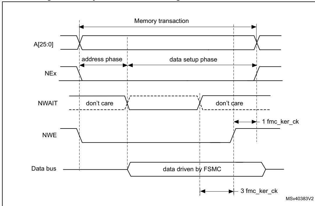
Figure 118. Asynchronous wait during a write access waveforms
