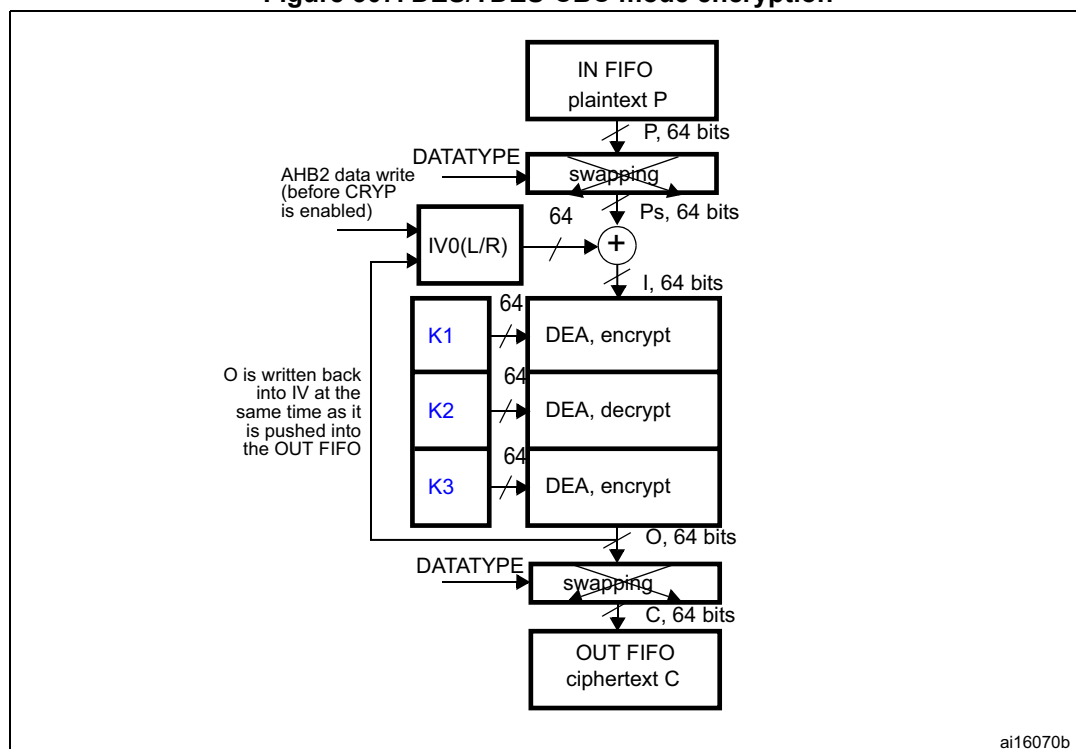
Figure 307. DES/TDES-CBC mode encryption
