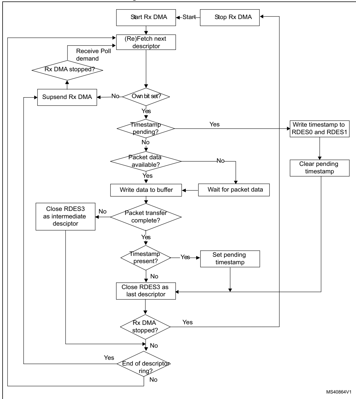
Figure 825. Receive DMA flow
