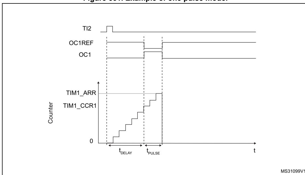
Figure 551. Example of one pulse mode.
