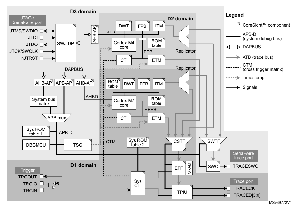
Figure 863. Power domains of debug infrastructure
