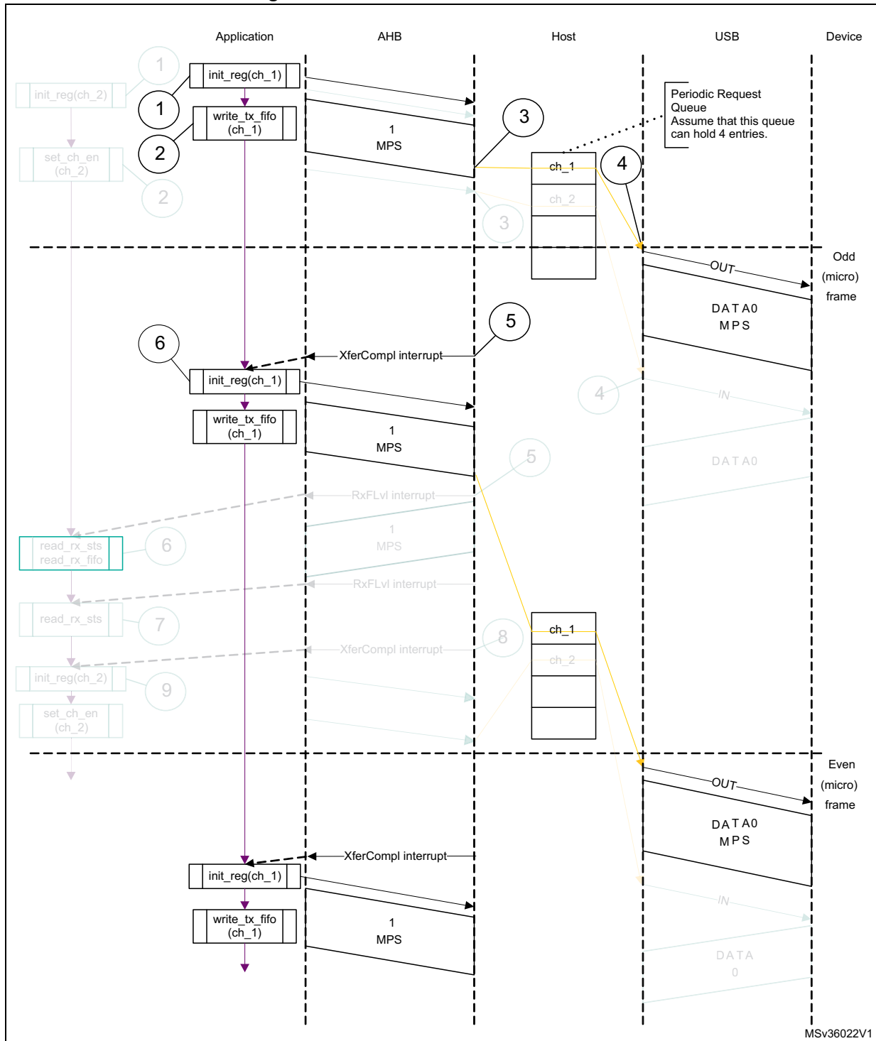
Figure 806. Isochronous OUT transactions
