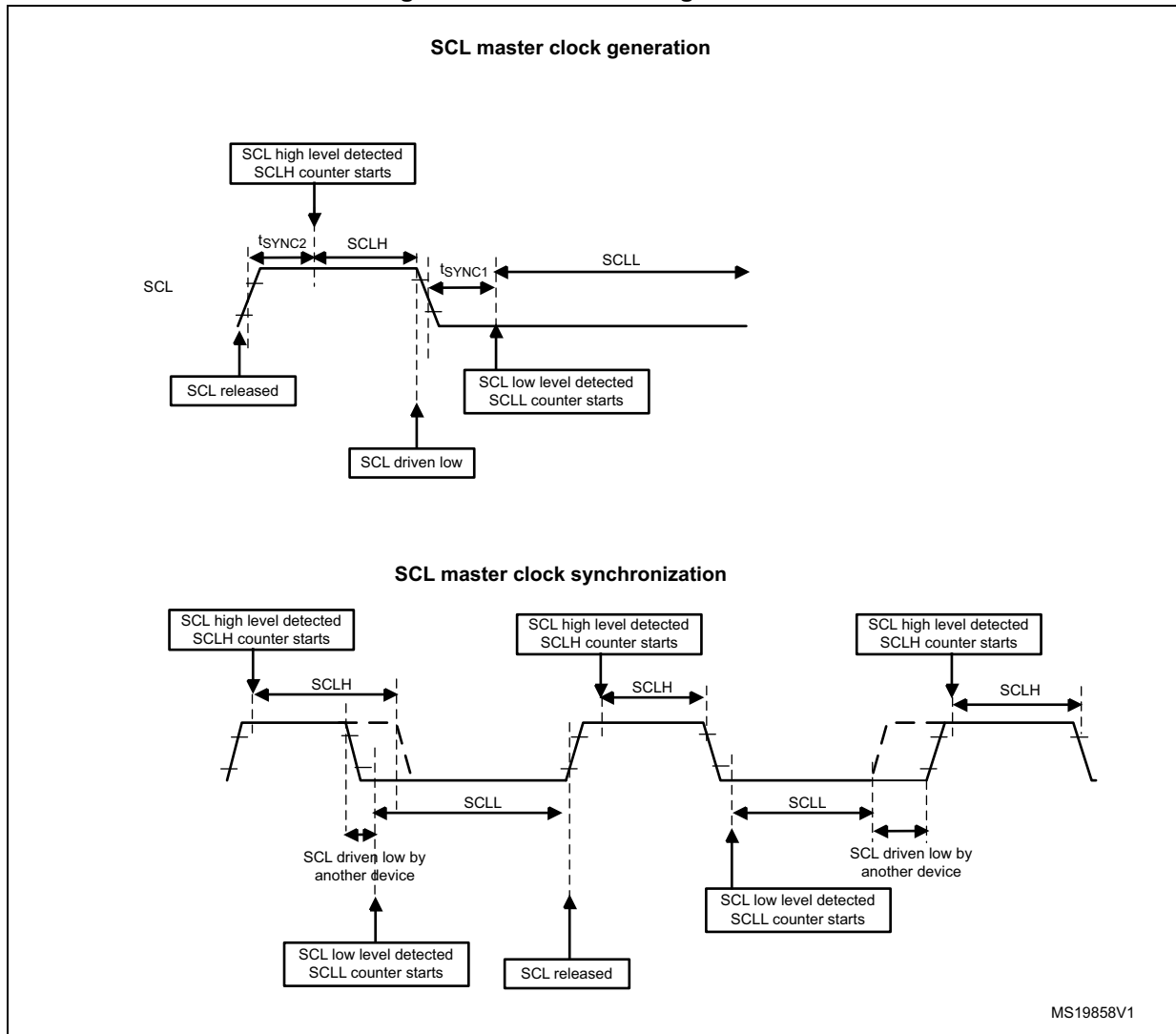
Figure 596. Master clock generation
