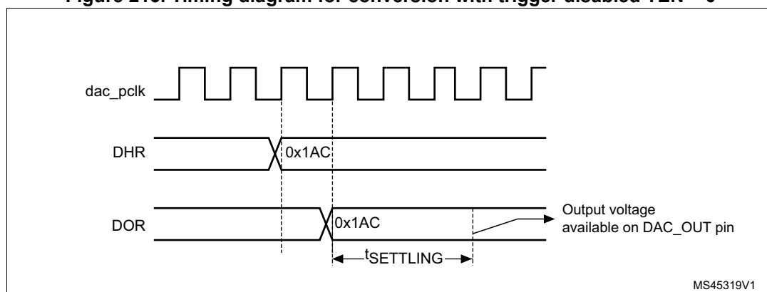
Figure 213. Timing diagram for conversion with trigger disabled TEN = 0
