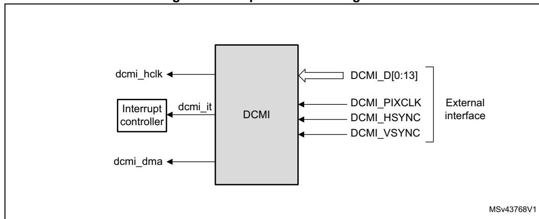
Figure 241. Top-level block diagram
