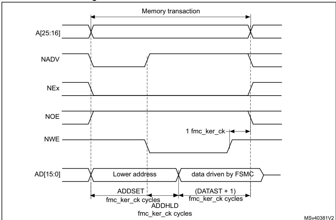
Figure 116. Muxed write access waveforms
