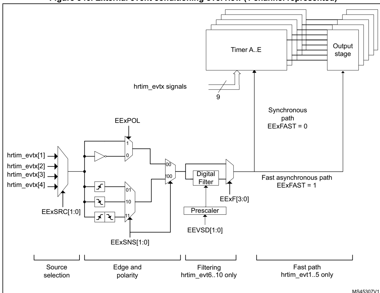
Figure 346. External event conditioning overview (1 channel represented)
