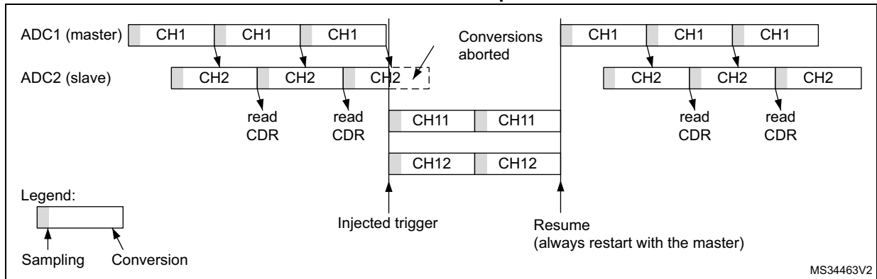
Figure 203. Two Interleaved channels (CH1, CH2) with injected sequence CH11, CH12 - case 2: Slave interrupted first
