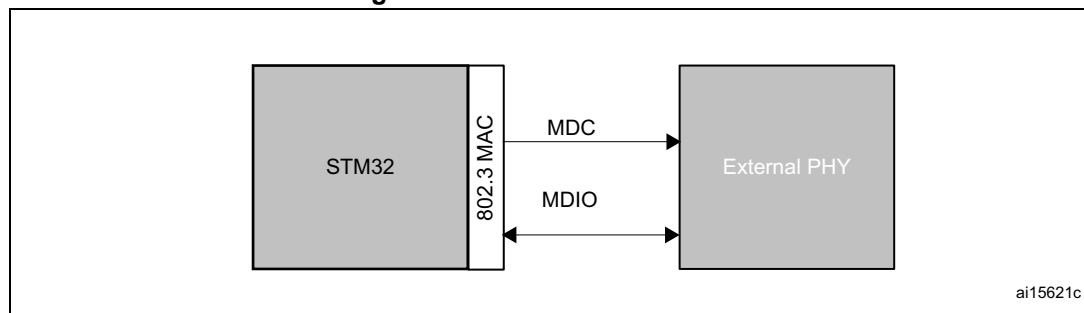
Figure 835. SMA Interface block
