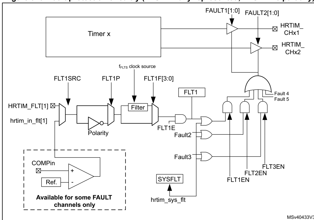
Figure 370. Fault protection circuitry (FAULT1 fully represented, FAULT2..5 partially)
