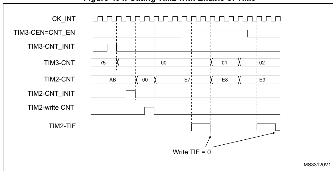
Figure 494. Gating TIM2 with Enable of TIM3
