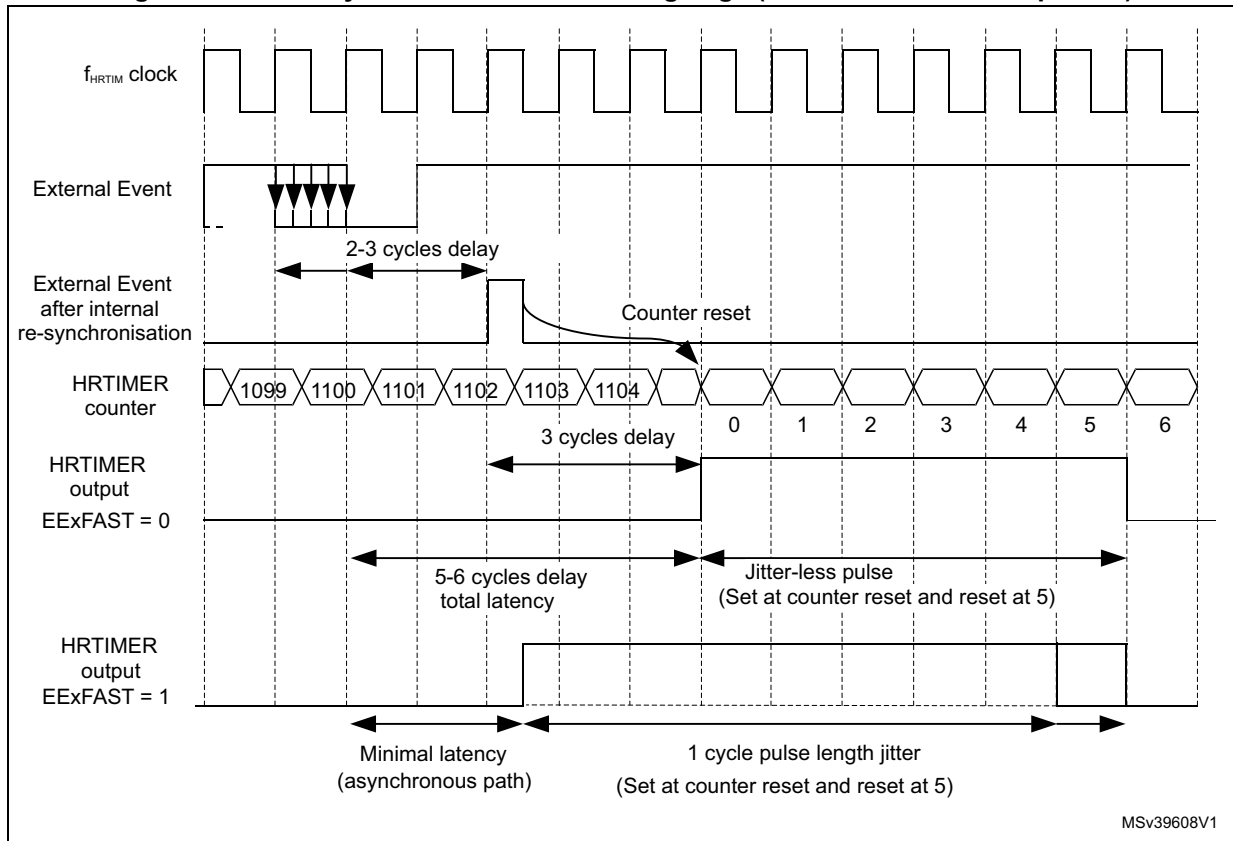
Figure 348. Latency to external events (output reset on external event)
