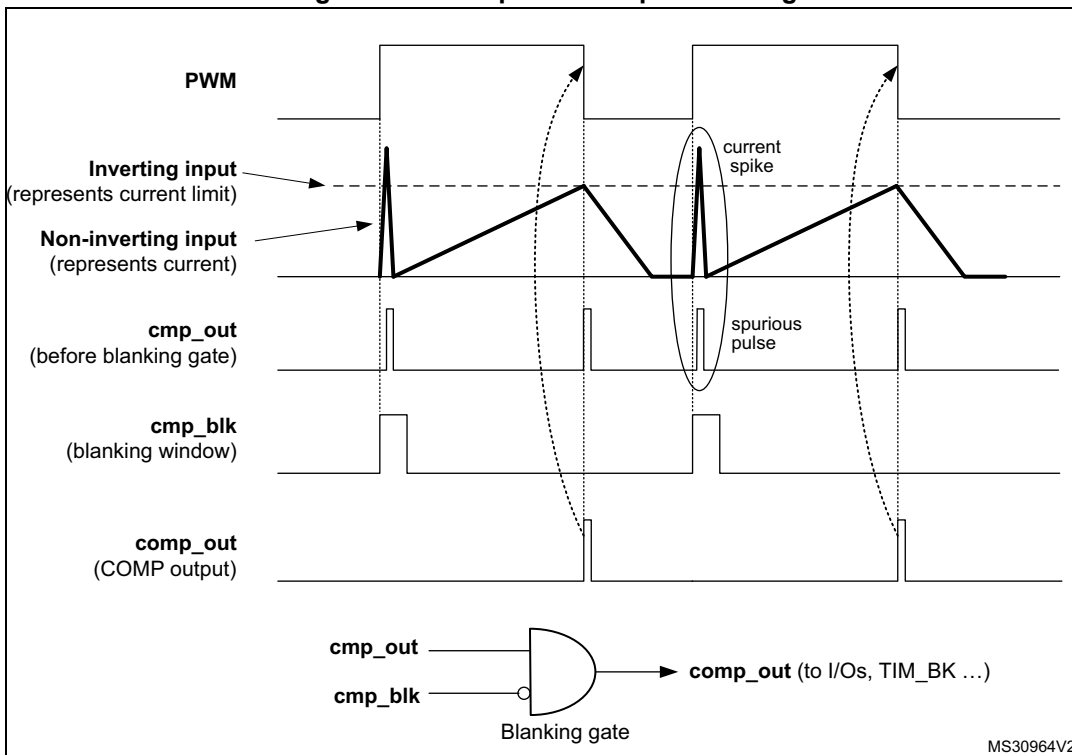
Figure 221. Comparator output blanking
