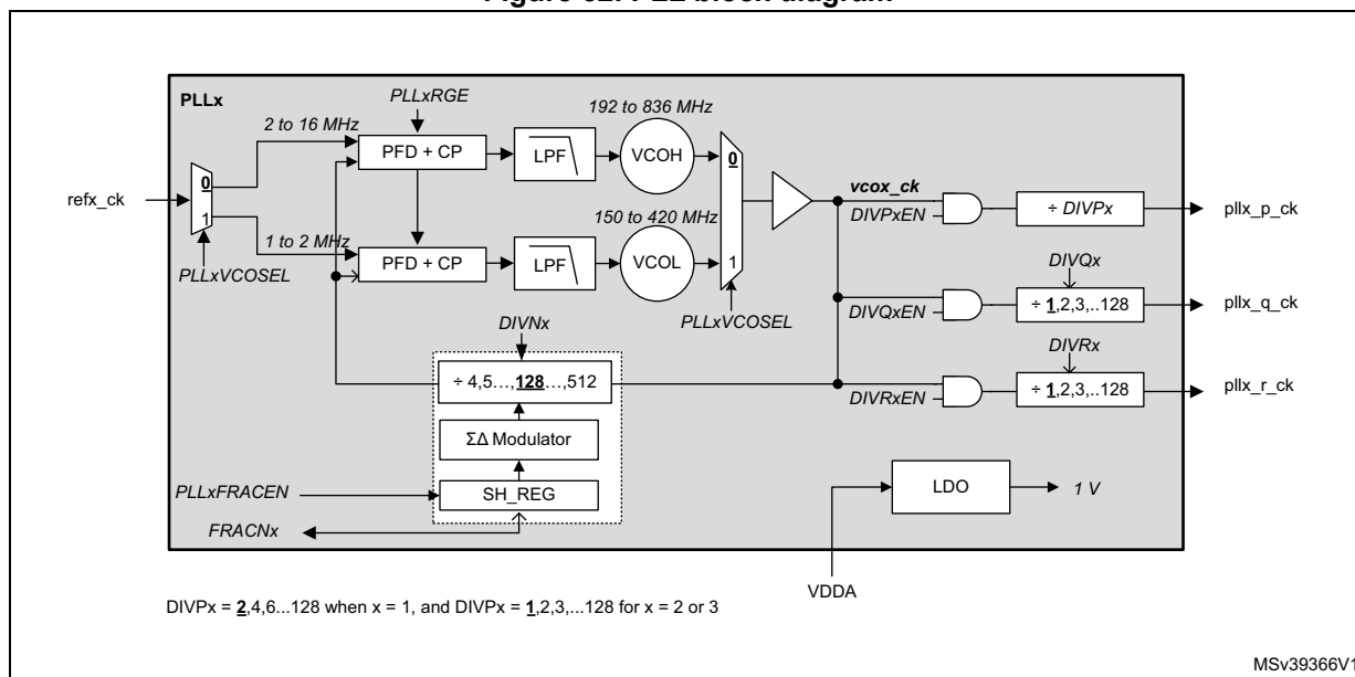
Figure 52. PLL block diagram
