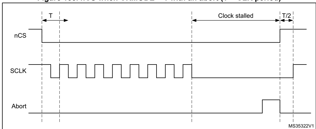
Figure 138. nCS when CKMODE = 1 with an abort (T = CLK period)
