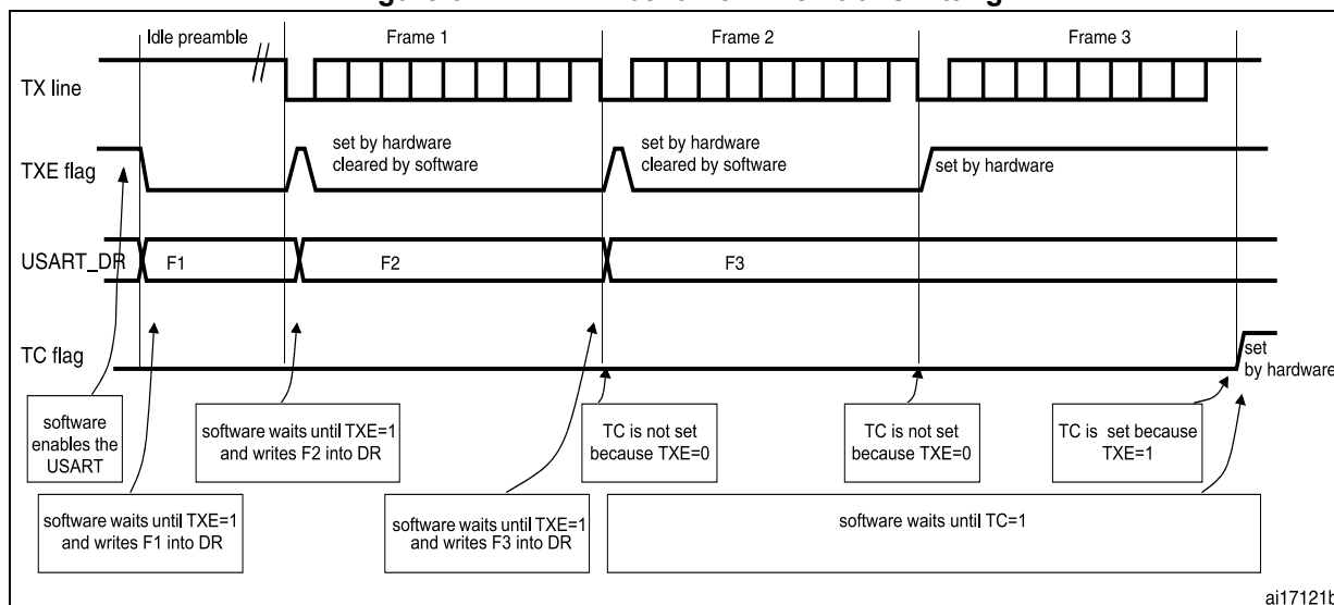
Figure 617. TC/TXE behavior when transmitting
