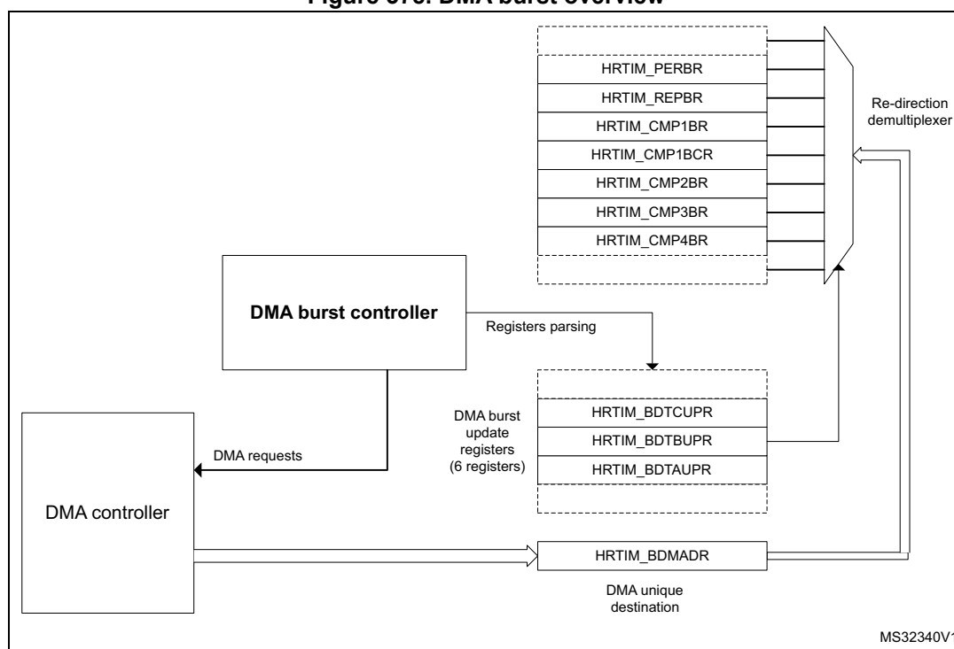
Figure 378. DMA burst overview
