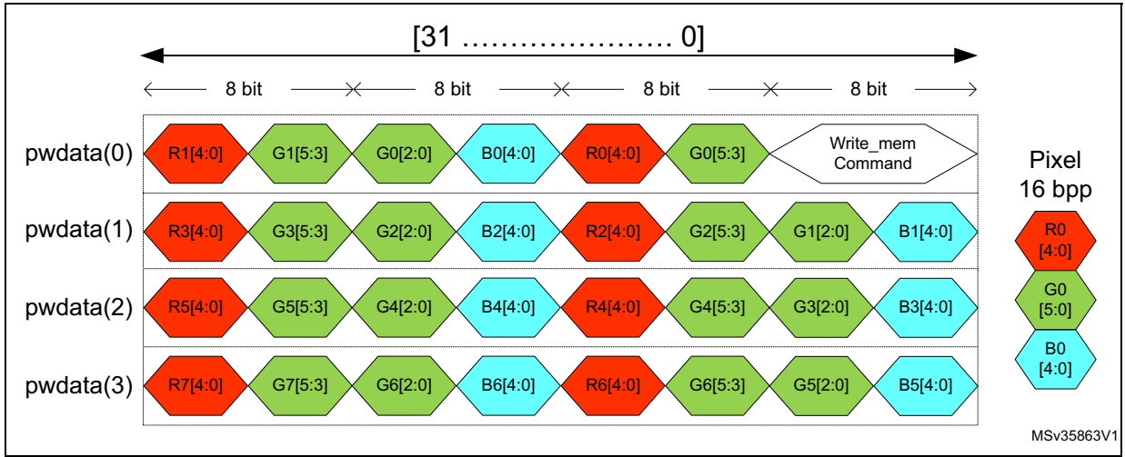
Figure 262. 16 bpp APB pixel to byte organization
