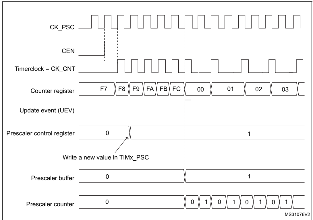
Figure 558. Counter timing diagram with prescaler division change from 1 to 2
