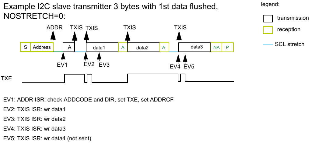
Figure 592. Transfer bus diagrams for I2C slave transmitter
