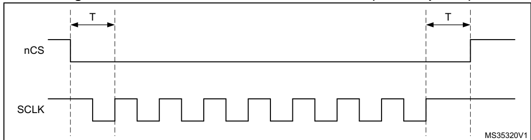
Figure 136. nCS when CKMODE = 1 in SDR mode (T = CLK period)
