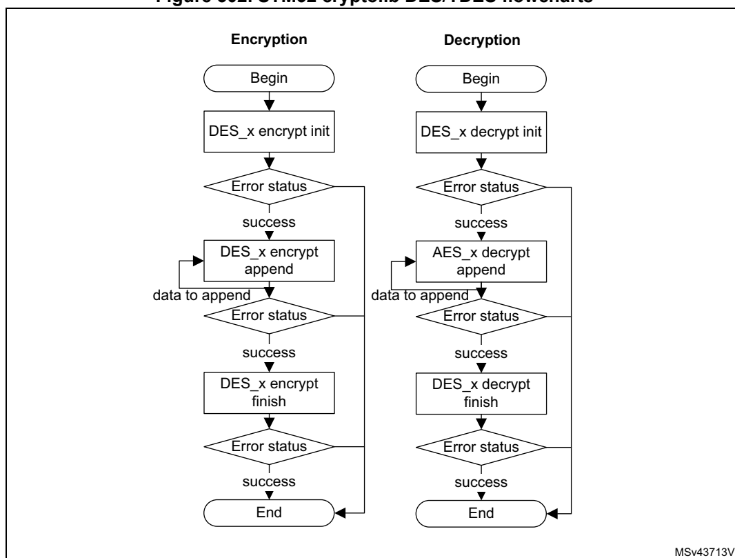
Figure 302. STM32 cryptolib DES/TDES flowcharts
