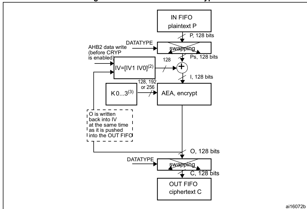
Figure 311. AES-CBC mode encryption
