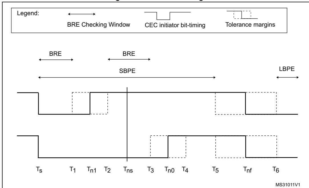
Figure 860. Error handling
