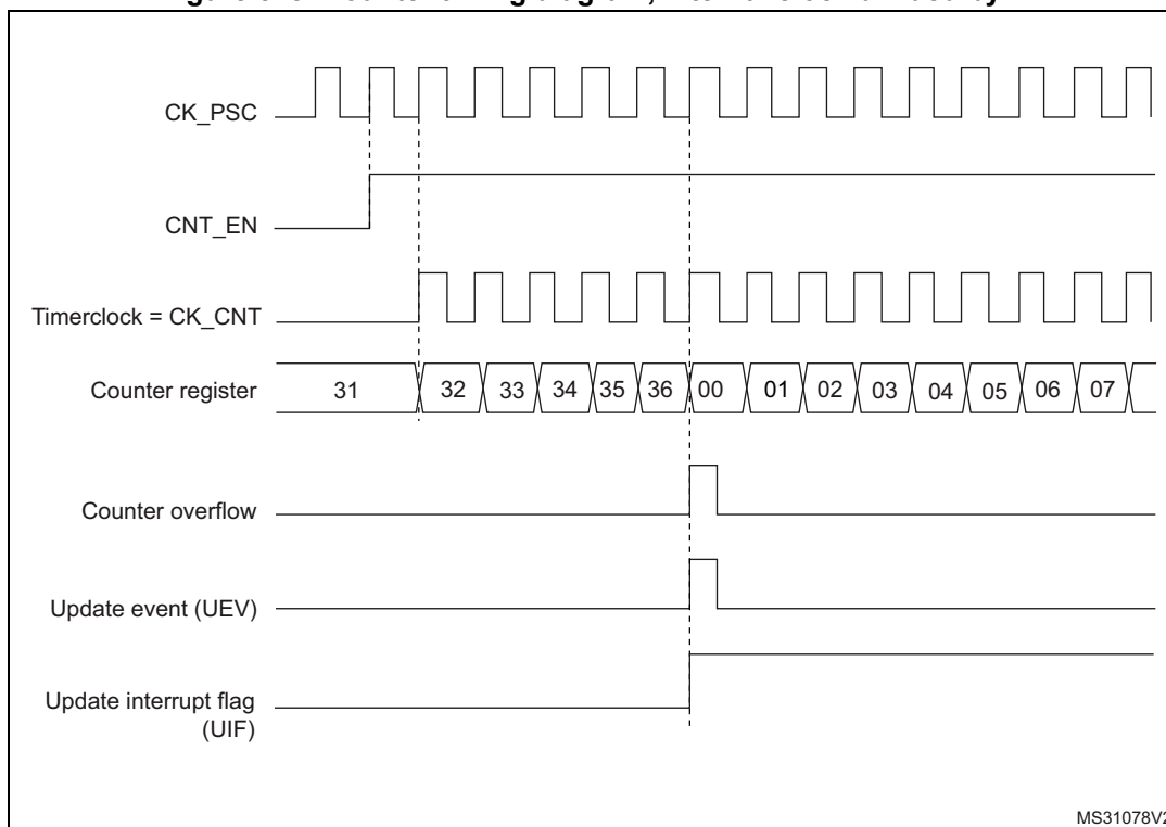
Figure 528. Counter timing diagram, internal clock divided by 1
