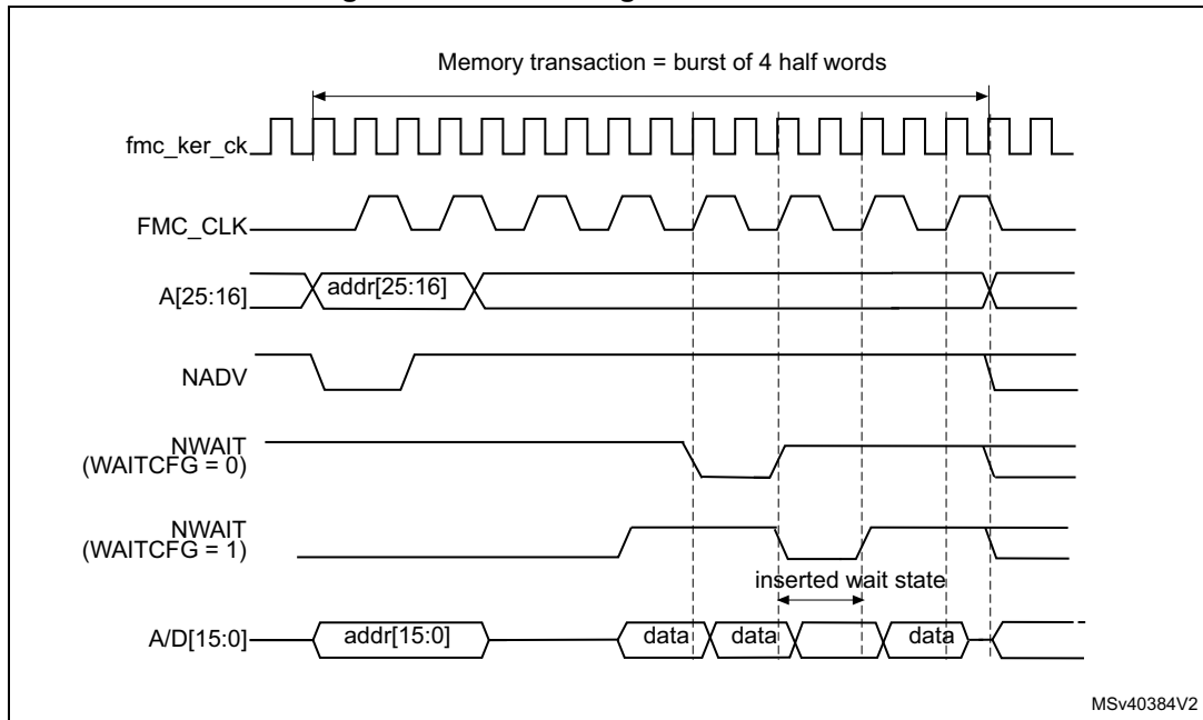
Figure 119. Wait configuration waveforms
