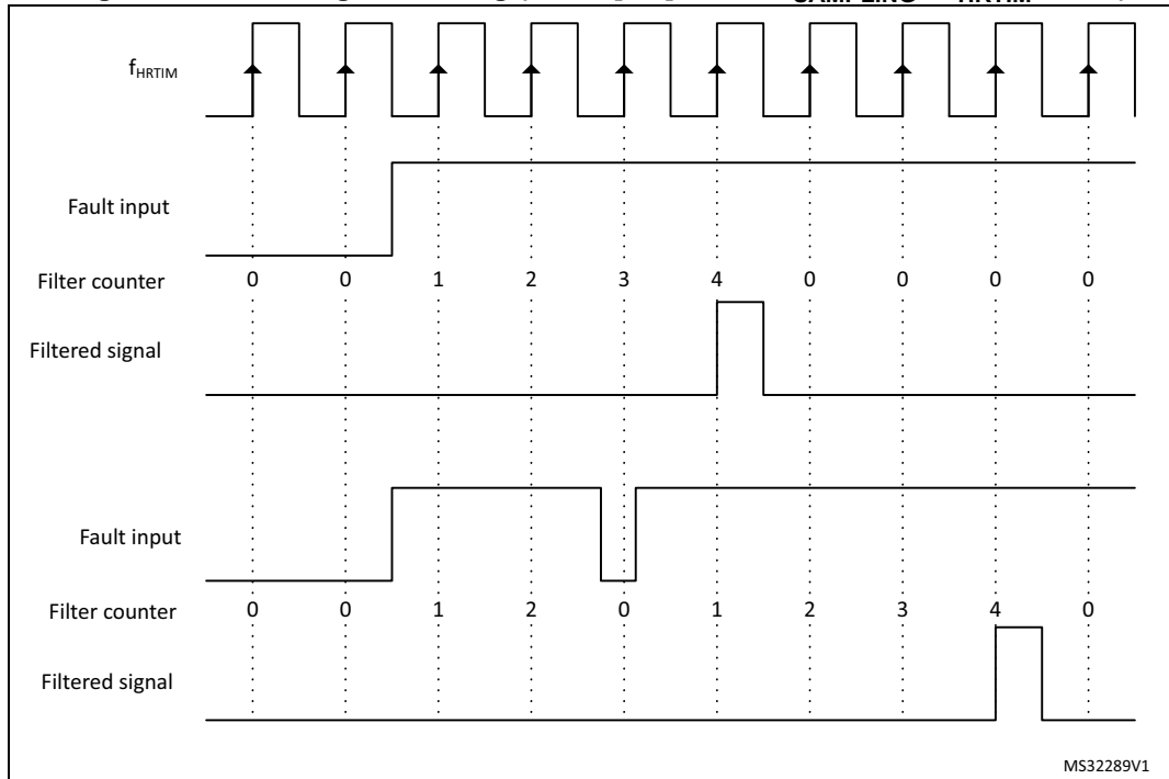
Figure 371. Fault signal filtering (FLTxF[3:0]= 0010: f_{\text{SAMPLING}} = f_{\text{HRTIM}} , N = 4)
