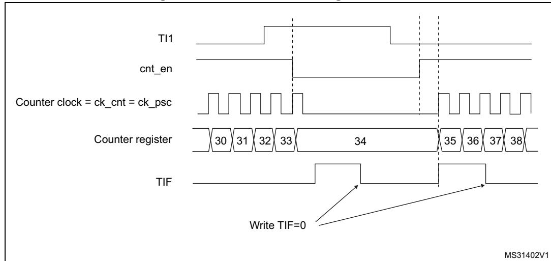
Figure 522. Control circuit in gated mode
