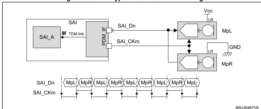
Figure 696. PDM typical connection and timing
