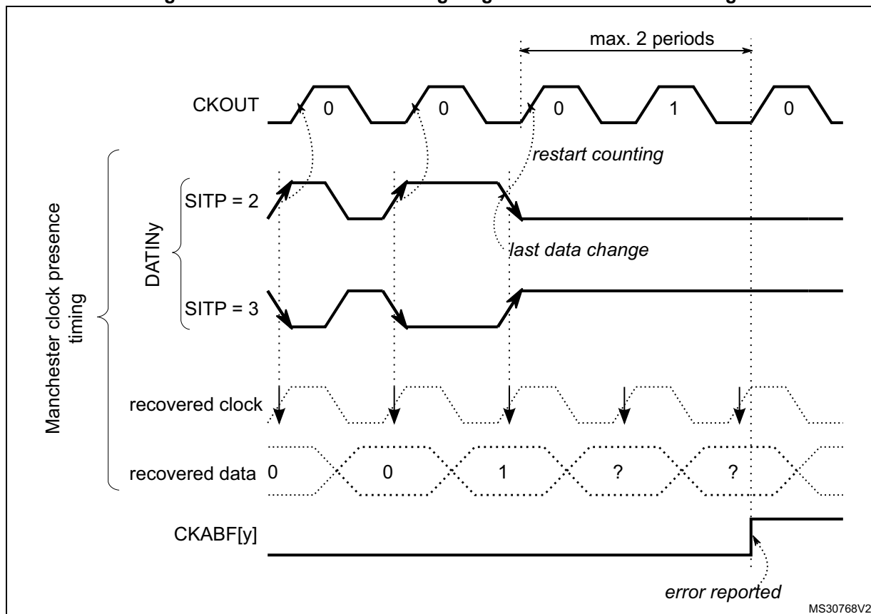
Figure 236. Clock absence timing diagram for Manchester coding
