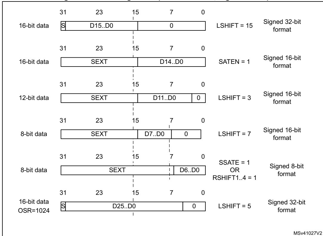
Figure 173. Left alignment (offset enabled, signed value)
