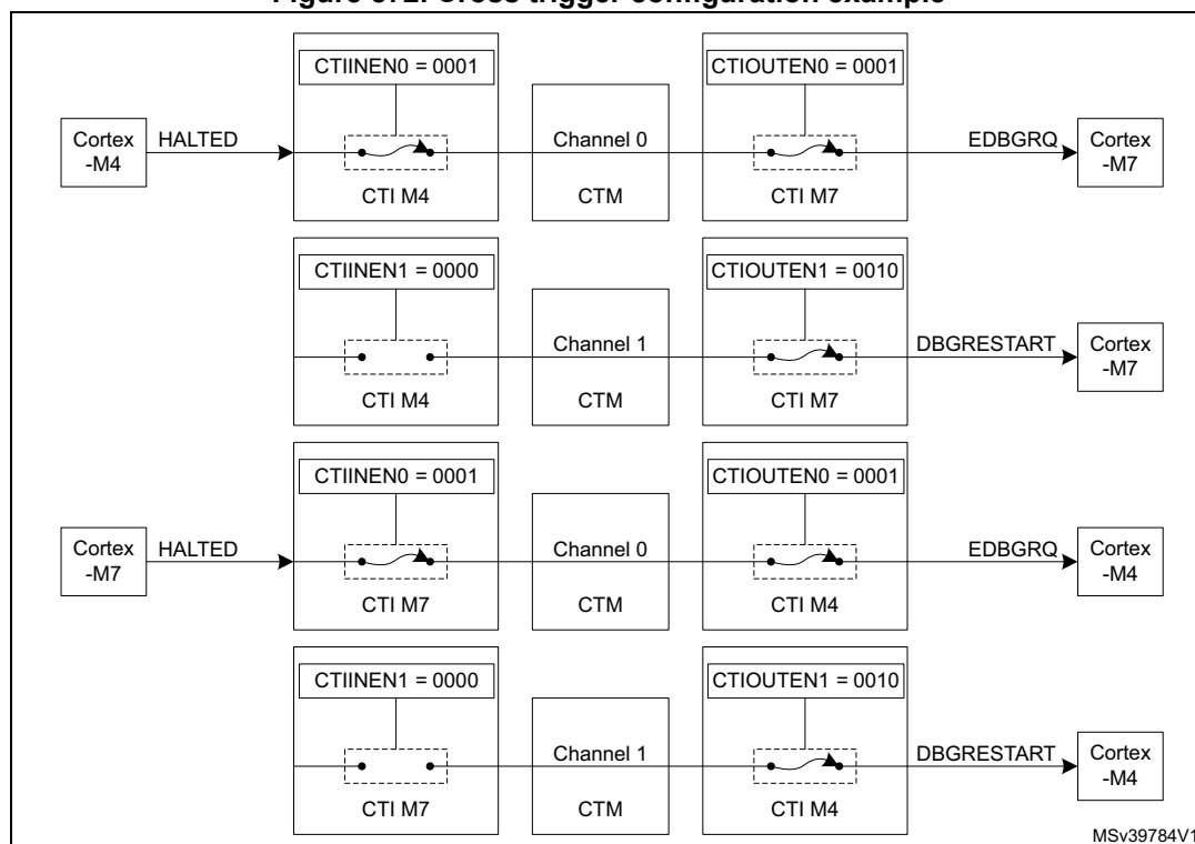
Figure 872. Cross trigger configuration example
