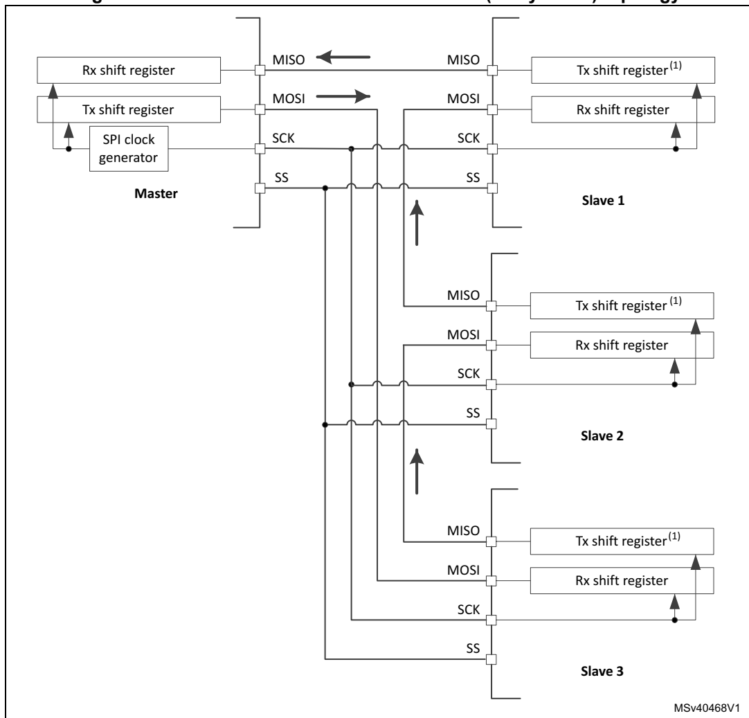
Figure 660. Master and three slaves at circular (daisy chain) topology
