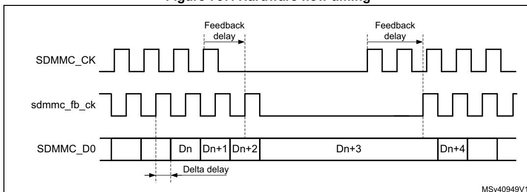
Figure 757. Hardware flow timing
