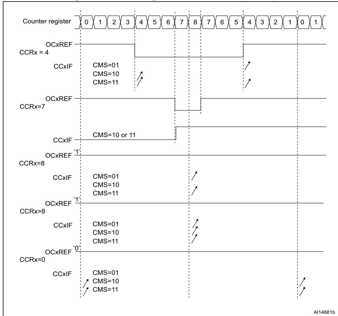
Figure 425. Center-aligned PWM waveforms (ARR=8)
