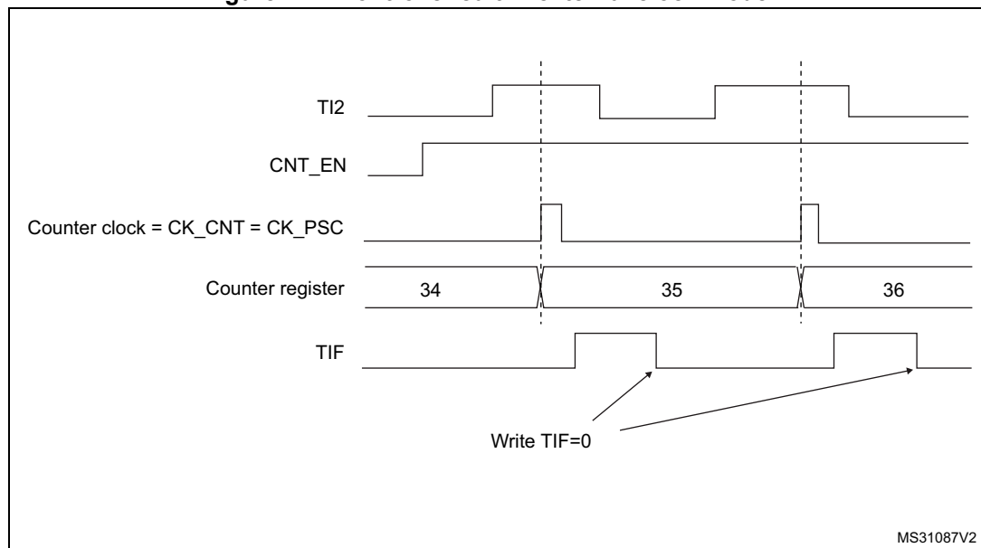
Figure 471. Control circuit in external clock mode 1
