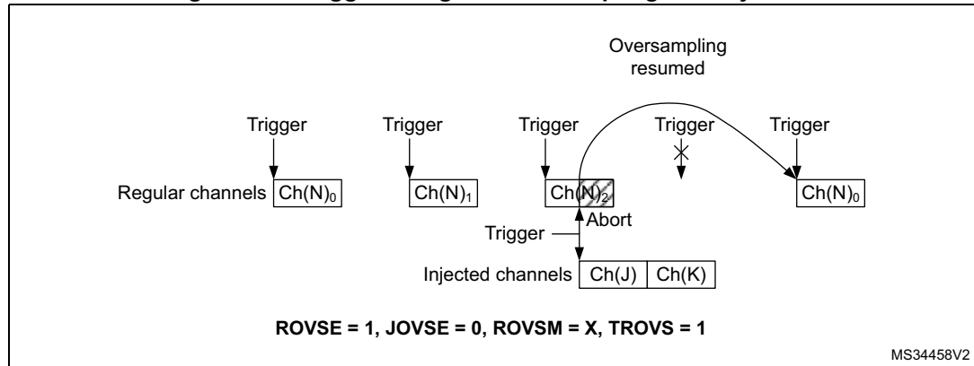
Figure 189. Triggered regular oversampling with injection
