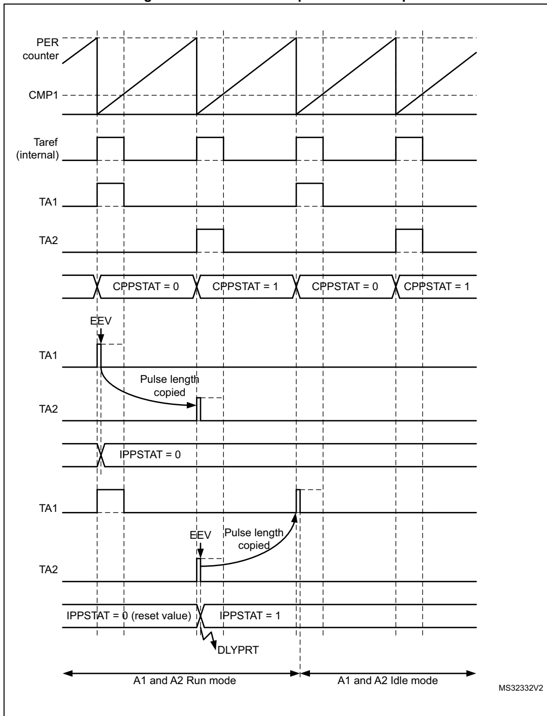
Figure 359. Balanced Idle protection example
