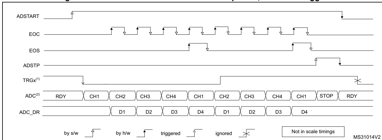
Figure 169. Continuous conversions of a sequence, hardware trigger
