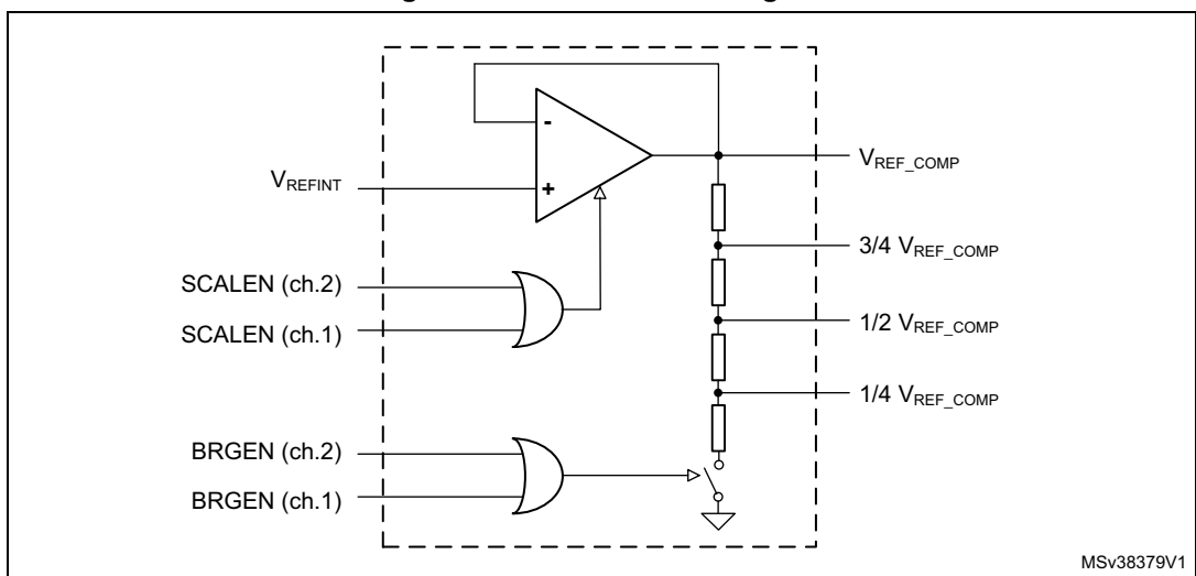
Figure 223. Scaler block diagram
