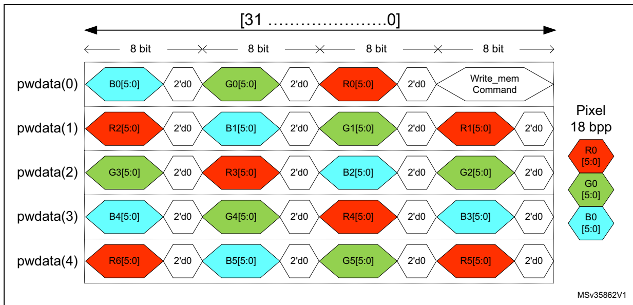
Figure 261. 18 bpp APB pixel to byte organization
