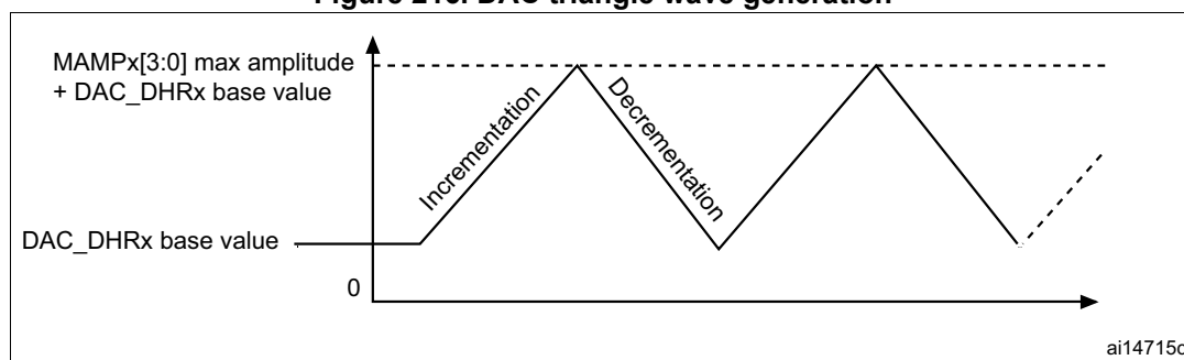
Figure 216. DAC triangle wave generation
