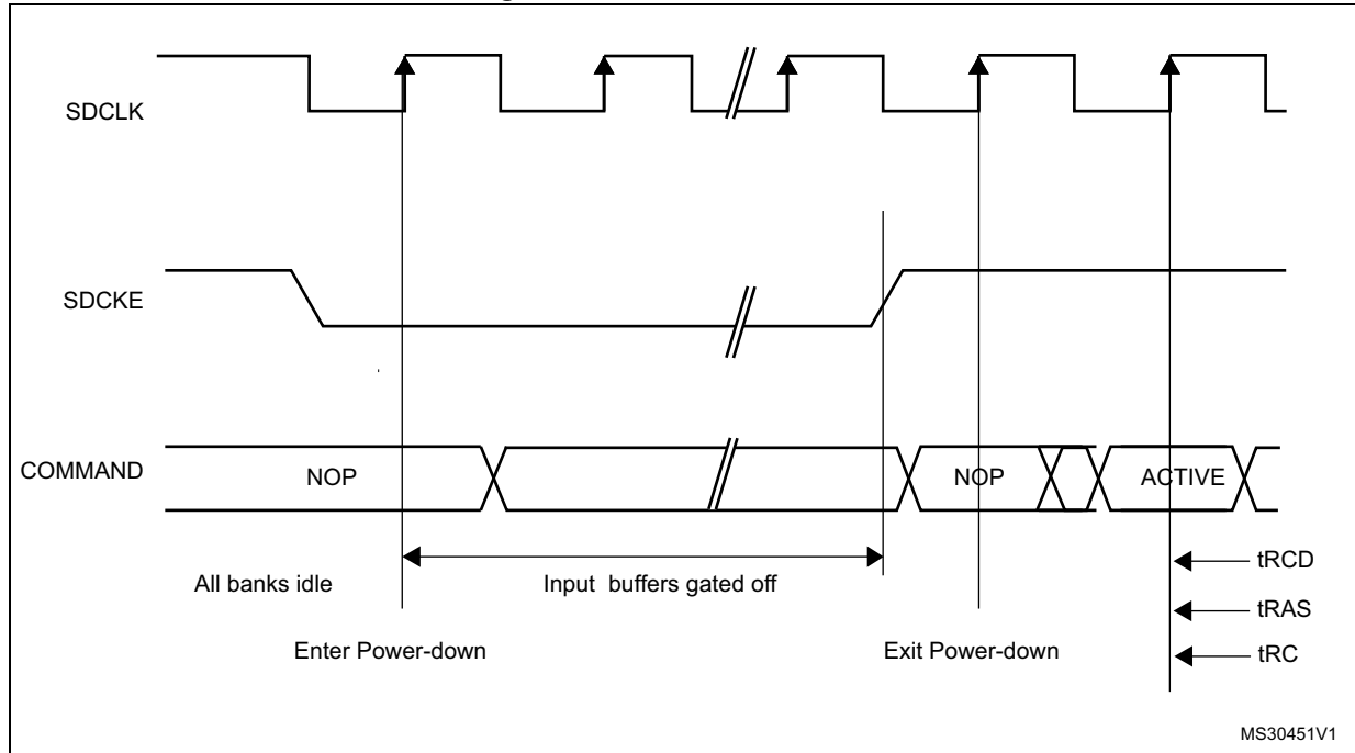
Figure 130. Power-down mode
