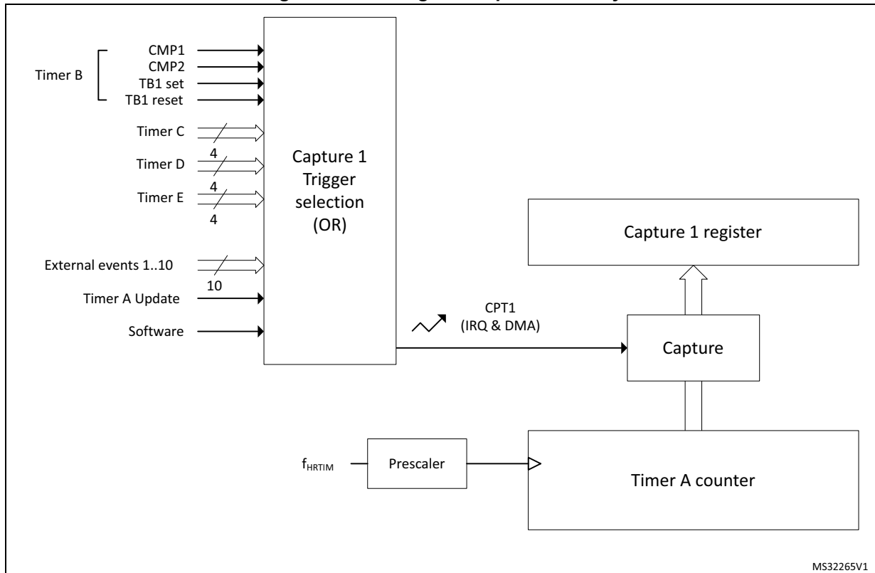
Figure 334. Timing unit capture circuitry
