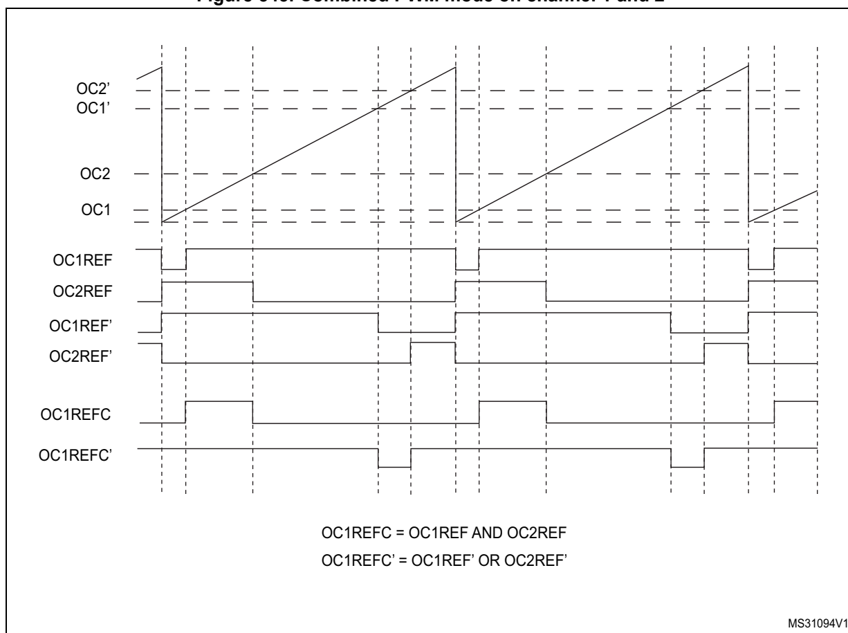
Figure 545. Combined PWM mode on channel 1 and 2
