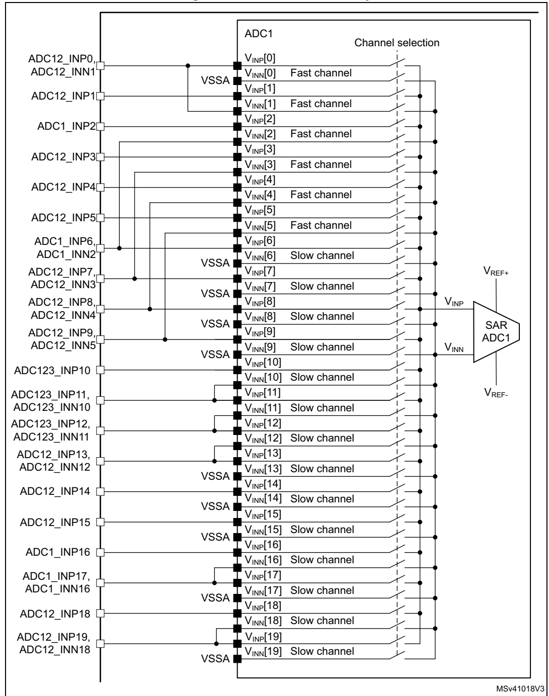
Figure 142. ADC1 connectivity
