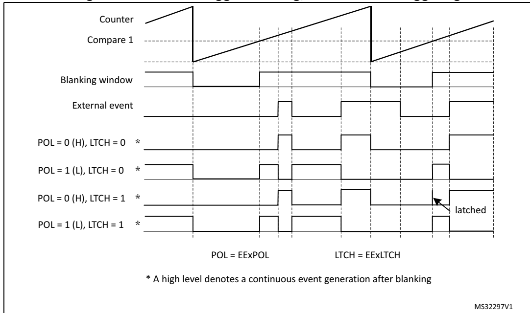
Figure 352. External trigger blanking, level sensitive triggering
