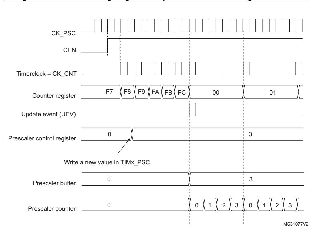
Figure 559. Counter timing diagram with prescaler division change from 1 to 4
