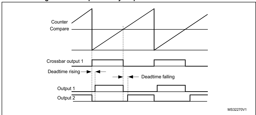
Figure 339. Complementary outputs with deadtime insertion
