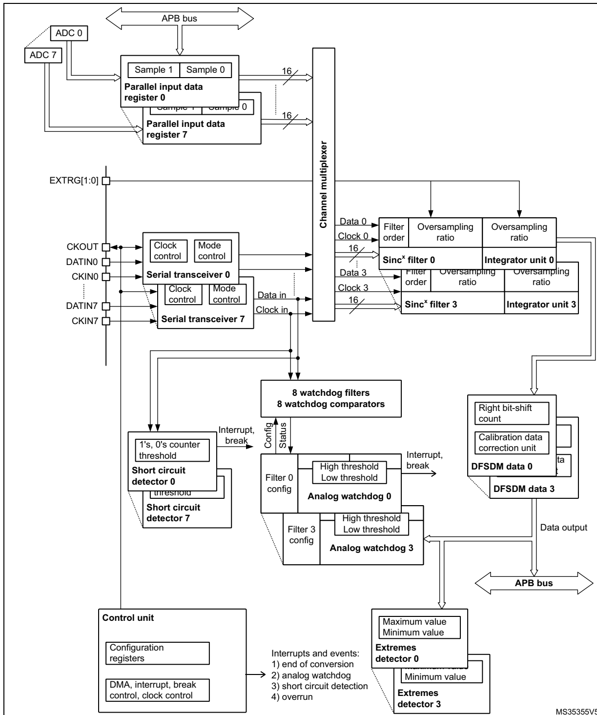
Figure 232. Single DFSDM block diagram
