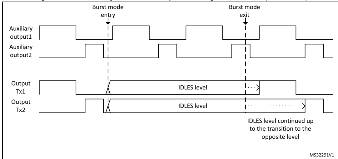
Figure 373. Auxiliary and main outputs during burst mode (DIDLx = 0)
