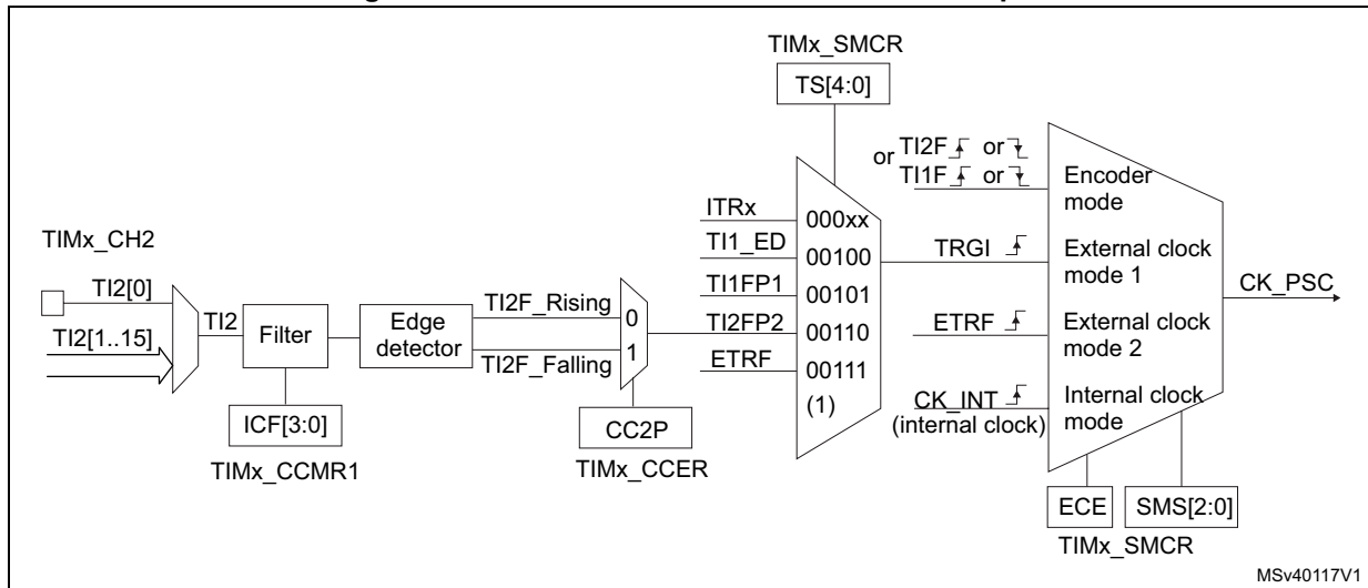
Figure 413. T12 external clock connection example
