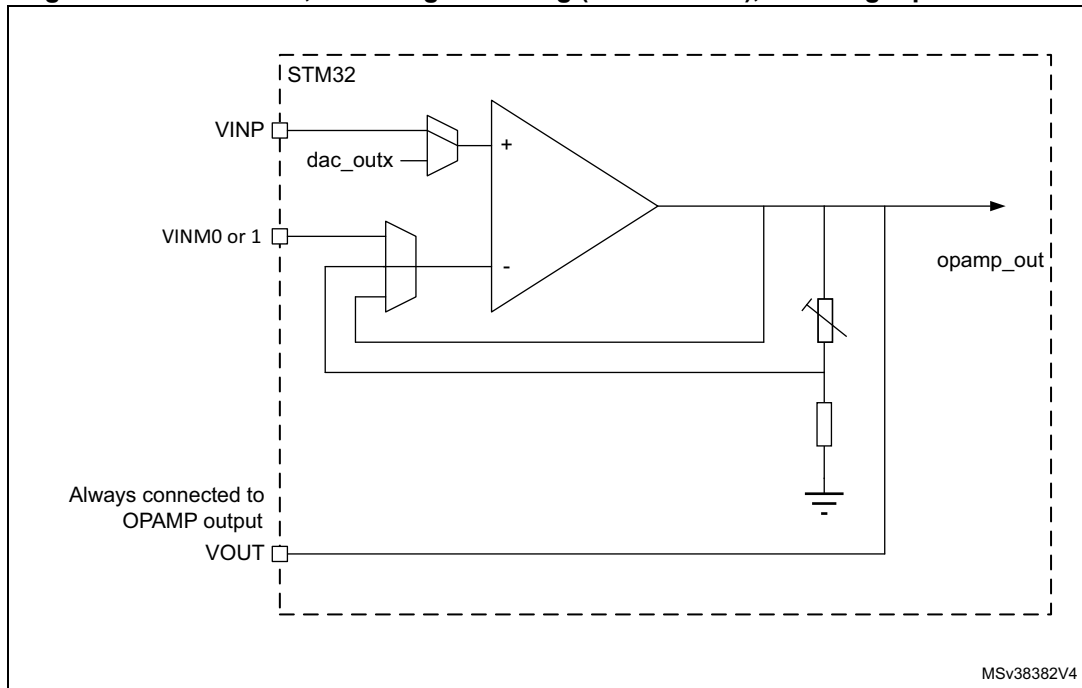
Figure 226. PGA mode, internal gain setting (x2/x4/x8/x16), inverting input not used
