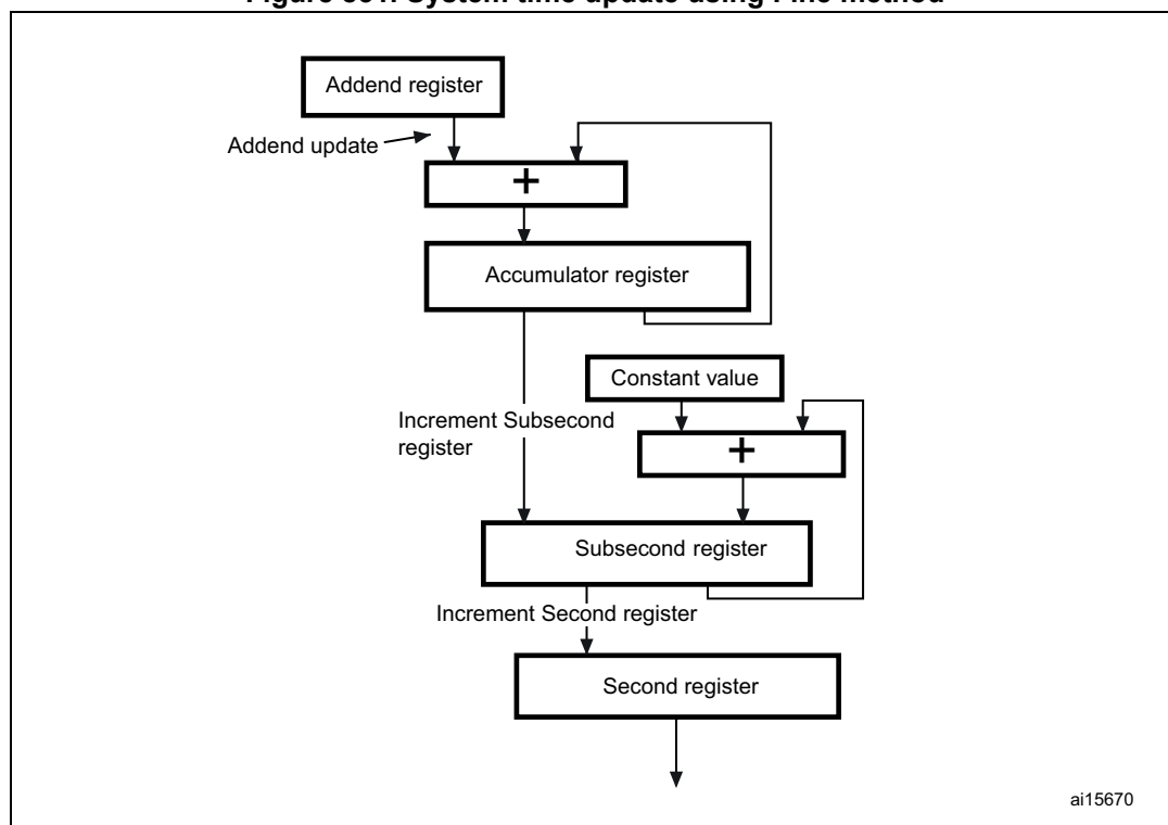
Figure 831. System time update using Fine method
