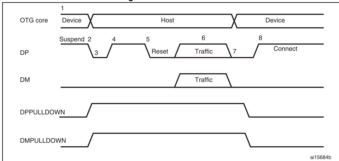
Figure 821. B-device HNP
