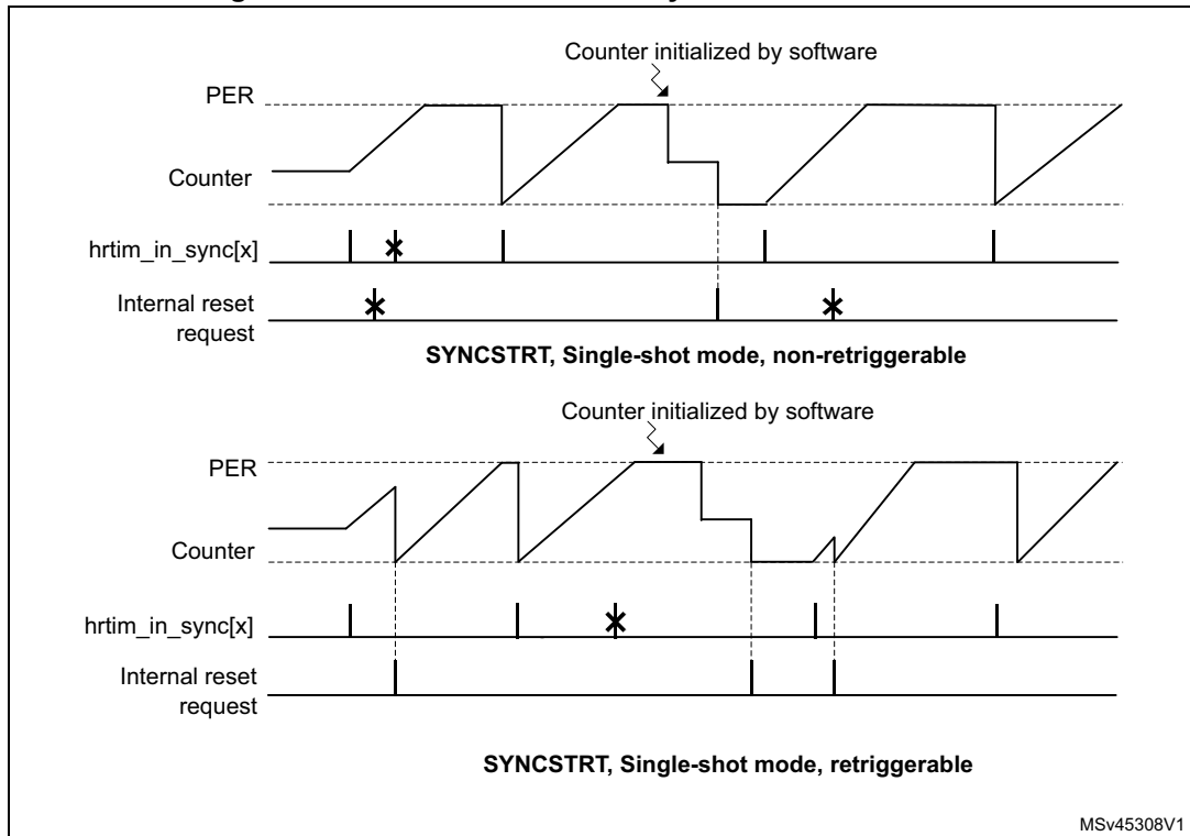
Figure 375. Counter behavior in synchronized start mode
