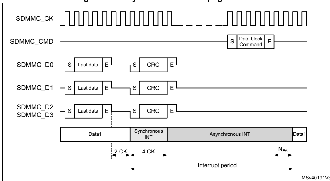
Figure 758. Asynchronous interrupt generation
