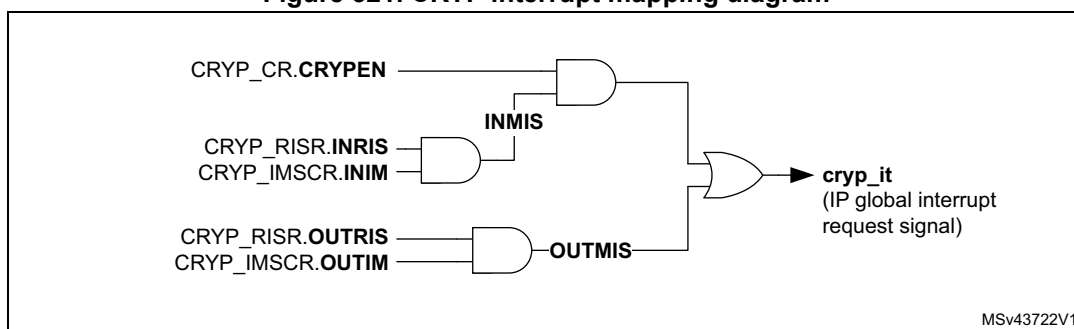
Figure 321. CRYP interrupt mapping diagram
