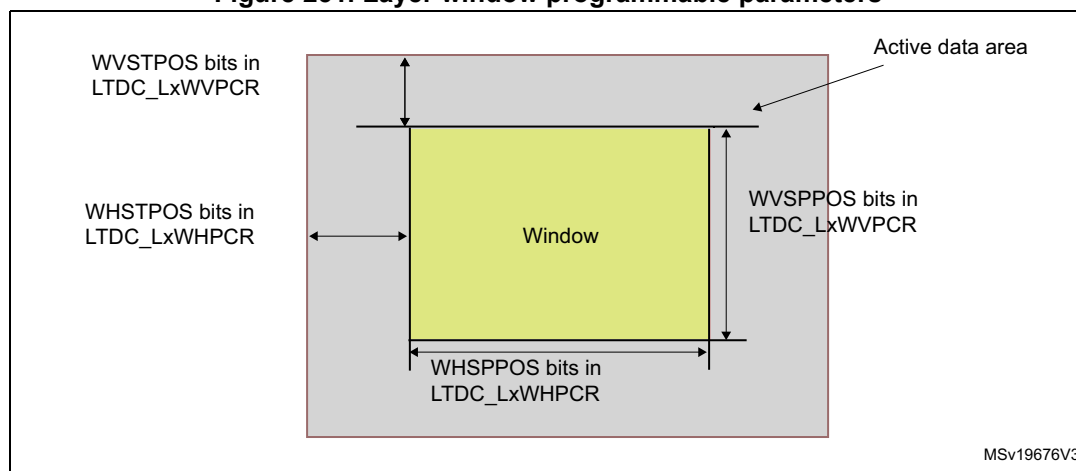
Figure 251. Layer window programmable parameters
