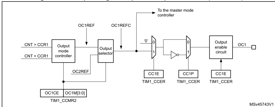
Figure 513. Output stage of capture/compare channel (channel 1)
