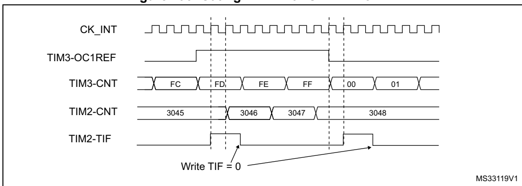
Figure 493. Gating TIM2 with OC1REF of TIM
