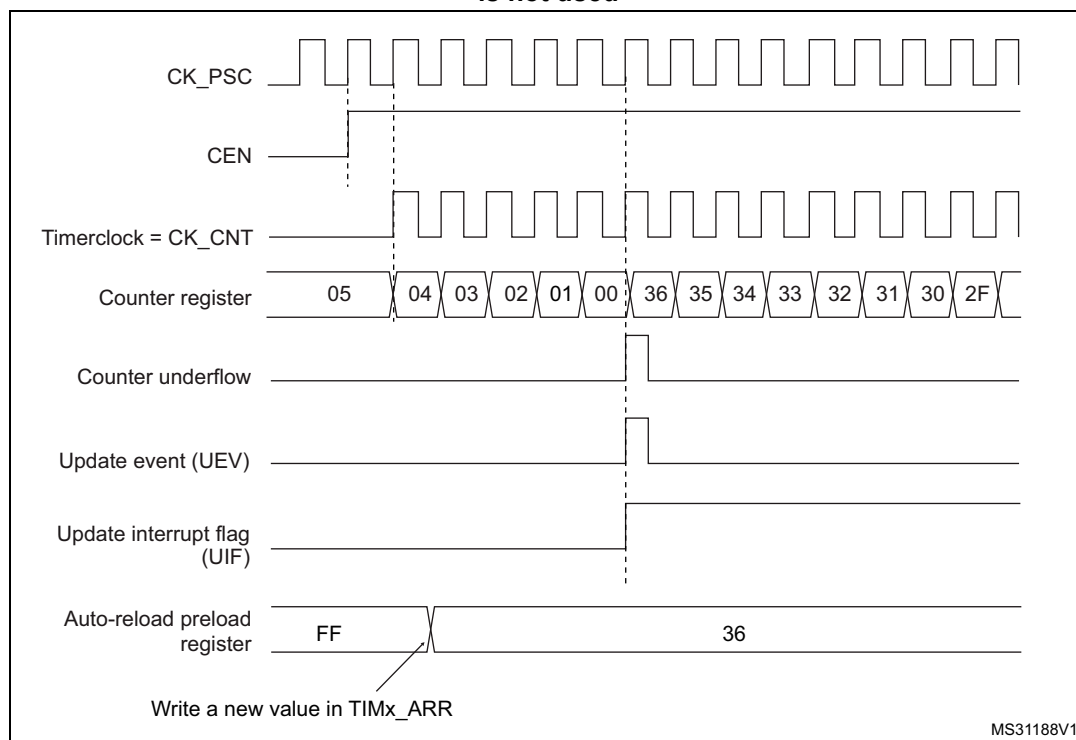
Figure 462. Counter timing diagram, Update event when repetition counter is not used
