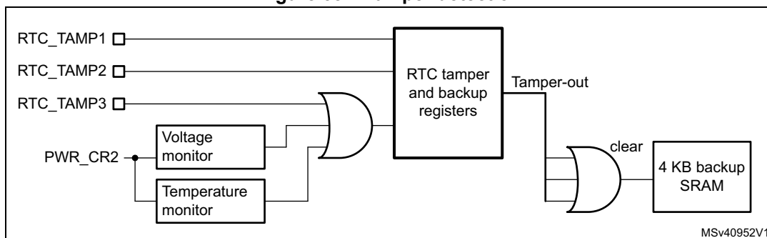
Figure 582. Tamper detection
