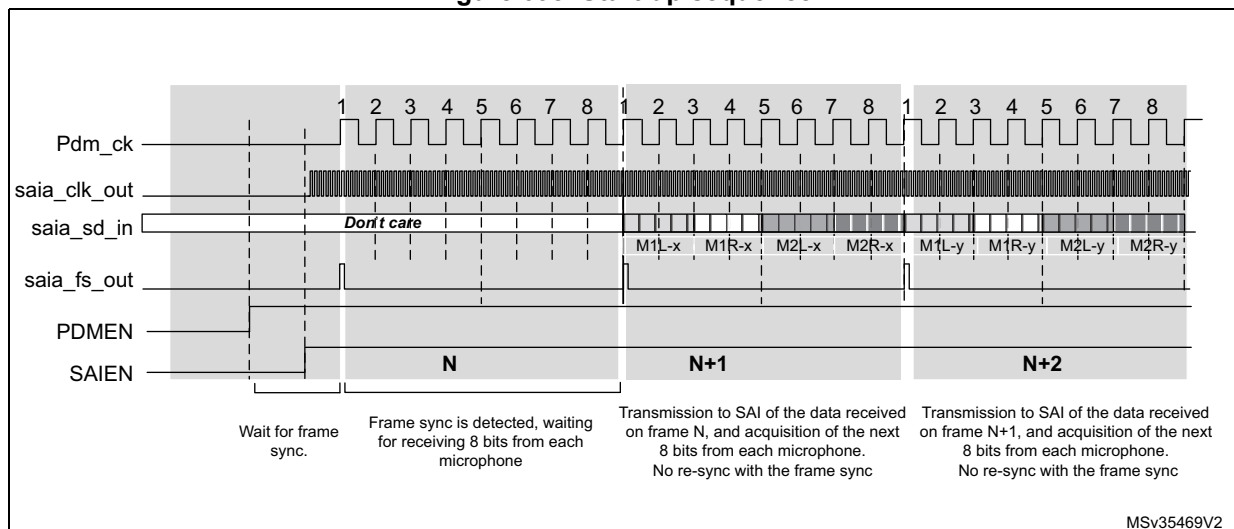
Figure 698. Start-up sequence
