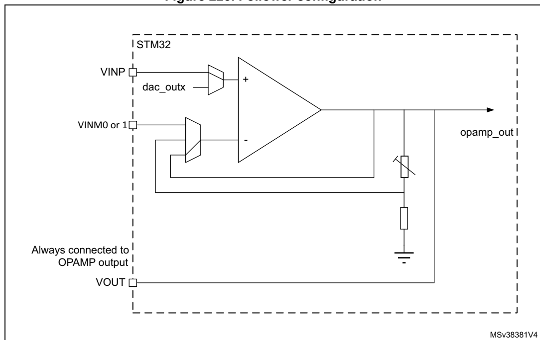
Figure 225. Follower configuration
