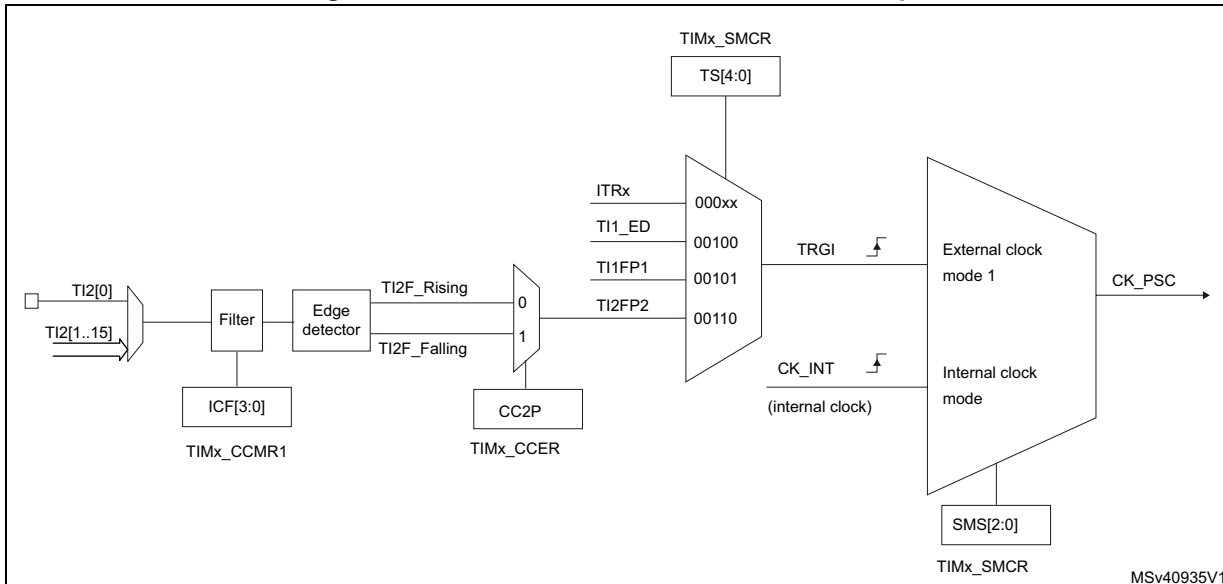
Figure 536. TI2 external clock connection example
