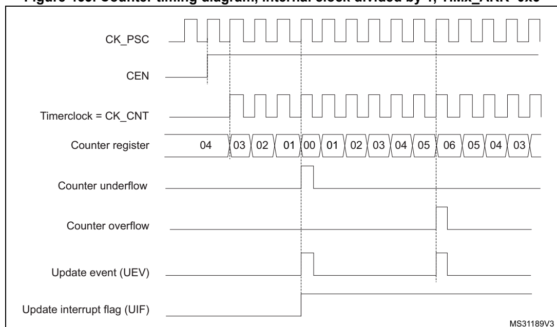
Figure 463. Counter timing diagram, internal clock divided by 1, TIMx_ARR=0x6
