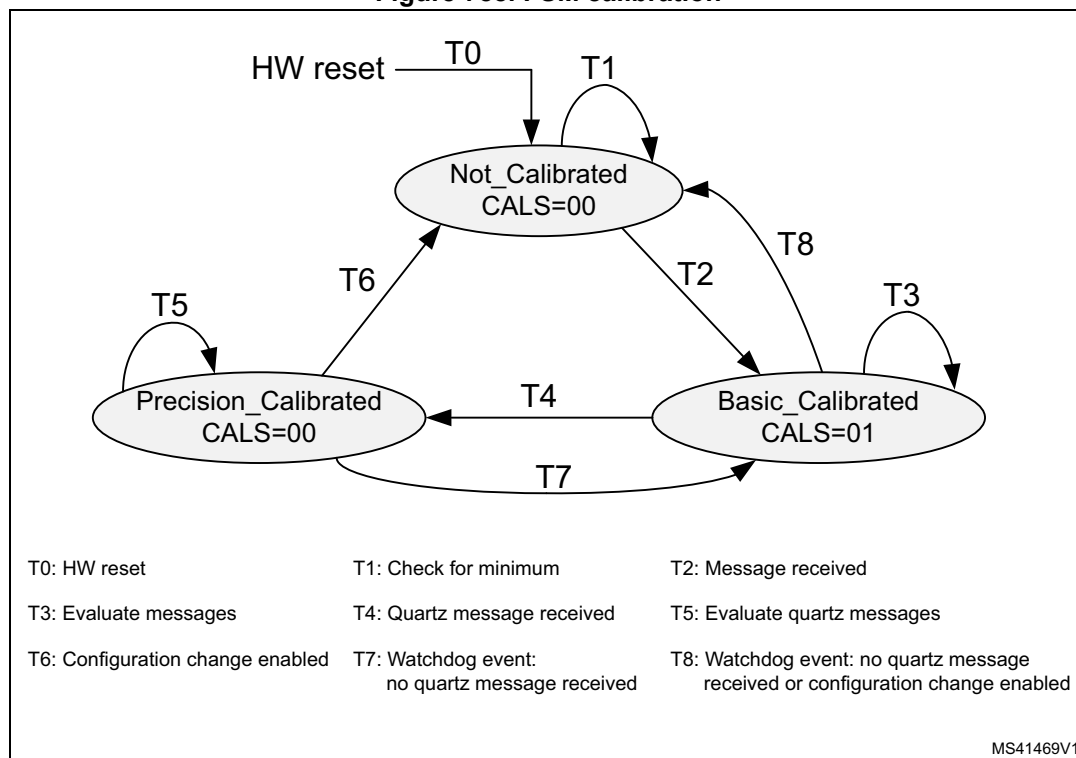
Figure 788. FSM calibration
