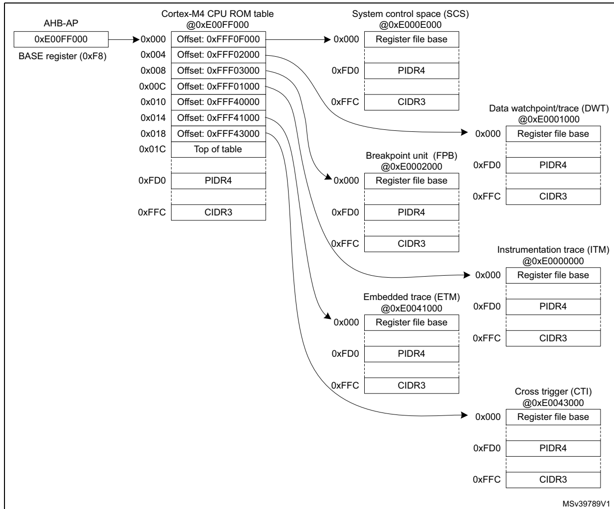
Figure 875. Cortex-M4 CoreSight Topology
