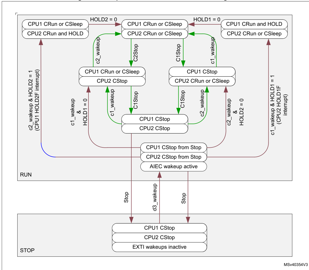
Figure 42. Stop mode hold mechanism state diagram
