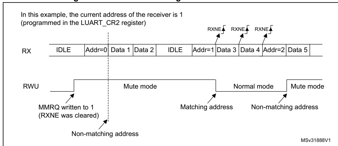
Figure 647. Mute mode using address mark detection
