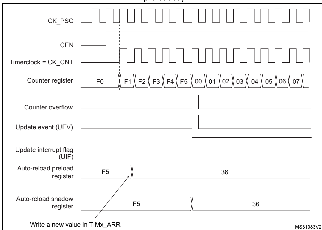
Figure 507. Counter timing diagram, update event when ARPE=1 (TIMx_ARR preloaded)
