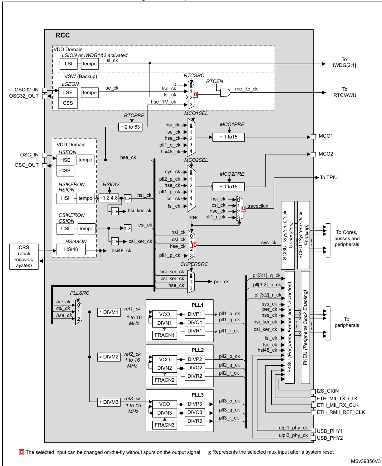
Figure 50. Top-level clock tree
