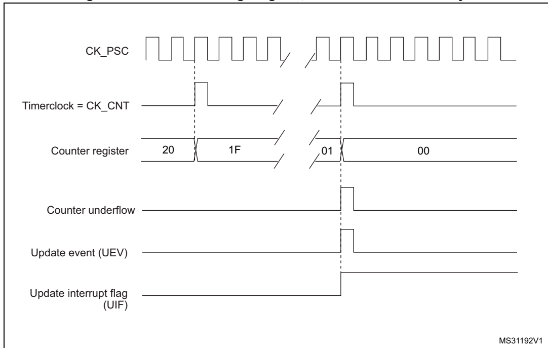
Figure 407. Counter timing diagram, update event with ARPE=1 (counter underflow)
