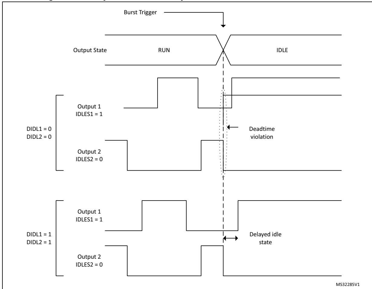
Figure 364. Delayed burst mode entry with deadtime enabled and IDLESx = 1
