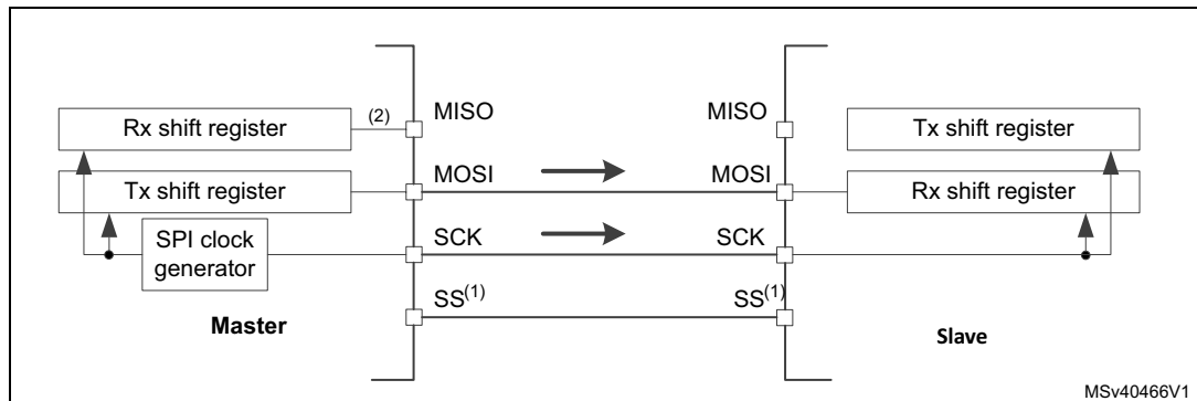
Figure 658. Simplex single master/single slave application (master in transmit-only/ slave in receive-only mode)
