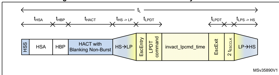
Figure 274. VLPSIZE for non-burst with sync events
