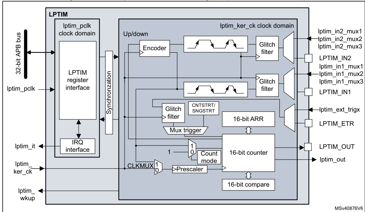
Figure 567. Low-power timer block diagram (LPTIM1 and LPTIM2)
