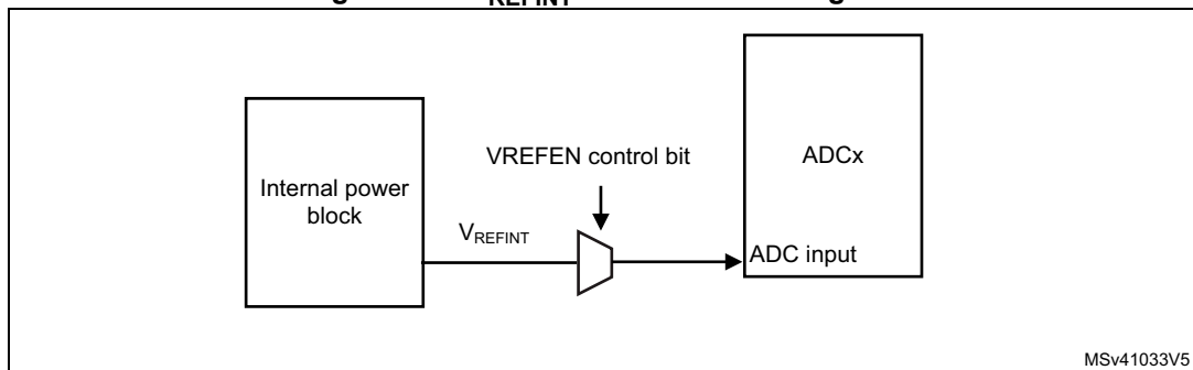
Figure 209. V_{REFINT} channel block diagram
