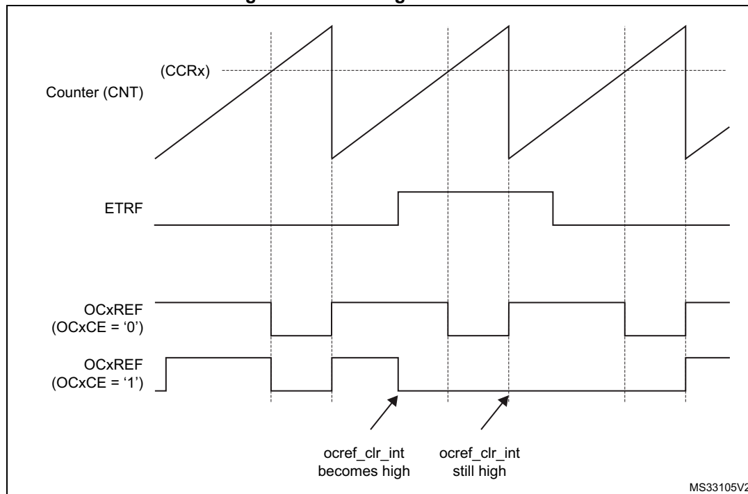
Figure 483. Clearing TIMx OCxREF
