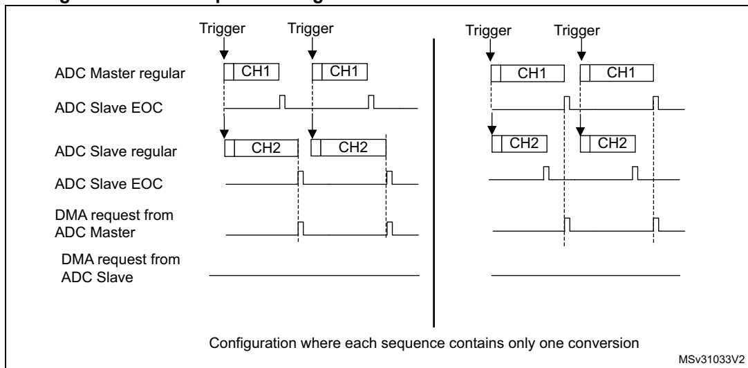
Figure 206. DMA requests in interleaved mode when DAMDF=0b10
