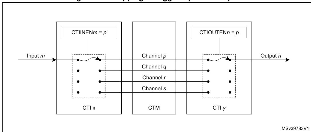
Figure 871. Mapping of trigger inputs to outputs
