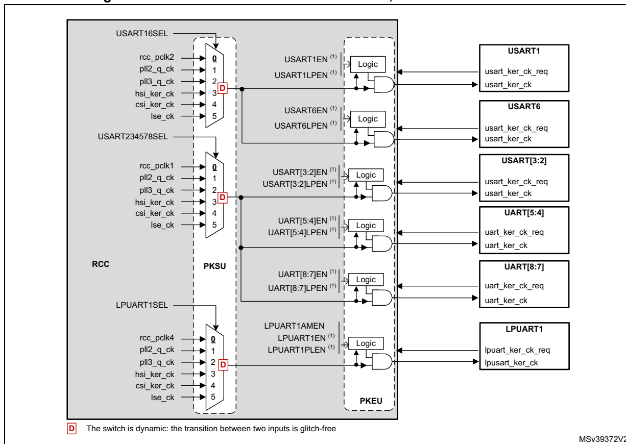
Figure 58. Kernel clock distribution for UARTs, USARTs and LPUART1
