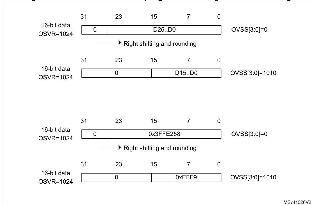
Figure 185. 16-bit result oversampling with 10-bits right shift and rounding
