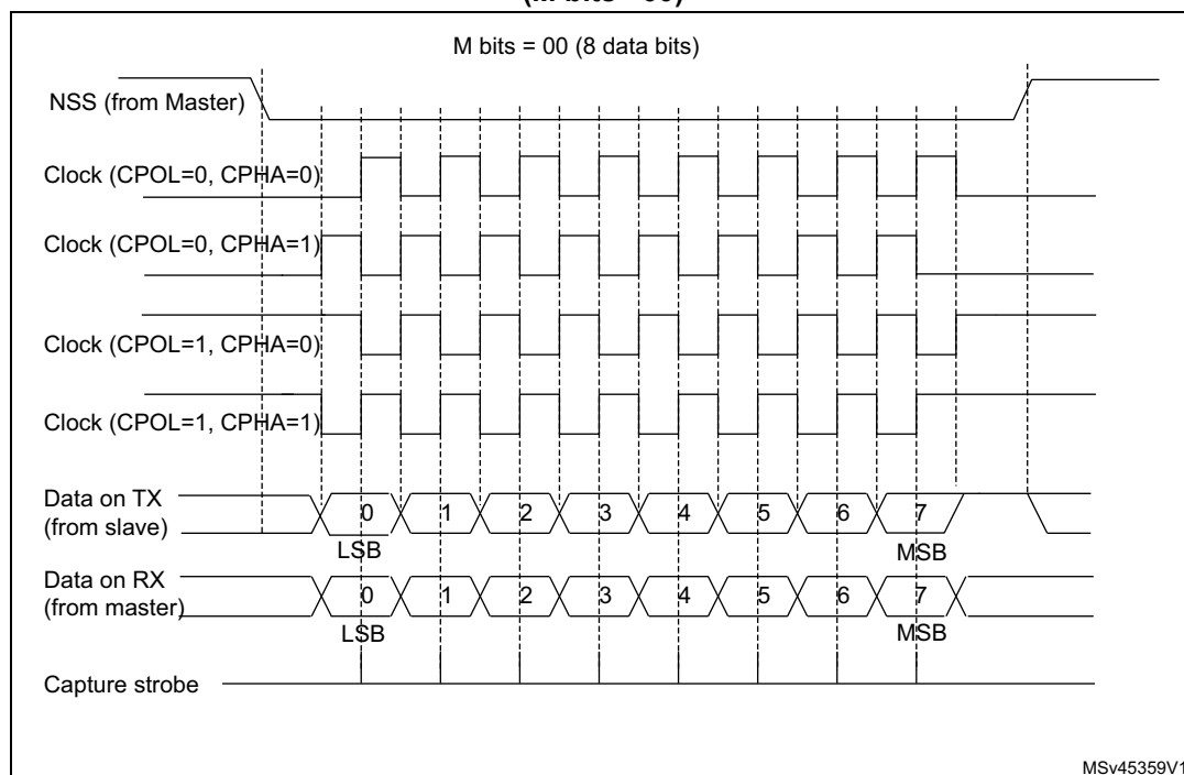
Figure 629. USART data clock timing diagram in synchronous slave mode (M bits =00)
