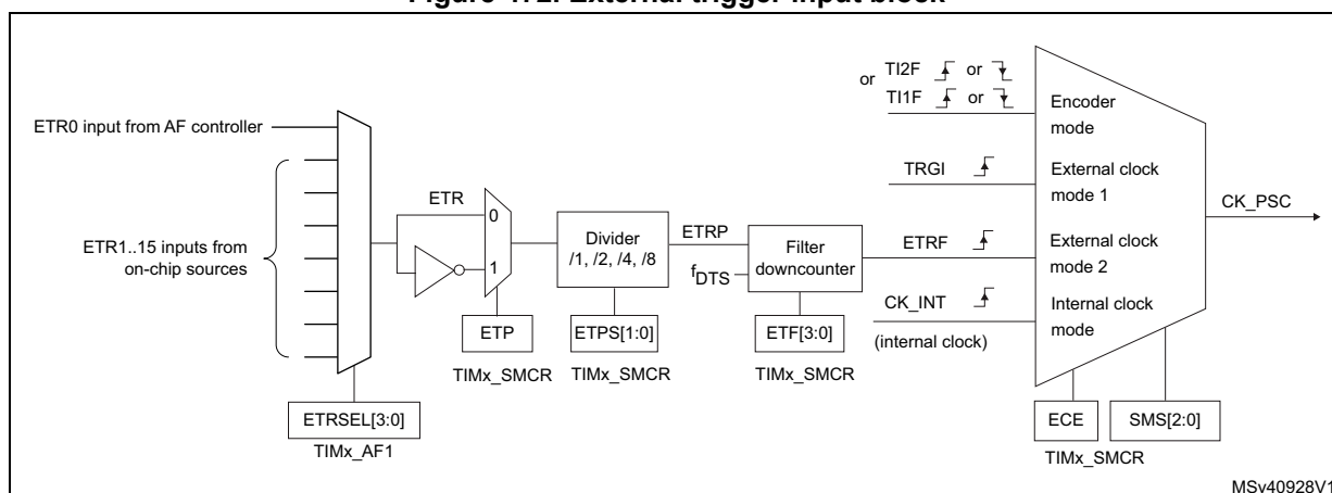
Figure 472. External trigger input block
