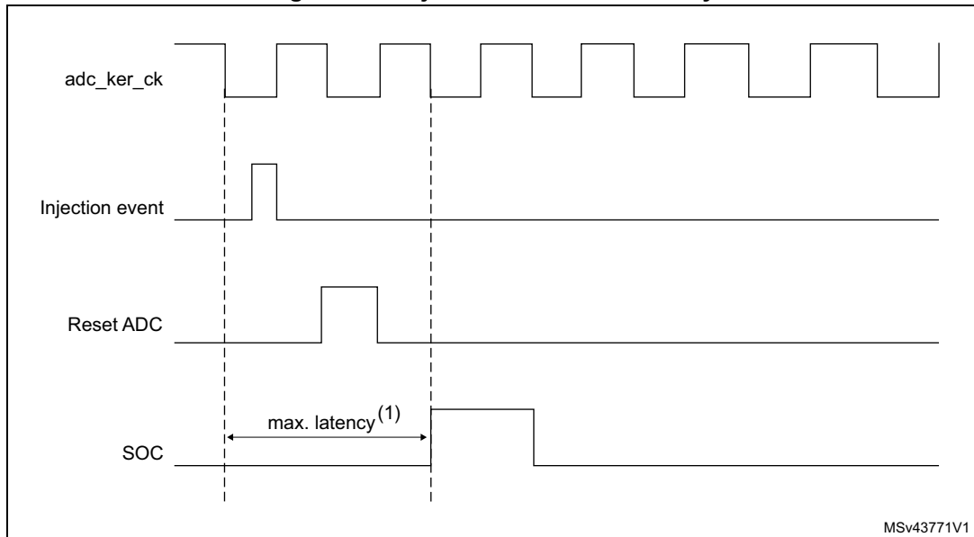
Figure 153. Injected conversion latency
