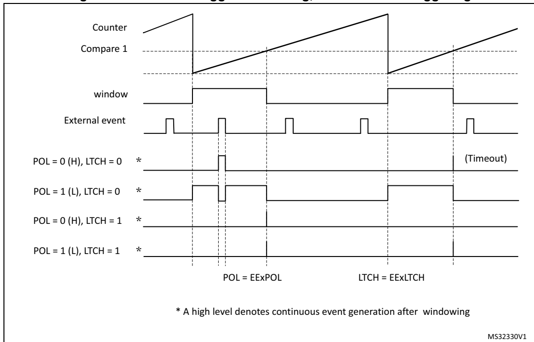
Figure 355. External trigger windowing, level sensitive triggering
