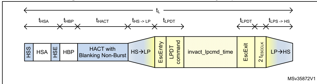
Figure 273. VLPSIZE for non-burst with sync pulses
