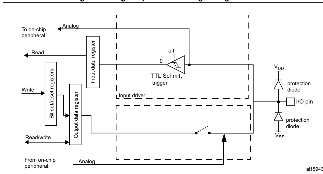
Figure 80. High impedance-analog configuration
