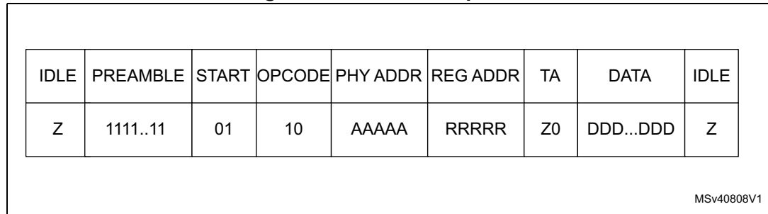
Figure 838. Read data packet
