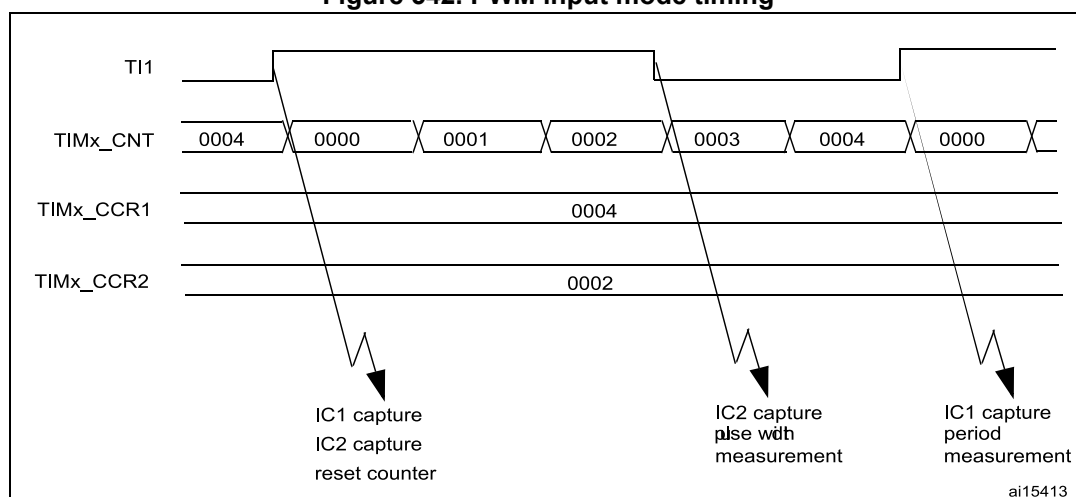
Figure 542. PWM input mode timing
