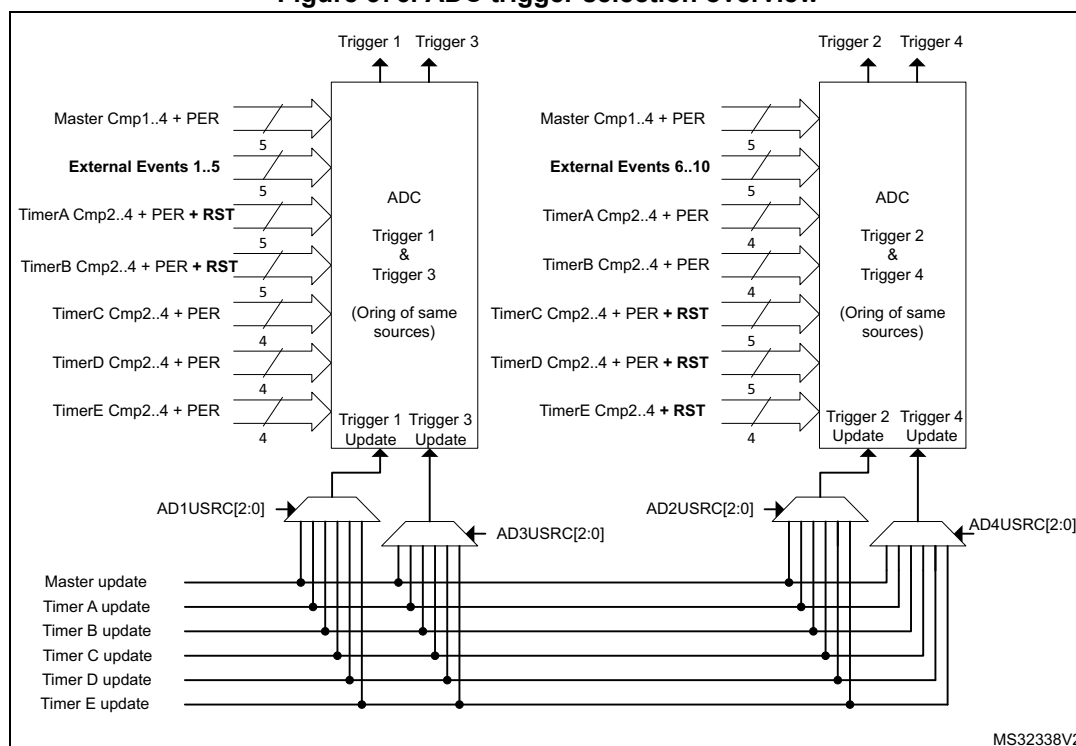
Figure 376. ADC trigger selection overview
