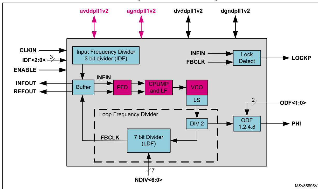
Figure 286. PLL block diagram
