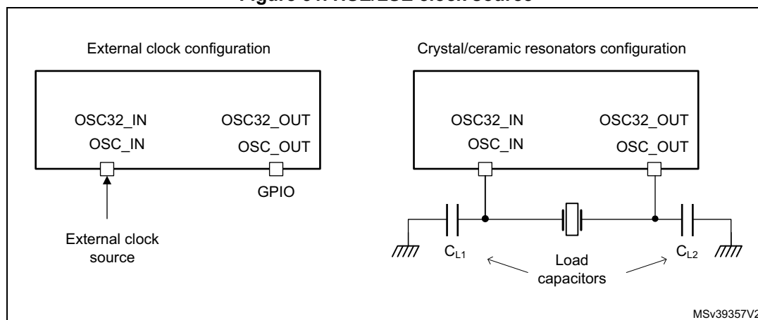
Figure 51. HSE/LSE clock source
