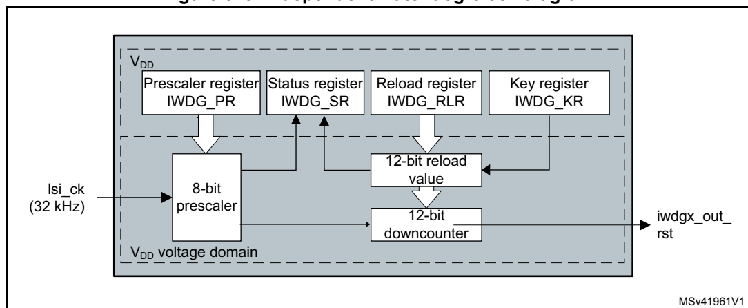
Figure 579. Independent watchdog block diagram
