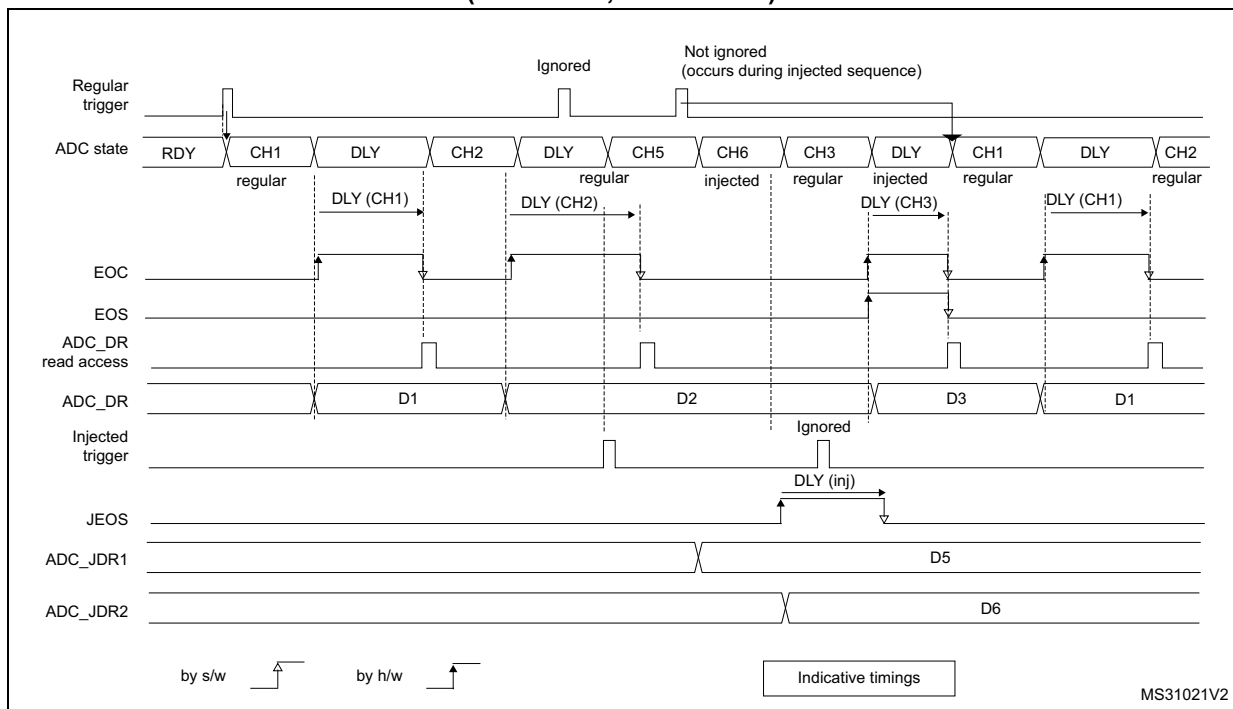
Figure 176. AUTDLY=1, regular HW conversions interrupted by injected conversions (DISCEN=0; JDISCEN=0)
