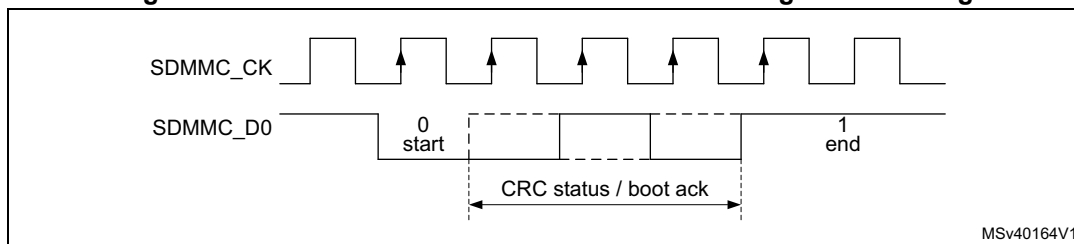
Figure 754. DDR mode CRC status / boot acknowledgment clocking
