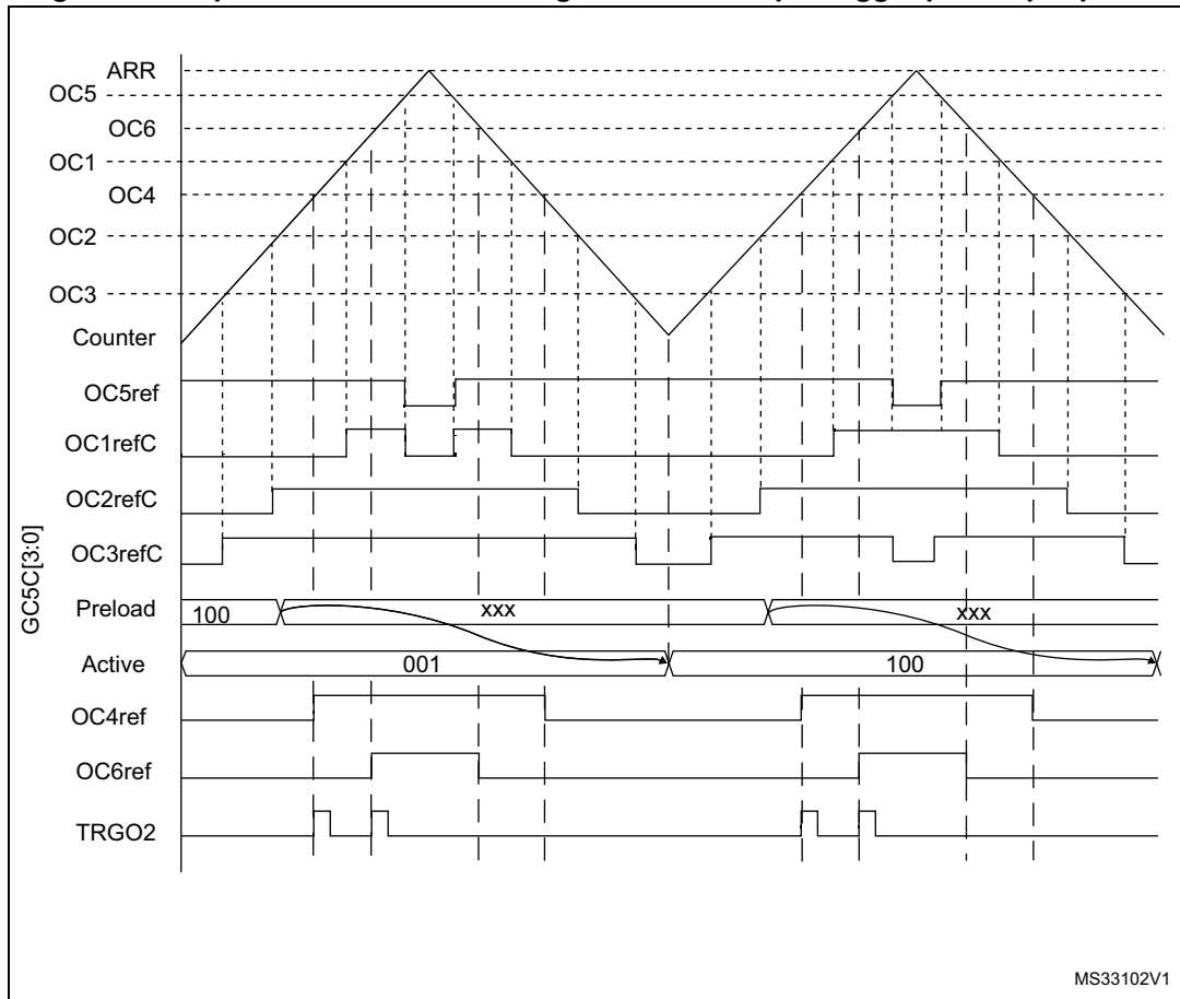
Figure 428. 3-phase combined PWM signals with multiple trigger pulses per period
