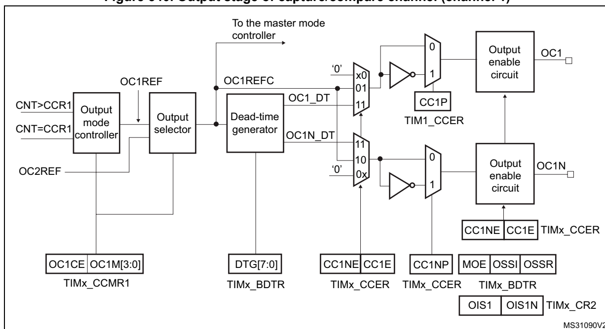
Figure 540. Output stage of capture/compare channel (channel 1)
