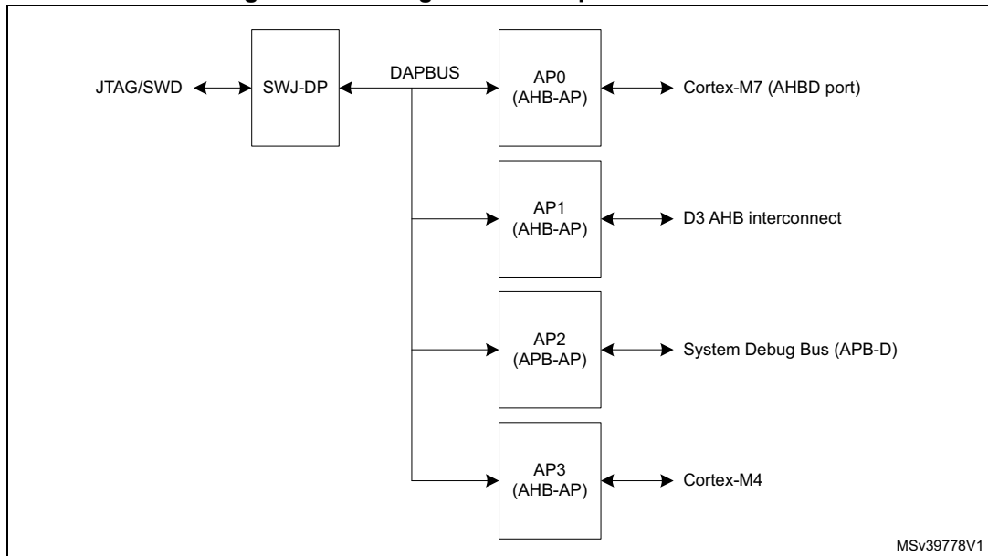
Figure 867. Debug and access port connections
