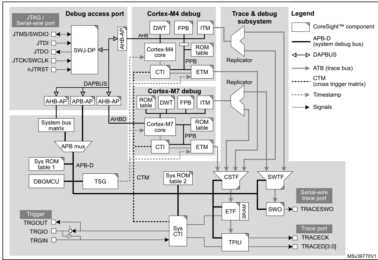
Figure 862. Block diagram of debug infrastructure
