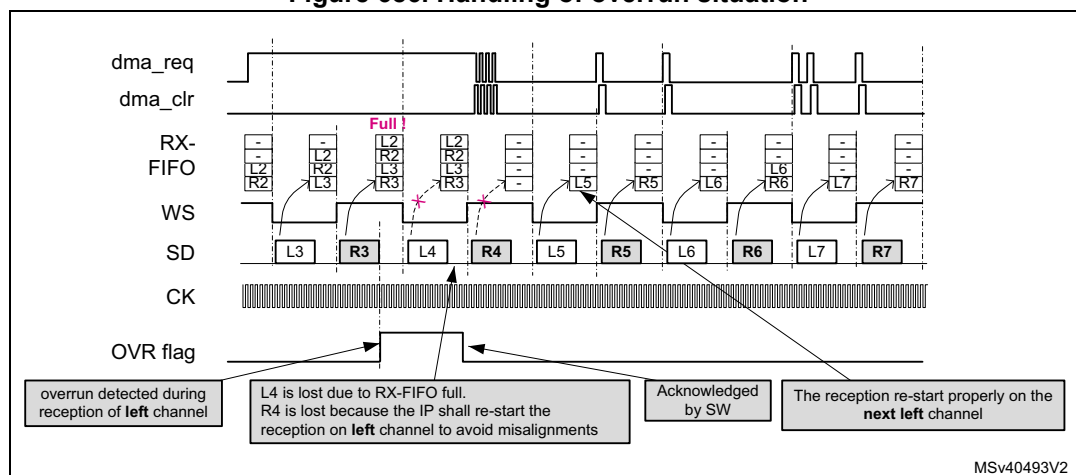
Figure 686. Handling of overrun situation
