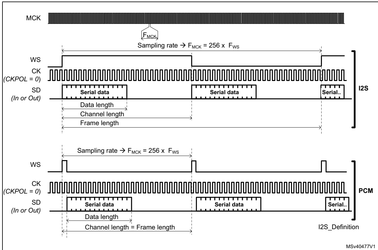
Figure 670. Waveform examples
