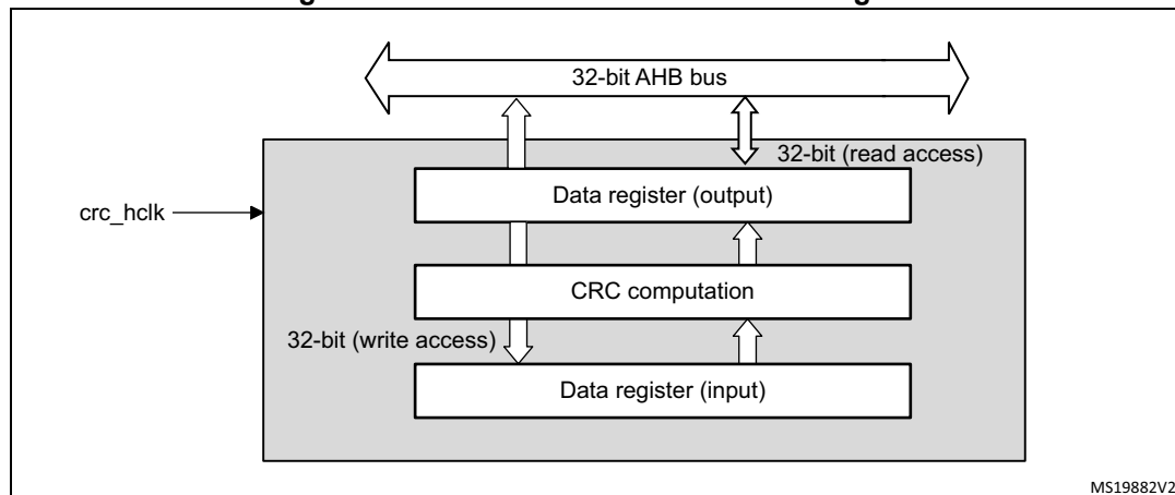
Figure 101. CRC calculation unit block diagram
