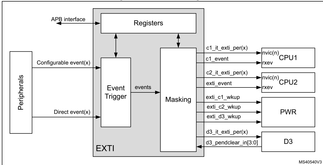
Figure 95. EXTI block diagram
