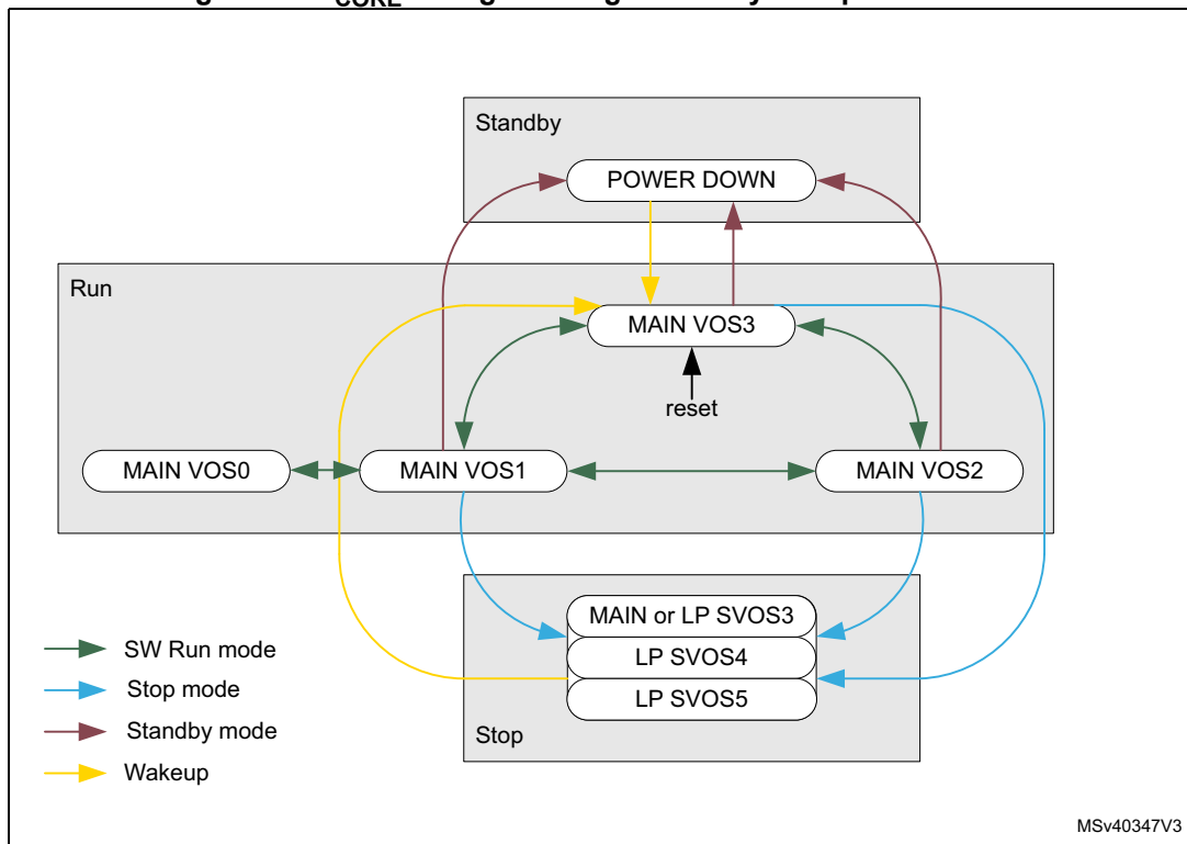
Figure 36. V CORE voltage scaling versus system power modes
