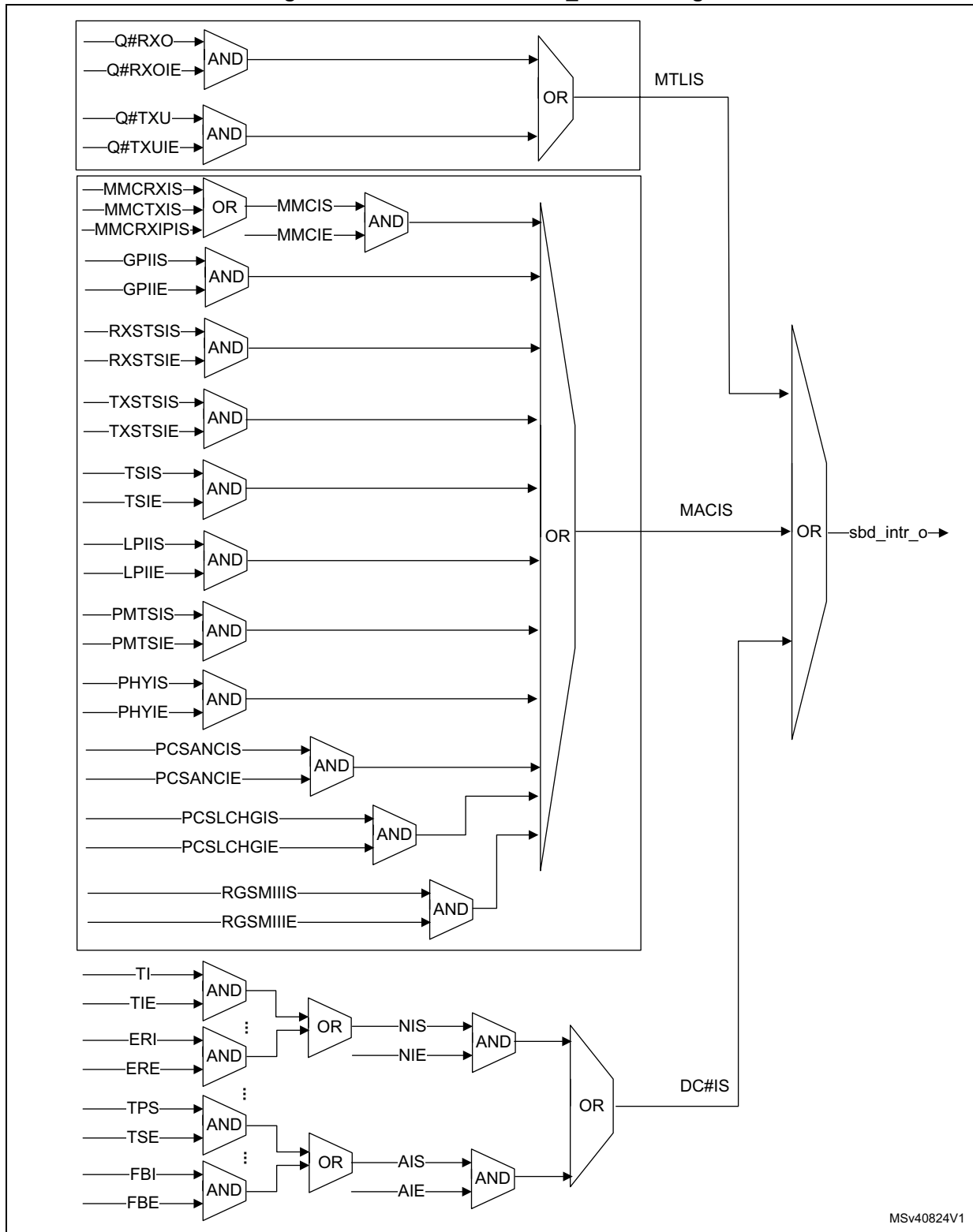
Figure 851. Generation of ETH_DMAISR flags
