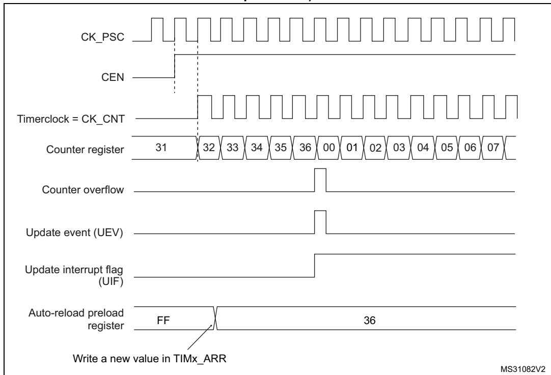
Figure 506. Counter timing diagram, update event when ARPE=0 (TIMx_ARR not preloaded)
