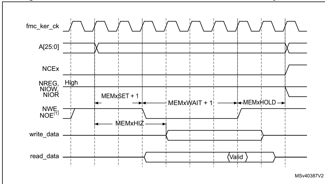
Figure 122. NAND Flash controller waveforms for common memory access
