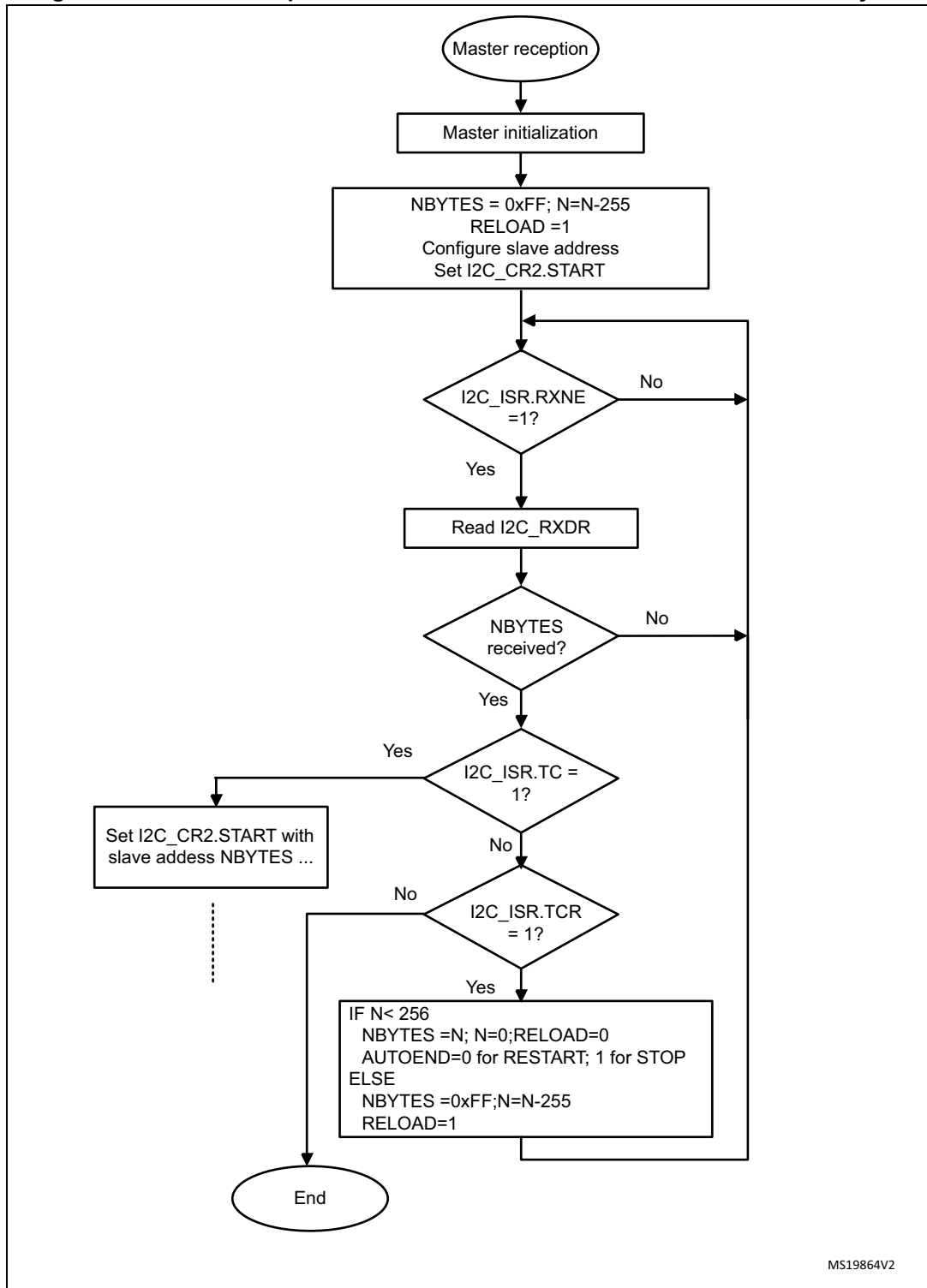
Figure 604. Transfer sequence flowchart for I2C master receiver for N >255 bytes
