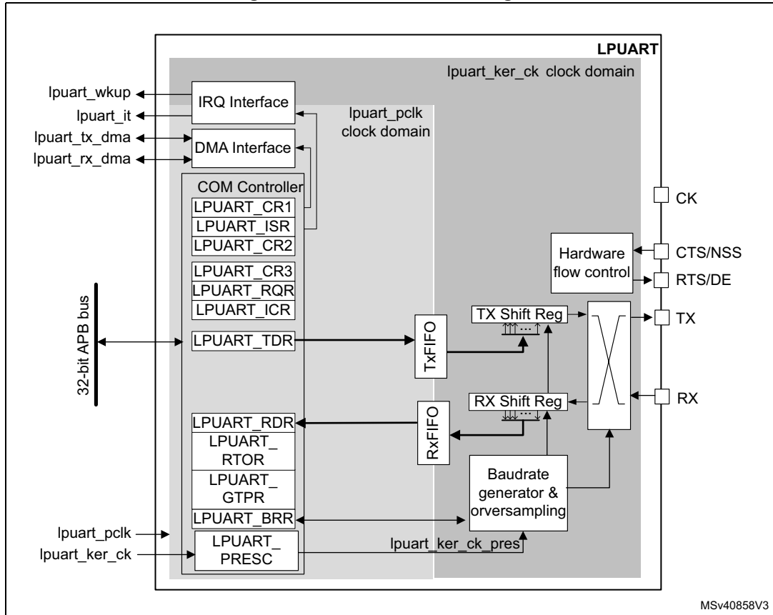
Figure 641. LPUART block diagram
