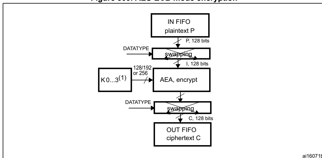
Figure 309. AES-ECB mode encryption
