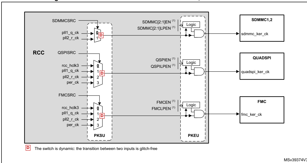
Figure 60. Kernel clock distribution for SDMMC, QUADSPI and FMC
