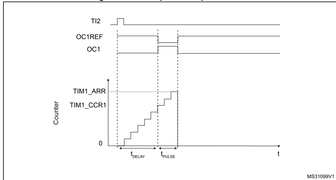
Figure 439. Example of one pulse mode.
