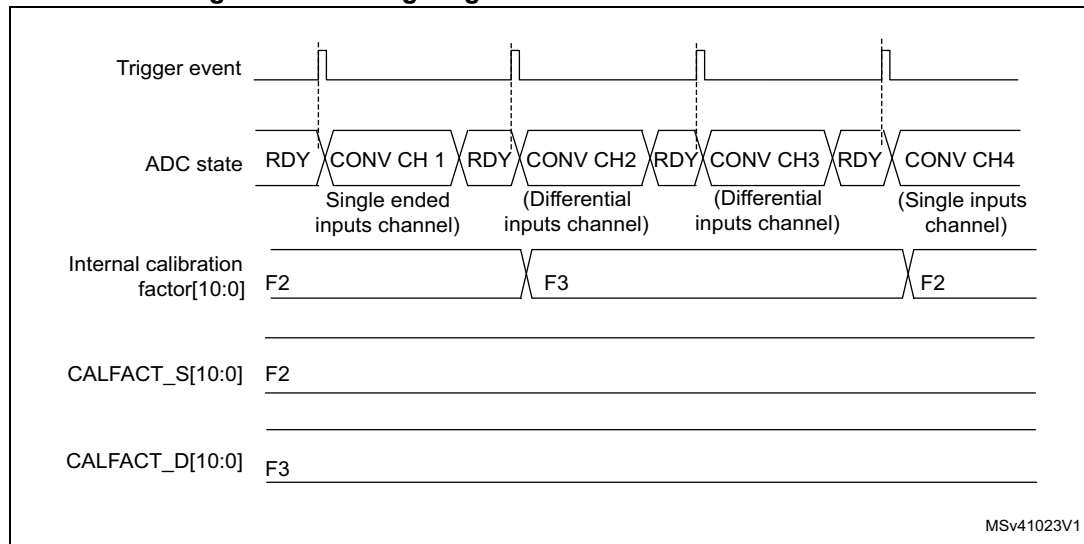
Figure 147. Mixing single-ended and differential channels
