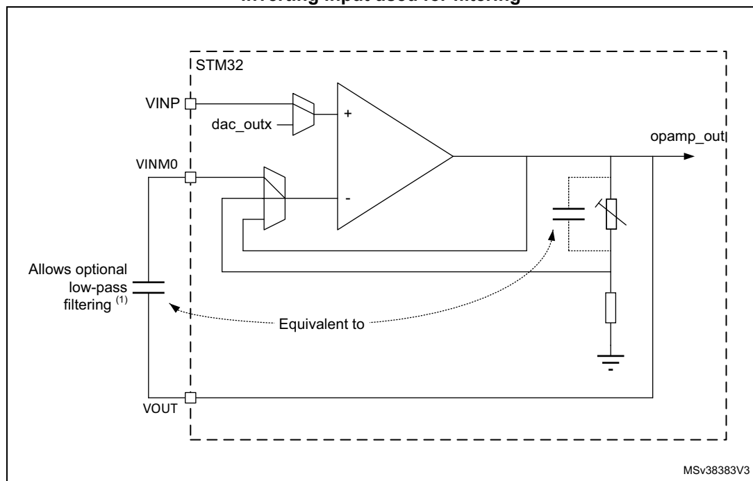
Figure 227. PGA mode, internal gain setting (x2/x4/x8/x16), inverting input used for filtering
