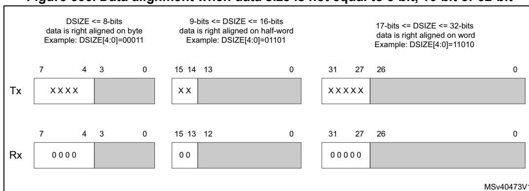
Figure 666. Data alignment when data size is not equal to 8-bit, 16-bit or 32-bit
