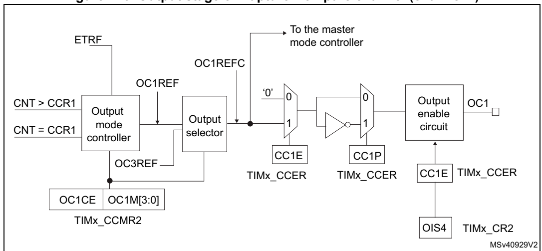
Figure 476. Output stage of Capture/Compare channel (channel 1)
