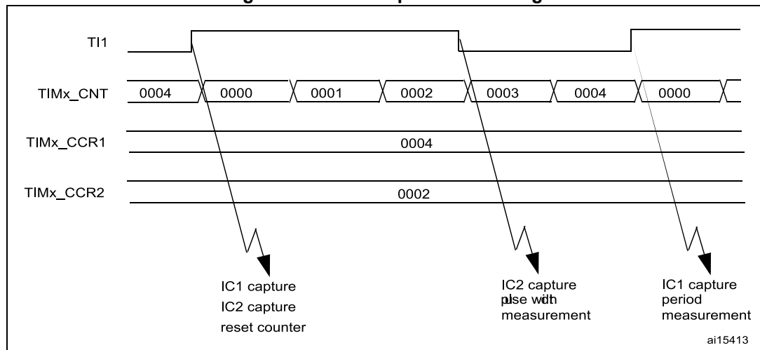
Figure 422. PWM input mode timing
