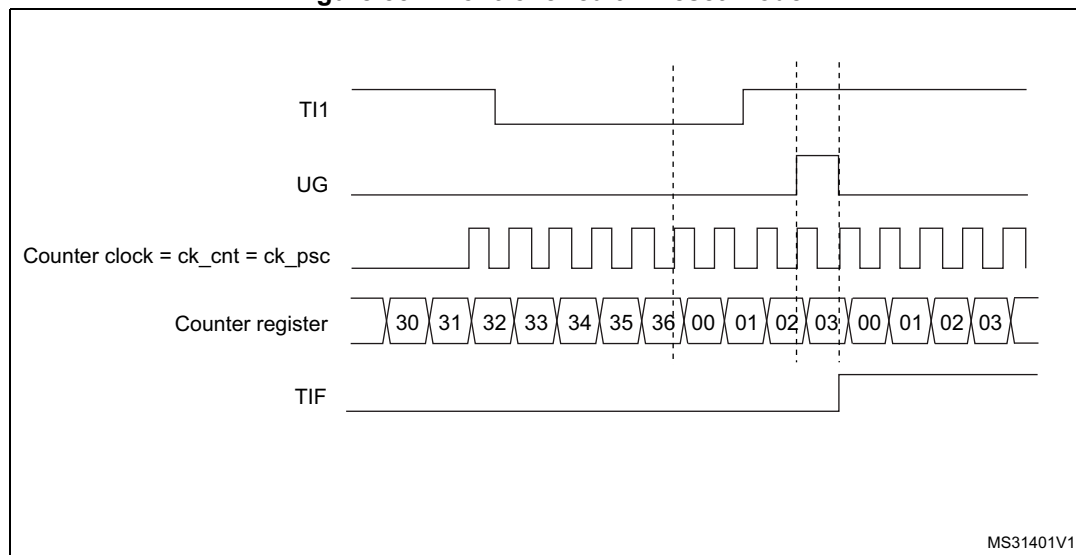
Figure 554. Control circuit in reset mode
