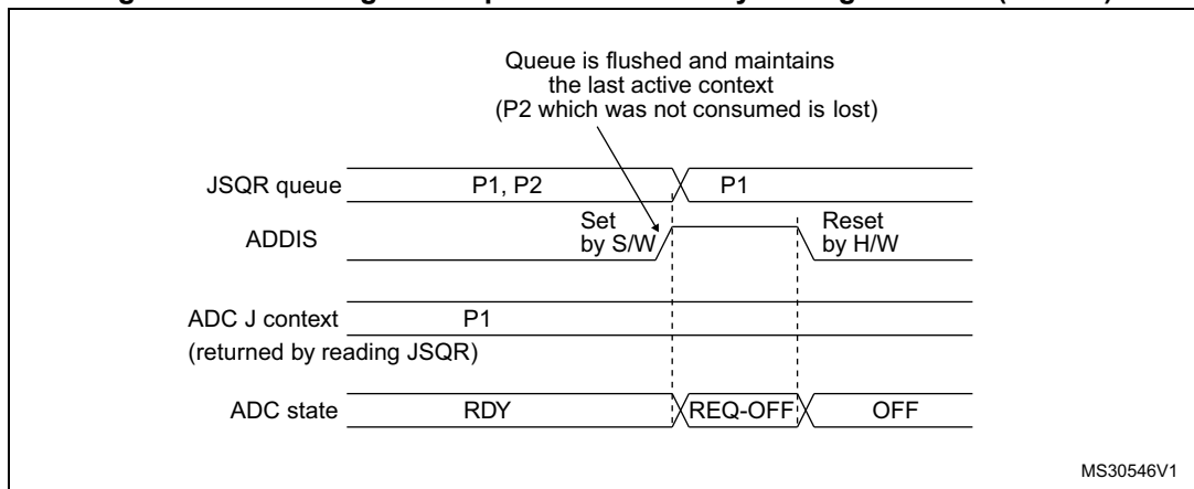
Figure 164. Flushing JSQR queue of context by setting ADDIS=1 (JQM=0)
