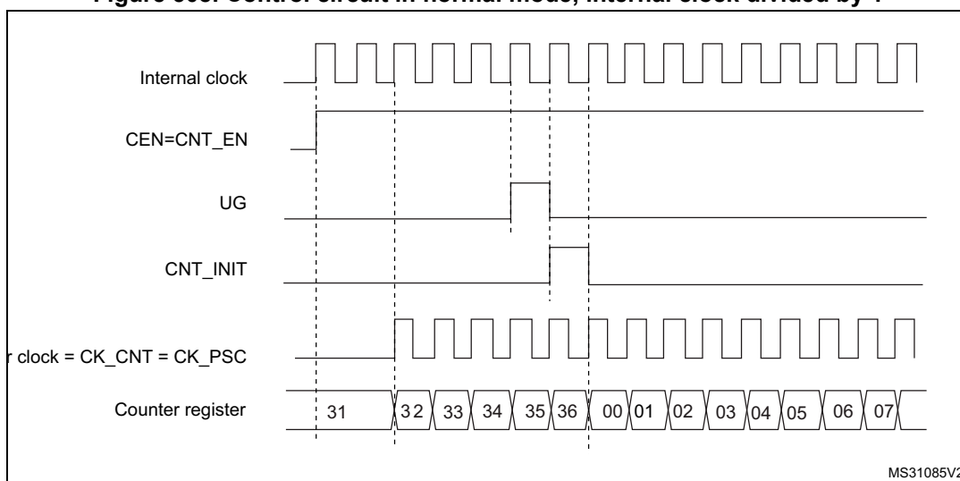
Figure 508. Control circuit in normal mode, internal clock divided by 1
