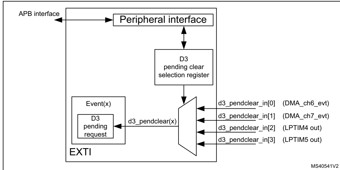
Figure 100. D3 domain Pending request clear logic
