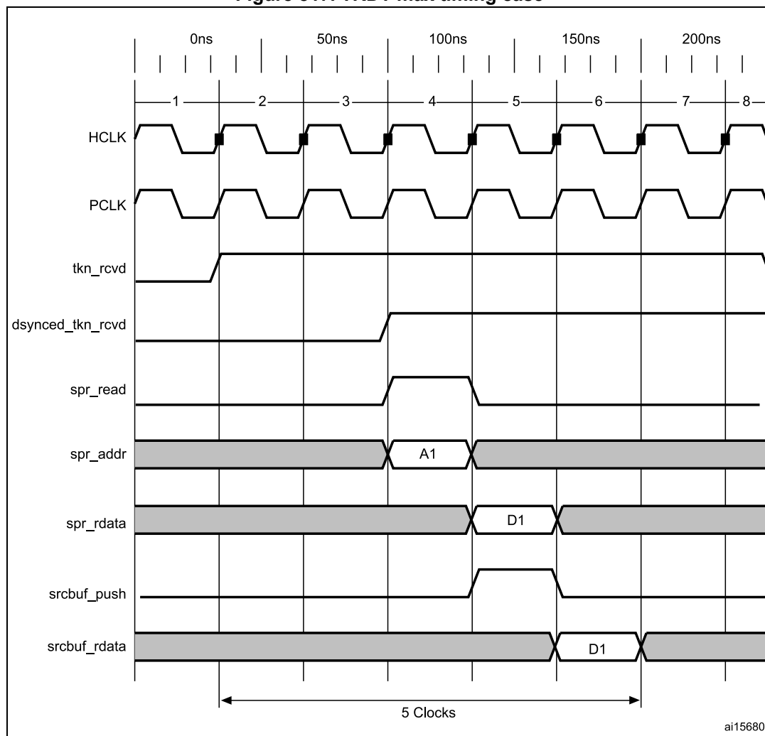
Figure 817. TRDT max timing case
