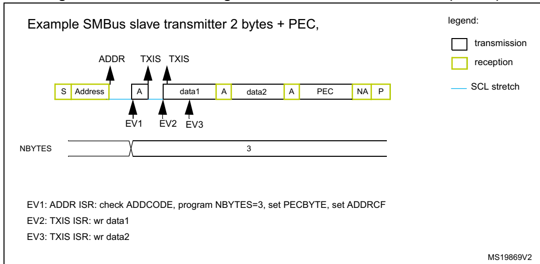
Figure 608. Transfer bus diagrams for SMBus slave transmitter (SBC=1)
