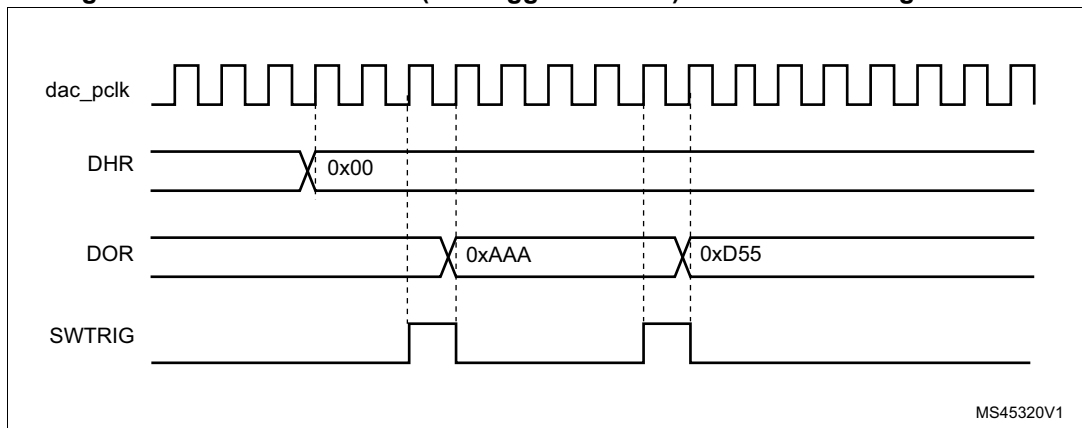
Figure 215. DAC conversion (SW trigger enabled) with LFSR wave generation
