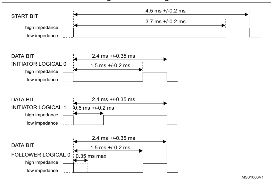
Figure 855. Bit timings
