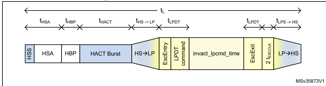
Figure 275. VLPSIZE for burst mode
