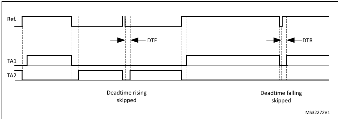
Figure 341. Complementary outputs for low pulse width (SDTRx = SDTFx = 0)
