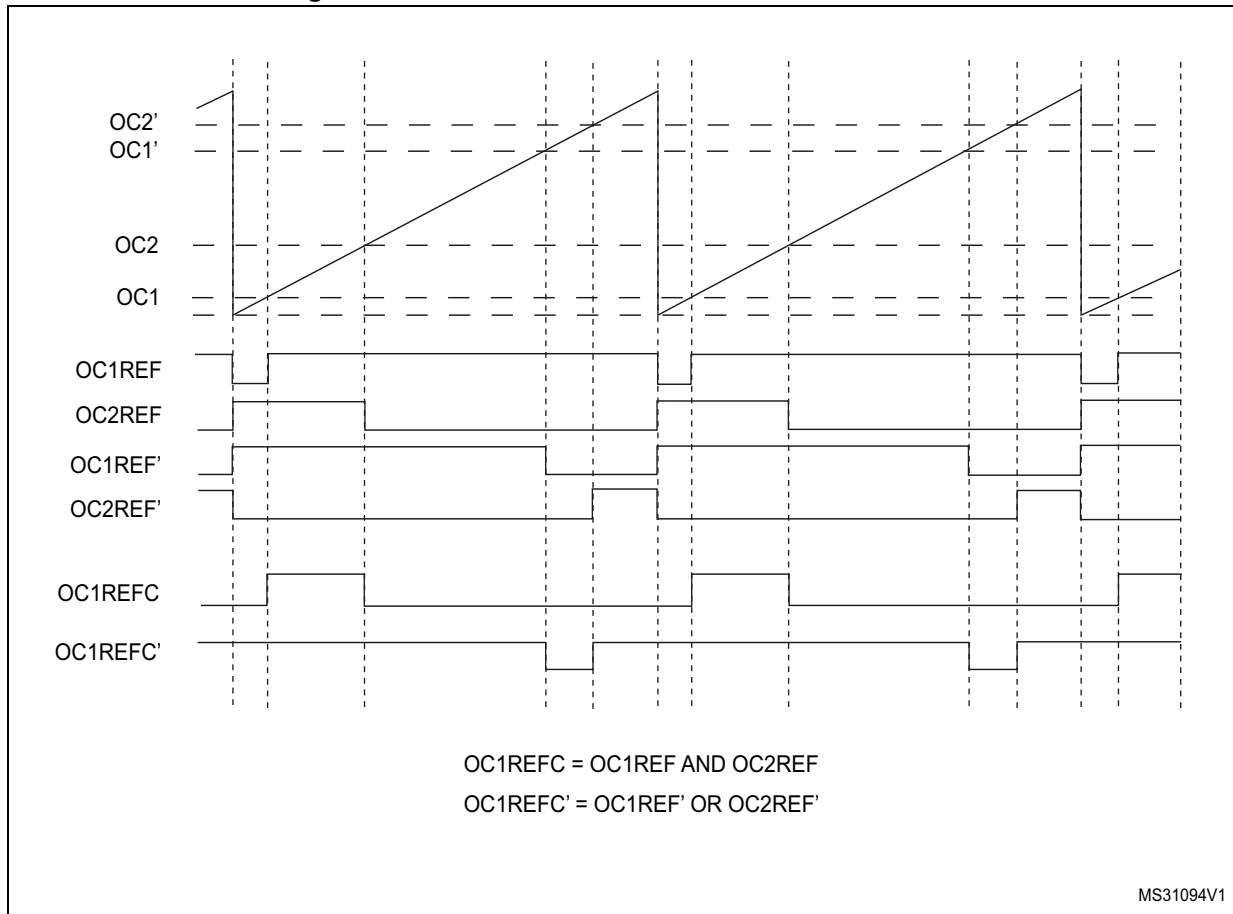
Figure 517. Combined PWM mode on channel 1 and 2
