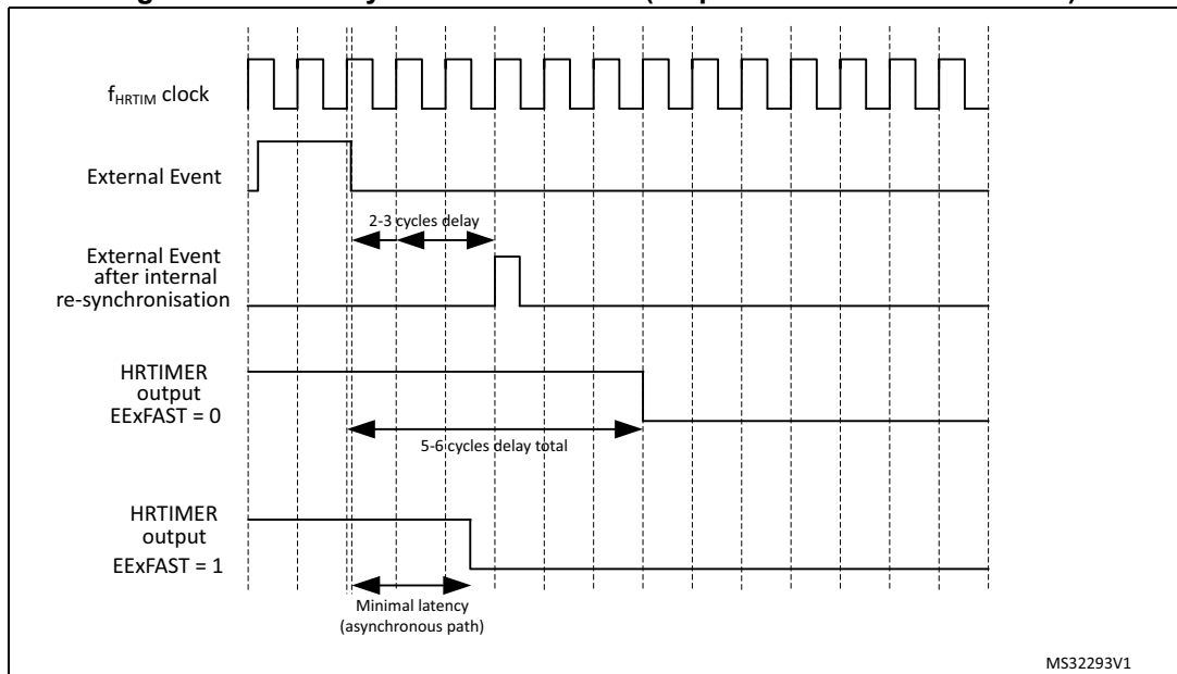
Figure 348. Latency to external events (output reset on external event)
