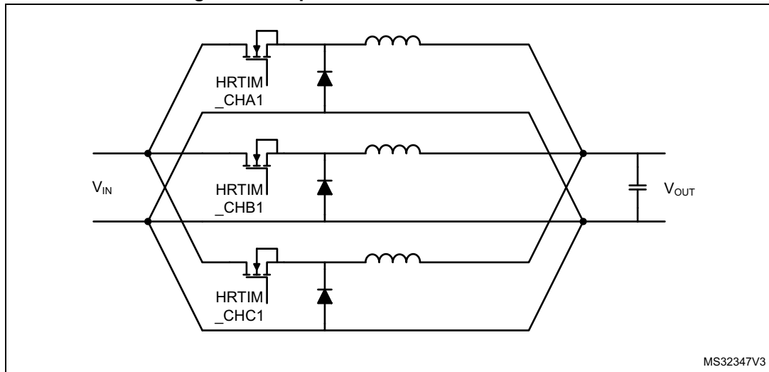
Figure 385. 3-phase interleaved buck converter
