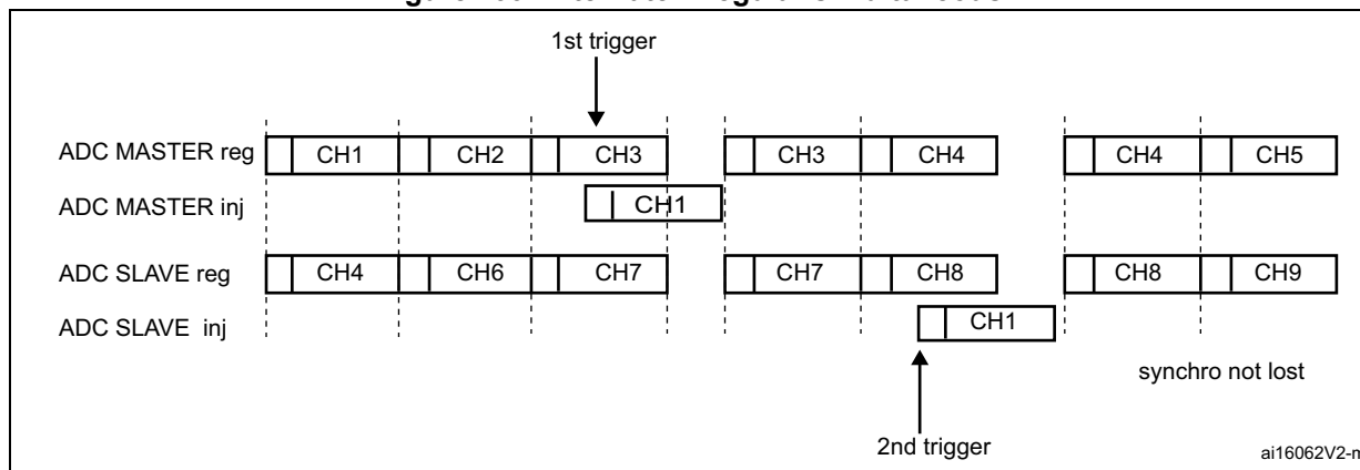
Figure 199. Alternate + regular simultaneous
