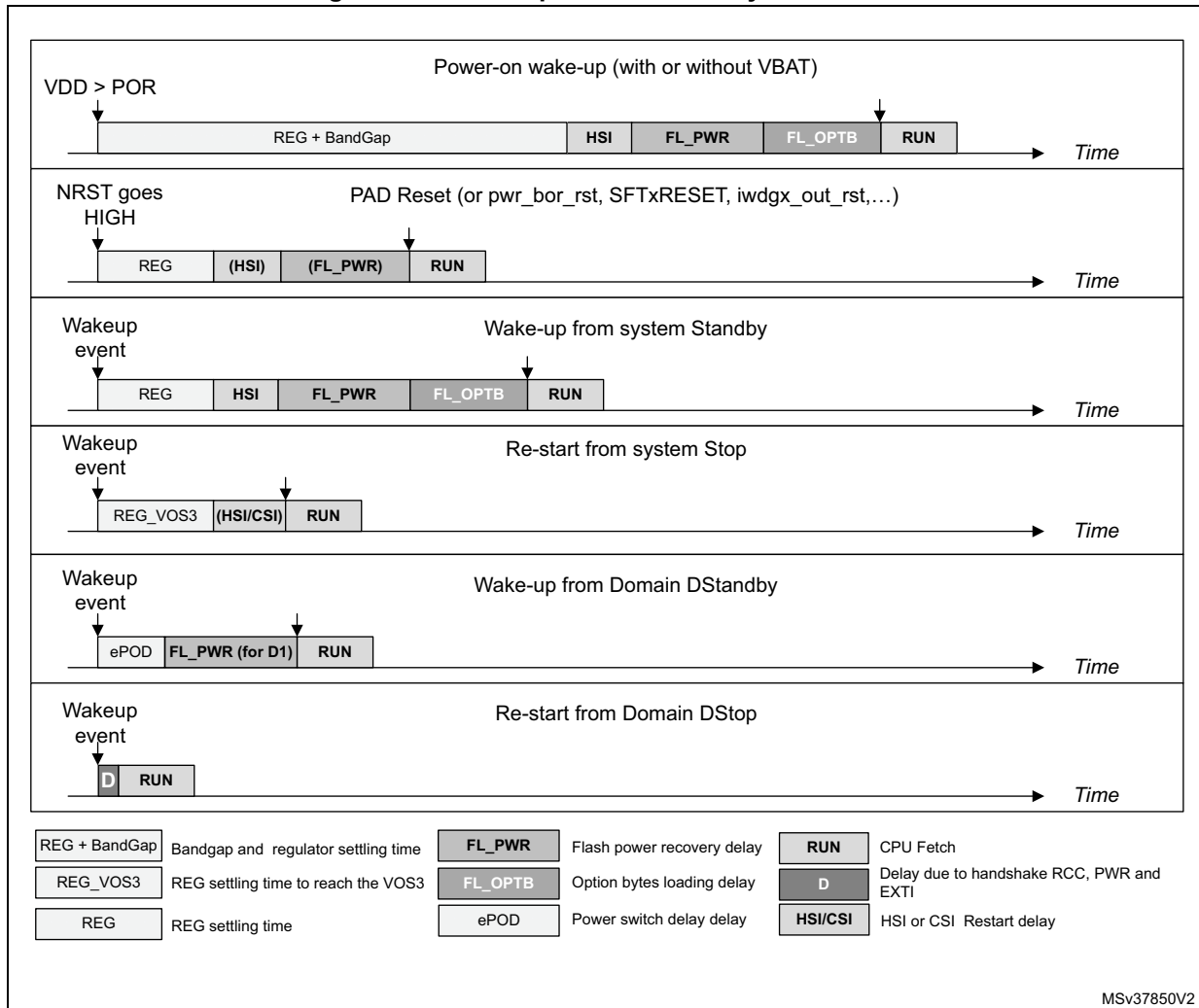
Figure 49. Boot sequences versus system states
