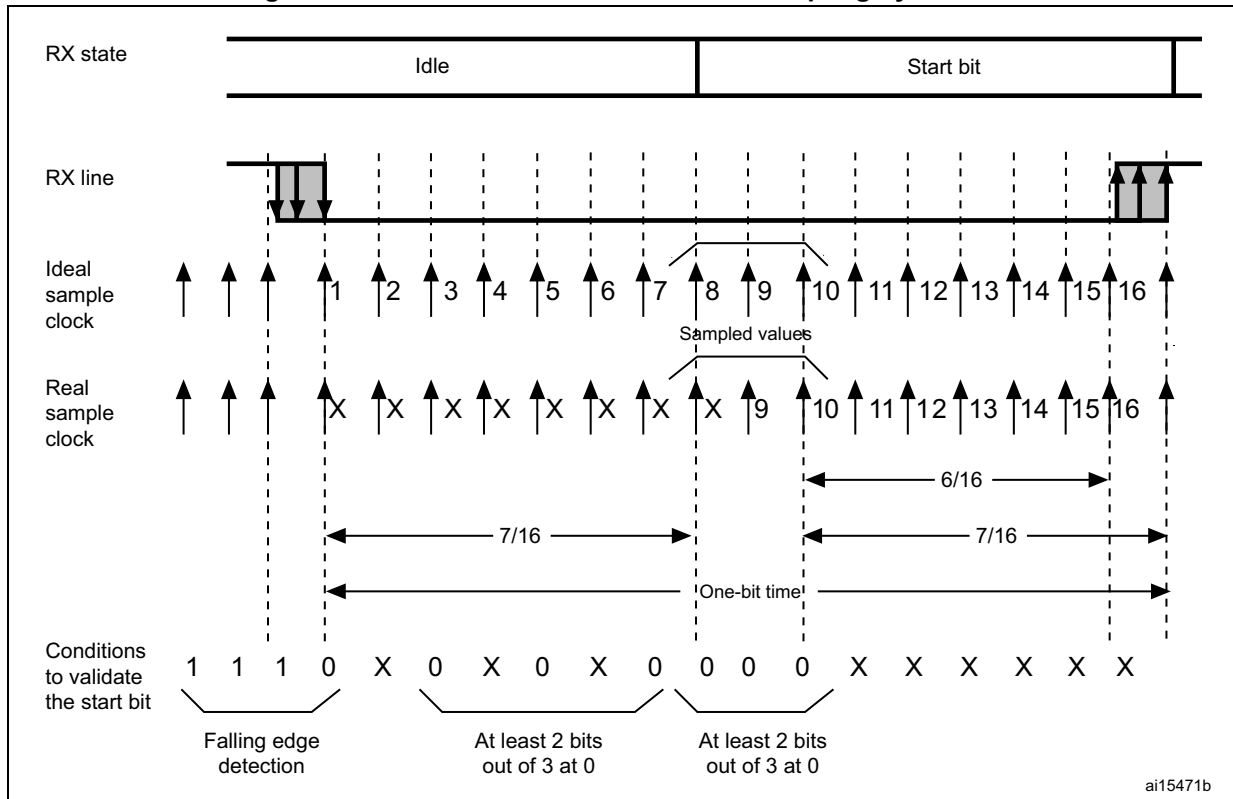
Figure 618. Start bit detection when oversampling by 16 or 8
