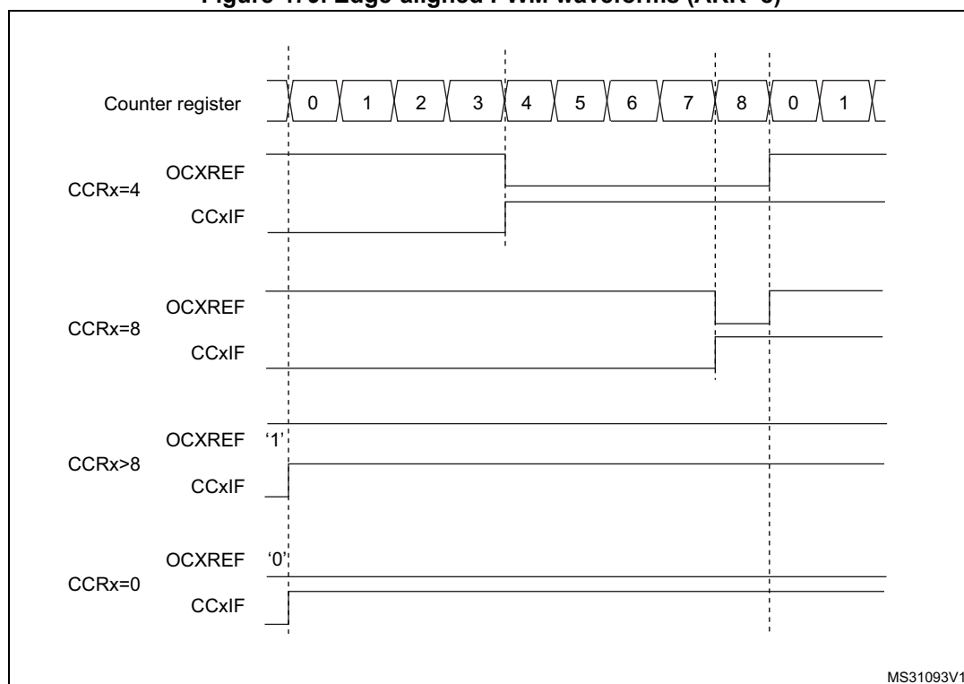
Figure 479. Edge-aligned PWM waveforms (ARR=8)
