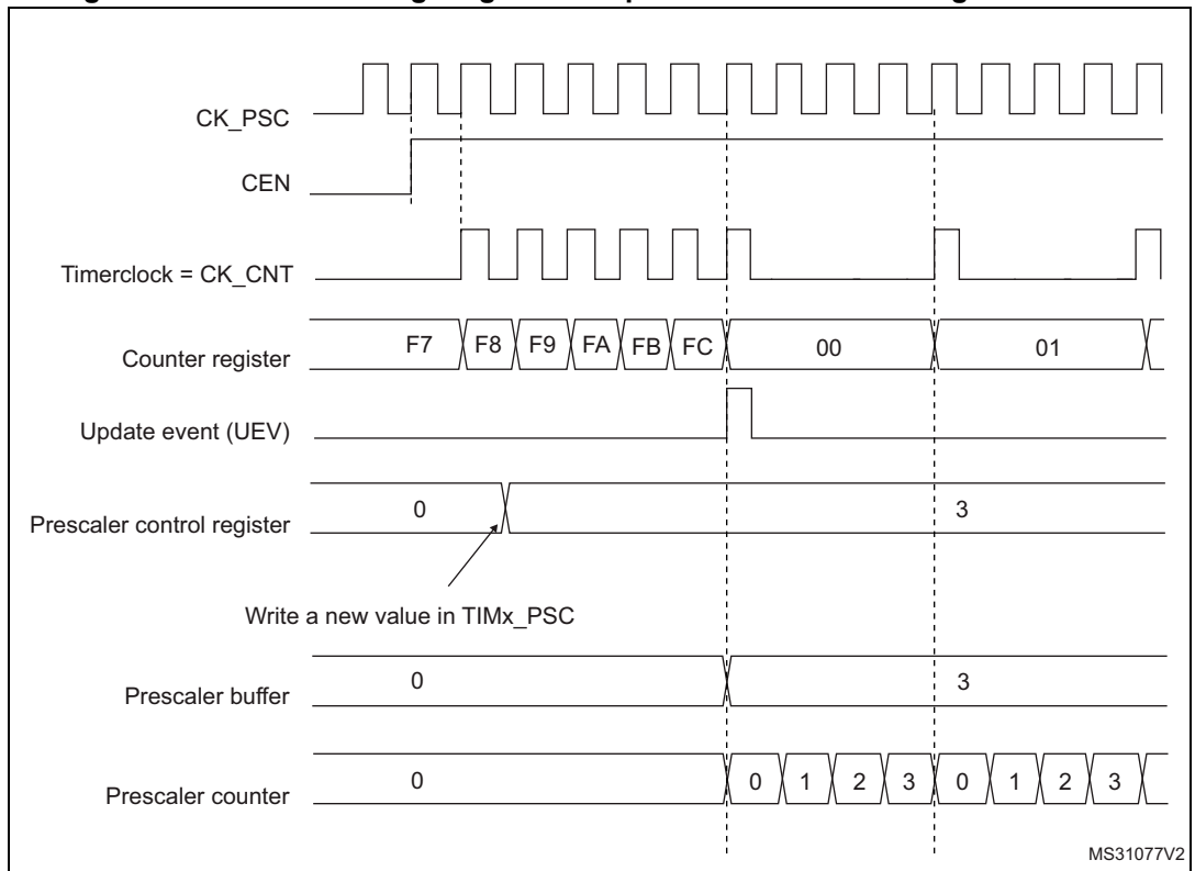
Figure 527. Counter timing diagram with prescaler division change from 1 to 4
