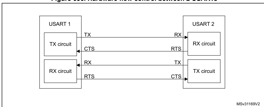
Figure 636. Hardware flow control between 2 USARTs
