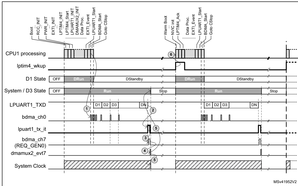
Figure 46. Timing diagram of LPUART1 transmission with D3 domain in Autonomous mode
