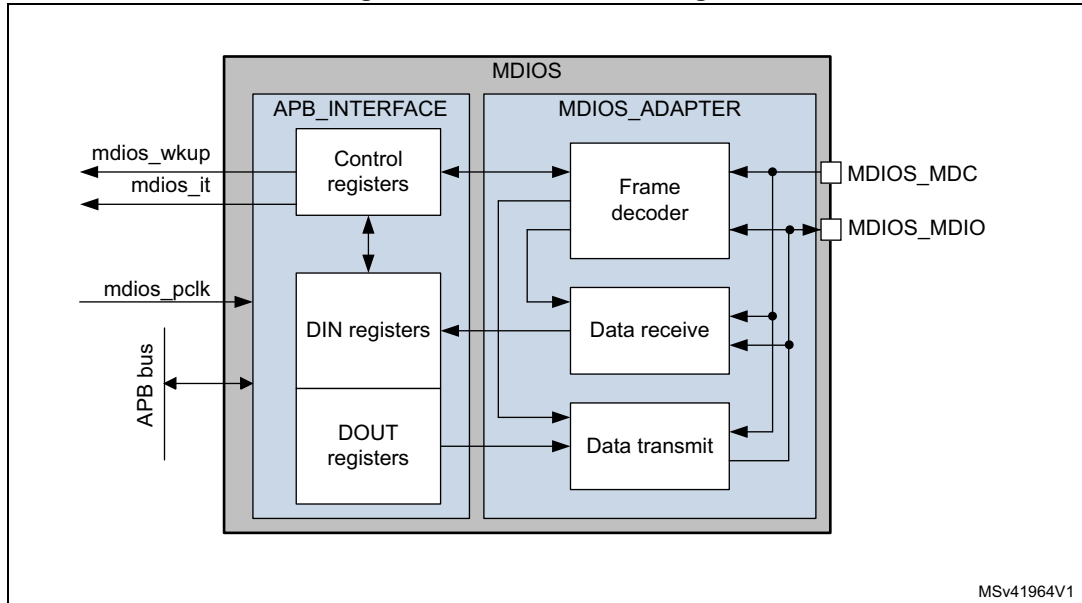
Figure 739. MDIOS block diagram
