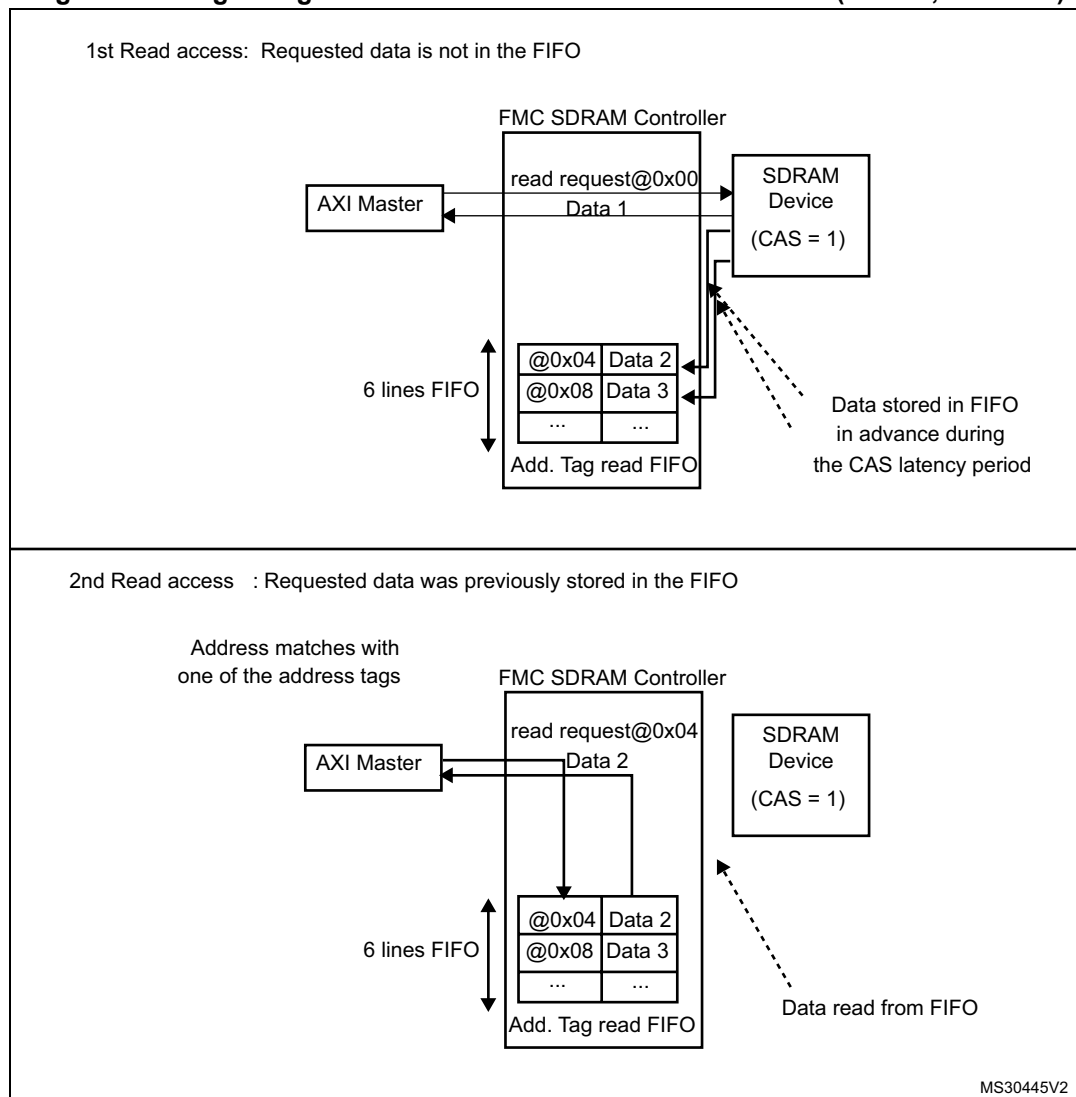
Figure 126. Logic diagram of Read access with RBURST bit set (CAS=2, RPIPE=0)
