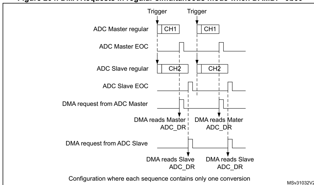
Figure 204. DMA Requests in regular simultaneous mode when DAMDF=0b00
