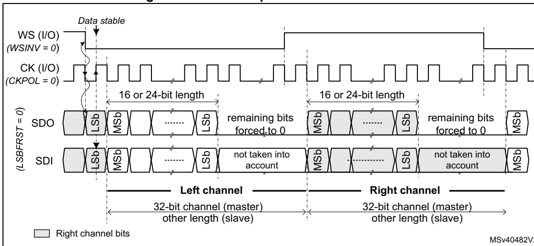
Figure 672. I2S Philips standard waveforms
