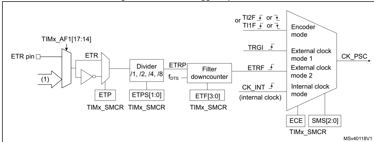
Figure 415. External trigger input block
