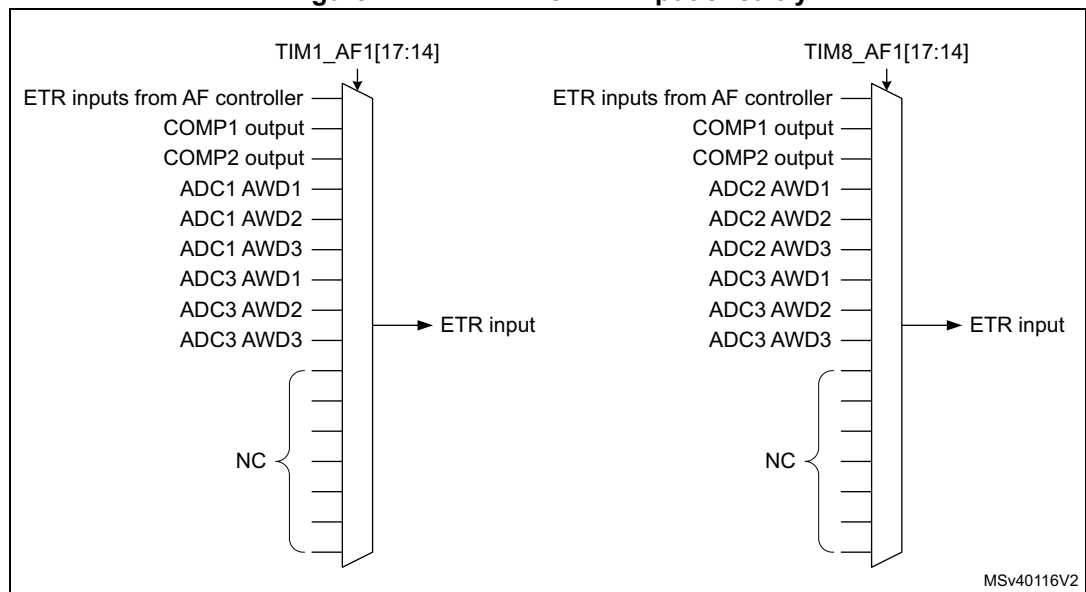
Figure 411. TIM1/TIM8 ETR input circuitry
