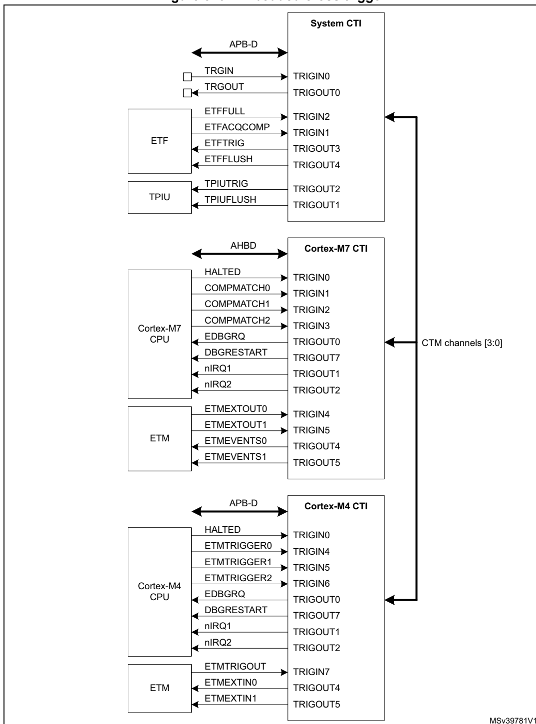
Figure 870. Embedded cross trigger
