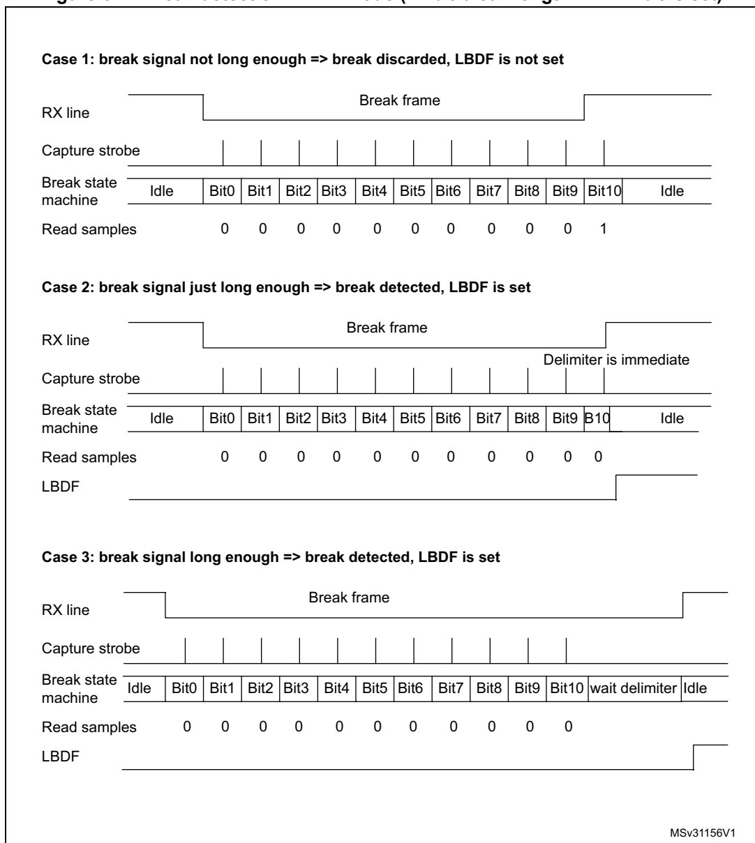
Figure 624. Break detection in LIN mode (11-bit break length - LBDL bit is set)
