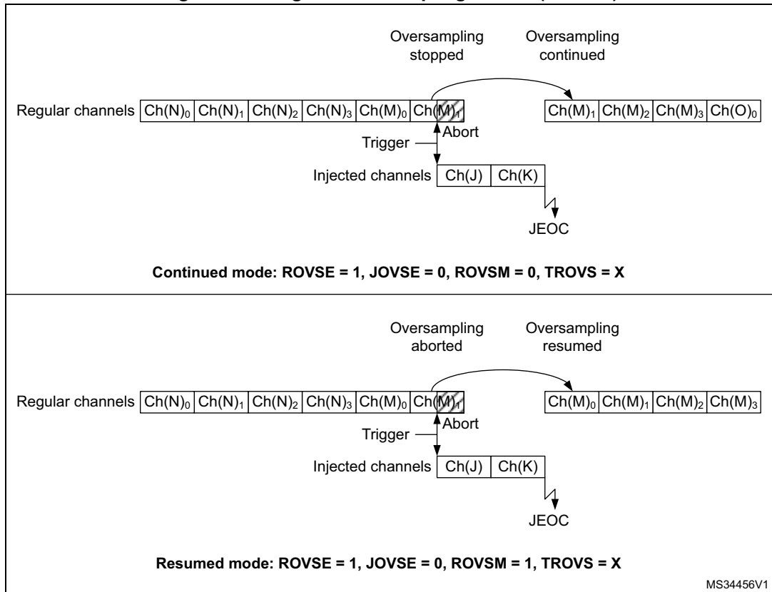
Figure 187. Regular oversampling modes (4x ratio)
