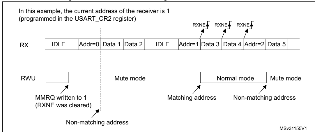
Figure 623. Mute mode using address mark detection
