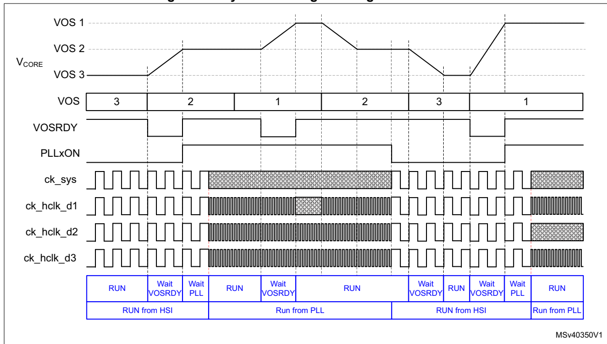
Figure 38. Dynamic voltage scaling in Run mode
