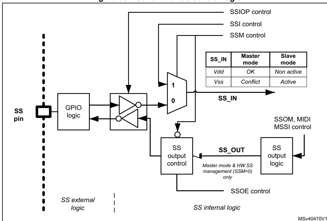
Figure 662. Scheme of SS control logic
