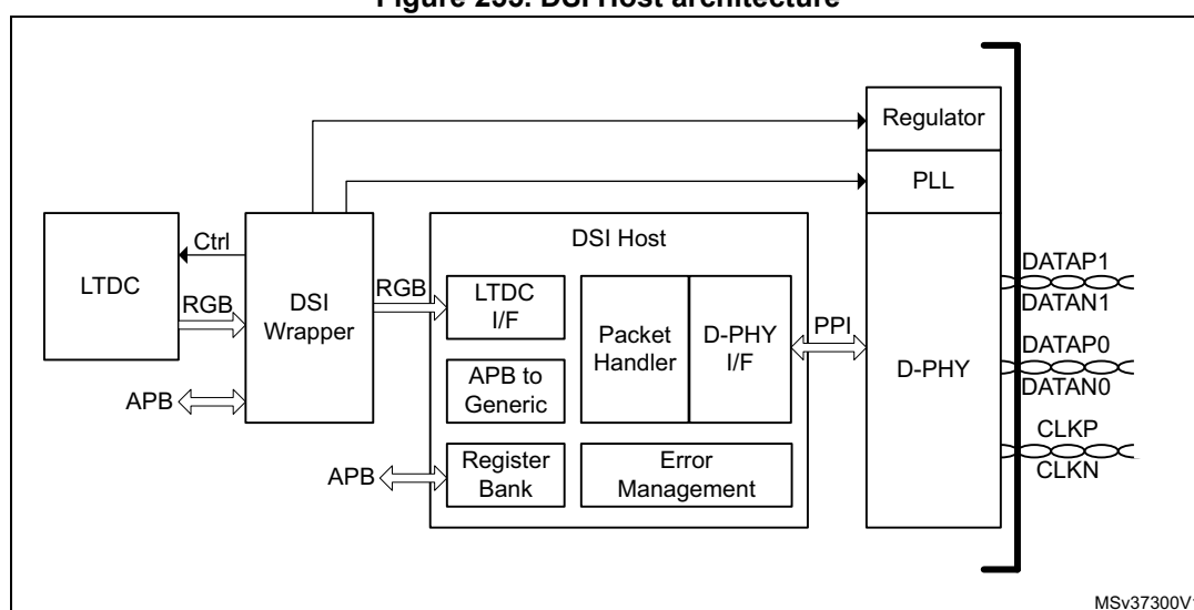
Figure 255. DSI Host architecture
