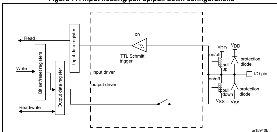
Figure 77. Input floating/pull up/pull down configurations
