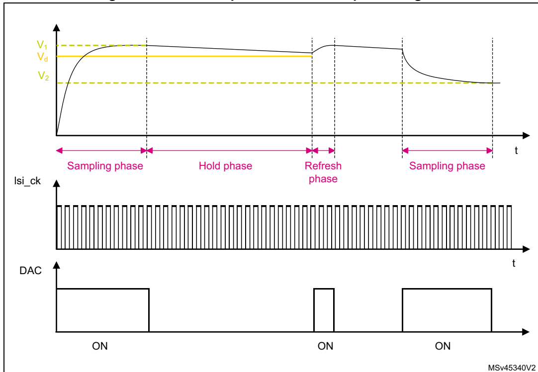
Figure 218. DAC Sample and Hold mode phase diagram
