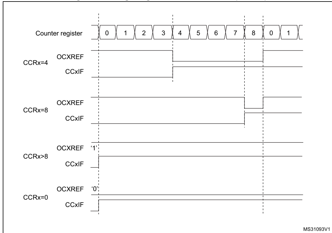
Figure 544. Edge-aligned PWM waveforms (ARR=8)
