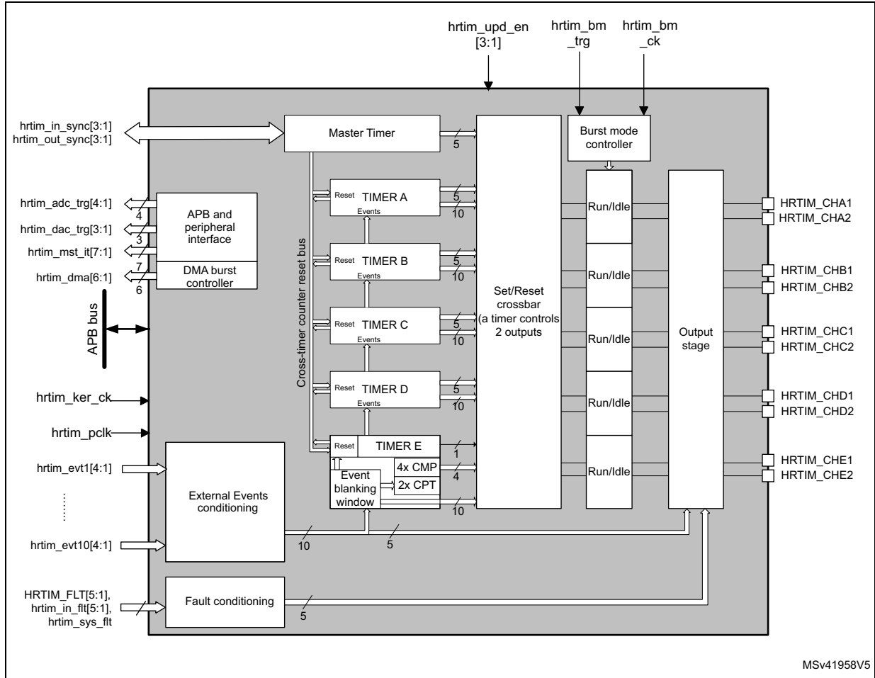
Figure 326. High-resolution timer block diagram
