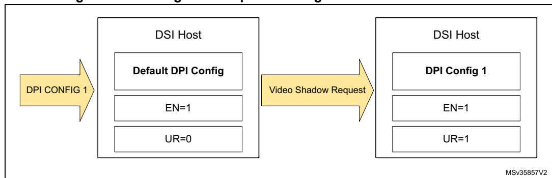
Figure 258. Configuration update during the transmission of a frame
