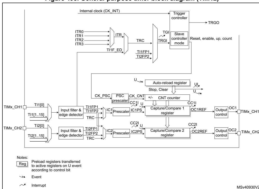
Figure 498. General-purpose timer block diagram (TIM12)
