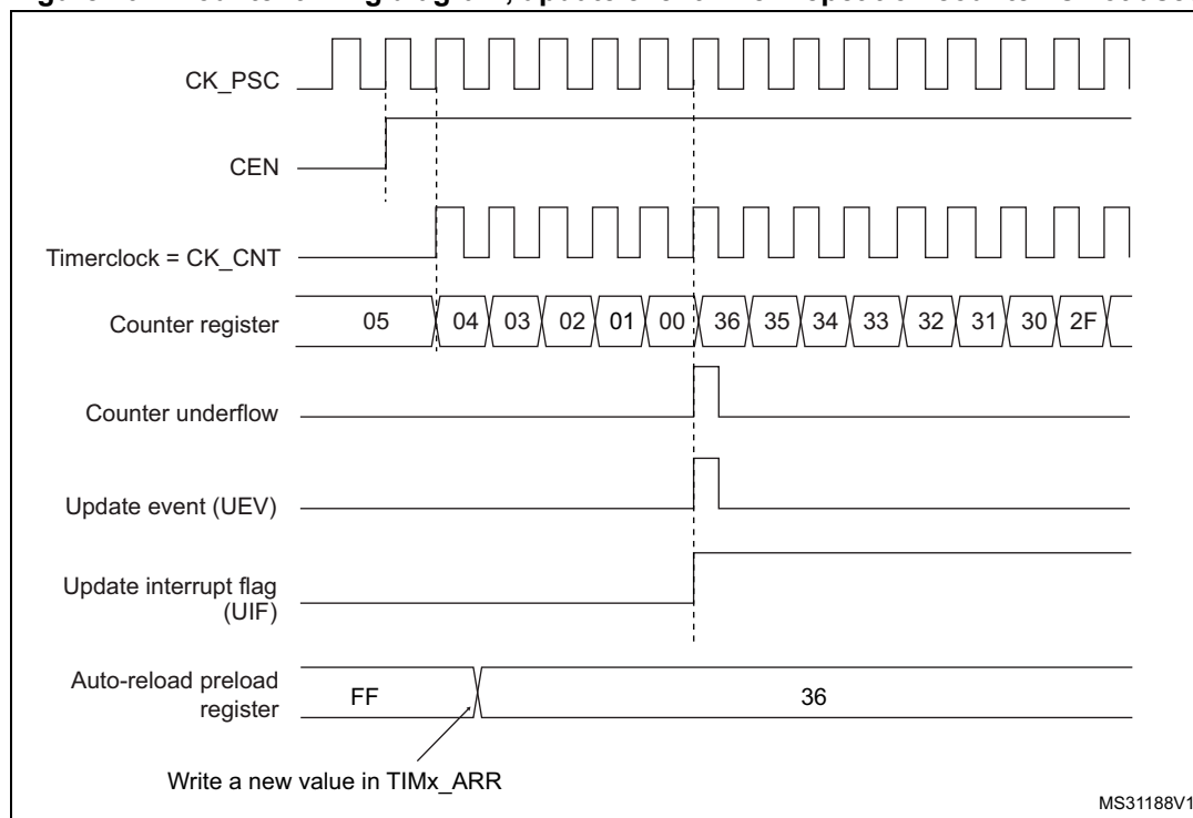
Figure 402. Counter timing diagram, update event when repetition counter is not used
