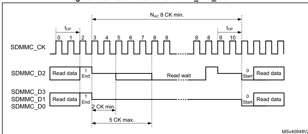
Figure 766. ReadWait with SDMMC_CK ≥ 50 MHz
