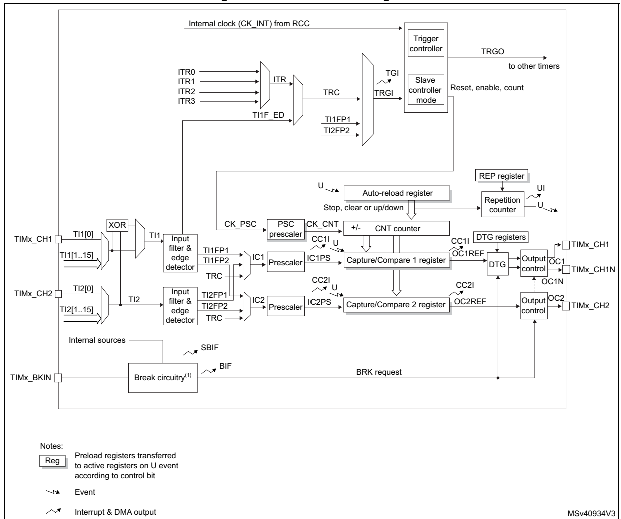
Figure 524. TIM15 block diagram
