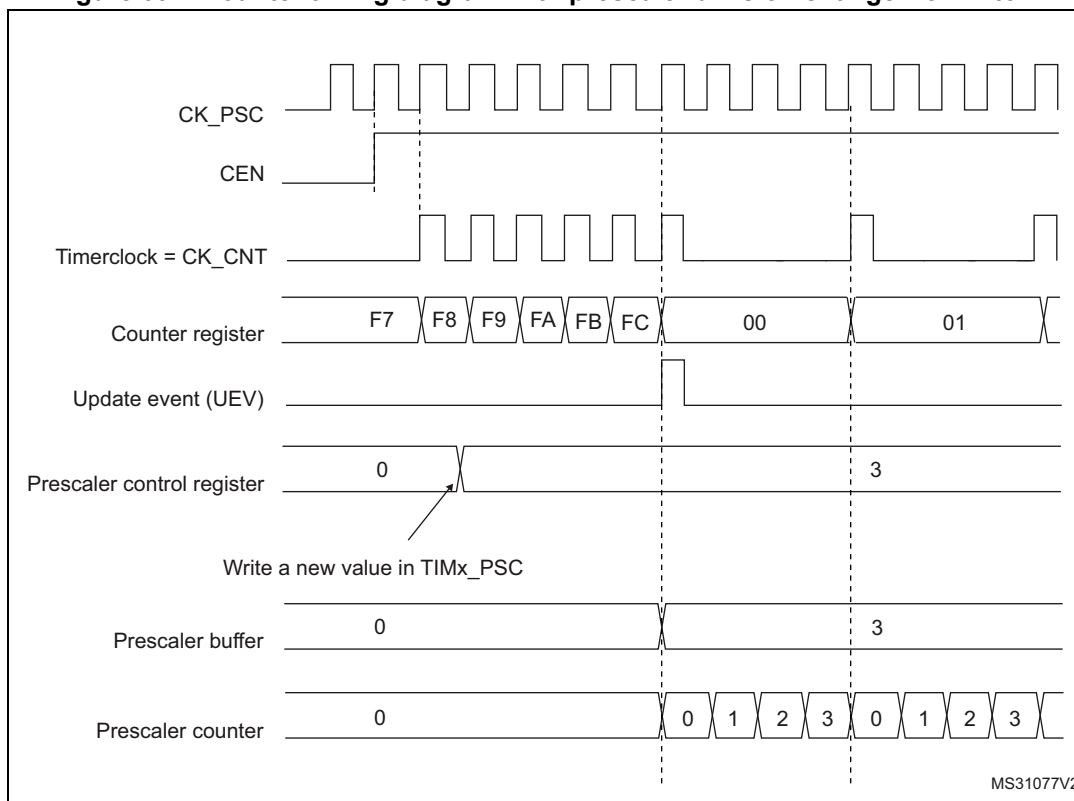
Figure 391. Counter timing diagram with prescaler division change from 1 to 4
