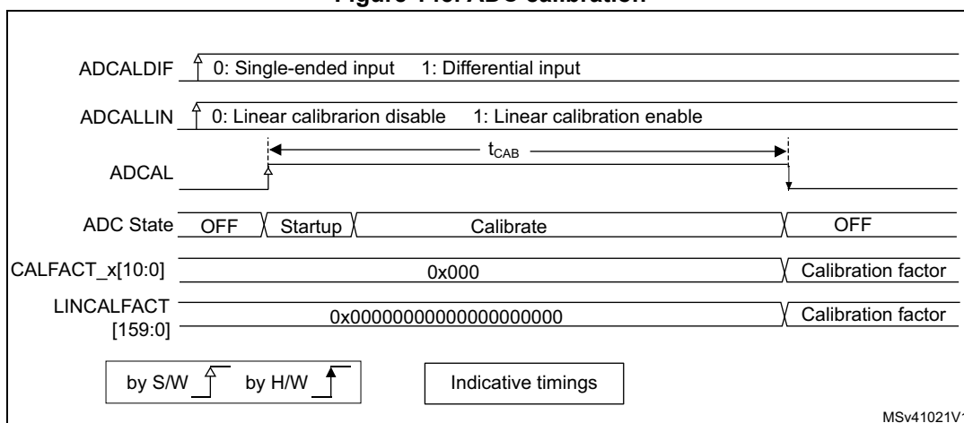
Figure 145. ADC calibration
