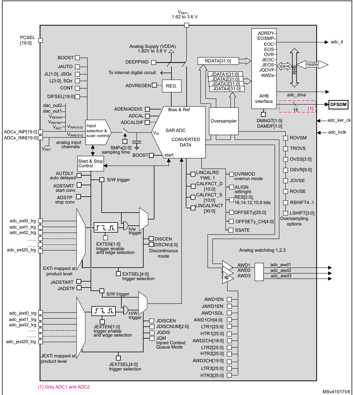
Figure 140. ADC block diagram
