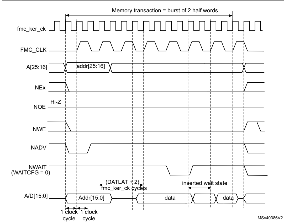
Figure 121. Synchronous multiplexed write mode waveforms - PSRAM (CRAM)
