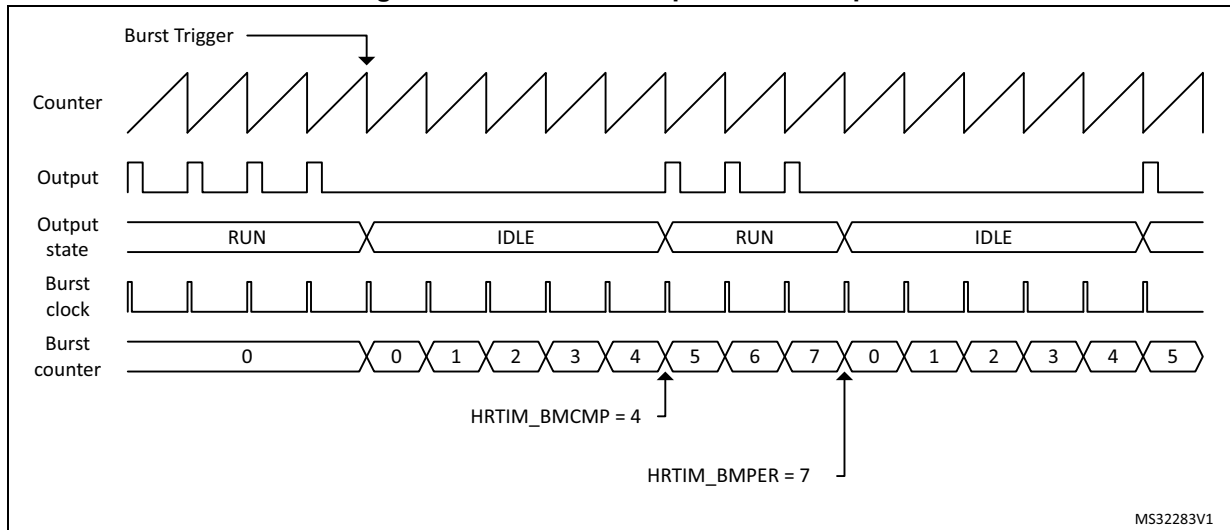
Figure 362. Burst mode operation example
