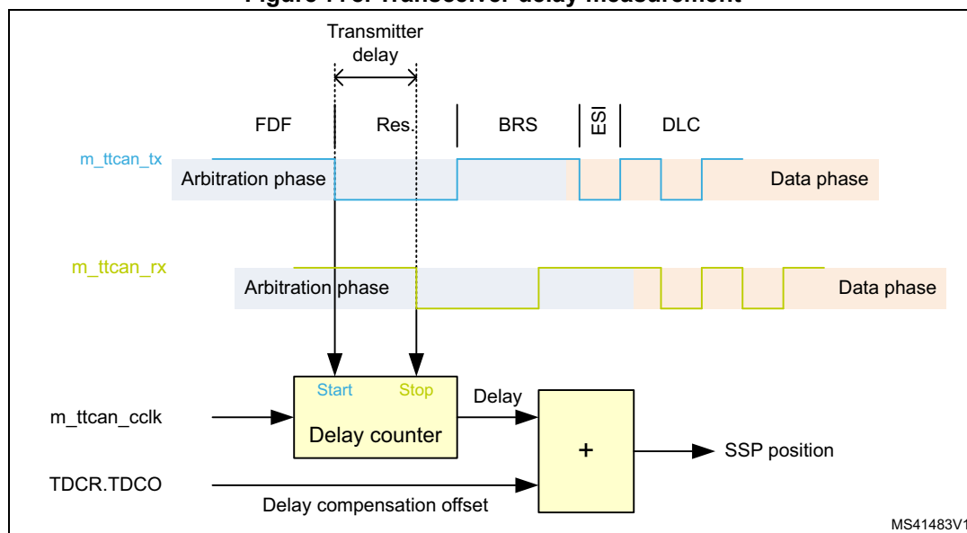
Figure 778. Transceiver delay measurement
