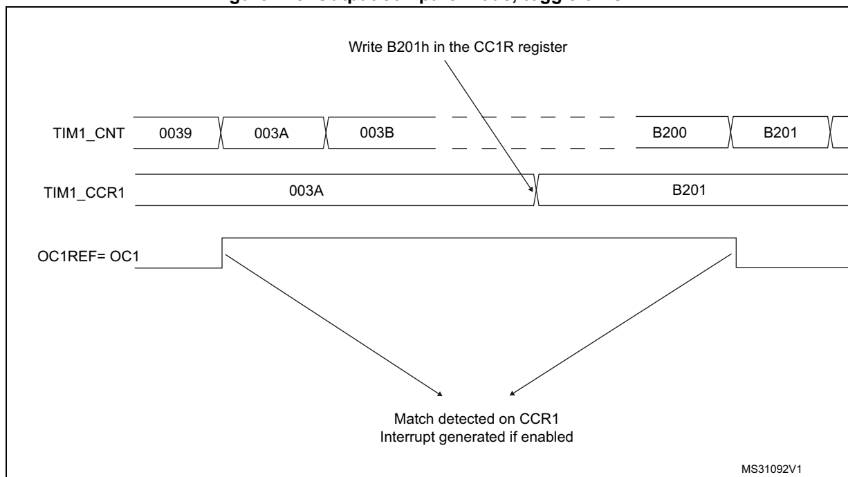
Figure 478. Output compare mode, toggle on OC1
