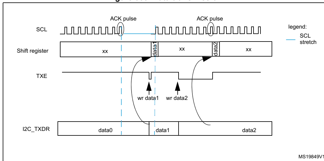
Figure 588. Data transmission
