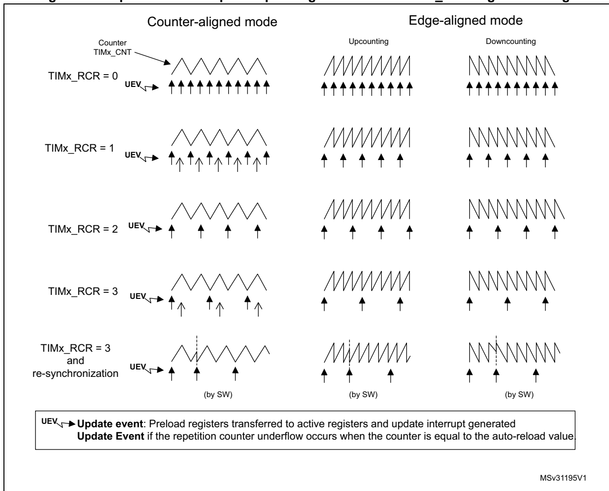
Figure 409. Update rate examples depending on mode and TIMx_RCR register settings
