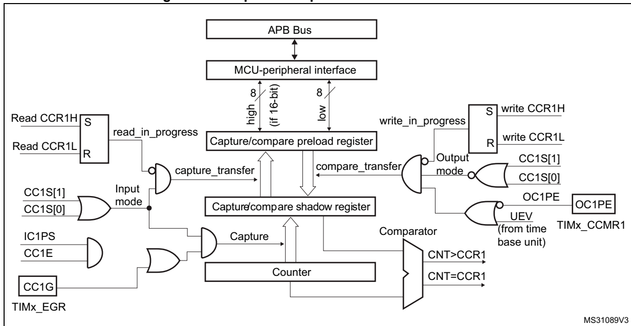
Figure 539. Capture/compare channel 1 main circuit
