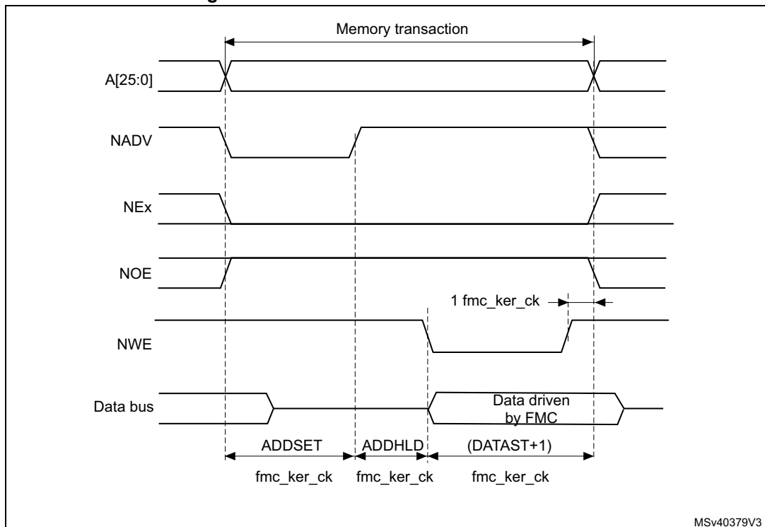
Figure 114. Mode D write access waveforms
