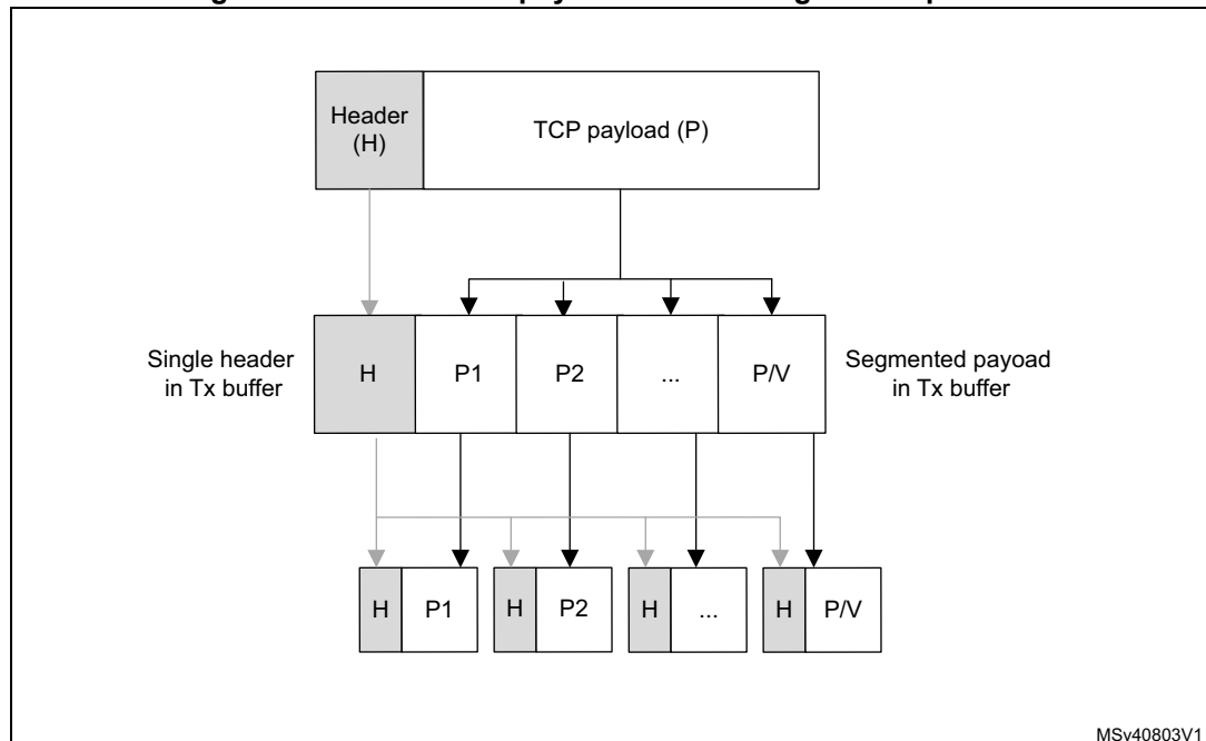
Figure 833. Header and payload fields of segmented packets
