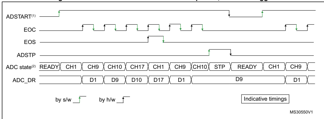
Figure 167. Continuous conversion of a sequence, software trigger
