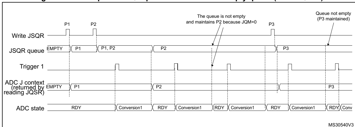
Figure 158. Example of JSQR queue of context with empty queue (case JQM=0)
