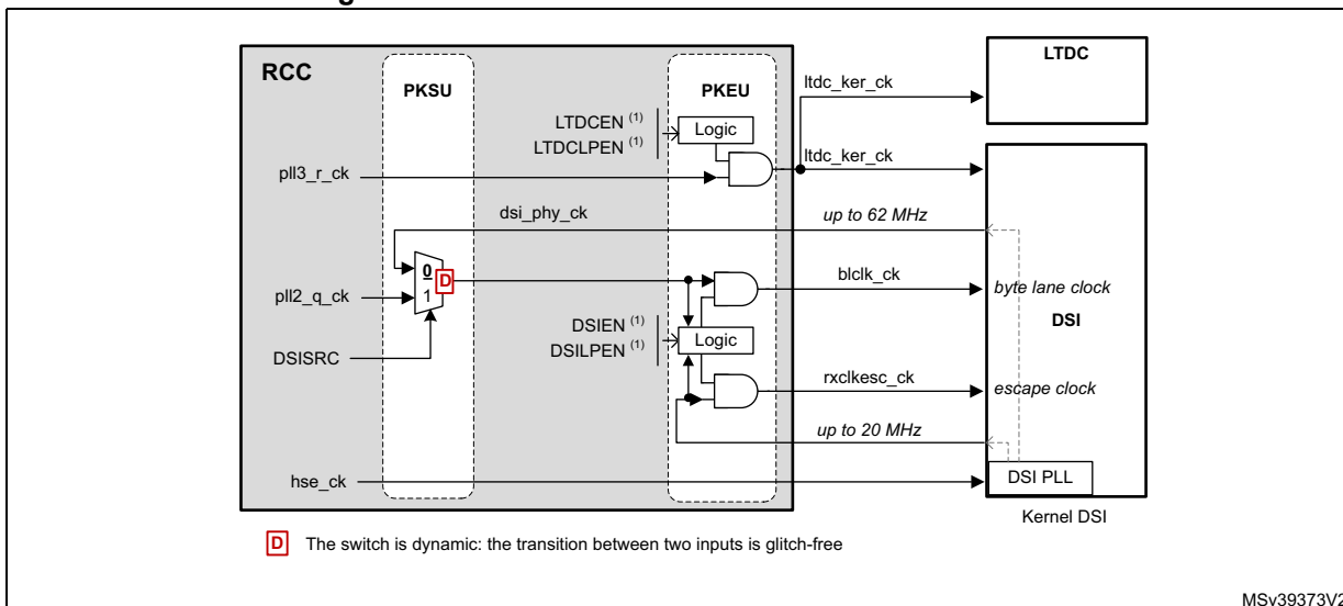
Figure 59. Kernel clock distribution for DSI and LTDC
