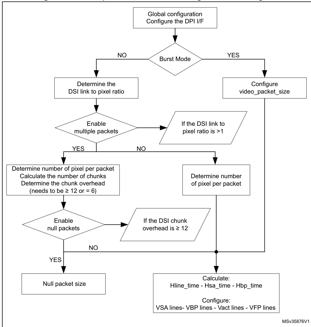
Figure 288. Video packet transmission configuration flow diagram
