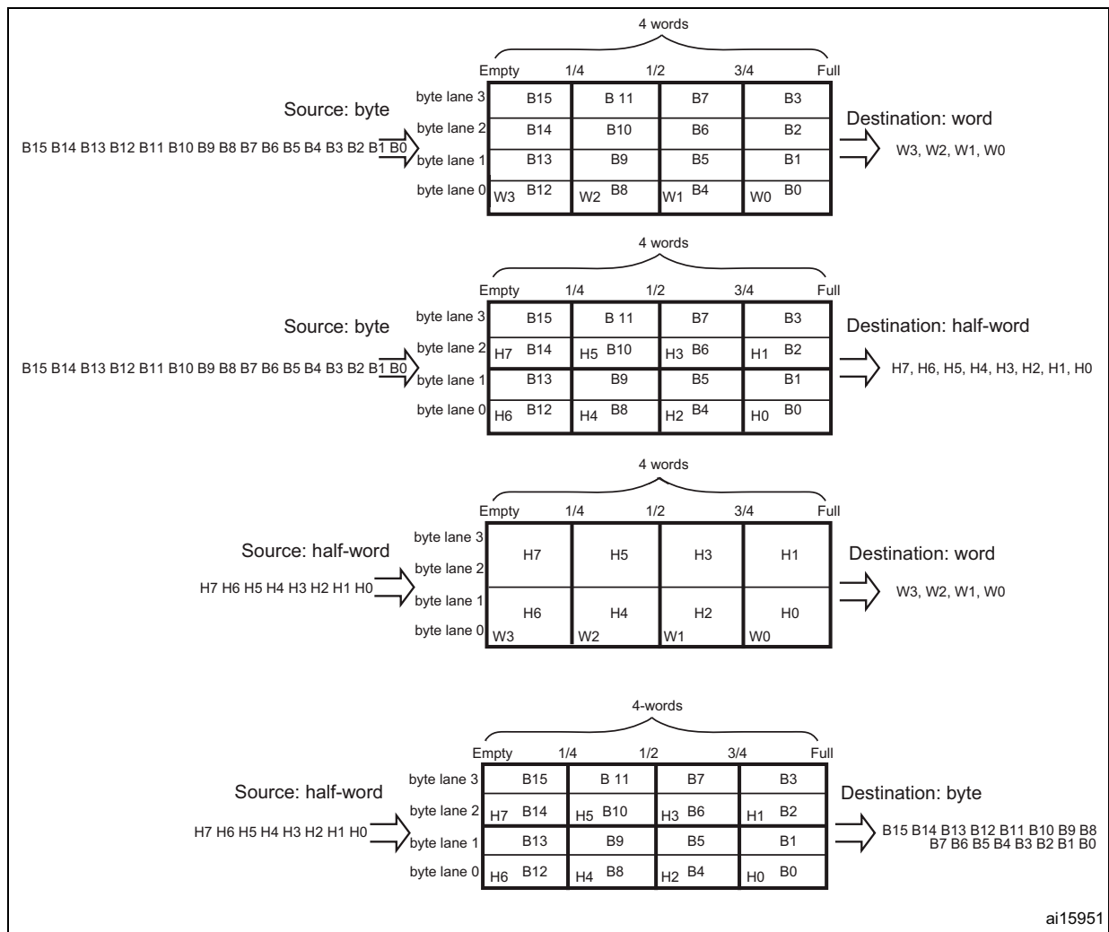
Figure 87. FIFO structure
