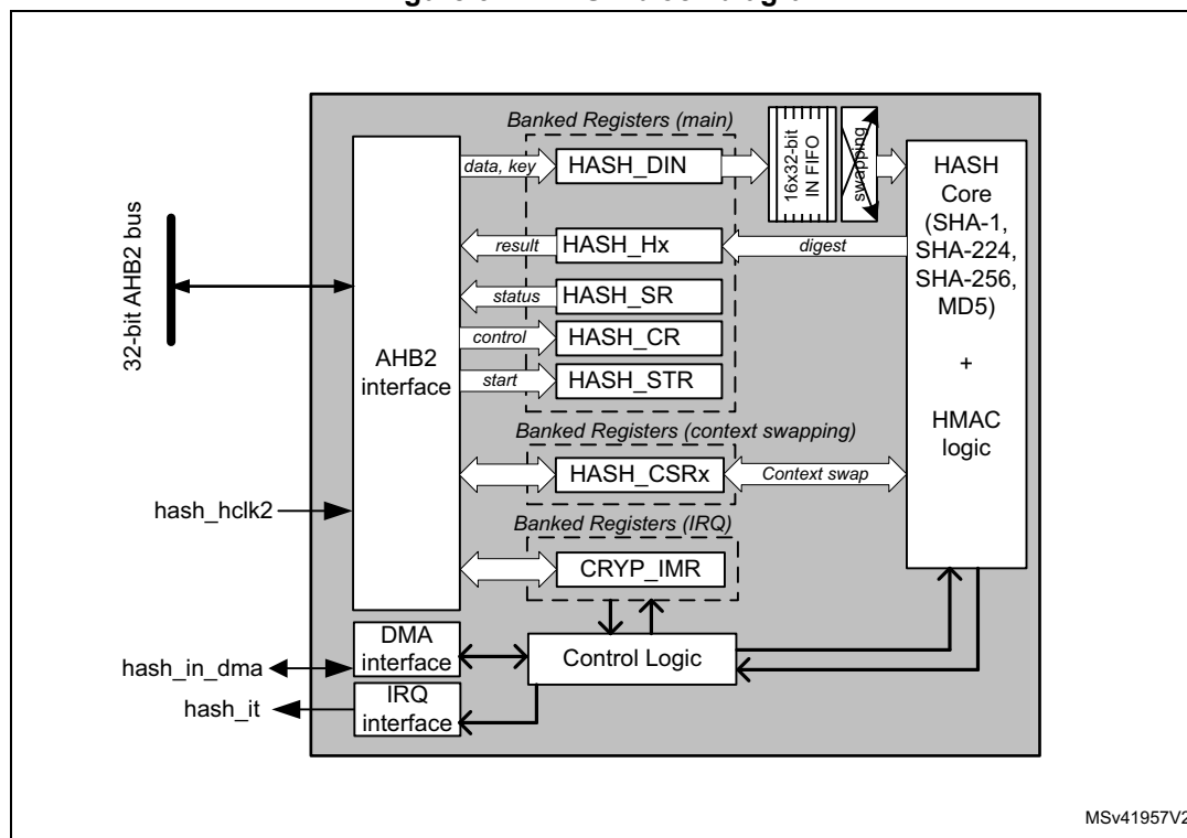
Figure 322. HASH block diagram
