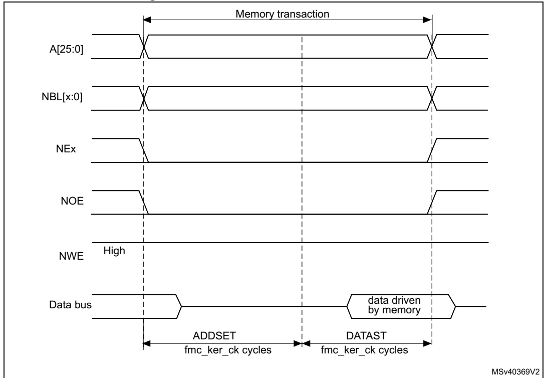
Figure 104. Mode 1 read access waveforms
