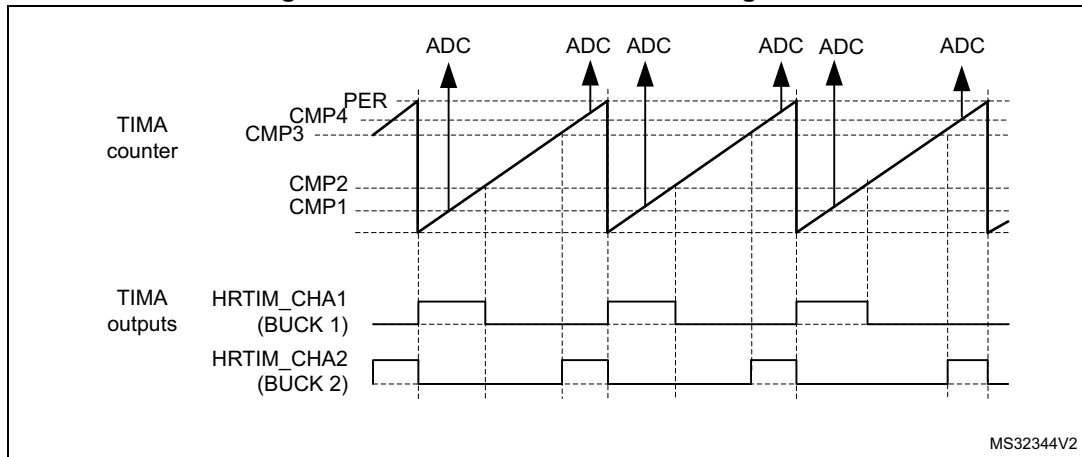
Figure 382. Dual Buck converter management
