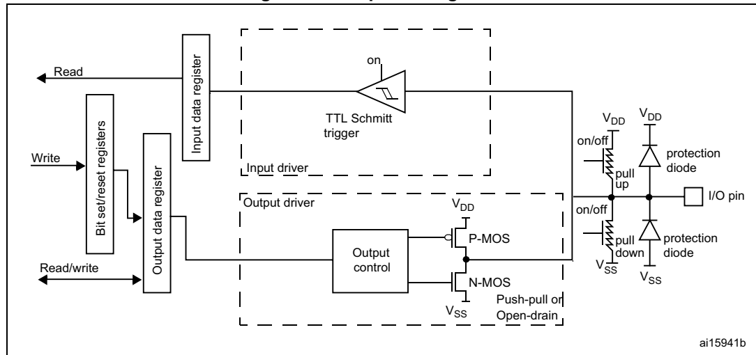
Figure 78. Output configuration
