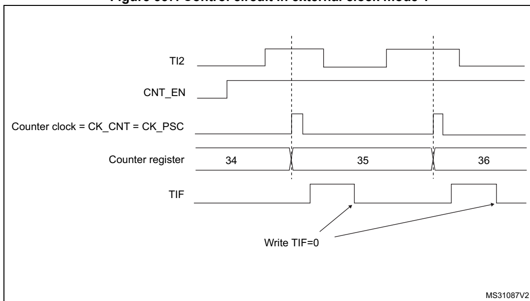
Figure 537. Control circuit in external clock mode 1
