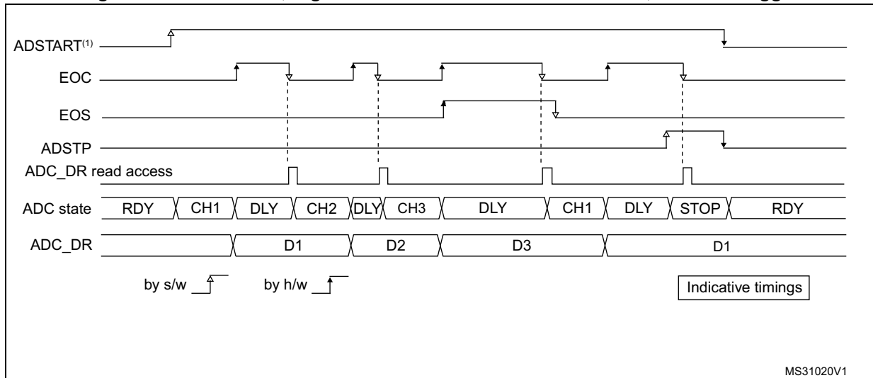
Figure 175. AUTDLY=1, regular conversion in continuous mode, software trigger
