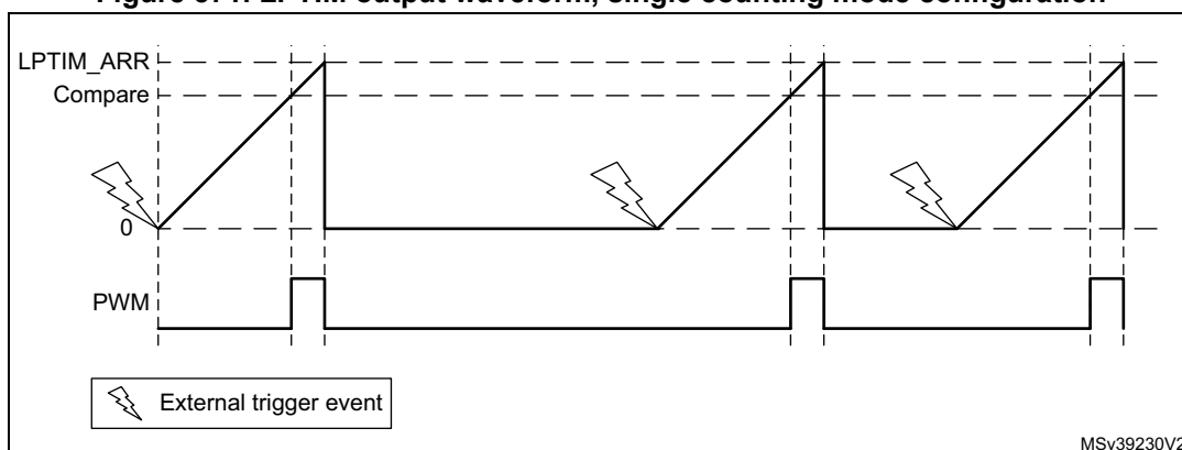
Figure 571. LPTIM output waveform, single counting mode configuration
