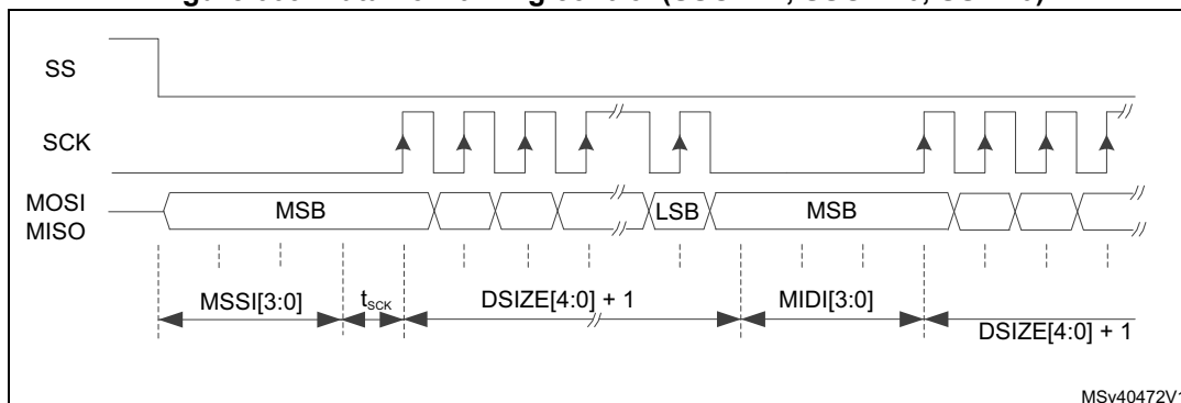
Figure 663. Data flow timing control (SSOE=1, SSOM=0, SSM=0)
