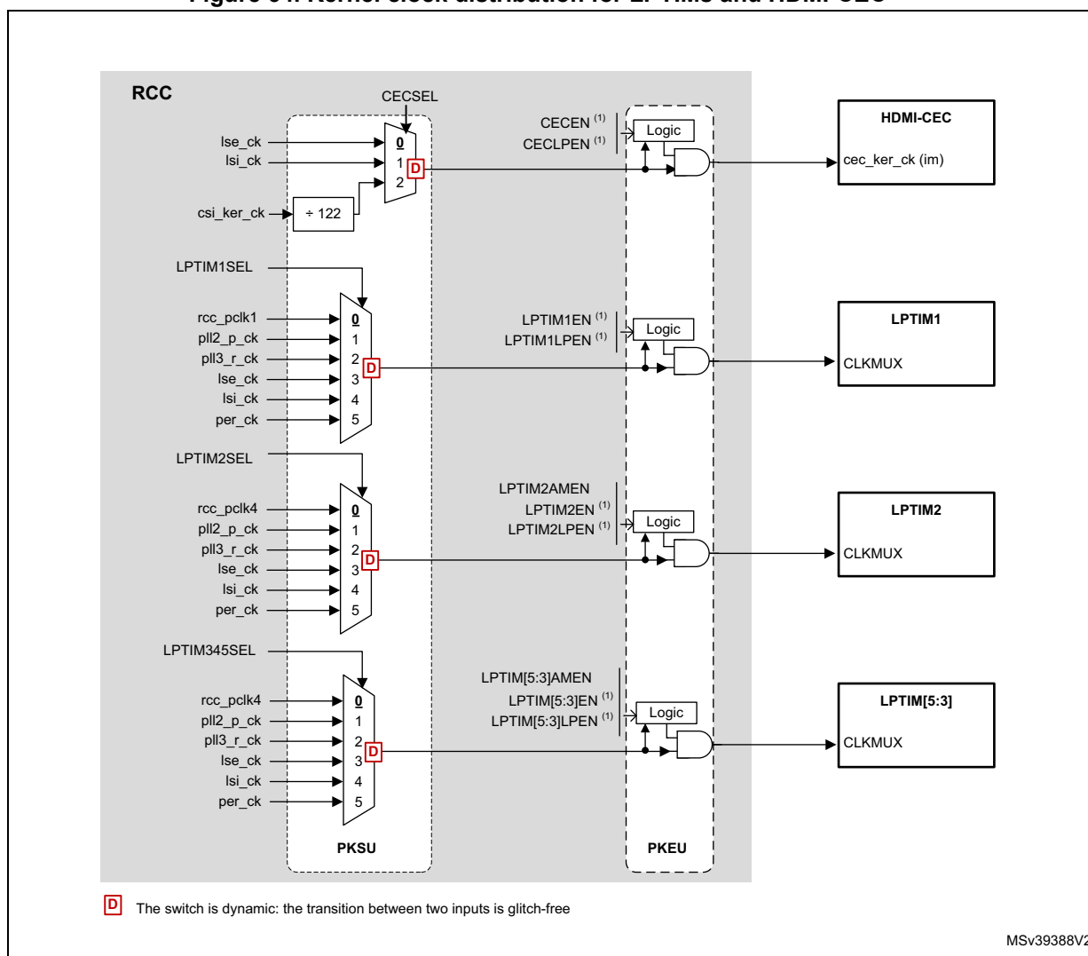
Figure 64. Kernel clock distribution for LPTIMs and HDMI-CEC (2)
