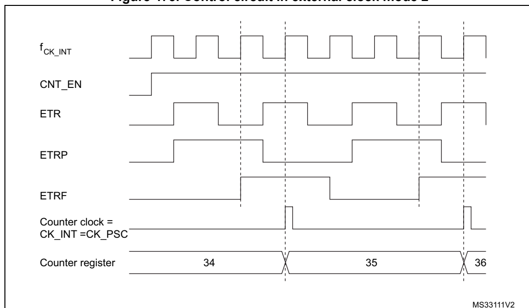
Figure 473. Control circuit in external clock mode 2
