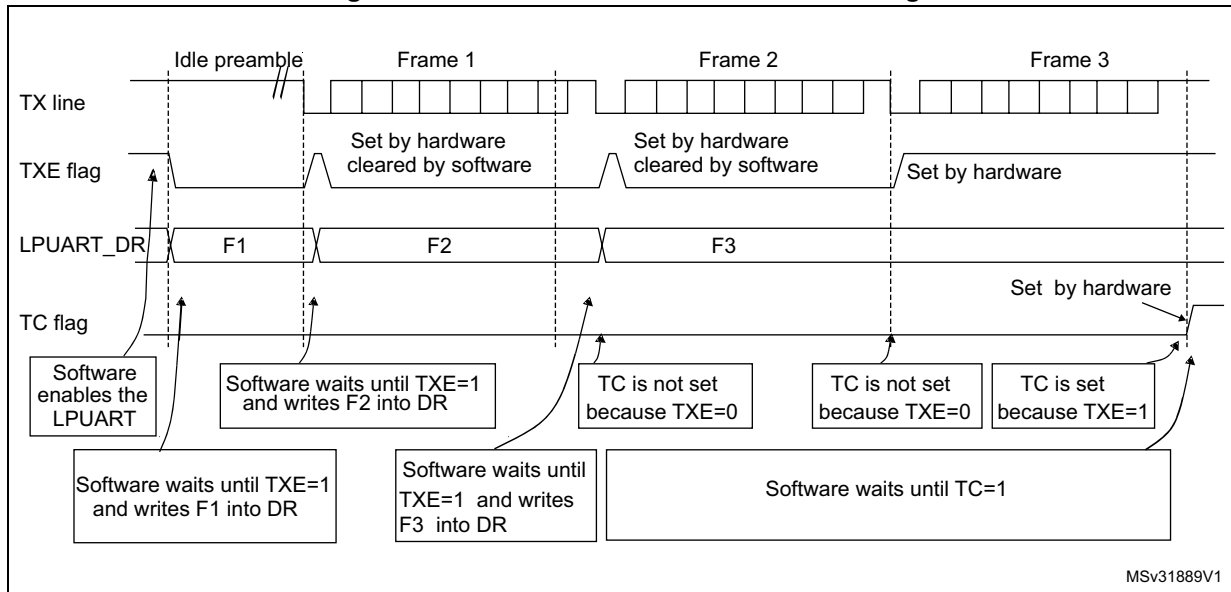
Figure 644. TC/TXE behavior when transmitting
