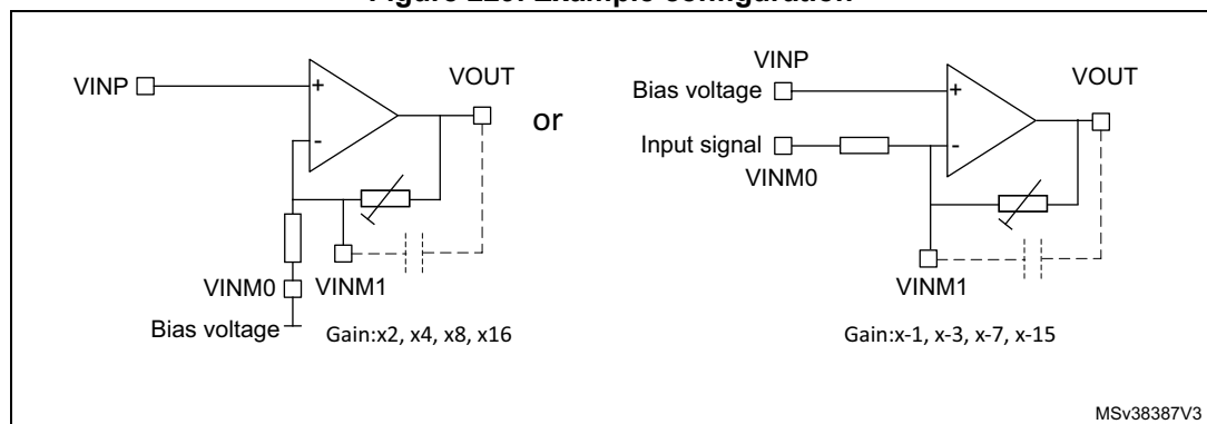
Figure 229. Example configuration
