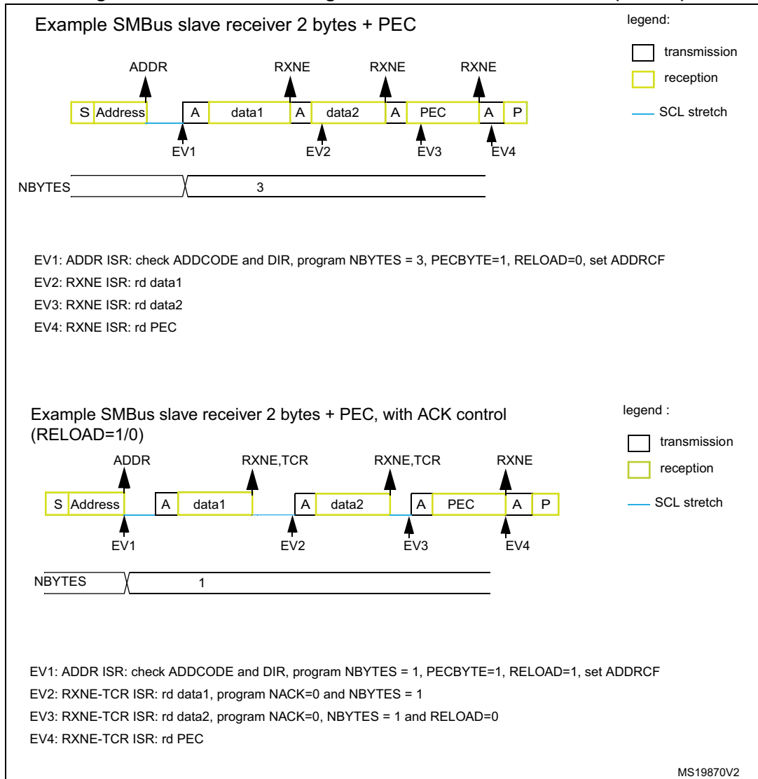
Figure 610. Bus transfer diagrams for SMBus slave receiver (SBC=1)
