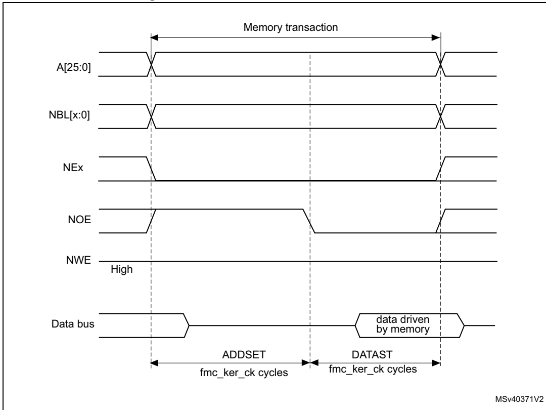
Figure 106. Mode A read access waveforms
