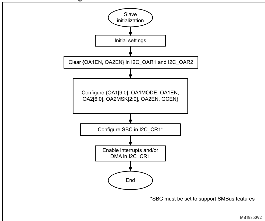
Figure 589. Slave initialization flowchart
