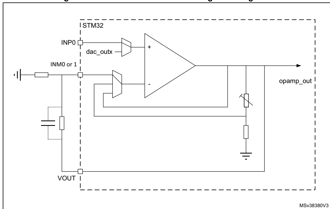
Figure 224. Standalone mode: external gain setting mode
