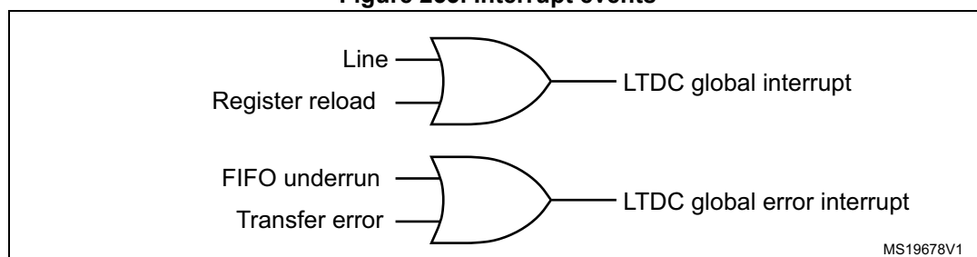
Figure 253. Interrupt events
