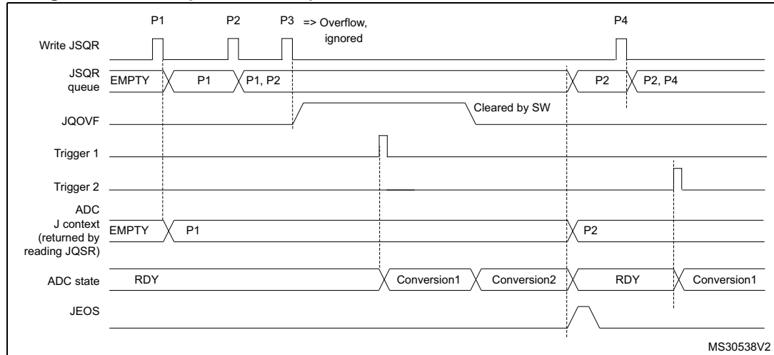
Figure 156. Example of JSQR queue of context with overflow before conversion
