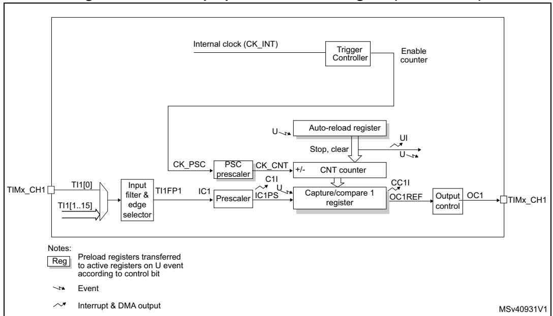
Figure 499. General-purpose timer block diagram (TIM13/TIM14)
