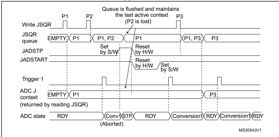
Figure 161. Flushing JSQR queue of context by setting JADSTP=1 (JQM=0). Case when JADSTP occurs during an ongoing conversion and a new trigger occurs.
