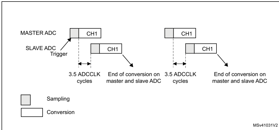
Figure 195. Interleaved mode on 1 channel in single conversion mode: dual ADC mode
