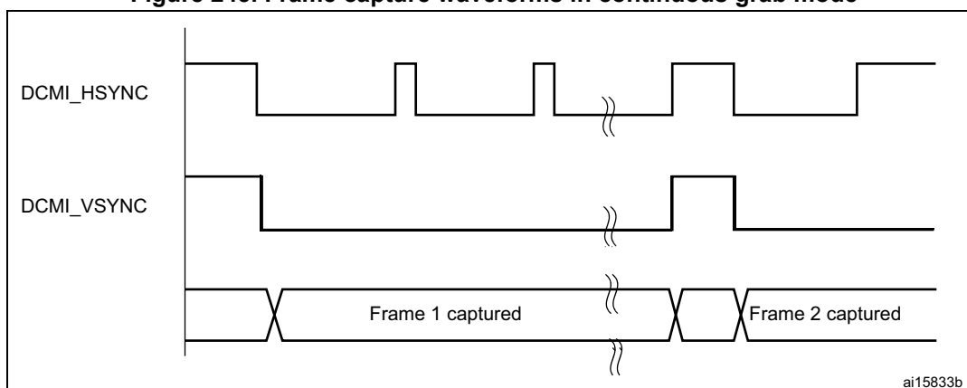
Figure 245. Frame capture waveforms in continuous grab mode
