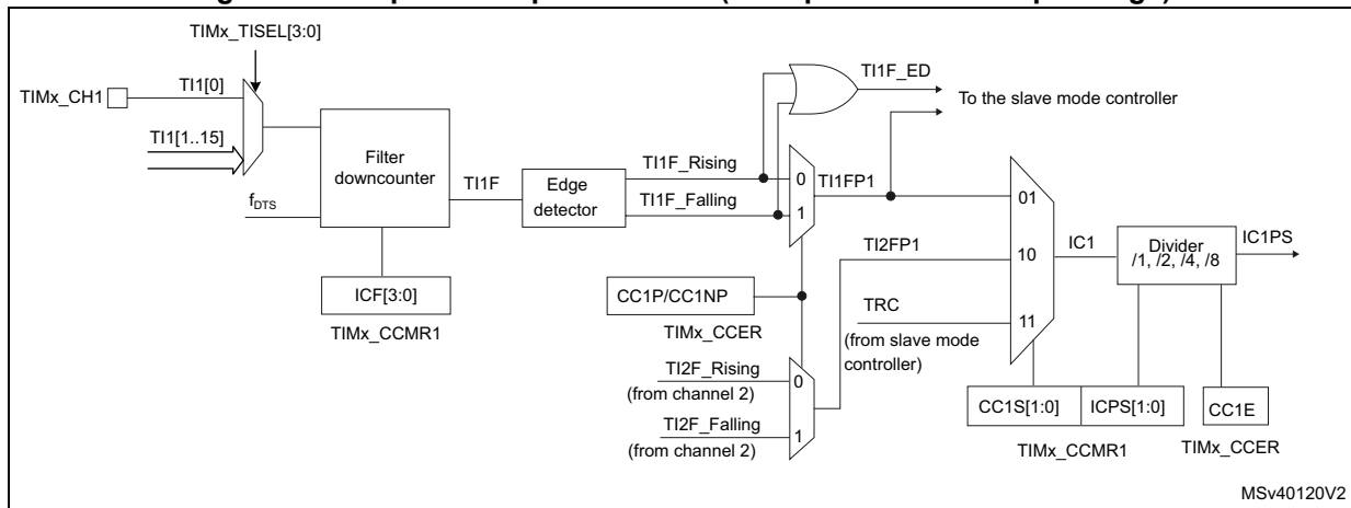
Figure 417. Capture/compare channel (example: channel 1 input stage)
