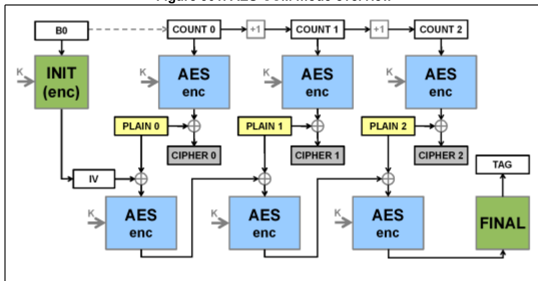
Figure 301. AES-CCM mode overview
