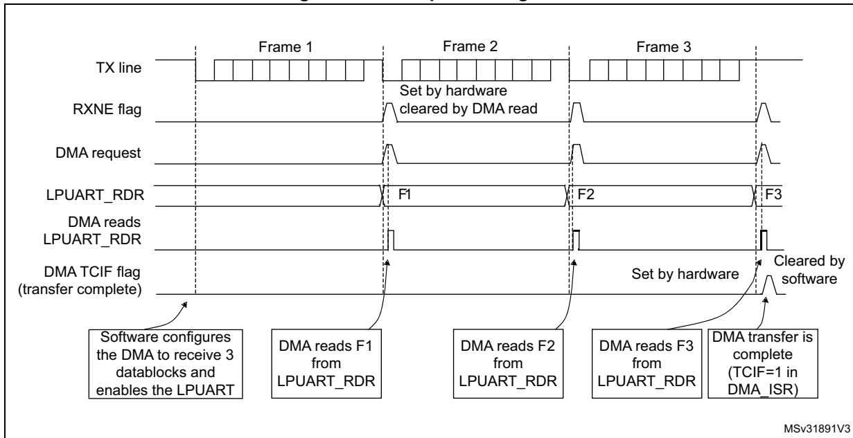
Figure 649. Reception using DMA
