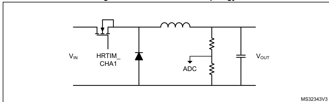
Figure 381. Buck converter topology
