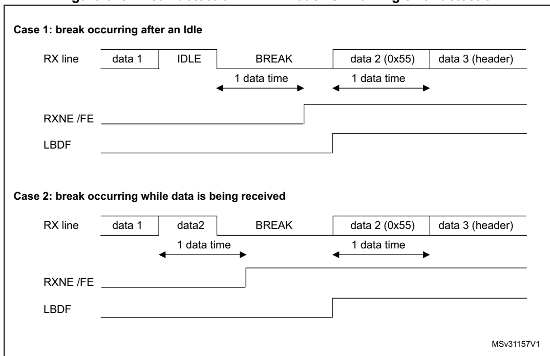
Figure 625. Break detection in LIN mode vs. Framing error detection
