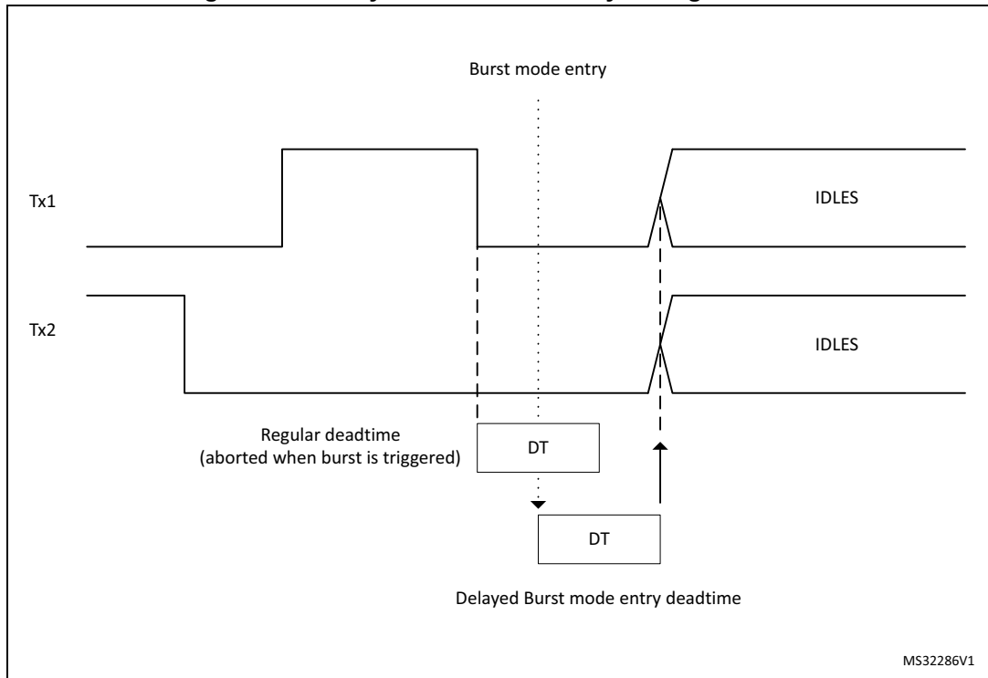
Figure 365. Delayed Burst mode entry during deadtime
