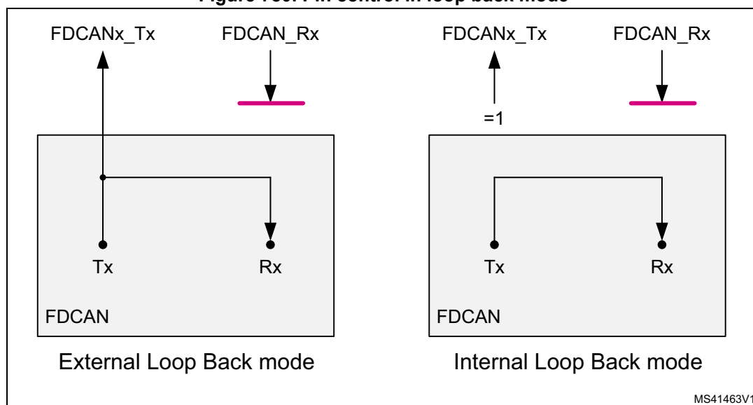
Figure 780. Pin control in loop back mode
