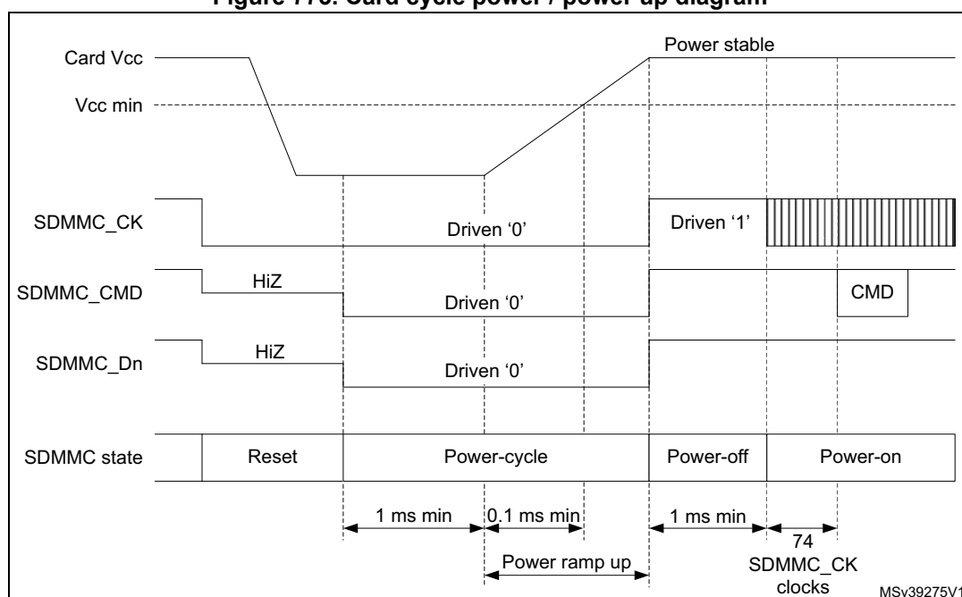
Figure 773. Card cycle power / power up diagram
