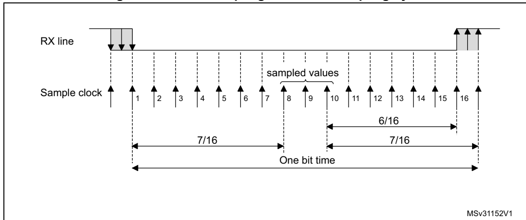
Figure 621. Data sampling when oversampling by 8
