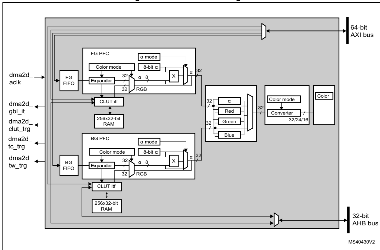
Figure 92. DMA2D block diagram
