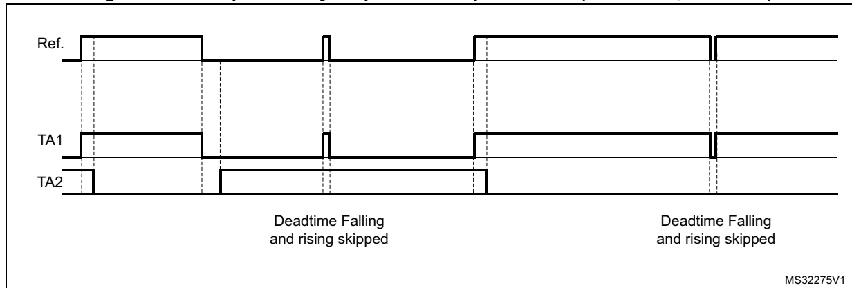
Figure 344. Complementary outputs for low pulse width (SDTRx = 1, SDTFx=0)
