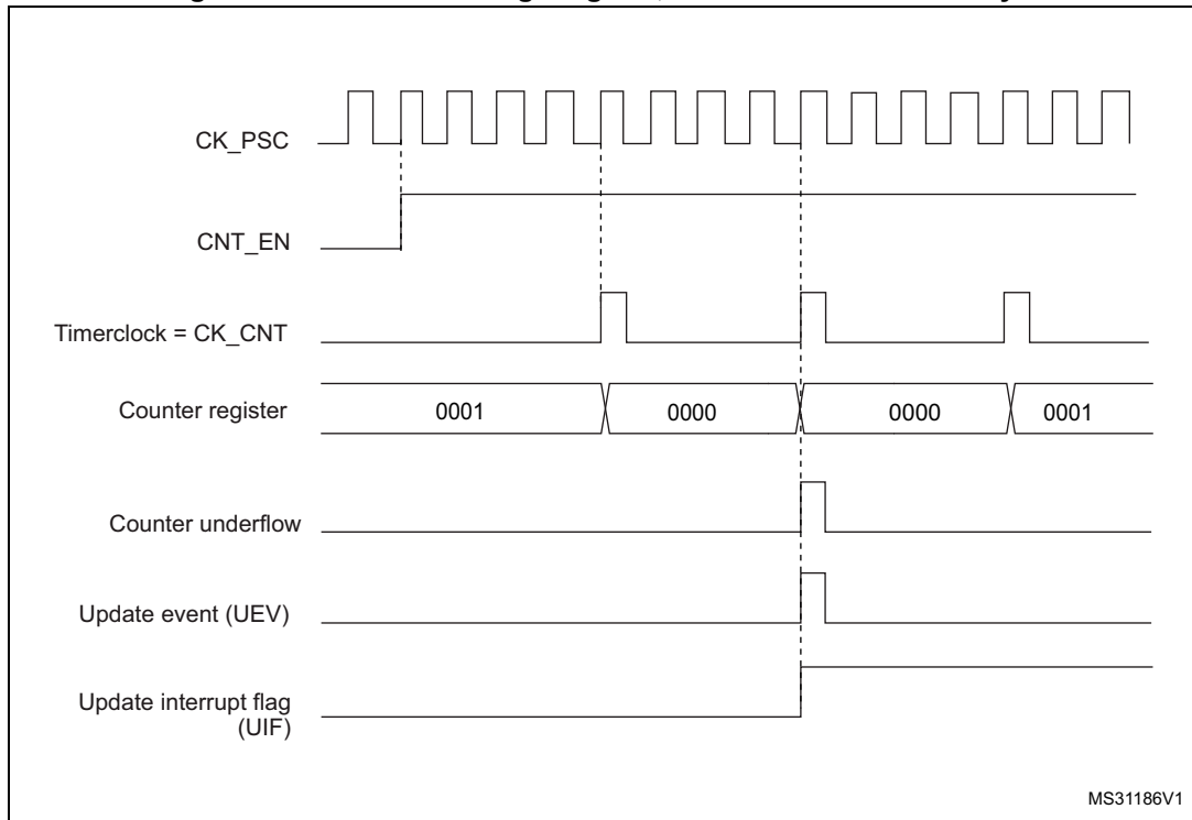
Figure 461. Counter timing diagram, internal clock divided by N
