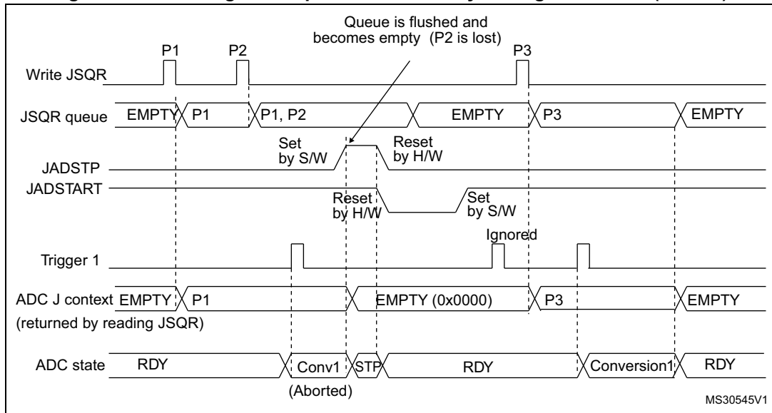
Figure 163. Flushing JSQR queue of context by setting JADSTP=1 (JQM=1)
