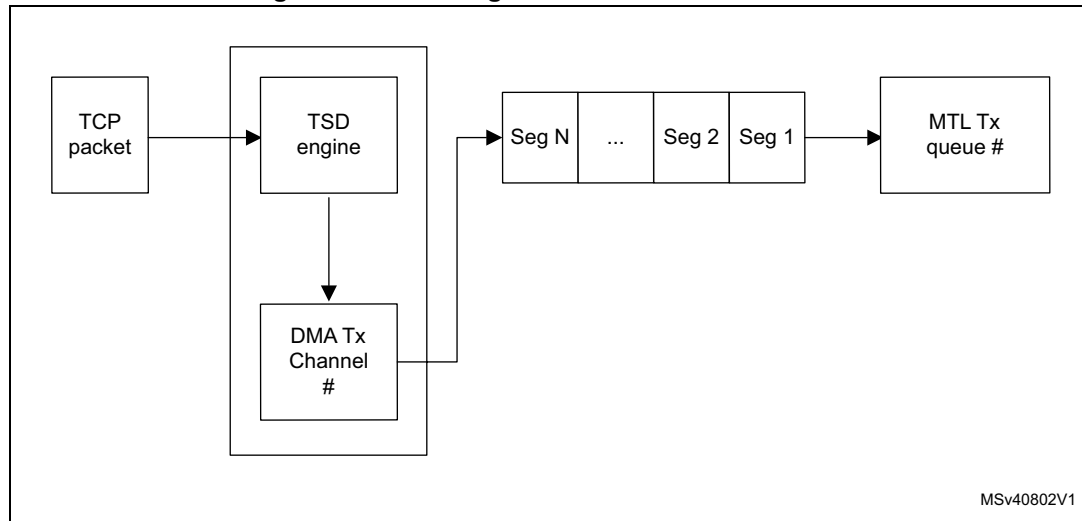
Figure 832. TCP segmentation offload overview
