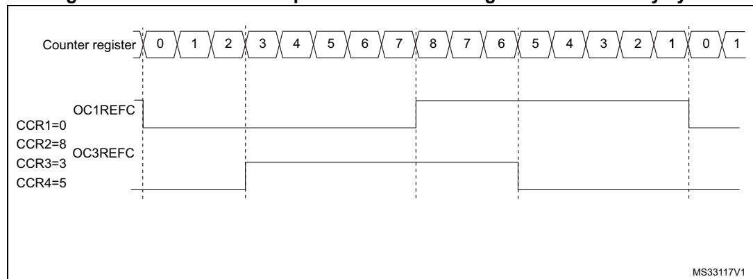
Figure 481. Generation of 2 phase-shifted PWM signals with 50% duty cycle
