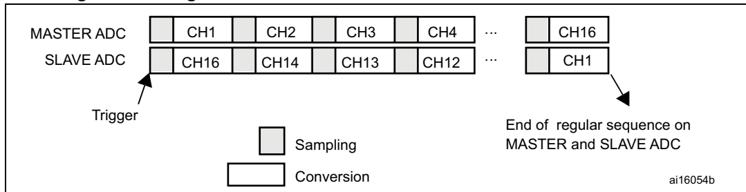
Figure 193. Regular simultaneous mode on 16 channels: dual ADC mode
