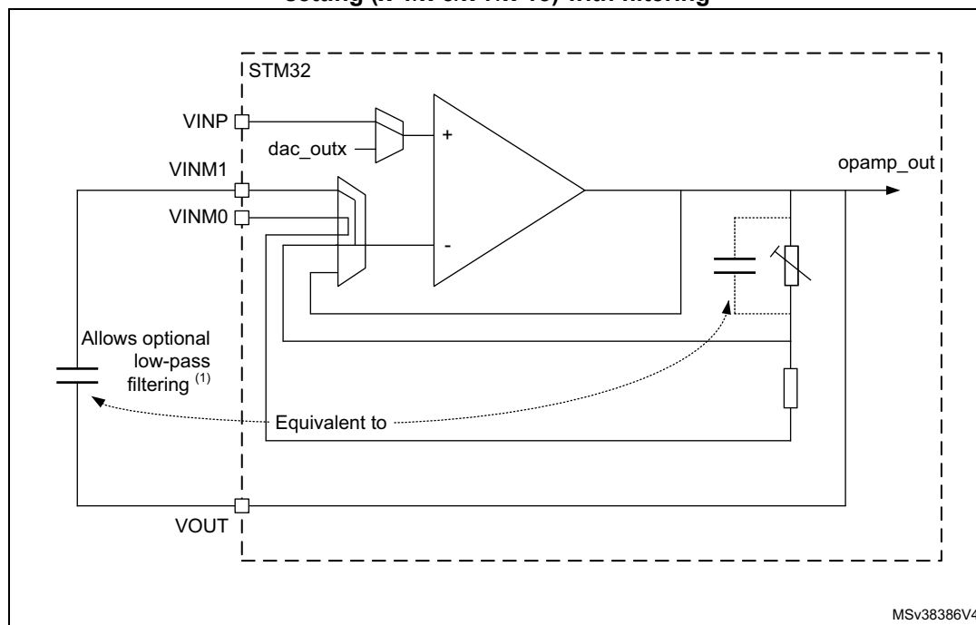
Figure 230. PGA mode, non-inverting gain setting (x2/x4/x8/x16) or inverting gain setting (x-1/x-3/x-7/x-15) with filtering
