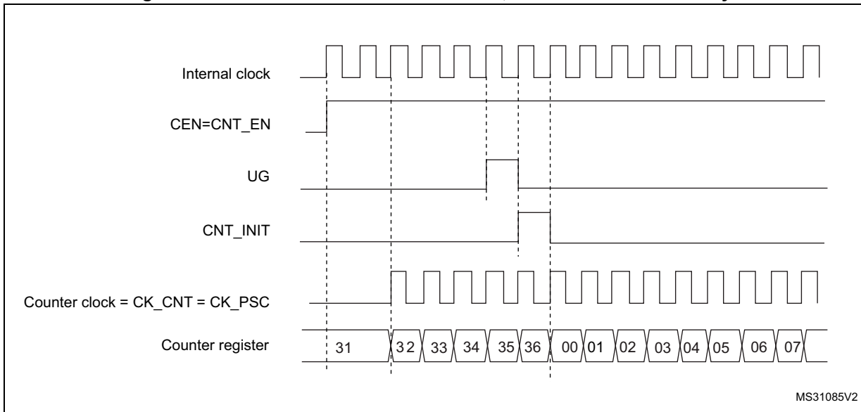
Figure 469. Control circuit in normal mode, internal clock divided by 1
