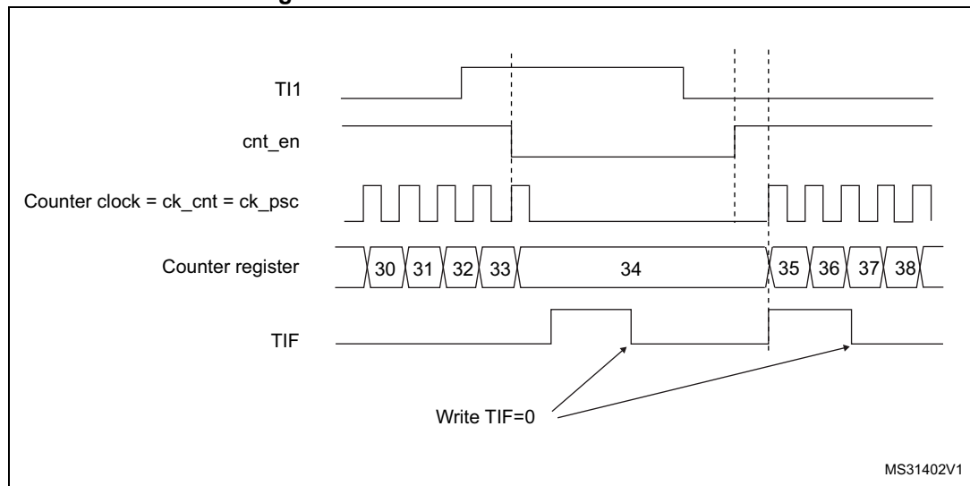
Figure 446. Control circuit in Gated mode
