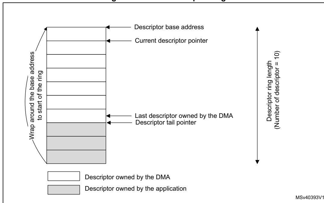
Figure 844. DMA descriptor ring
