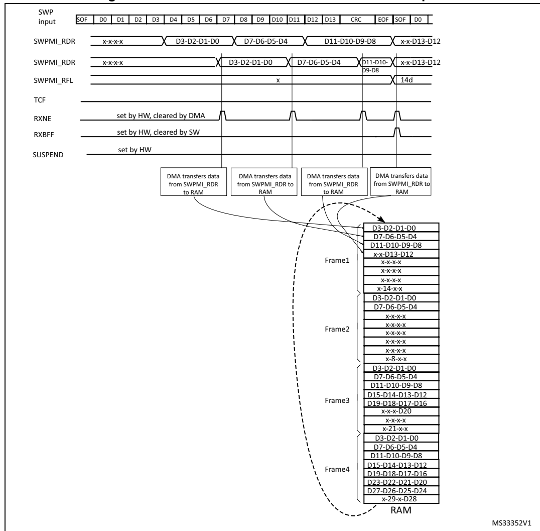
Figure 737. SWPMI Multi software buffer mode reception
