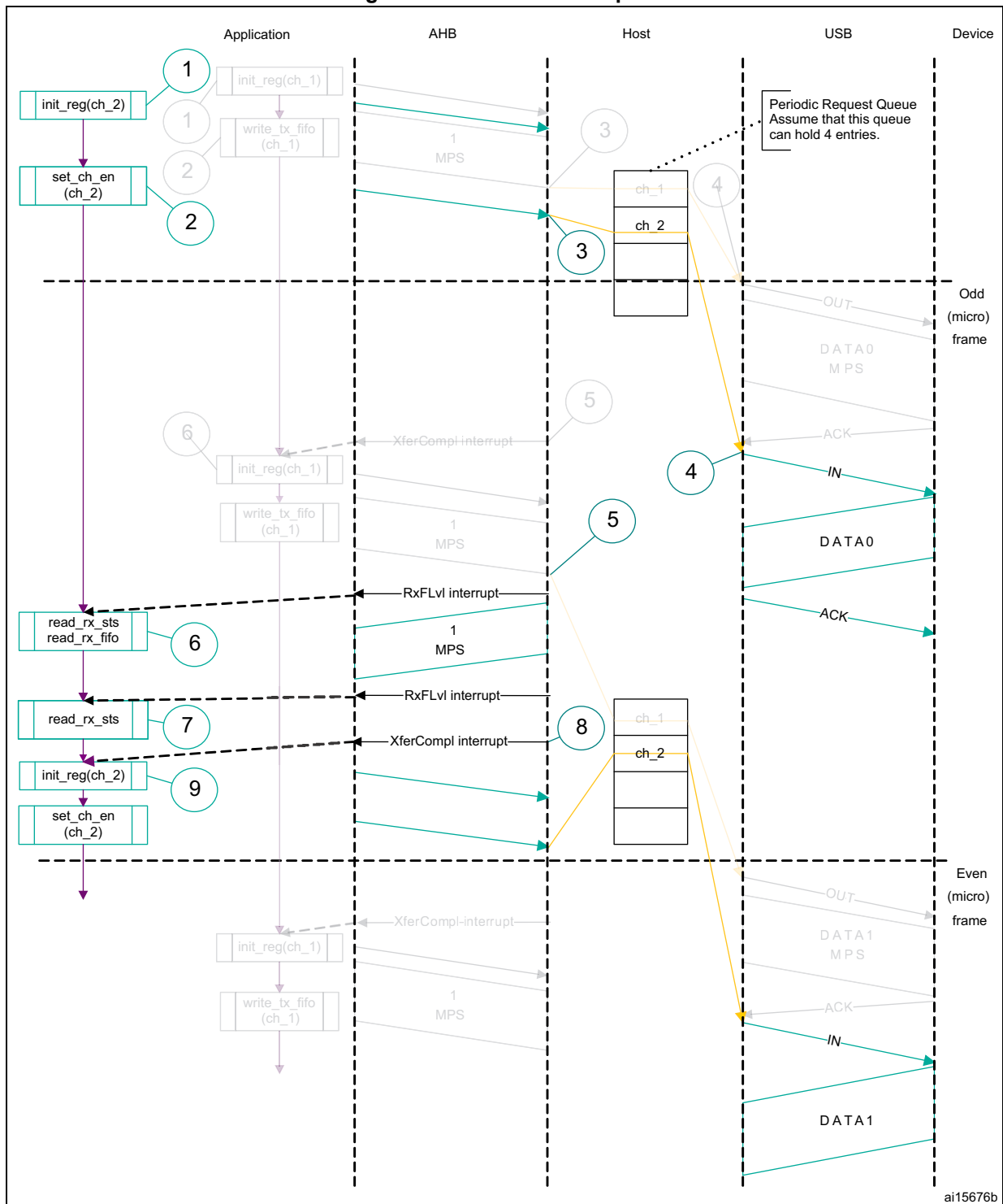
Figure 805. Normal interrupt IN
