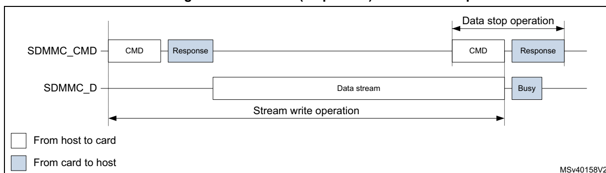
Figure 746. SDMMC (sequential) stream write operation
