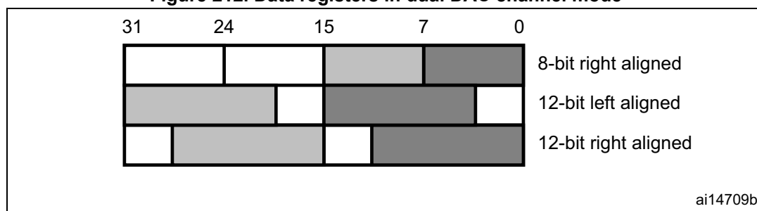
Figure 212. Data registers in dual DAC channel mode
