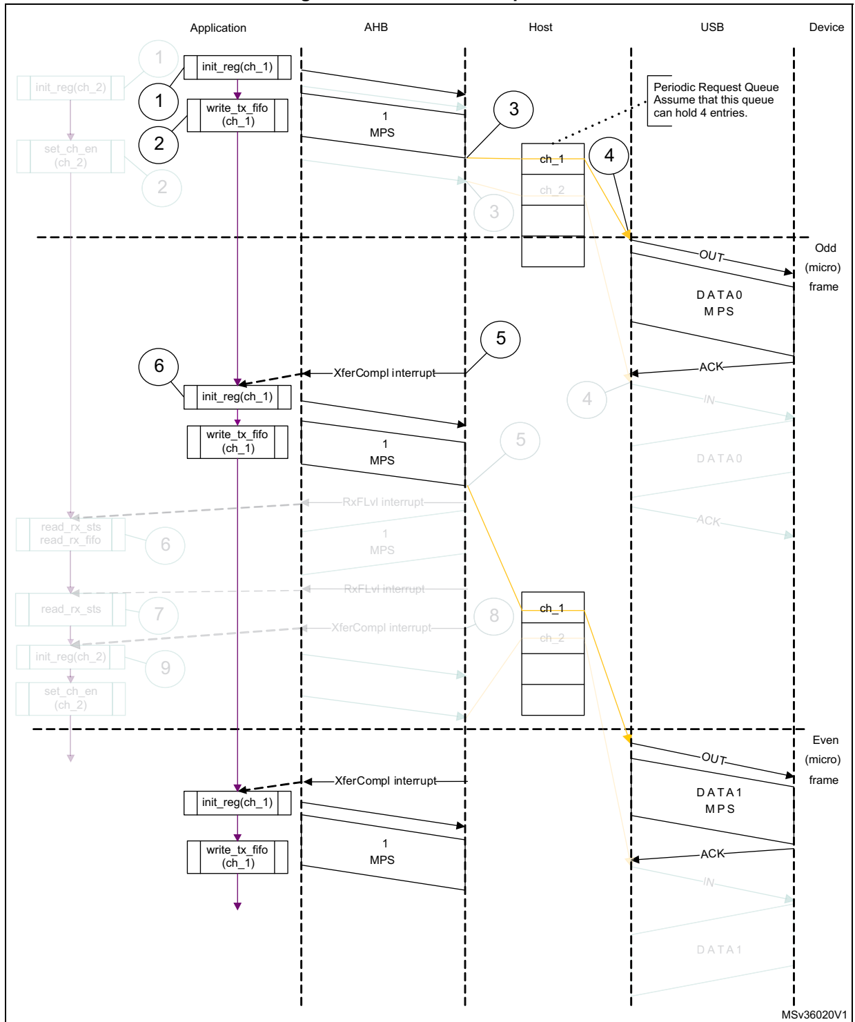
Figure 804. Normal interrupt OUT
