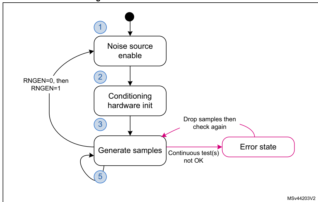
Figure 294. RNG initialization overview
