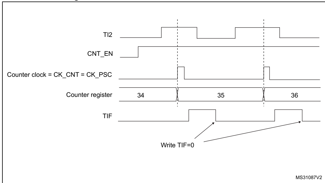
Figure 414. Control circuit in external clock mode 1
