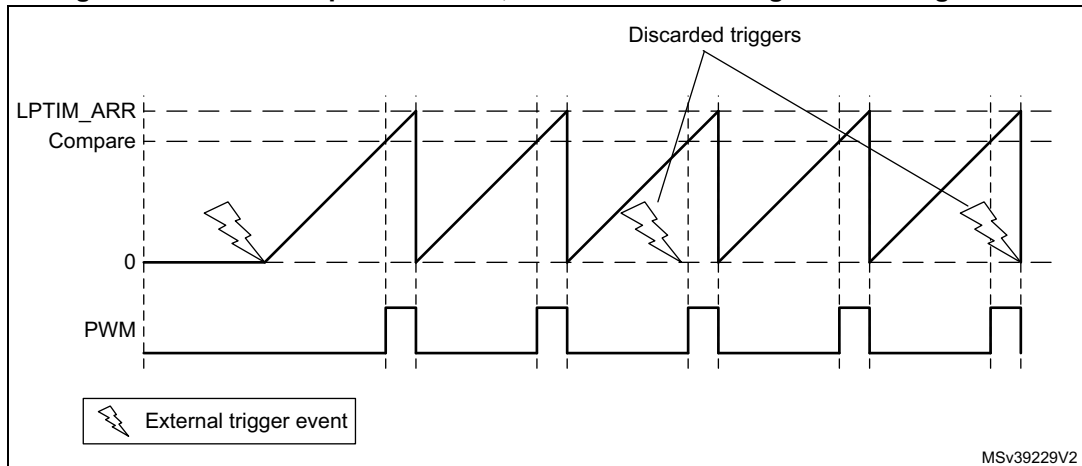
Figure 573. LPTIM output waveform, Continuous counting mode configuration
