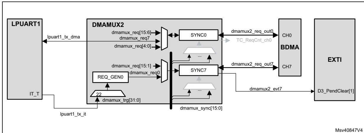
Figure 45. BDMA and DMAMUX2 interconnection
