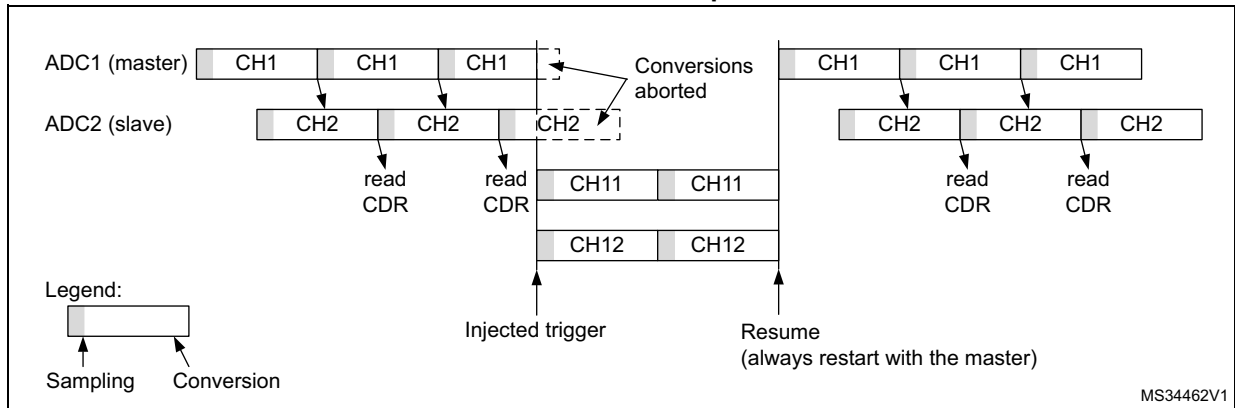
Figure 203. Two Interleaved channels (CH1, CH2) with injected sequence CH11, CH12 - case 2: Slave interrupted first
