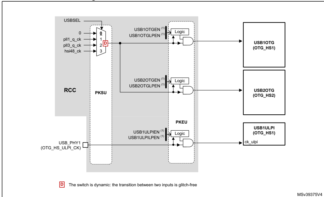
Figure 61. Kernel clock distribution For USB (2)
