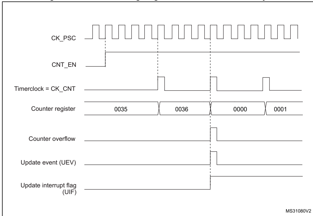
Figure 395. Counter timing diagram, internal clock divided by N
