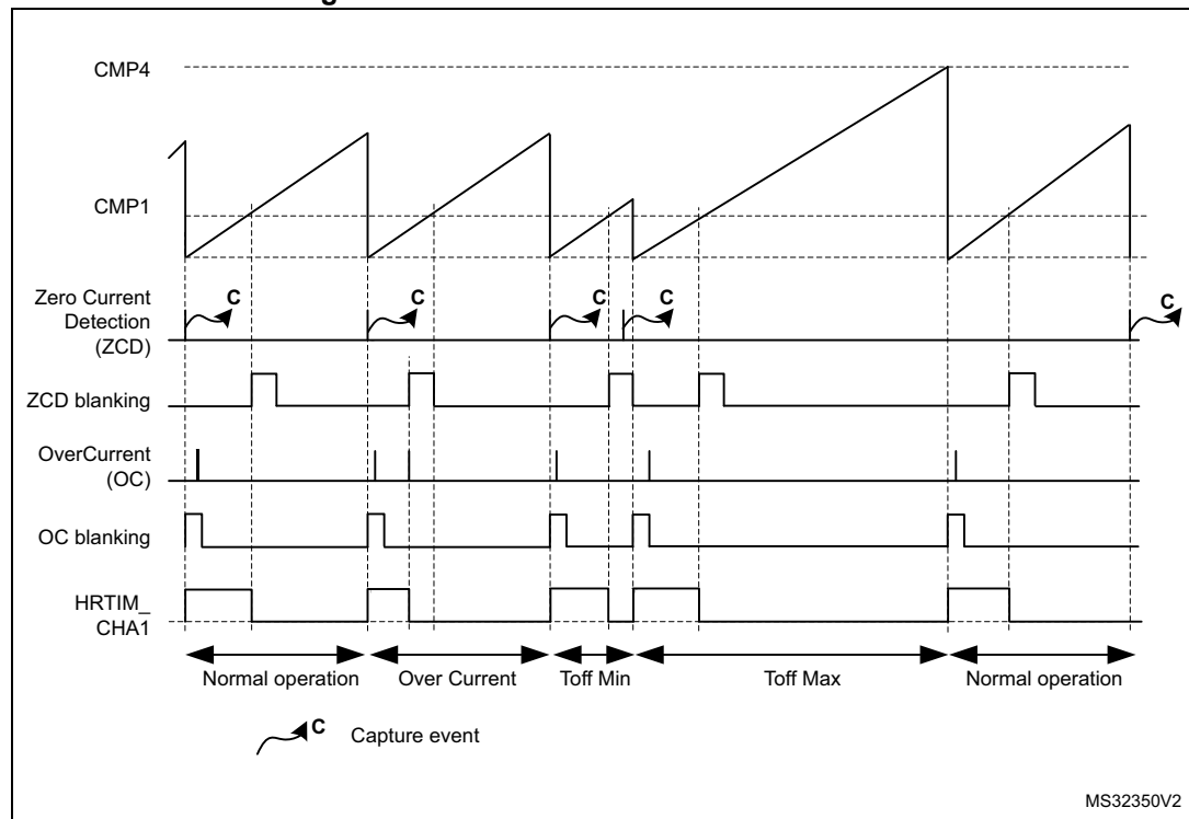
Figure 388. Transition mode PFC waveforms
