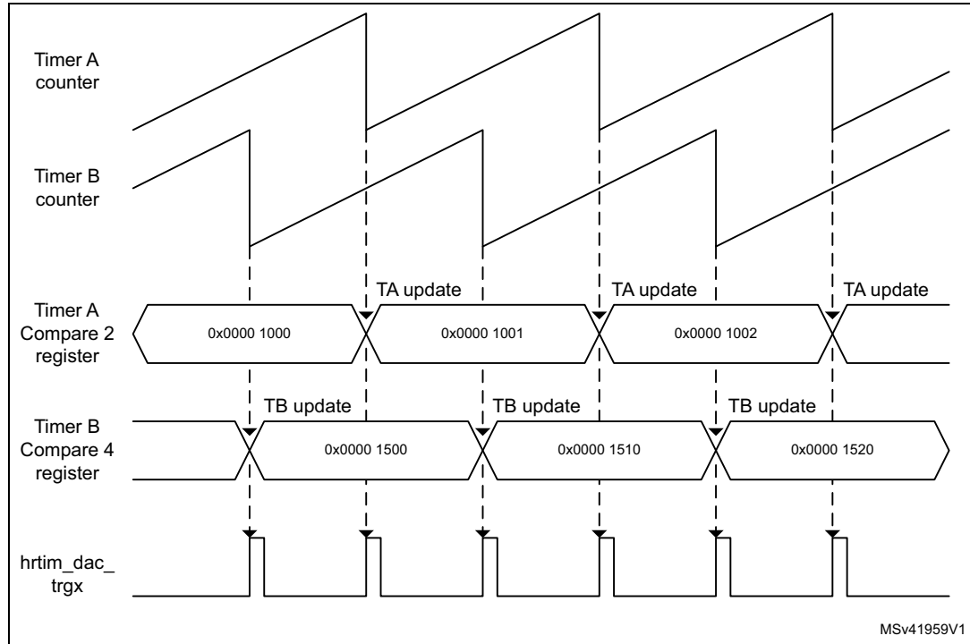
Figure 377. Combining several updates on a single hrtim_dac_trgx output
