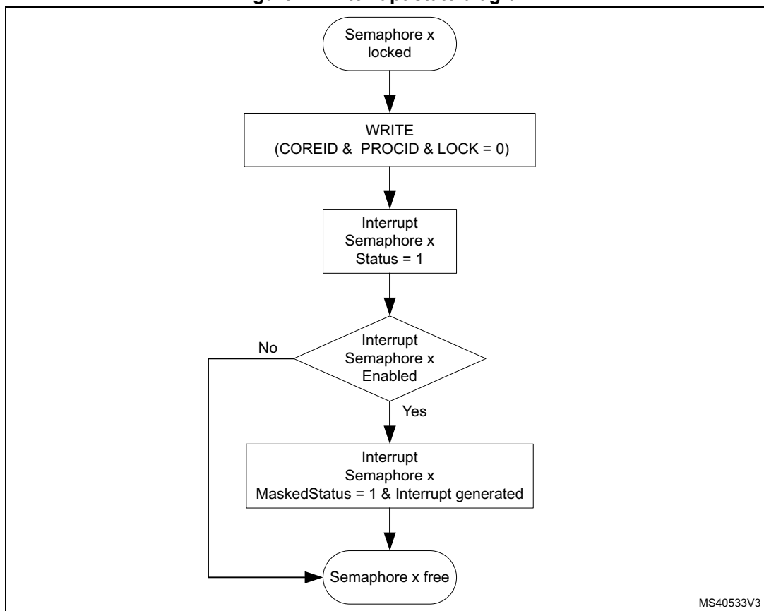
Figure 74. Interrupt state diagram
