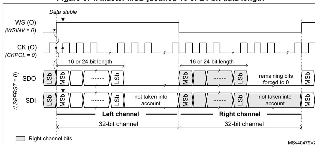
Figure 674. Master MSB justified 16 or 24-bit data length
