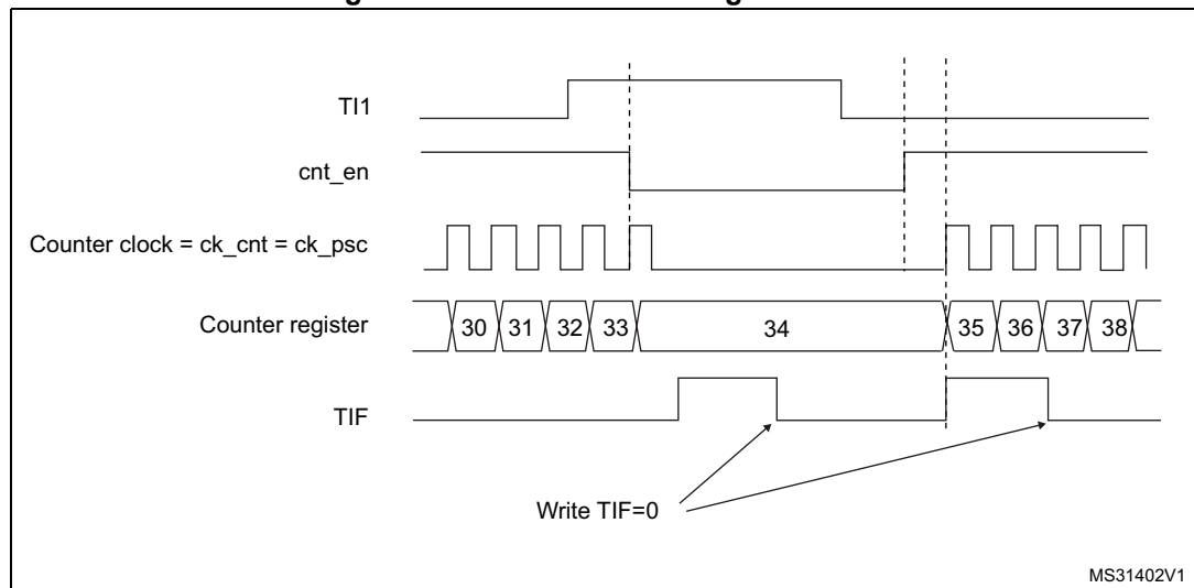
Figure 555. Control circuit in gated mode
