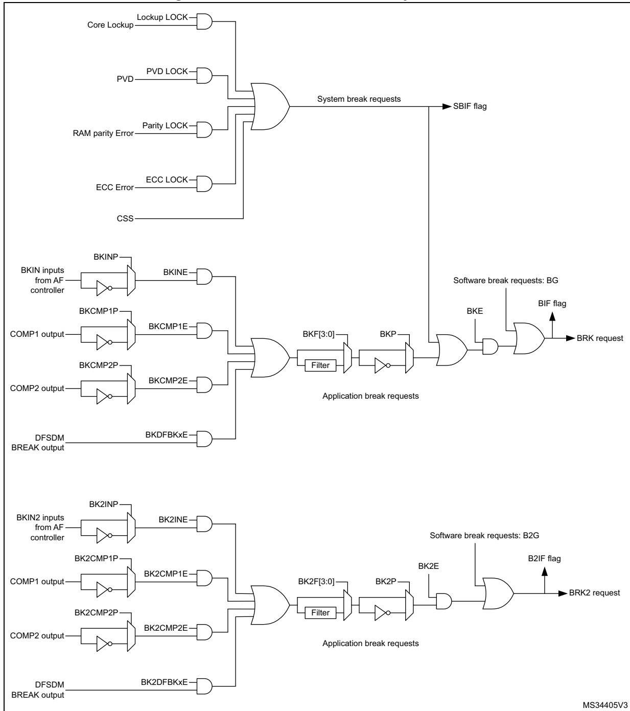
Figure 432. Break and Break2 circuitry overview
