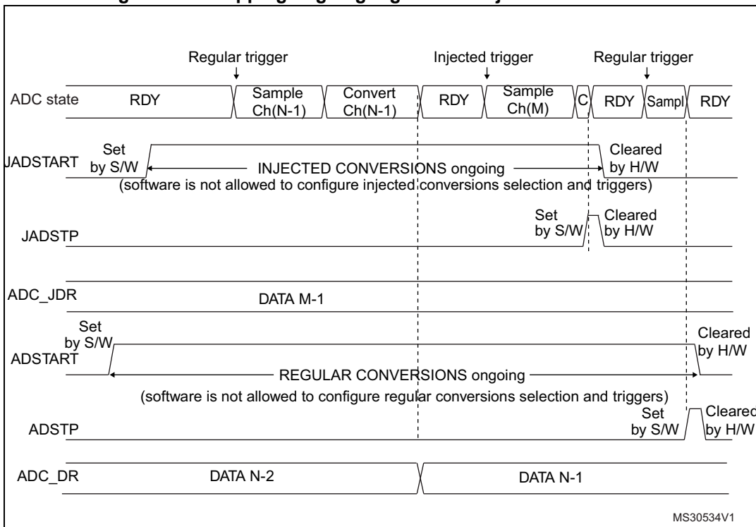
Figure 151. Stopping ongoing regular and injected conversions
