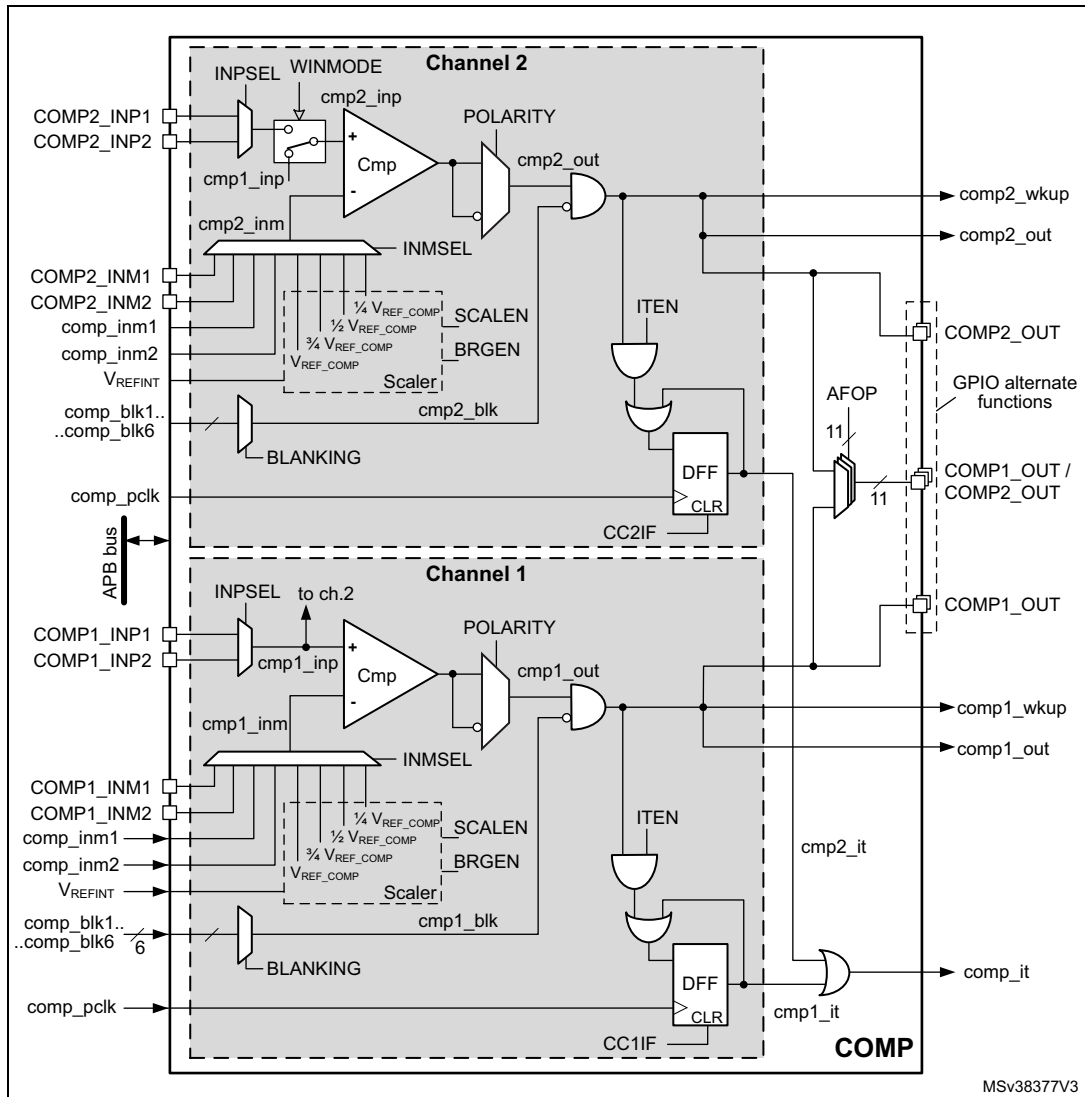
Figure 219. Comparator functional block diagram
