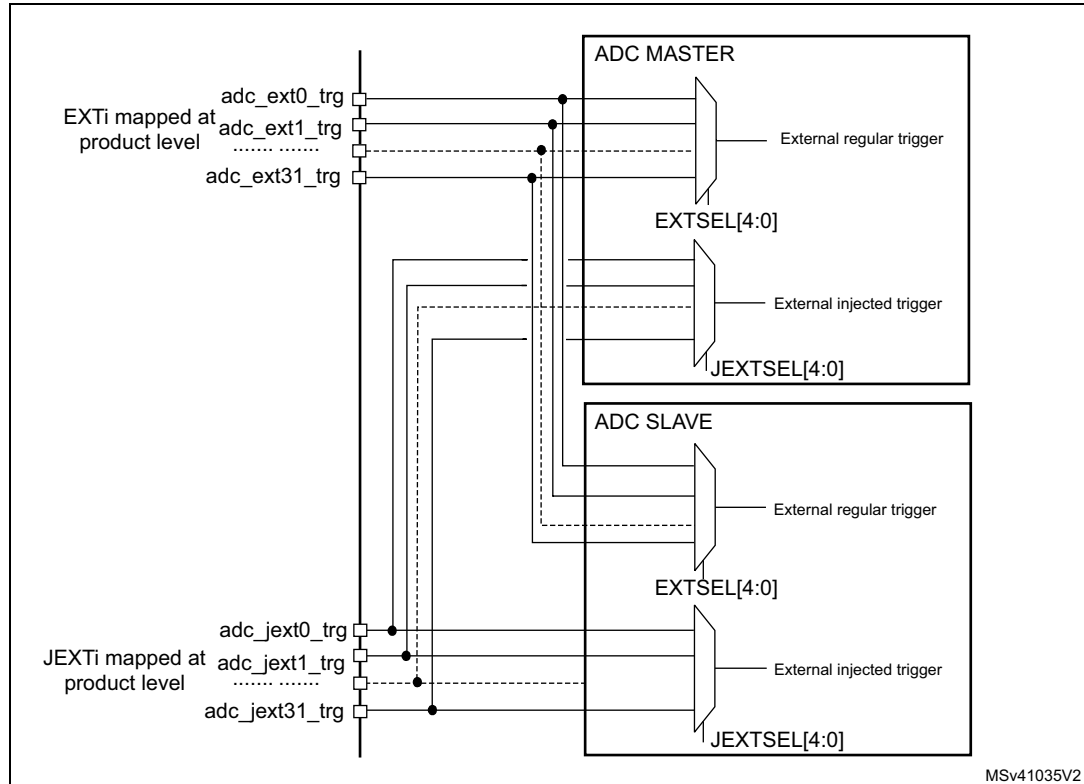
Figure 152. Triggers are shared between ADC master and ADC slave
