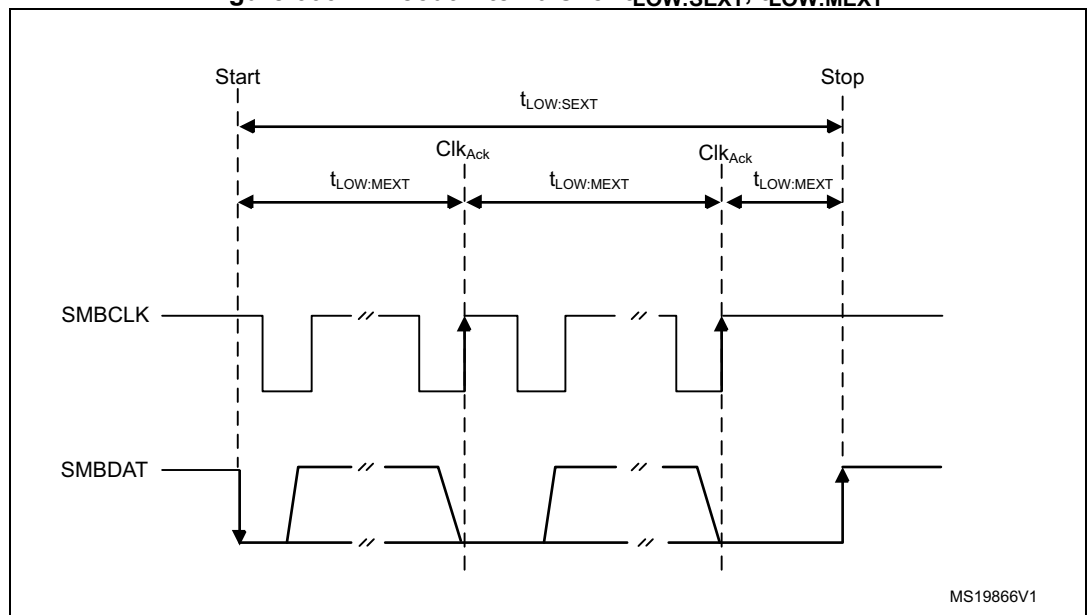
Figure 606. Timeout intervals for t_{\text{LOW:SEXT}} , t_{\text{LOW:MEXT}}
