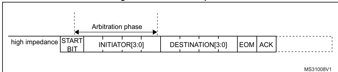
Figure 857. Arbitration phase
