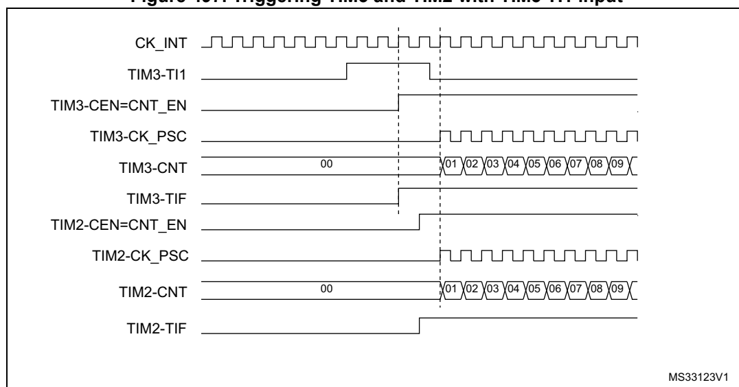
Figure 497. Triggering TIM3 and TIM2 with TIM3 TI1 input
