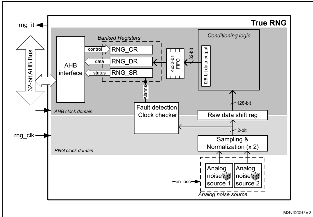
Figure 292. RNG block diagram
