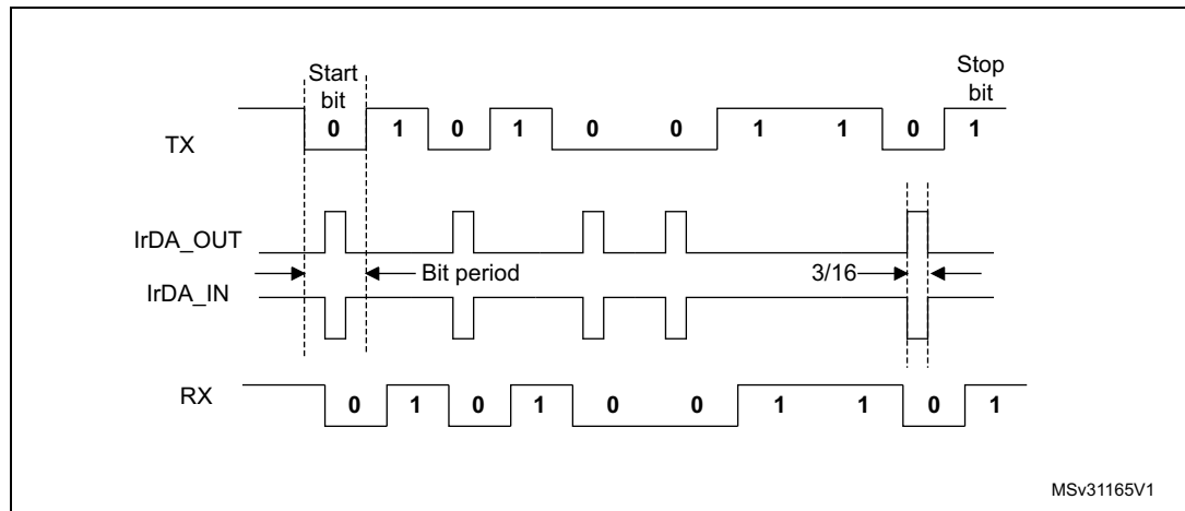
Figure 633. IrDA data modulation (3/16) - Normal mode
