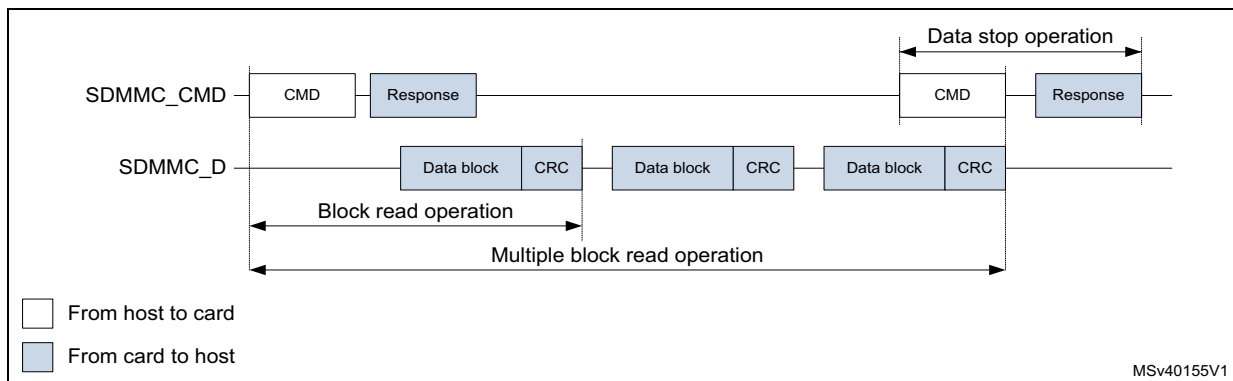
Figure 743. SDMMC (multiple) block read operation
