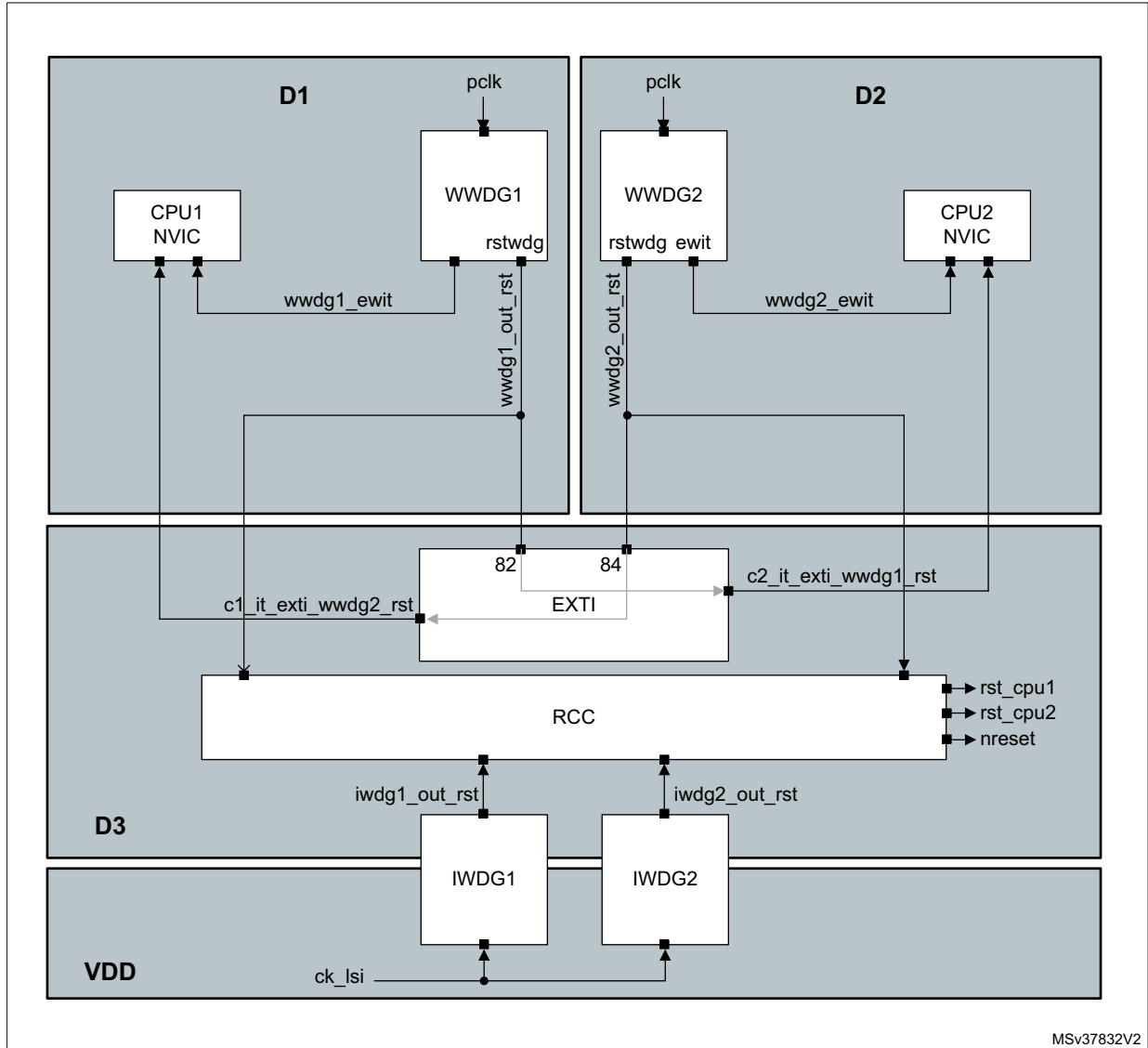
Figure 576. Watchdog high-level block diagram
