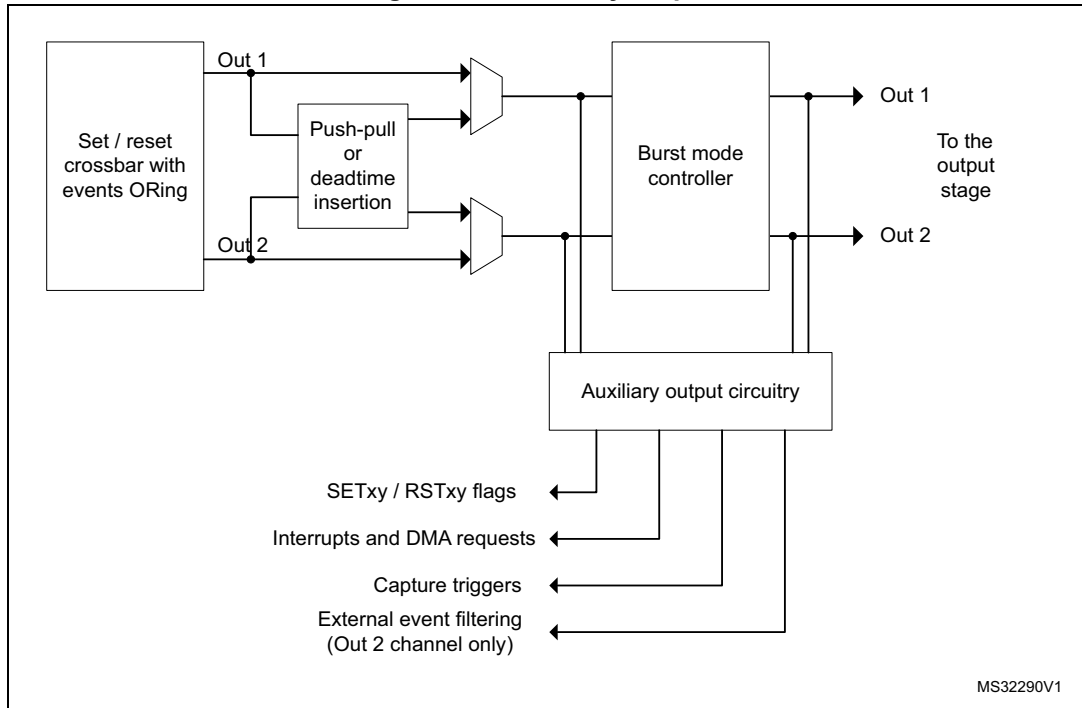
Figure 372. Auxiliary outputs
