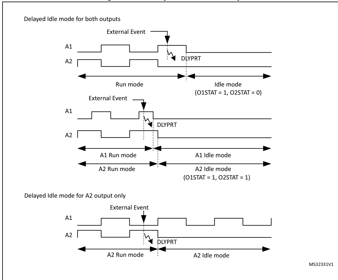
Figure 356. Delayed Idle mode entry
