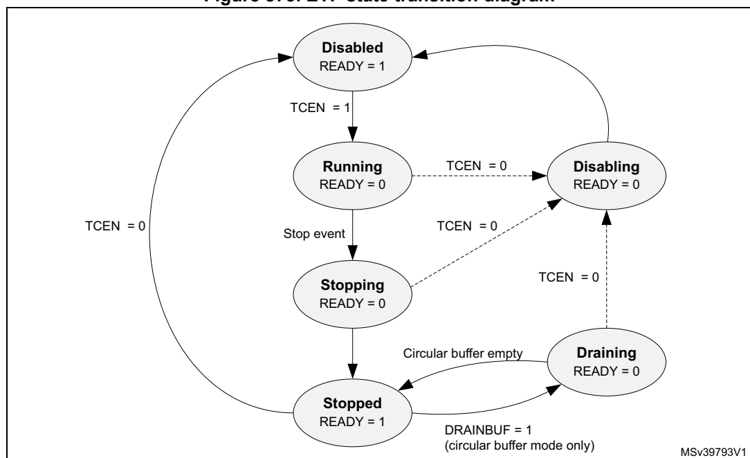
Figure 873. ETF state transition diagram
