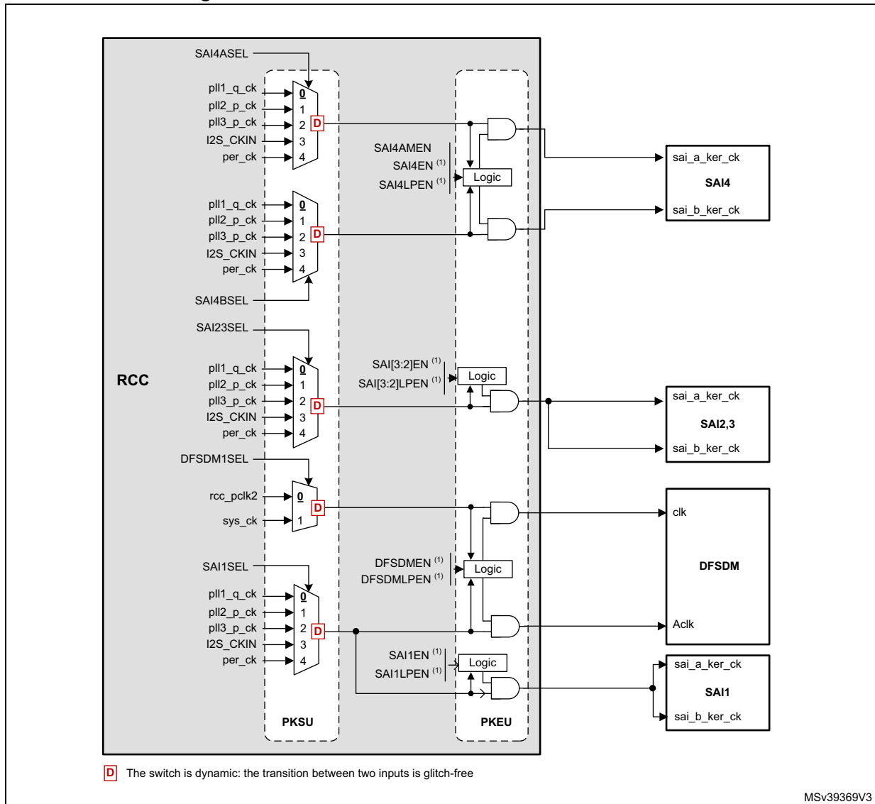
Figure 55. Kernel clock distribution for SAIs and DFSDM1
