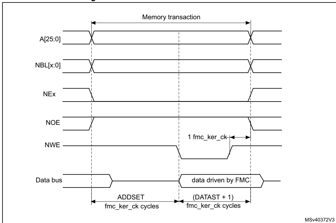
Figure 107. Mode A write access waveforms
