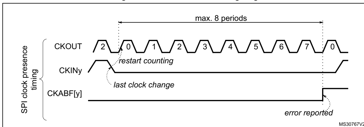
Figure 235. Clock absence timing diagram for SPI
