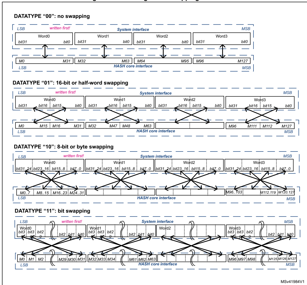
Figure 323. Message data swapping feature
