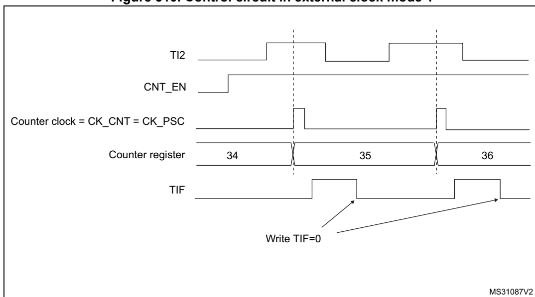
Figure 510. Control circuit in external clock mode 1
