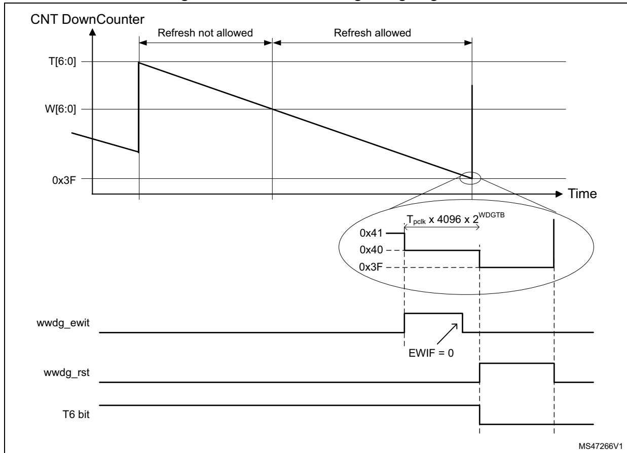
Figure 578. Window watchdog timing diagram
