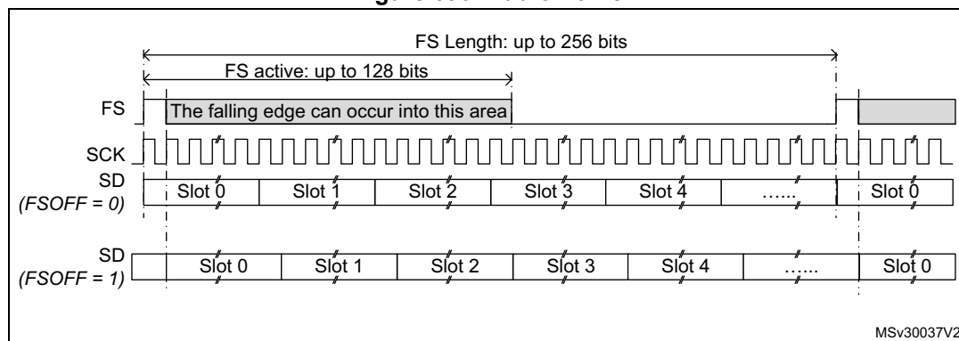
Figure 690. Audio frame
