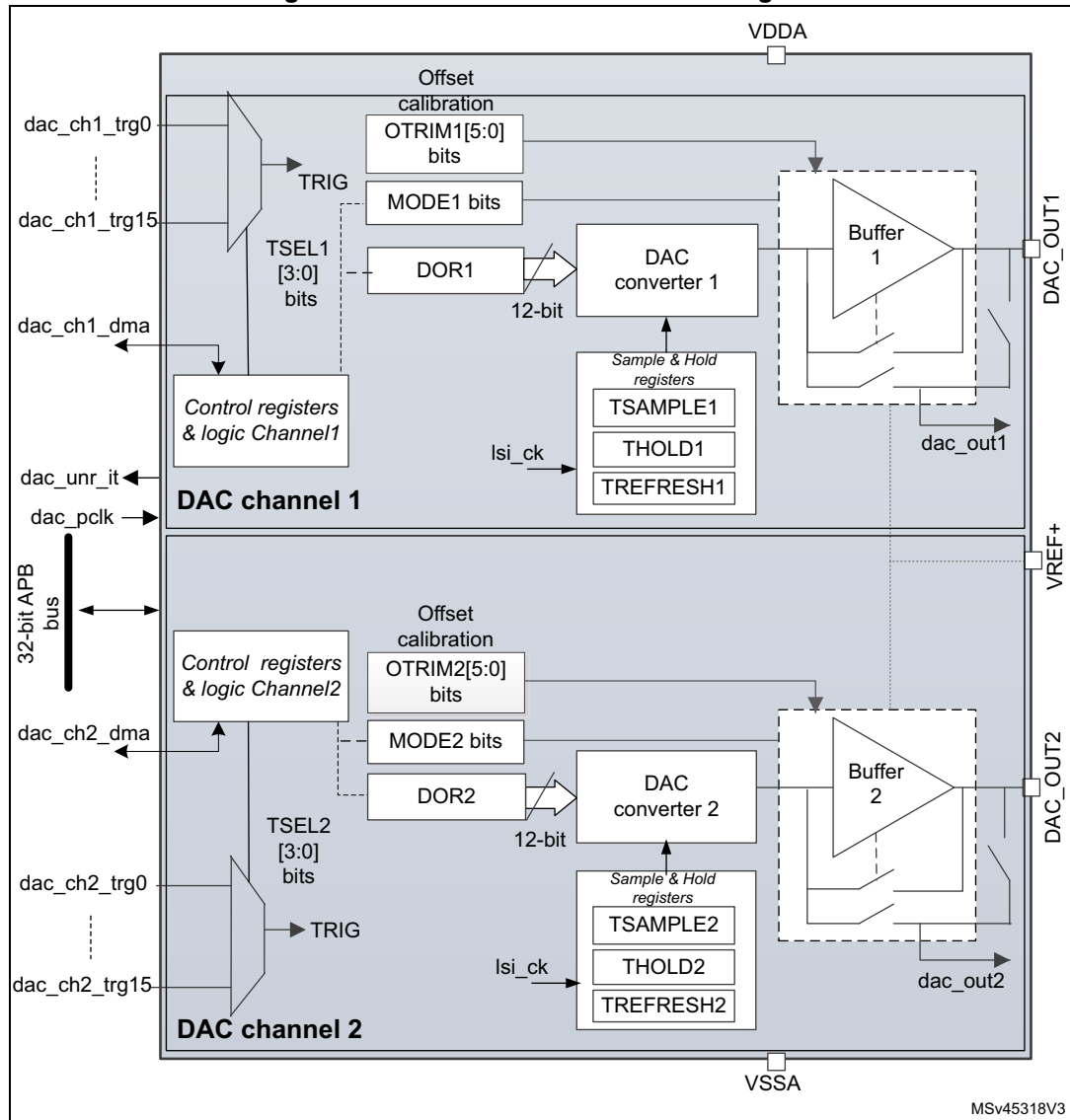
Figure 210. Dual-channel DAC block diagram
