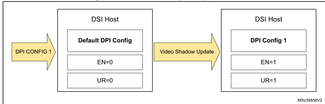
Figure 257. Immediate update procedure
