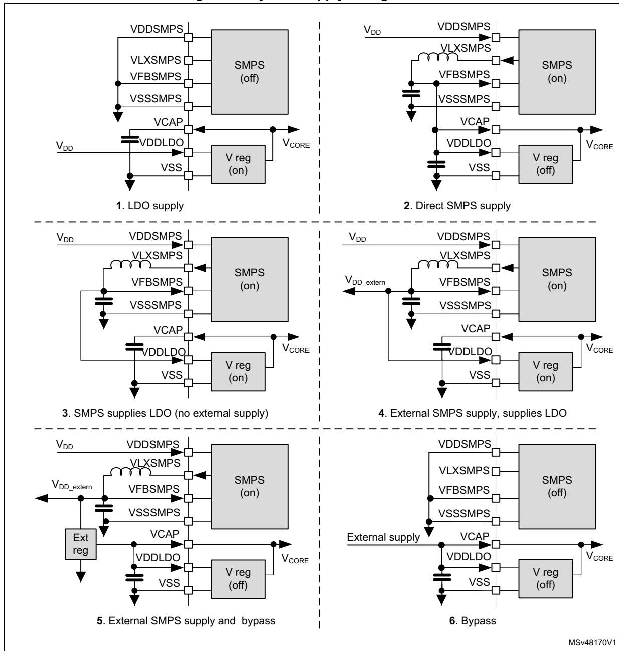
Figure 22. System supply configurations
