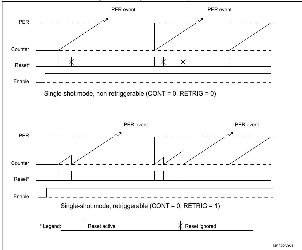
Figure 329. Single-shot timer operation
