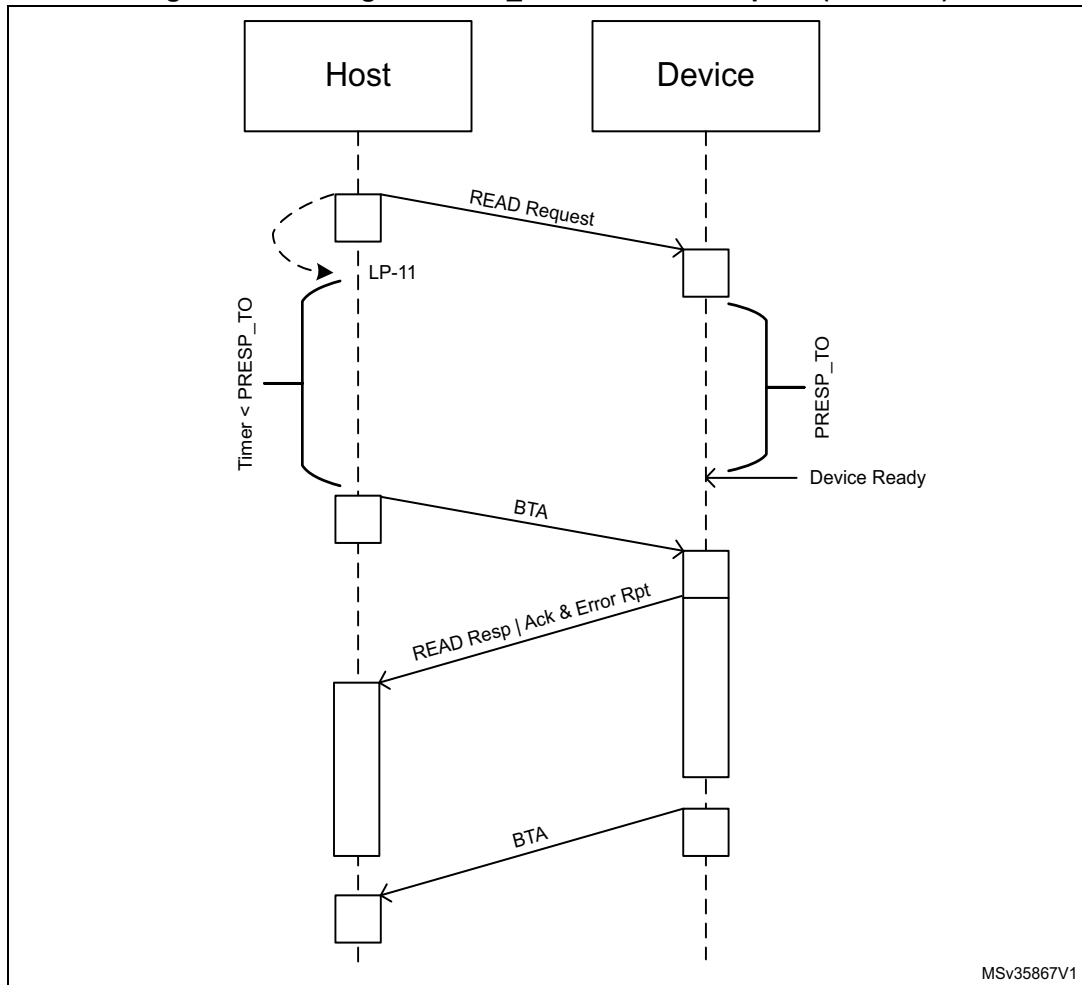
Figure 266. Timing of PRESP_TO after a read request (HS or LP)
