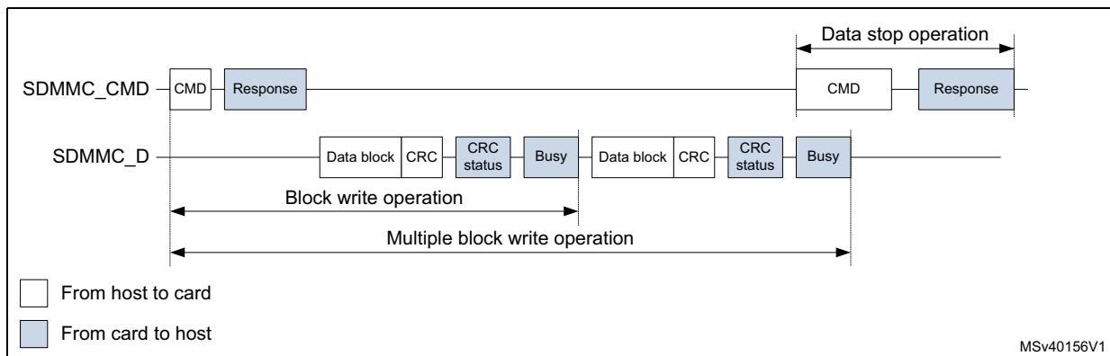
Figure 744. SDMMC (multiple) block write operation
