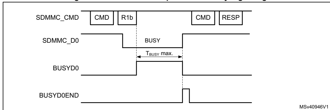
Figure 771. Command response R1b busy signaling
