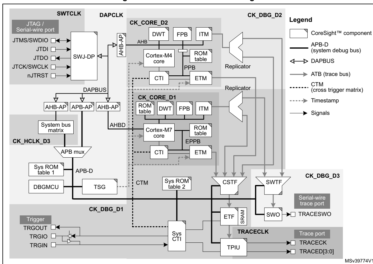
Figure 864. Clock domains of debug infrastructure
