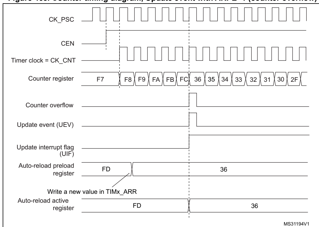
Figure 468. Counter timing diagram, Update event with ARPE=1 (counter overflow)
