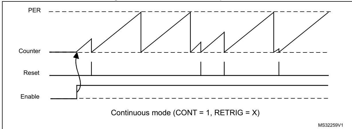
Figure 328. Continuous timer operation
