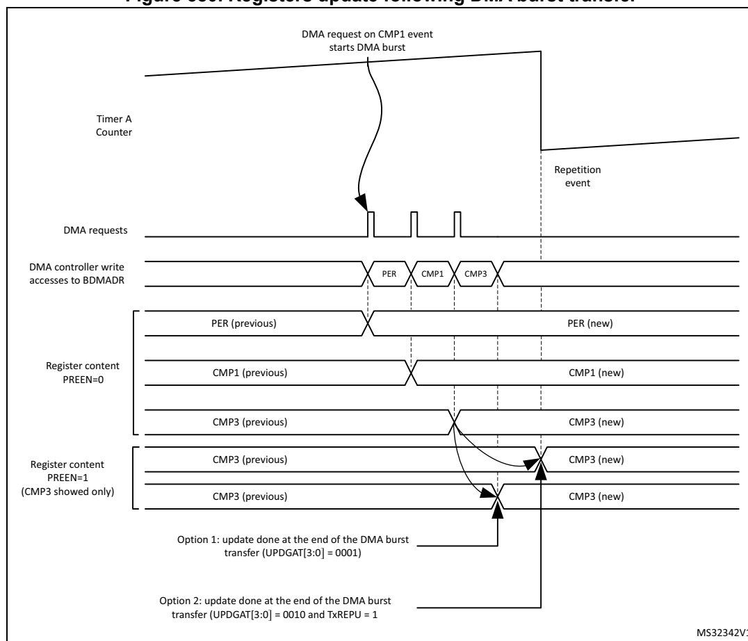
Figure 380. Registers update following DMA burst transfer
