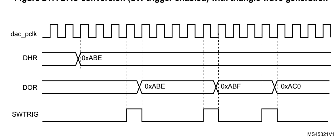
Figure 217. DAC conversion (SW trigger enabled) with triangle wave generation
