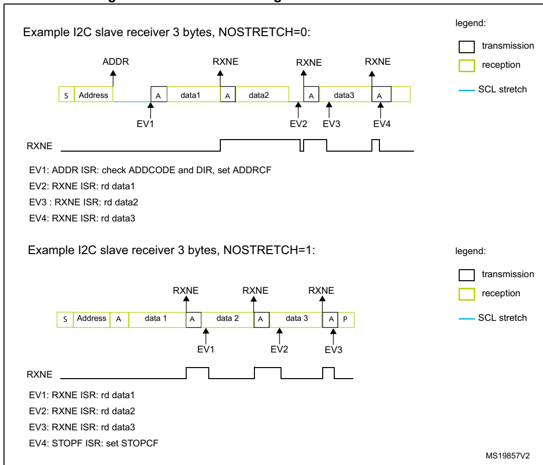
Figure 595. Transfer bus diagrams for I2C slave receiver
