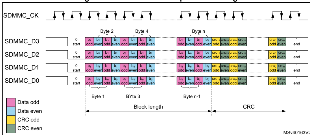
Figure 753. DDR mode data packet clocking
