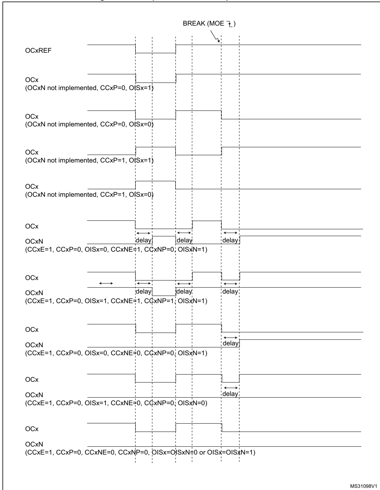
Figure 550. Output behavior in response to a break
