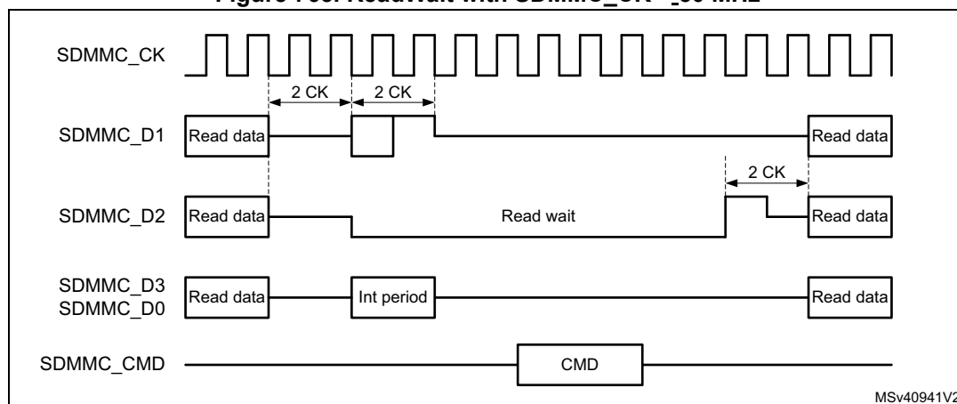
Figure 765. ReadWait with SDMMC_CK <_50 MHz
