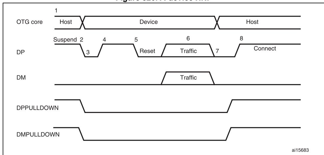
Figure 820. A-device HNP
