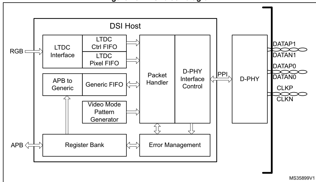
Figure 254. DSI block diagram
