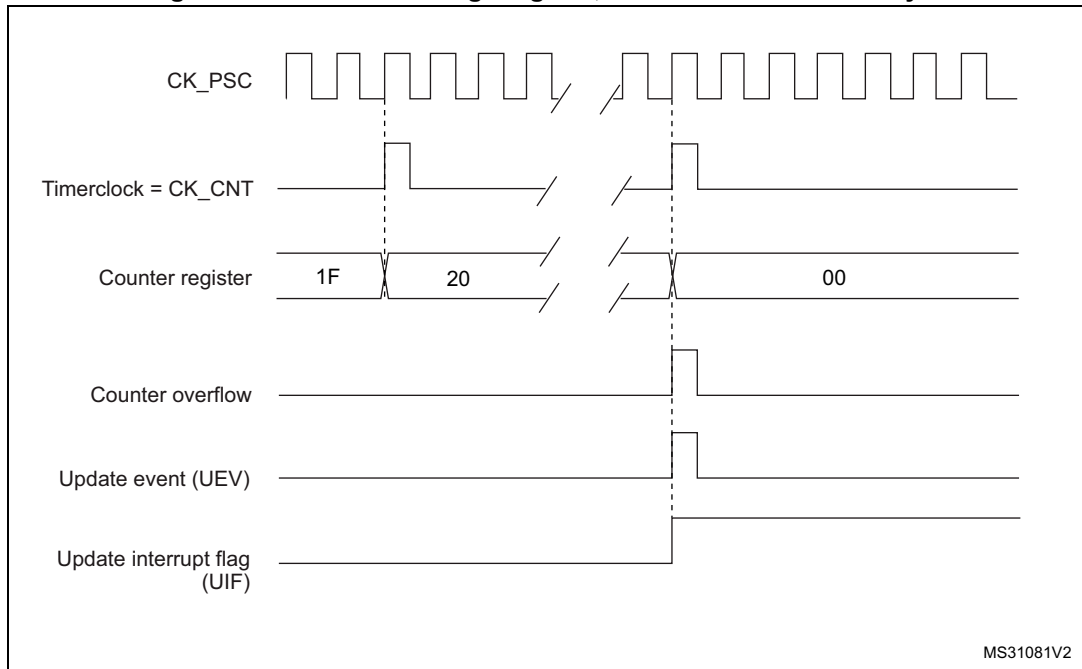
Figure 506. Counter timing diagram, update event when ARPE=0 (TIMx_ARR not preloaded)
