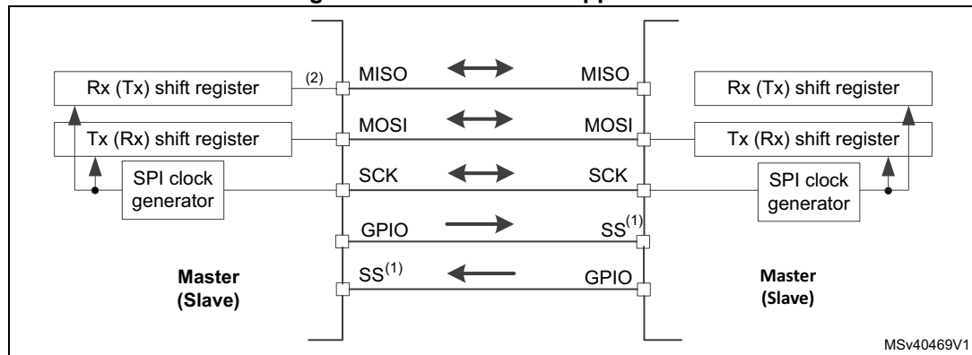
Figure 661. Multi-master application
