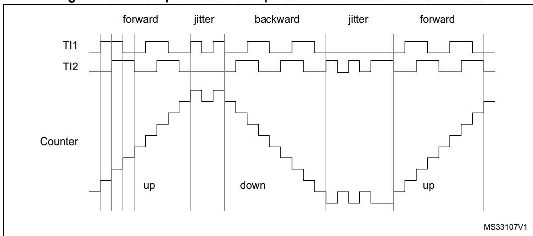
Figure 486. Example of counter operation in encoder interface mode
