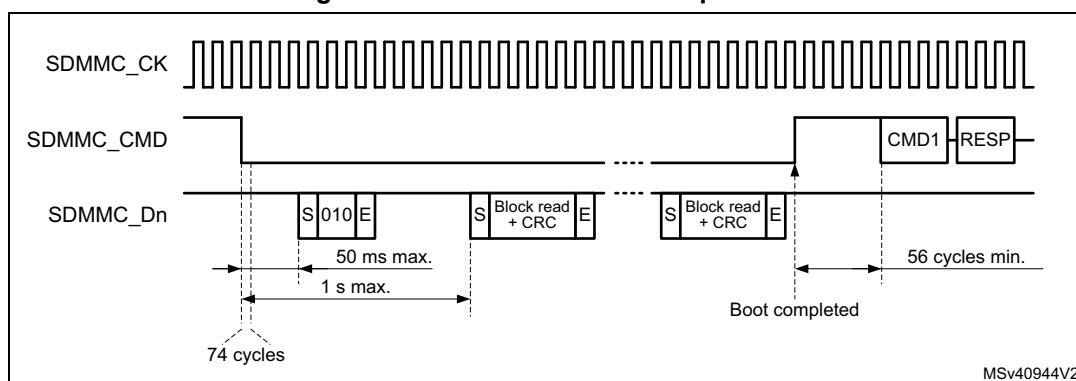
Figure 769. Normal boot mode operation
