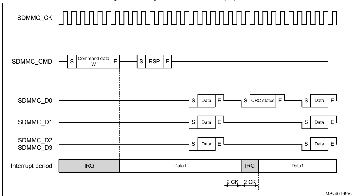
Figure 760. Synchronous interrupt period data write
