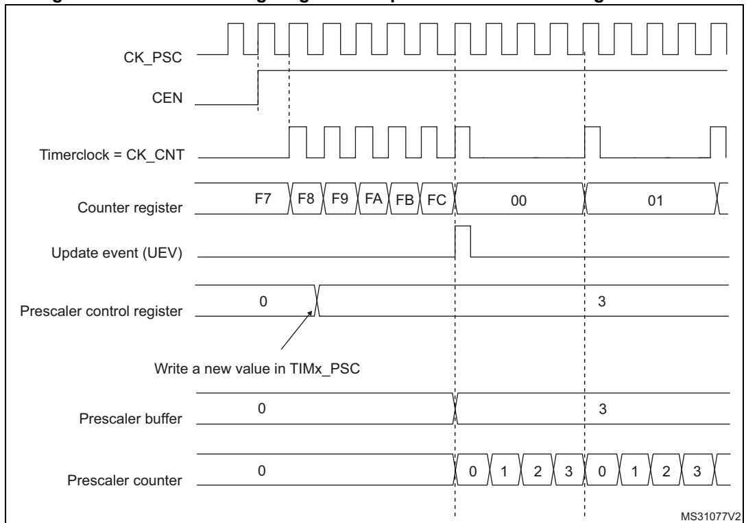
Figure 501. Counter timing diagram with prescaler division change from 1 to 4
