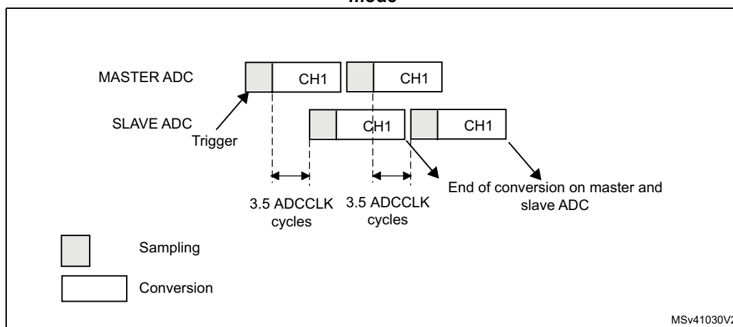
Figure 194. Interleaved mode on 1 channel in continuous conversion mode: dual ADC mode
