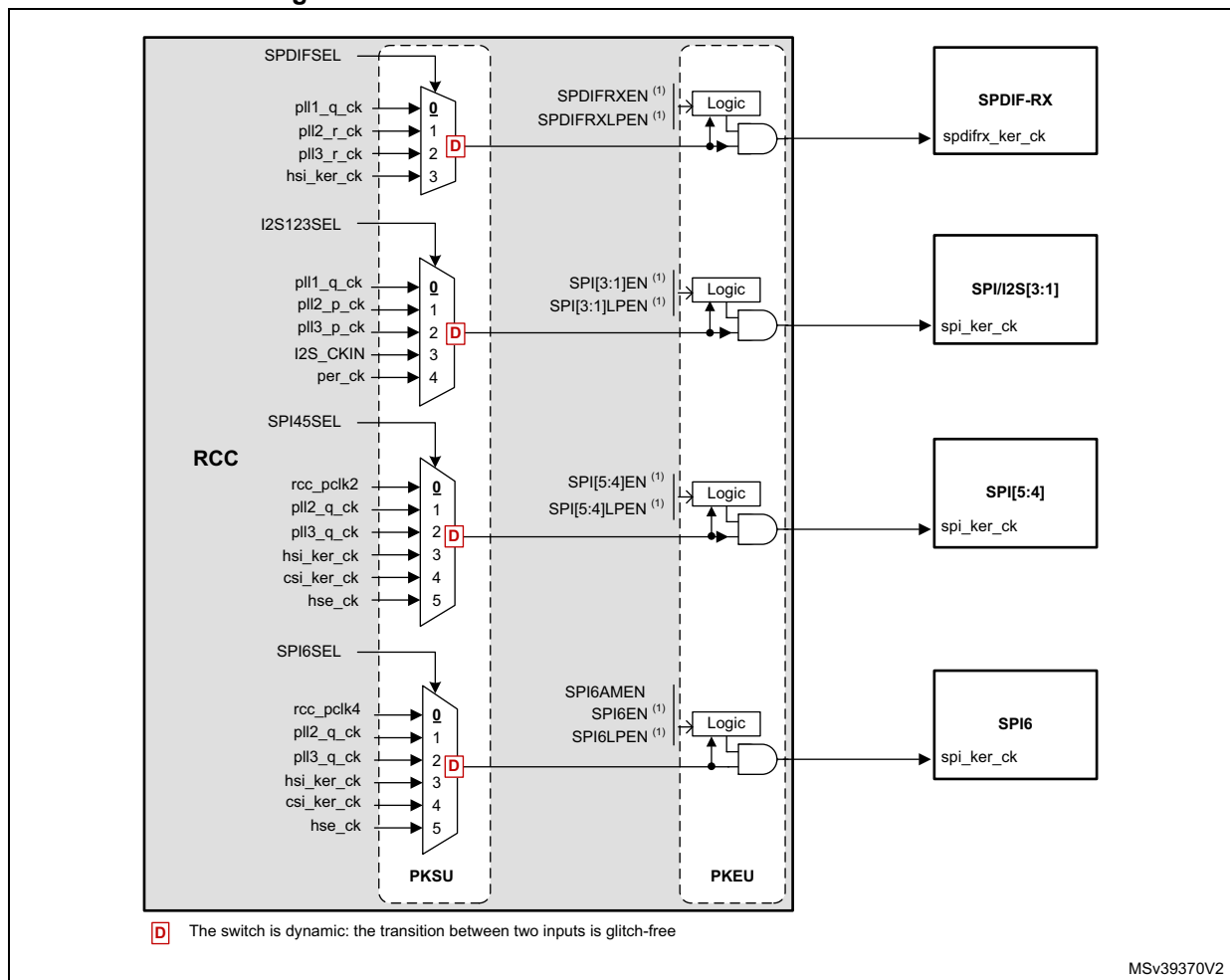
Figure 56. Kernel clock distribution for SPIs and SPI/I2S
