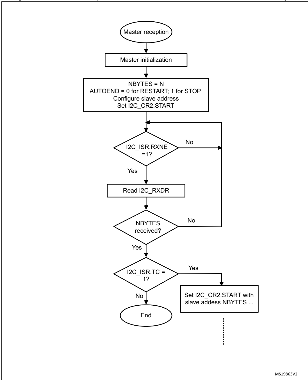
Figure 603. Transfer sequence flowchart for I2C master receiver for N≤255 bytes
