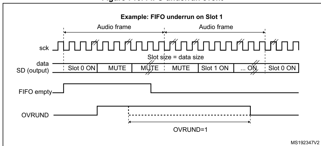
Figure 710. FIFO underrun event
