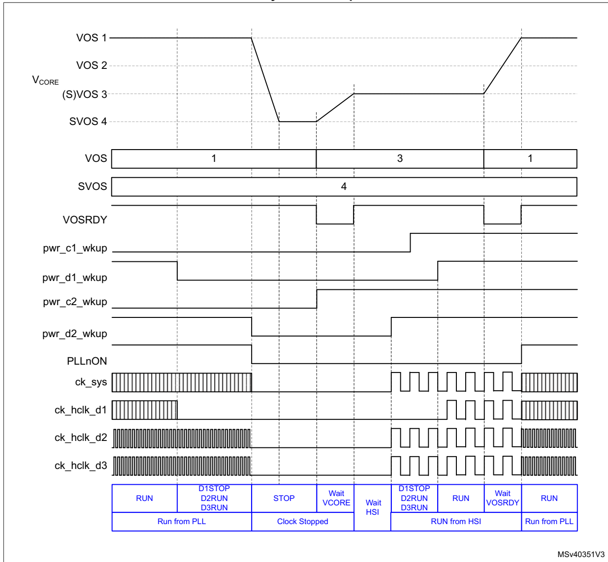
Figure 39. Dynamic voltage scaling behavior with D1, D2 and system in Stop mode
