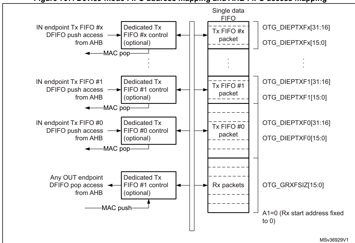
Figure 797. Device-mode FIFO address mapping and AHB FIFO access mapping
