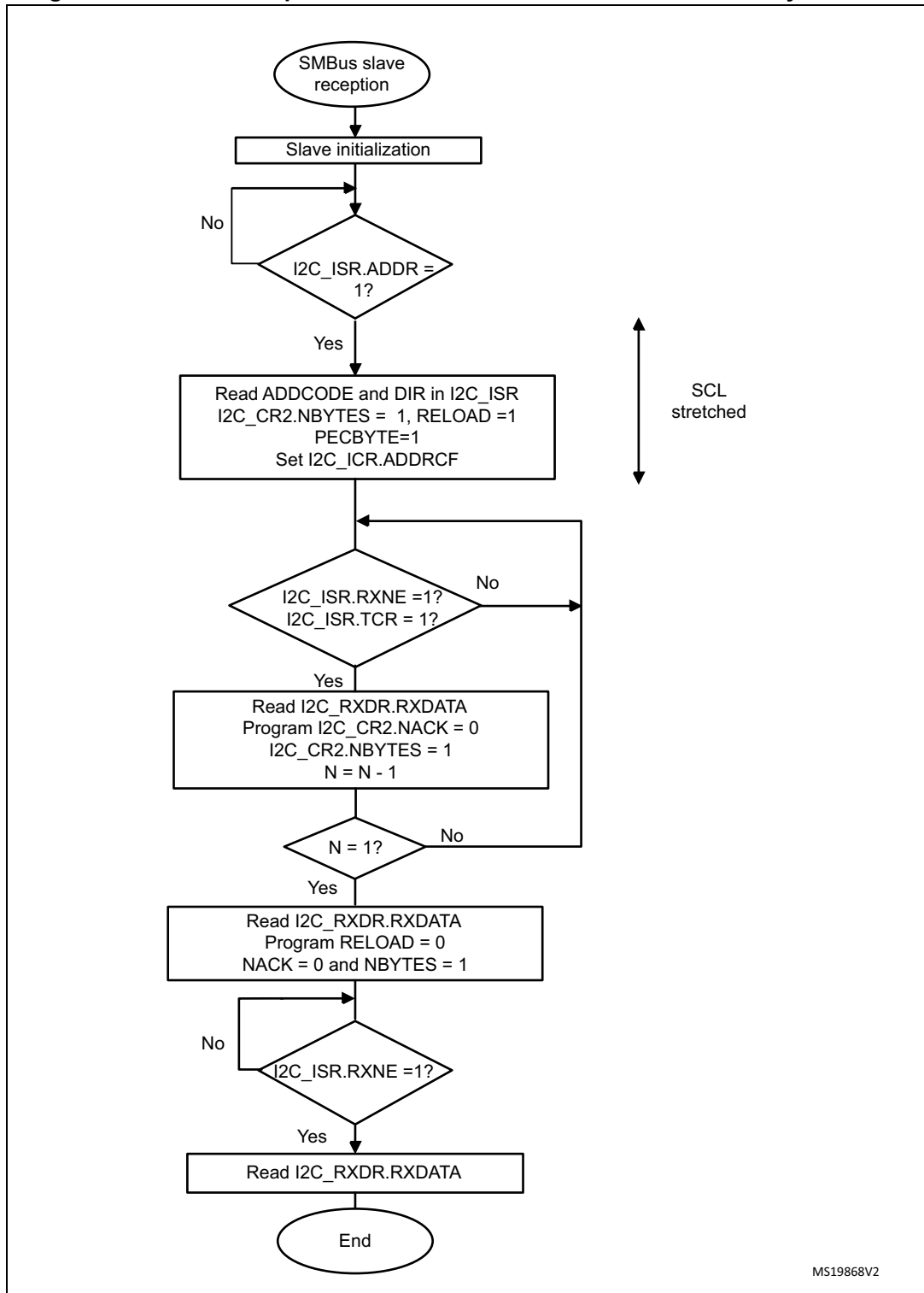
Figure 609. Transfer sequence flowchart for SMBus slave receiver N Bytes + PEC
