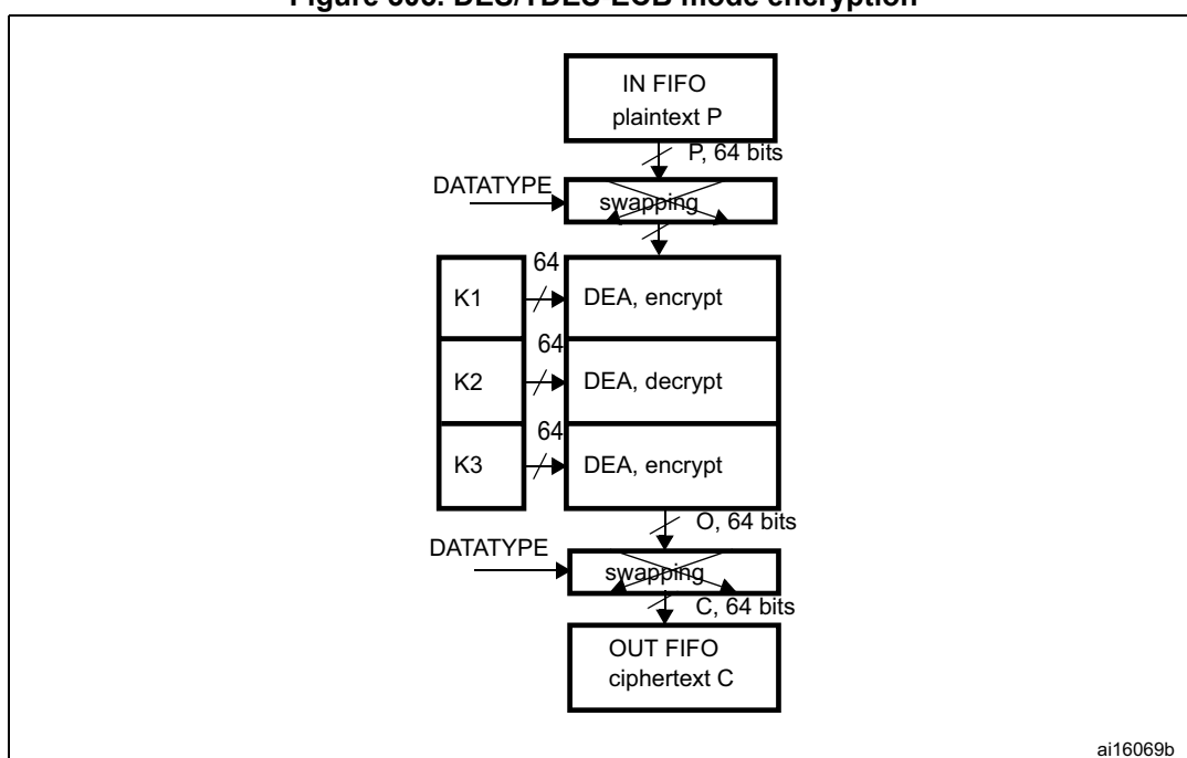
Figure 305. DES/TDES-ECB mode encryption
