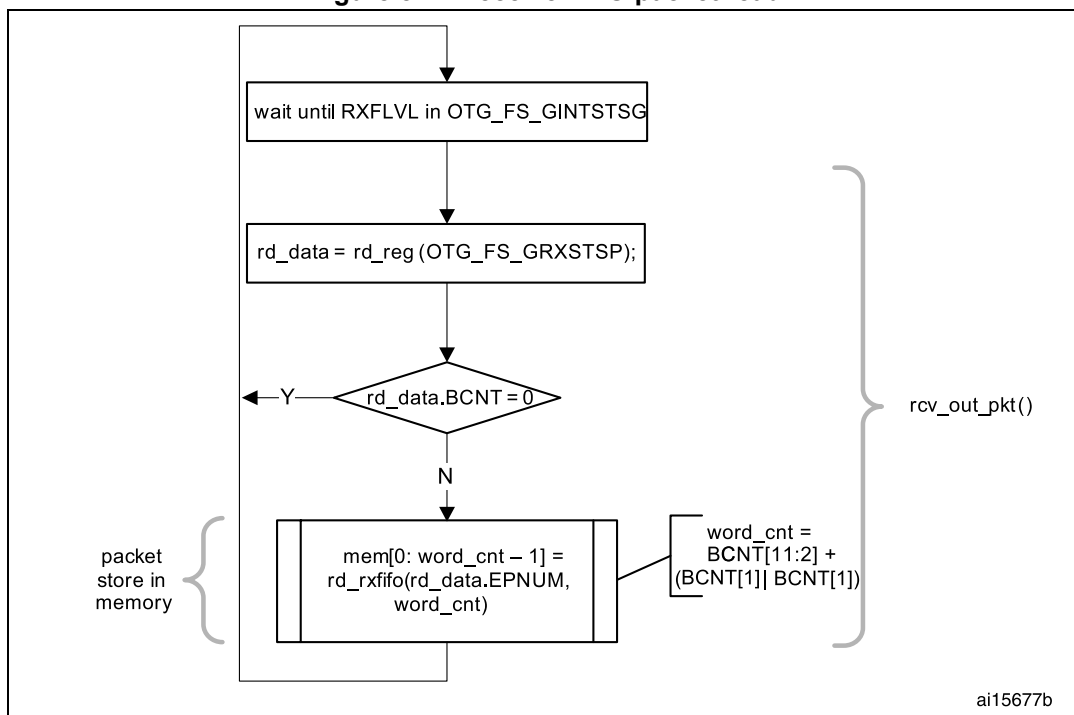
Figure 814. Receive FIFO packet read
