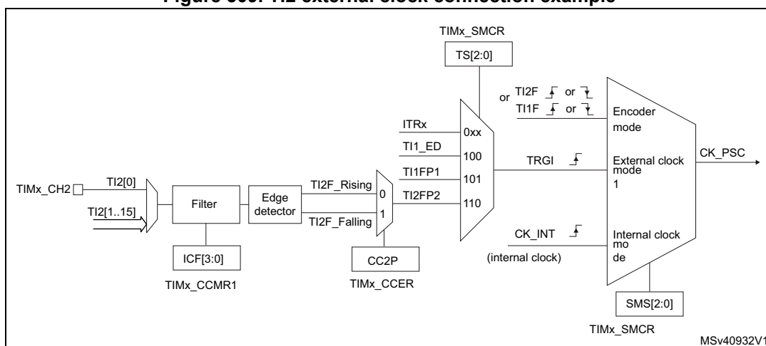
Figure 509. TI2 external clock connection example
