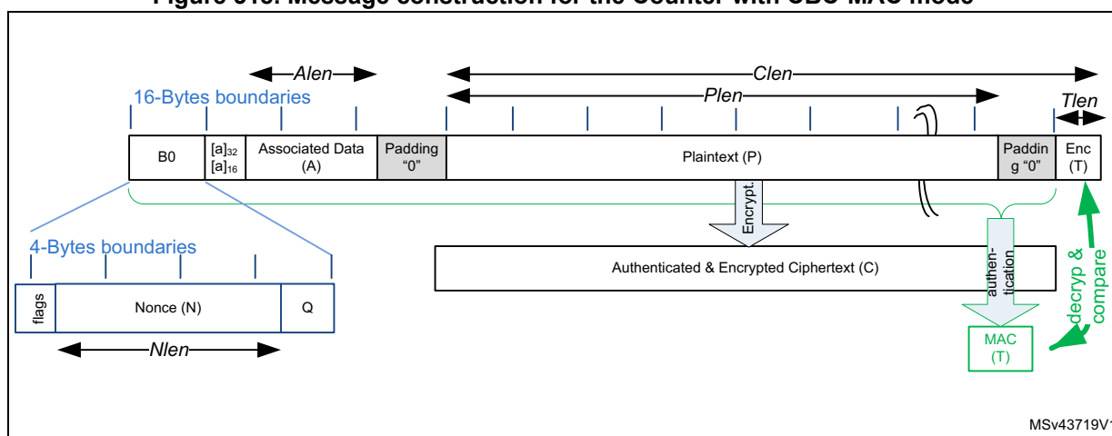
Figure 318. Message construction for the Counter with CBC-MAC mode
