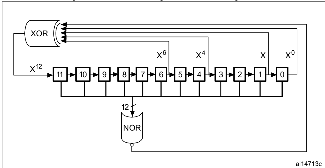
Figure 214. DAC LFSR register calculation algorithm
