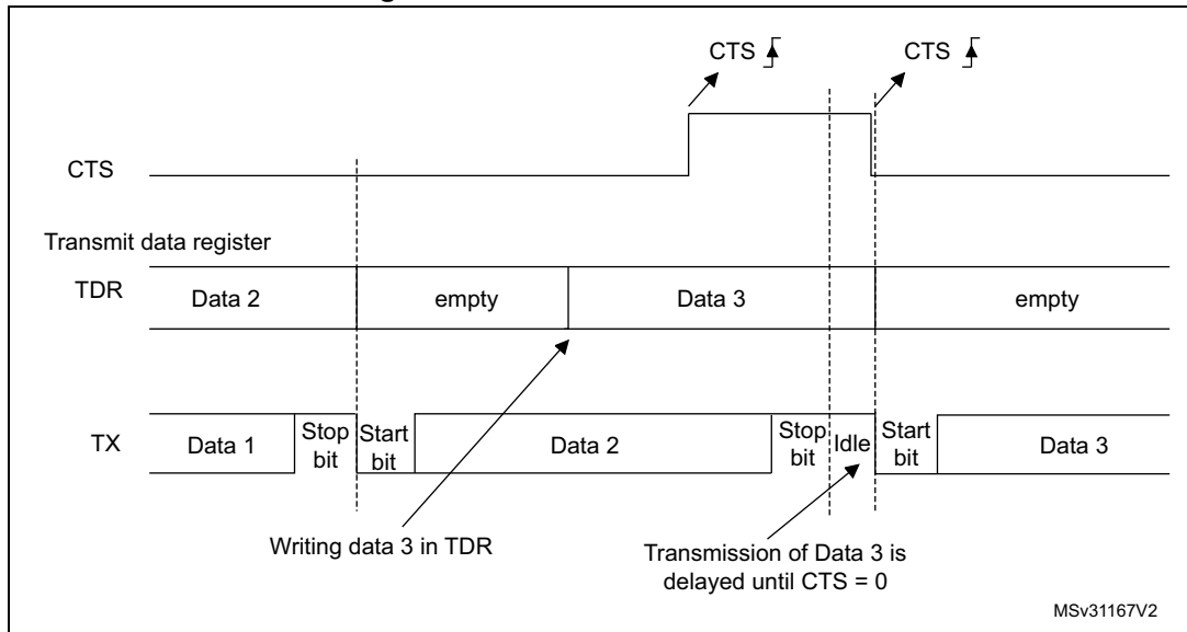
Figure 638. RS232 CTS flow control
