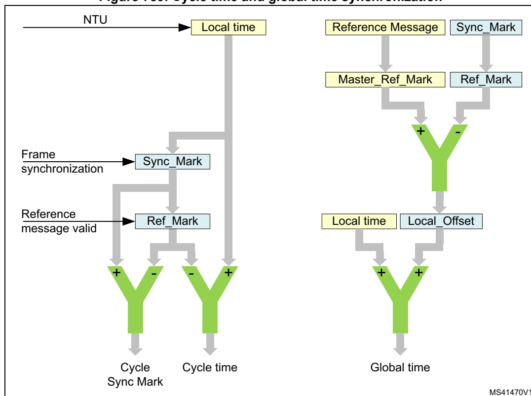
Figure 789. Cycle time and global time synchronization
