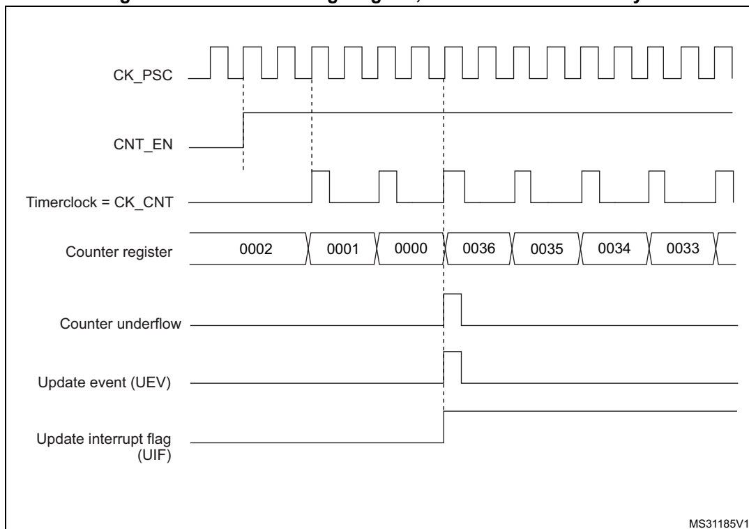
Figure 459. Counter timing diagram, internal clock divided by 2
