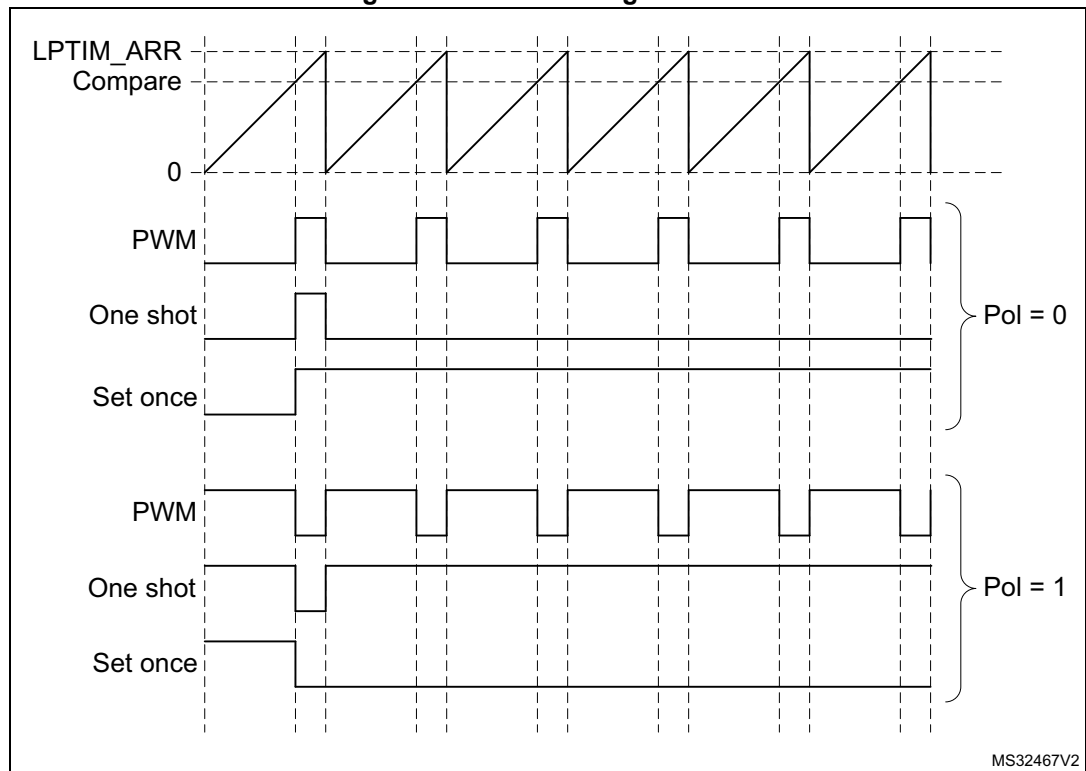
Figure 574. Waveform generation
