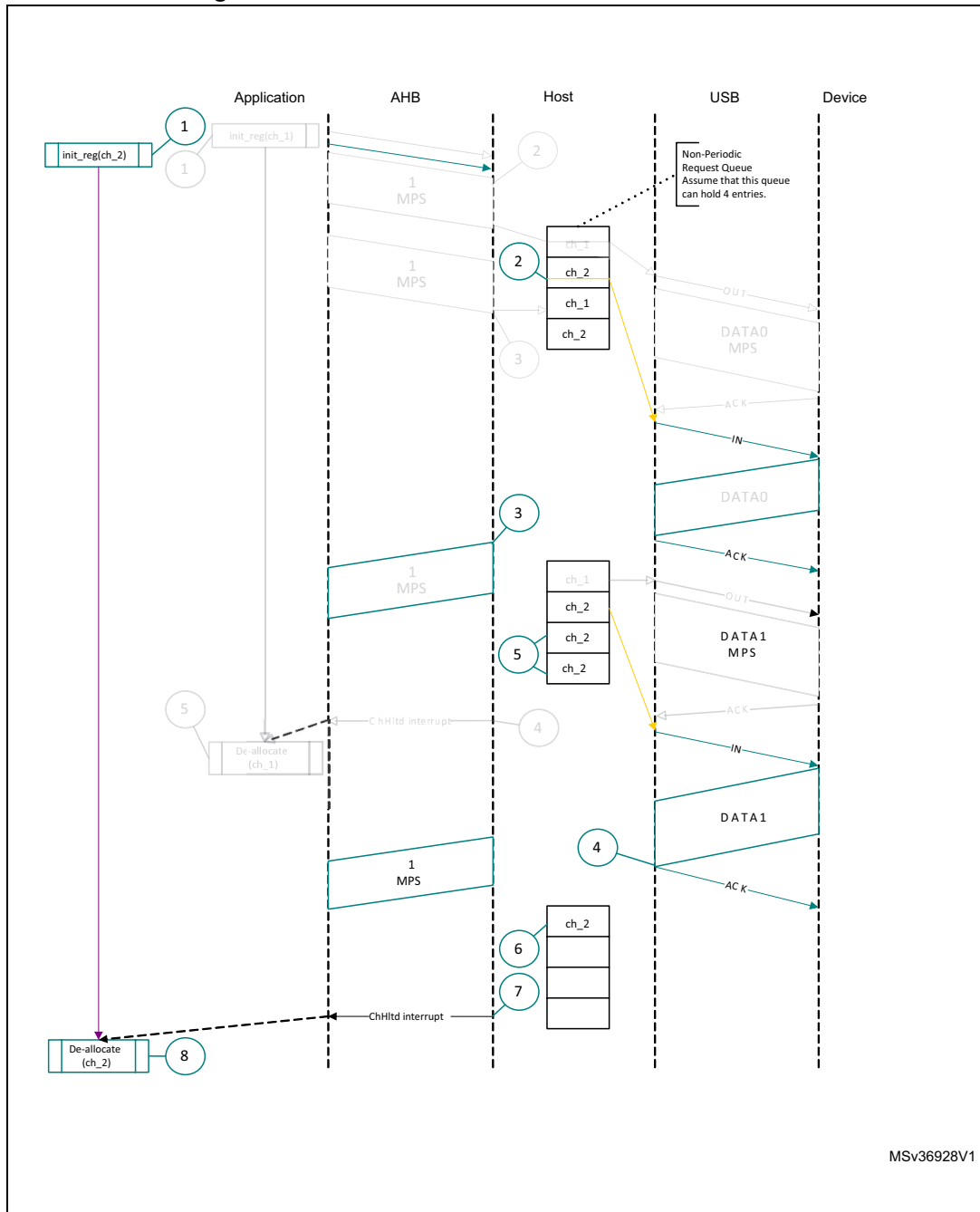
Figure 809. Normal bulk/control IN transaction - DMA
