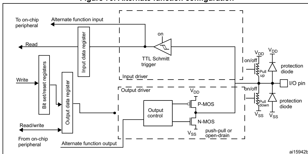
Figure 79. Alternate function configuration
