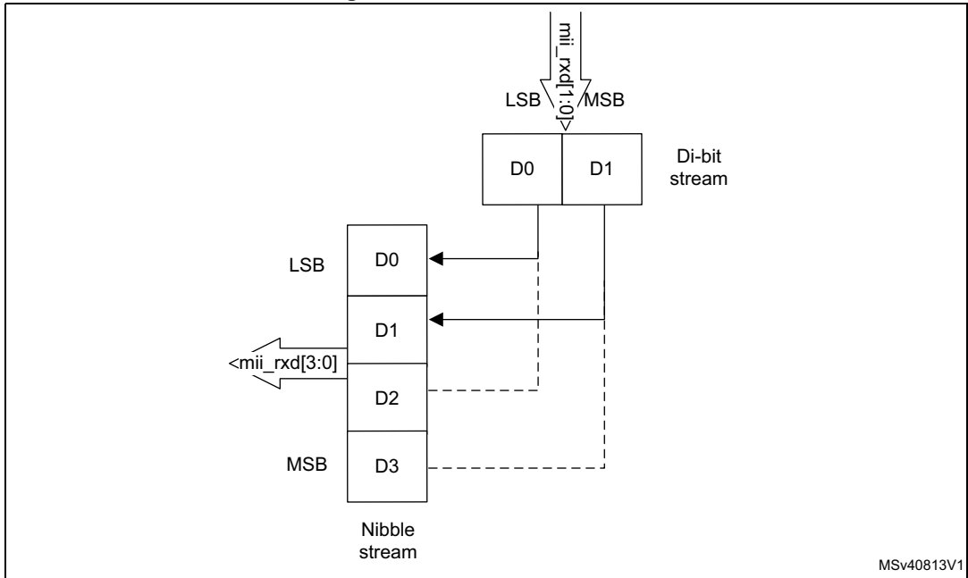
Figure 842. Receive bit order
