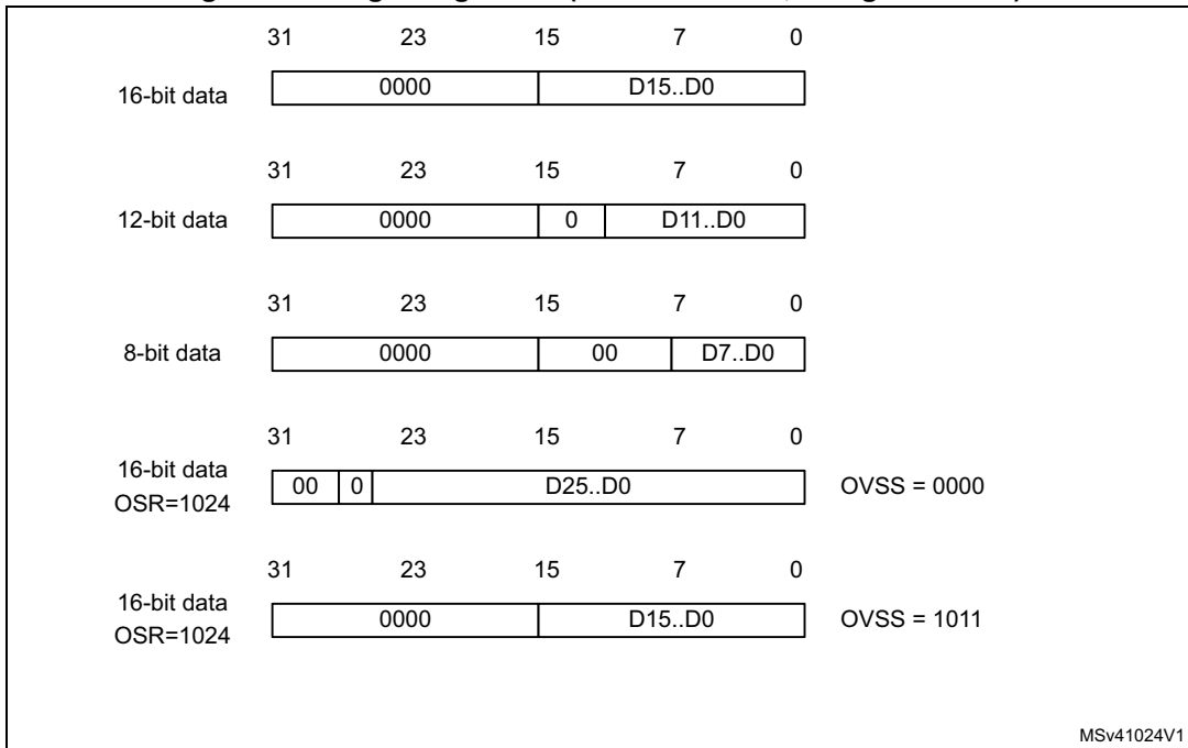
Figure 170. Right alignment (offset disabled, unsigned value)
