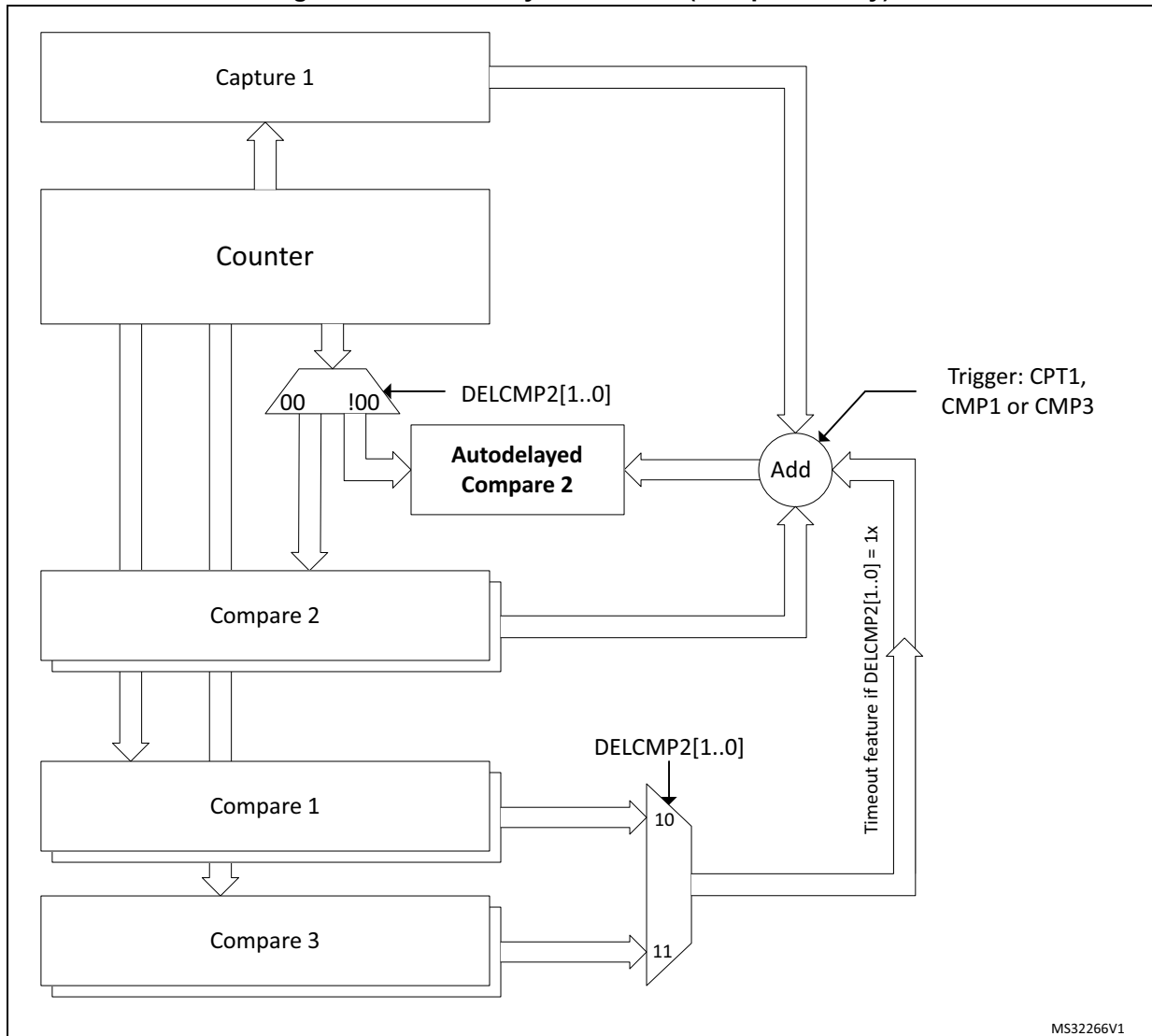
Figure 335. Auto-delayed overview (Compare 2 only)
