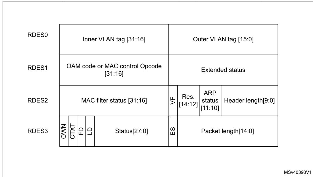
Figure 849. Receive normal descriptor (write-back format)
