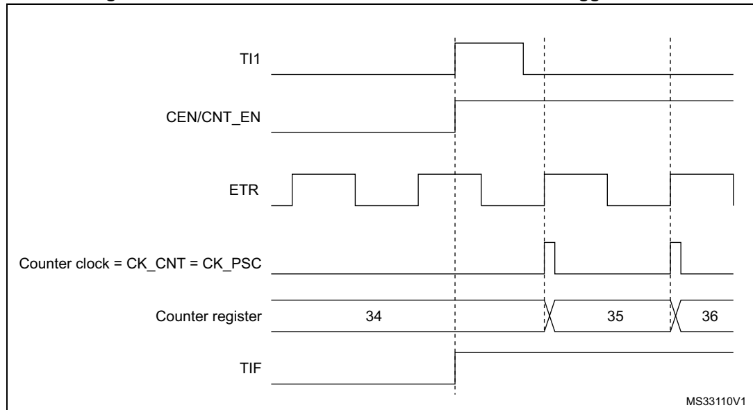
Figure 491. Control circuit in external clock mode 2 + trigger mode
