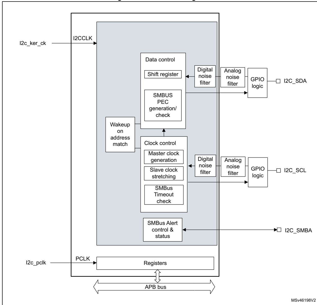
Figure 583. I2C block diagram
