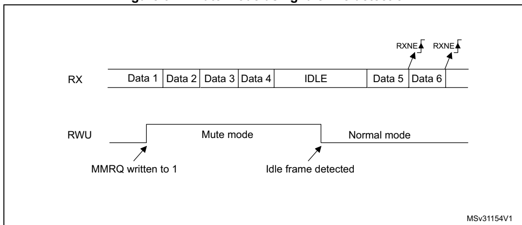
Figure 622. Mute mode using Idle line detection
