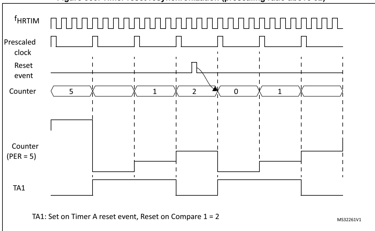
Figure 330. Timer reset resynchronization (prescaling ratio above 32)
