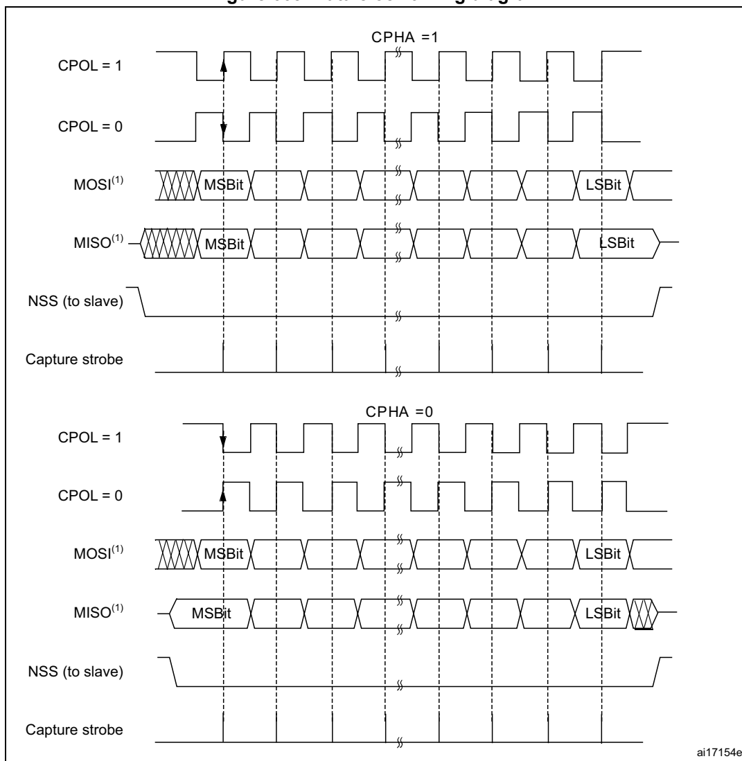
Figure 665. Data clock timing diagram
