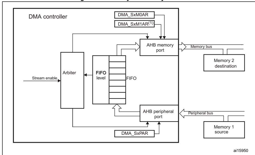
Figure 86. Memory-to-memory mode
