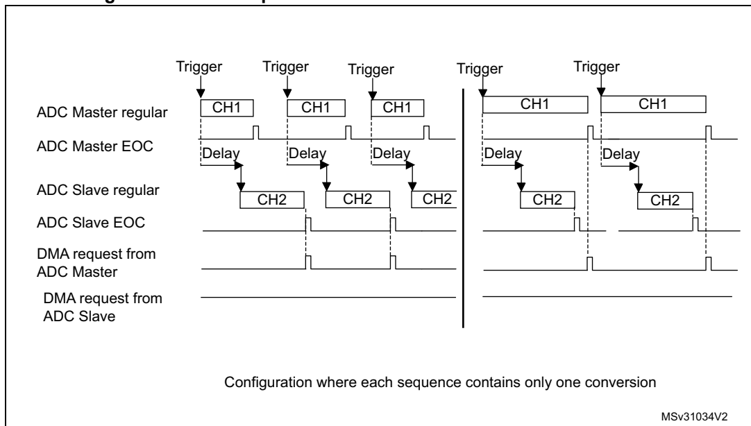
Figure 206. DMA requests in interleaved mode when DAMDF=0b10
