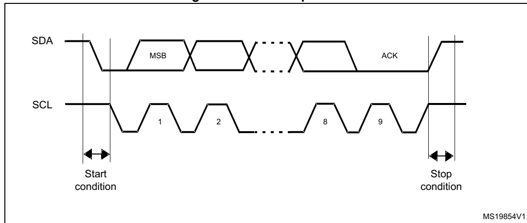
Figure 584. I 2 C bus protocol
