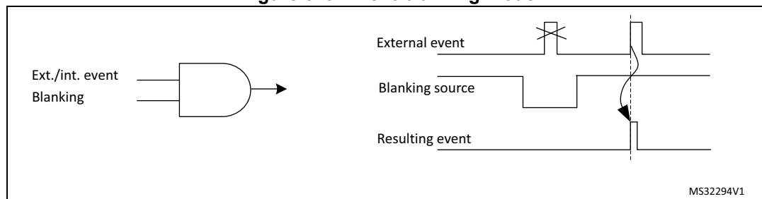
Figure 349. Event blanking mode
