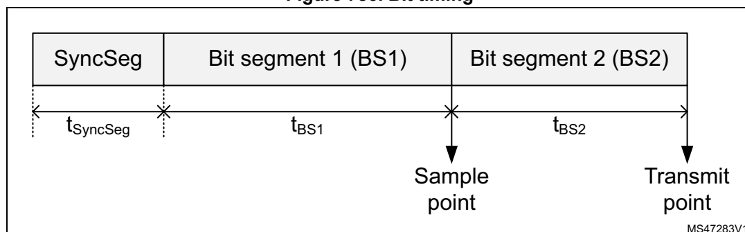
Figure 786. Bit timing
