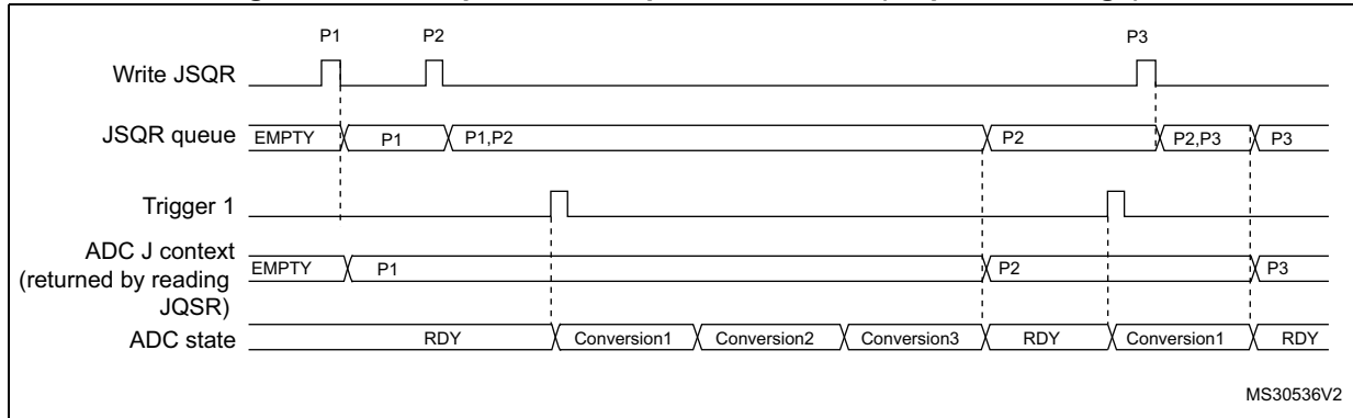
Figure 154. Example of JSQR queue of context (sequence change)
