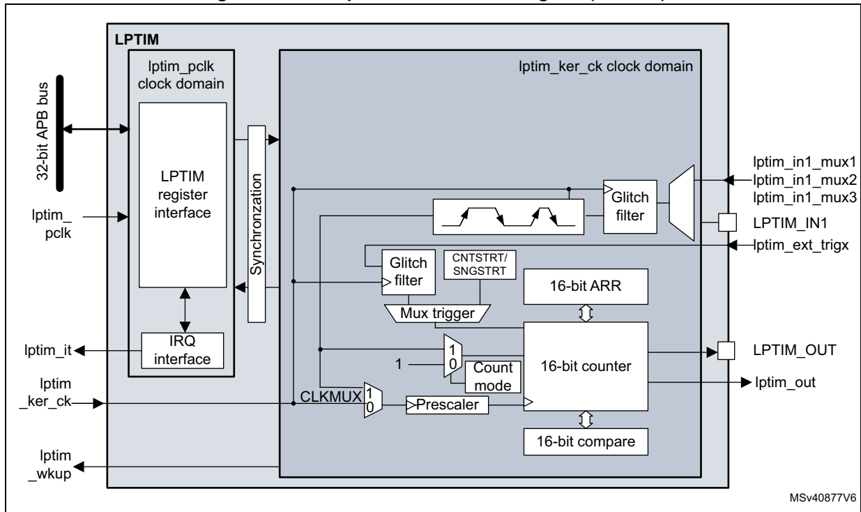
Figure 569. Low-power timer block diagram (LPTIM4 and LPTIM5)
