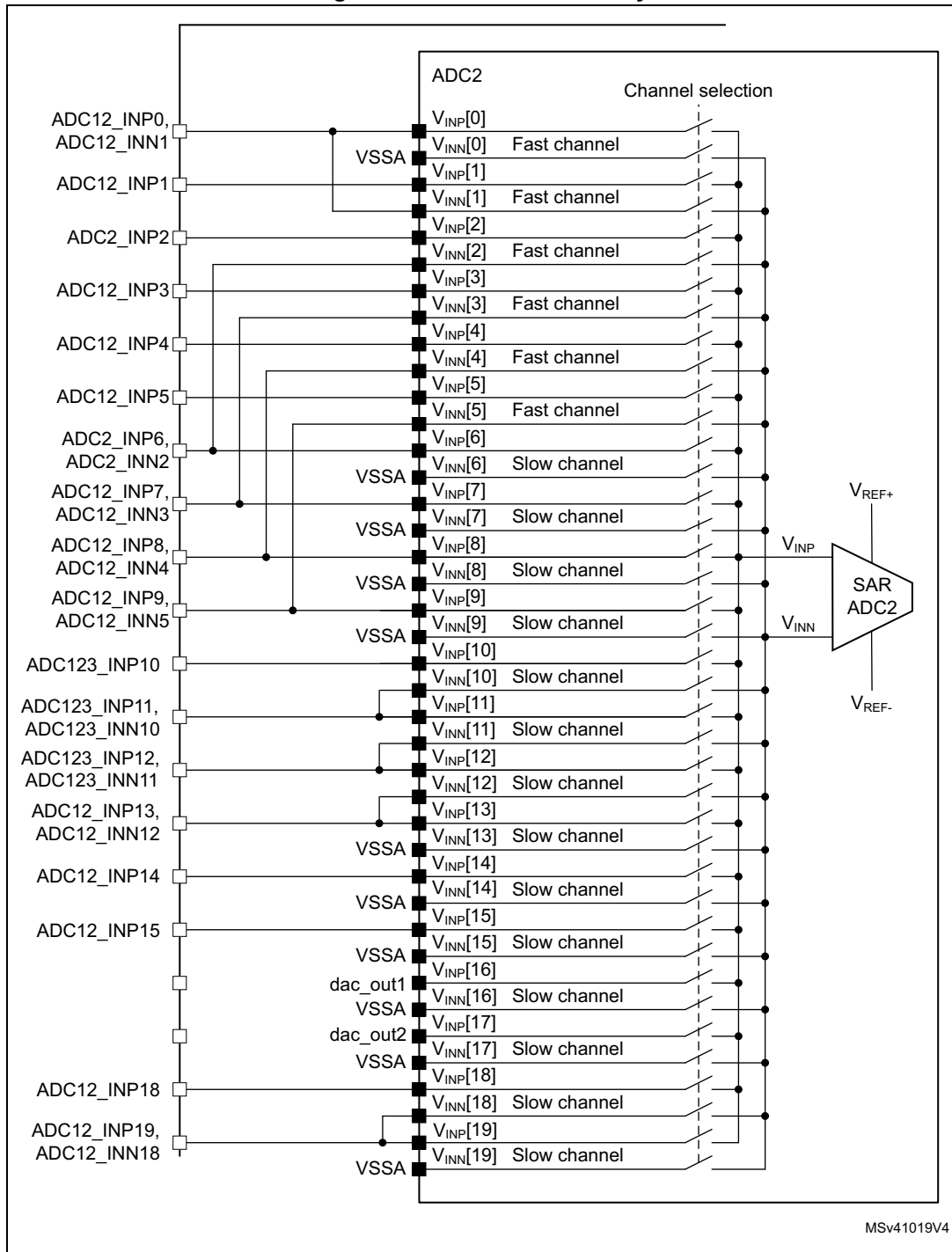
Figure 143. ADC2 connectivity
