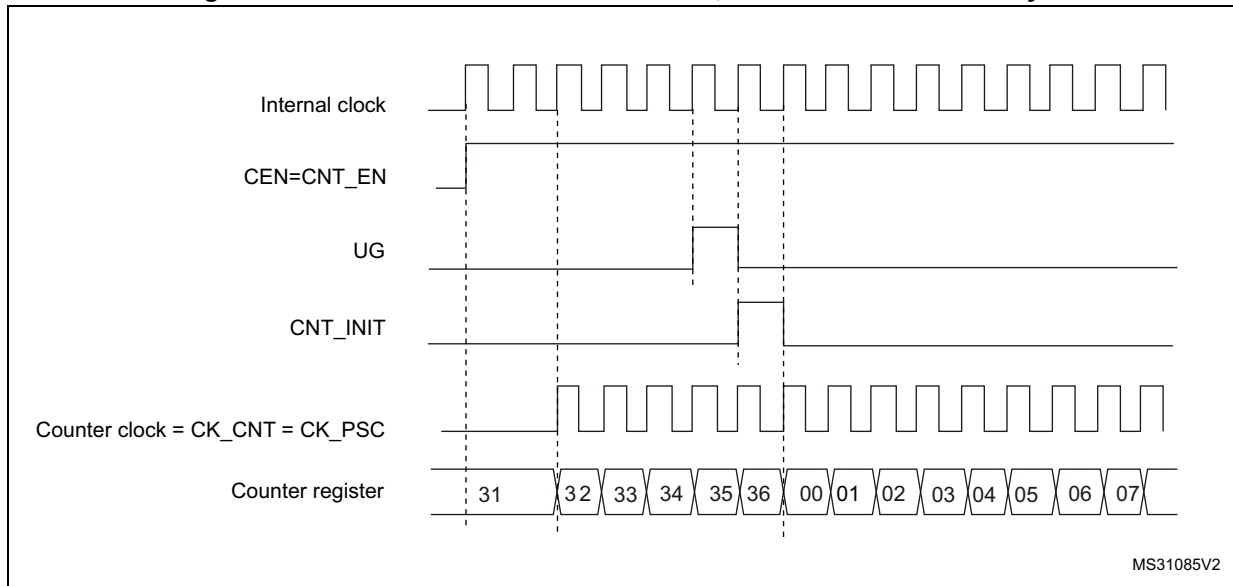
Figure 566. Control circuit in normal mode, internal clock divided by 1
