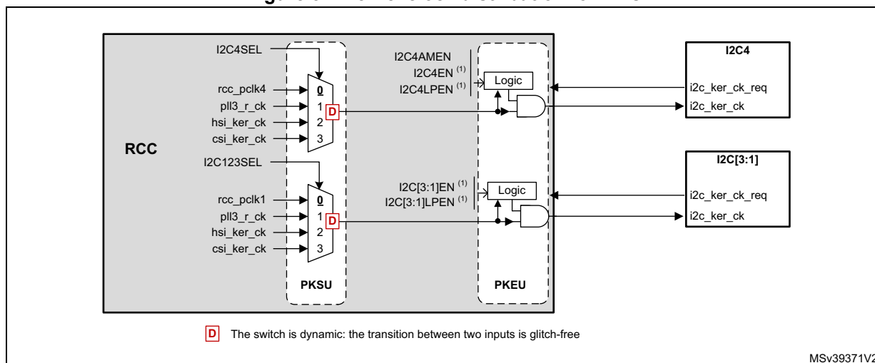
Figure 57. Kernel clock distribution for I2Cs
