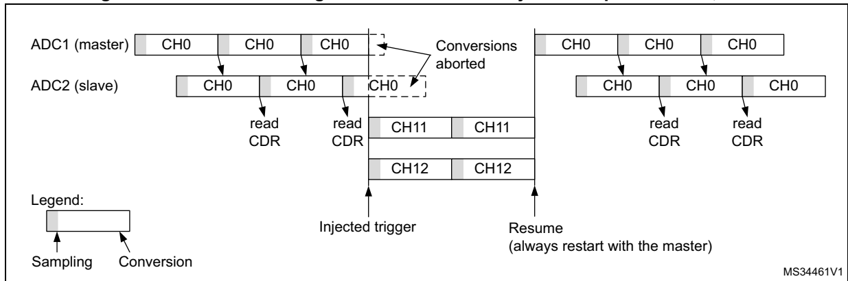
Figure 202. Two Interleaved channels (CH1, CH2) with injected sequence CH11, CH12 - case 1: Master interrupted first
