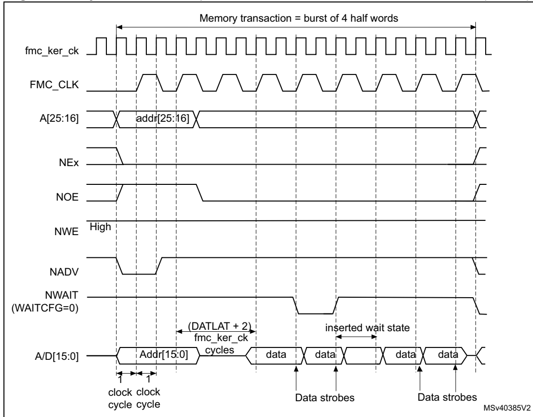
Figure 120. Synchronous multiplexed read mode waveforms - NOR, PSRAM (CRAM)
