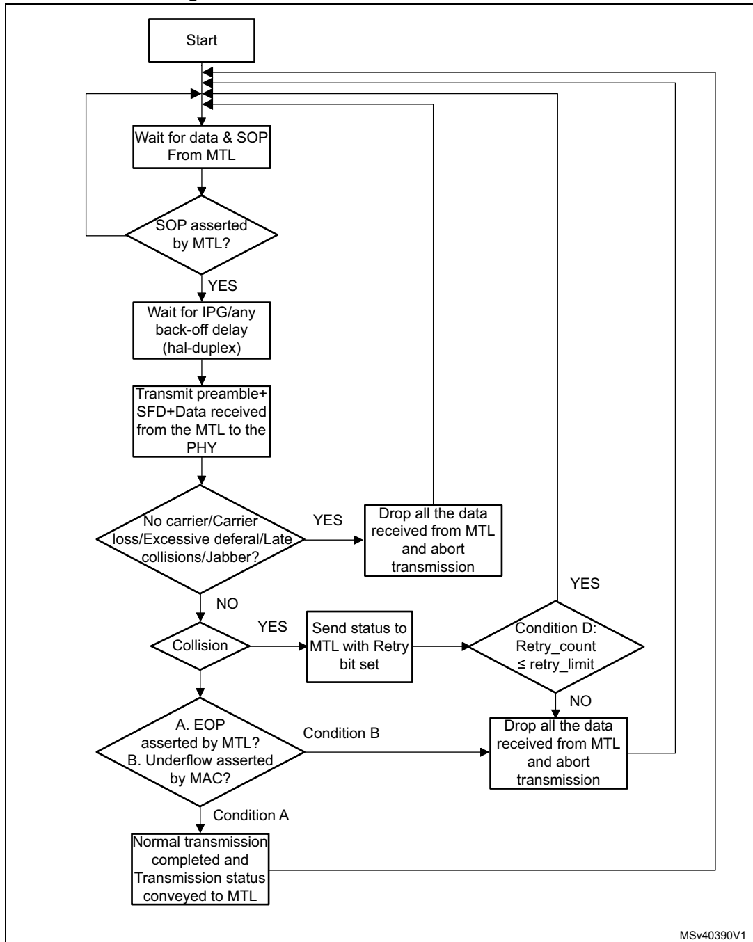
Figure 826. Overview of MAC transmission flow
