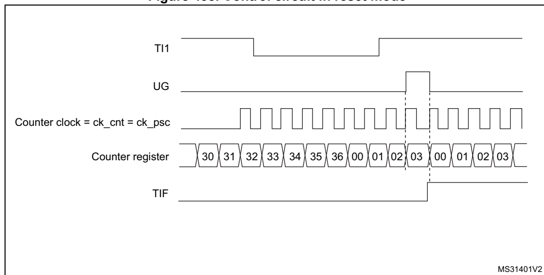
Figure 488. Control circuit in reset mode
