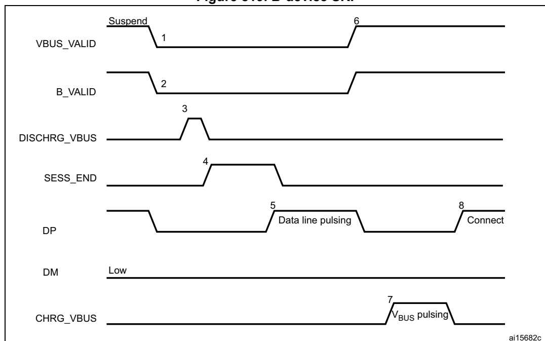
Figure 819. B-device SRP
