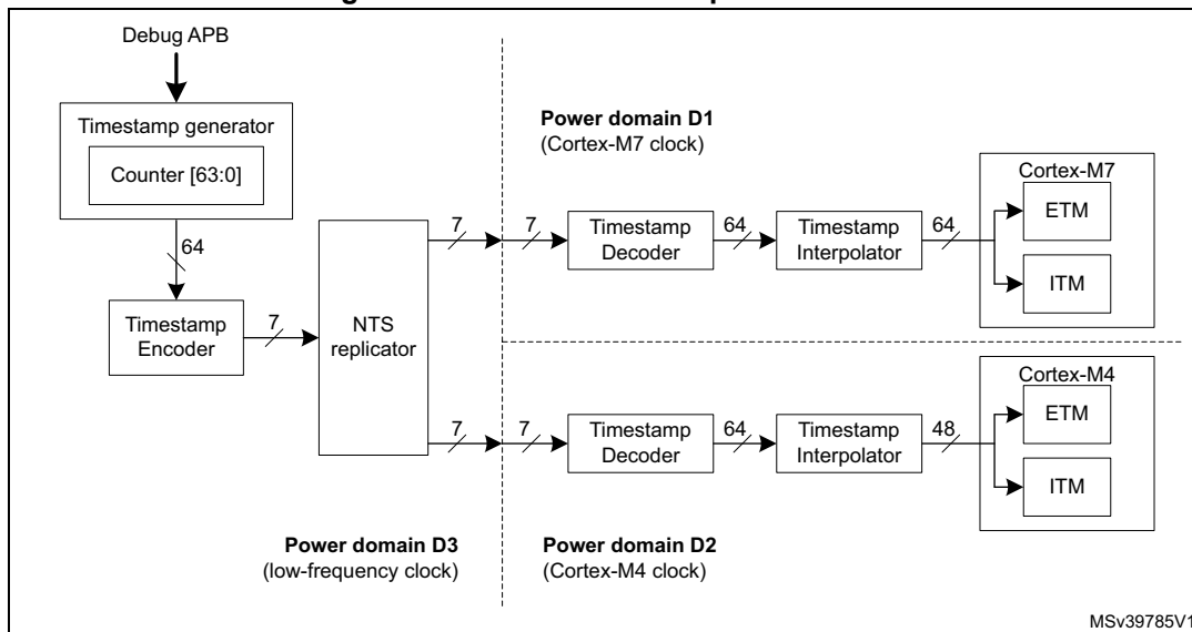
Figure 869. Global timestamp distribution
