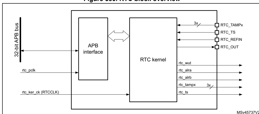
Figure 580. RTC block overview
