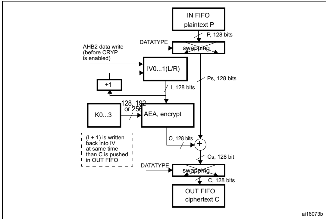
Figure 314. AES-CTR mode encryption
