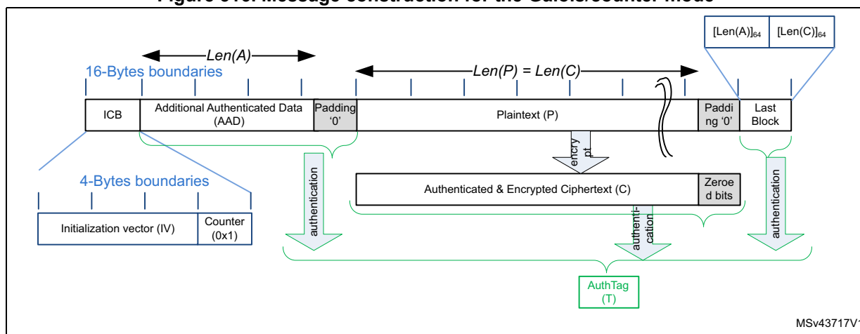
Figure 316. Message construction for the Galois/counter mode
