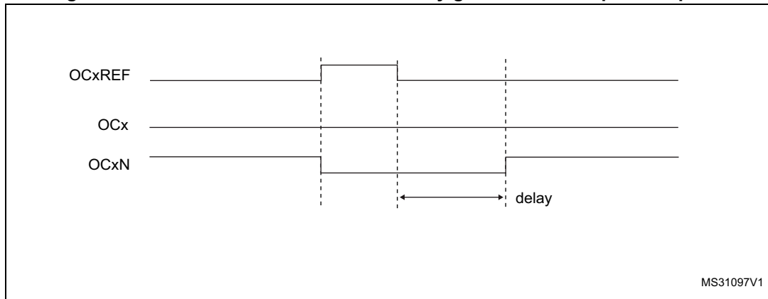
Figure 431. Dead-time waveforms with delay greater than the positive pulse
