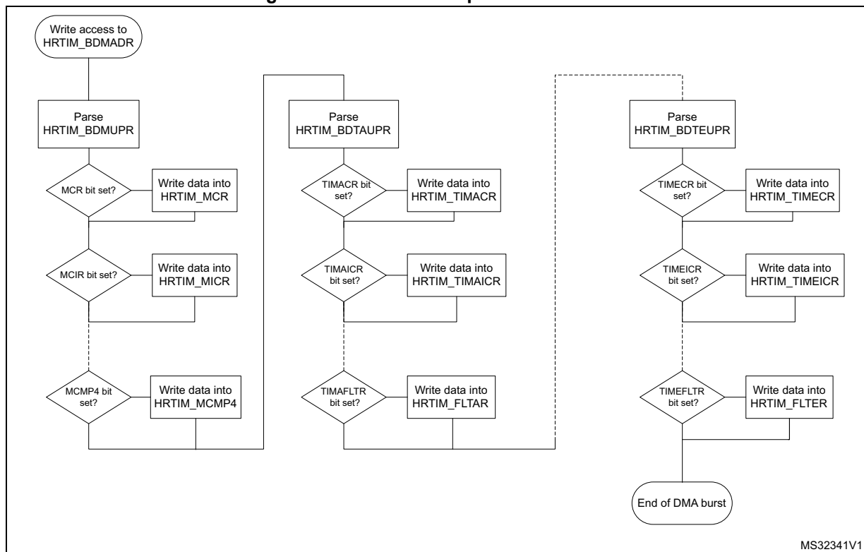
Figure 379. Burst DMA operation flowchart
