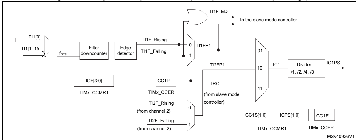
Figure 538. Capture/compare channel (example: channel 1 input stage)
