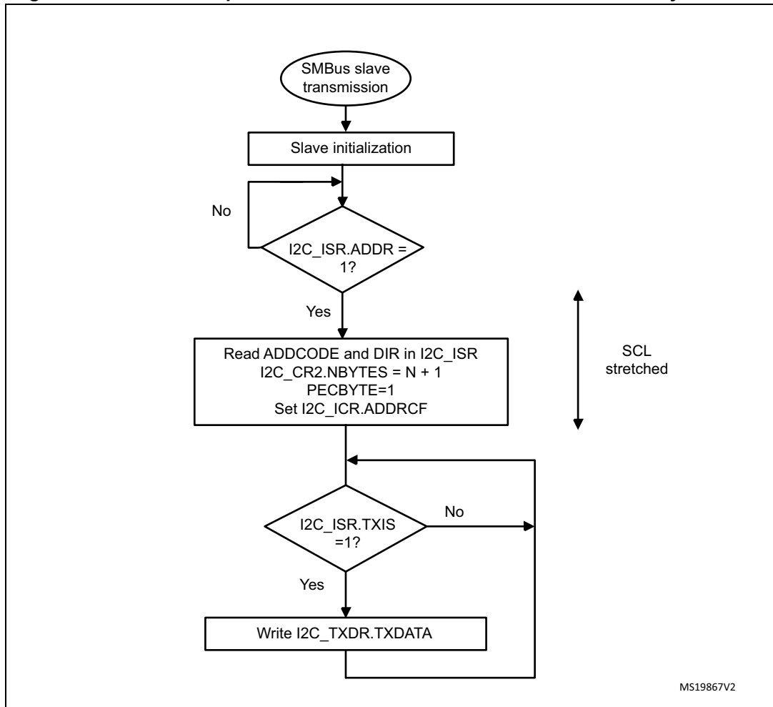
Figure 607. Transfer sequence flowchart for SMBus slave transmitter N bytes + PEC
