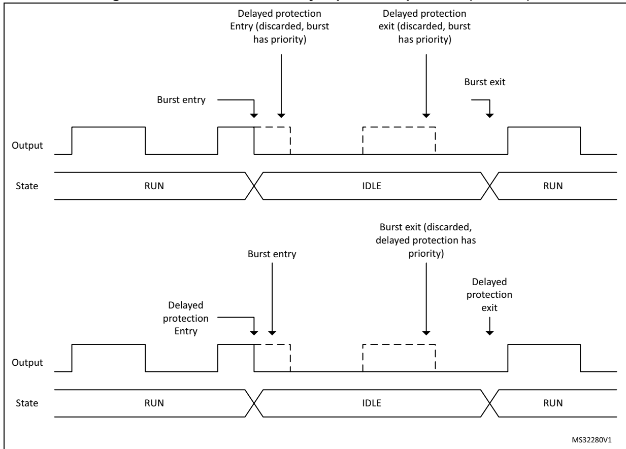
Figure 357. Burst mode and delayed protection priorities (DIDL = 0)
