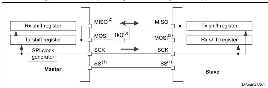
Figure 657. Half-duplex single master/ single slave application
