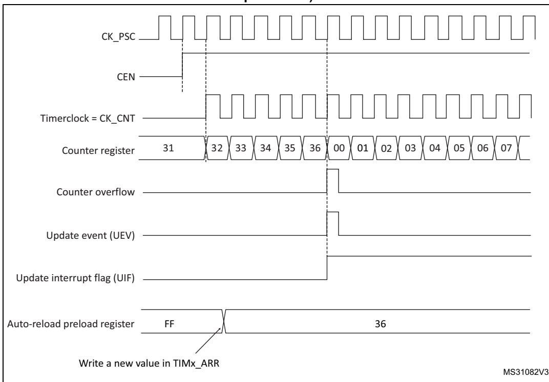
Figure 396. Counter timing diagram, update event when ARPE=0 (TIMx_ARR not preloaded)
