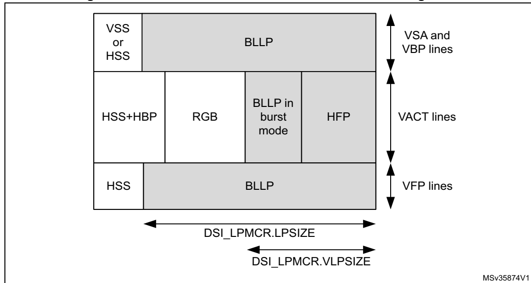
Figure 276. Location of LPSIZE and VLPSIZE in the image area
