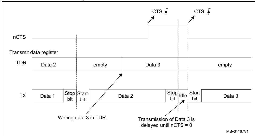
Figure 652. RS232 CTS flow control
