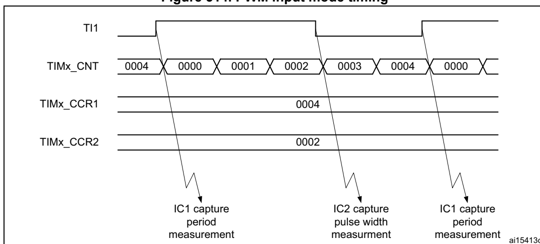
Figure 514. PWM input mode timing
