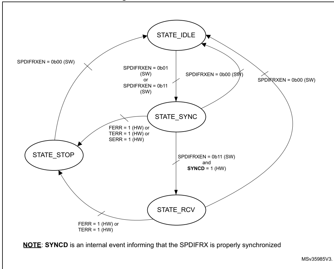
Figure 721. SPDIFRX States
