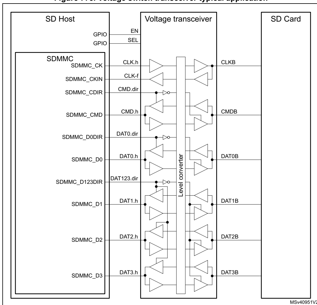
Figure 775. Voltage switch transceiver typical application
