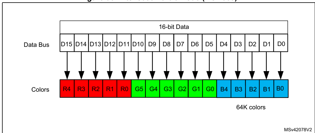
Figure 93. Intel 8080 16-bit mode (RGB565)
