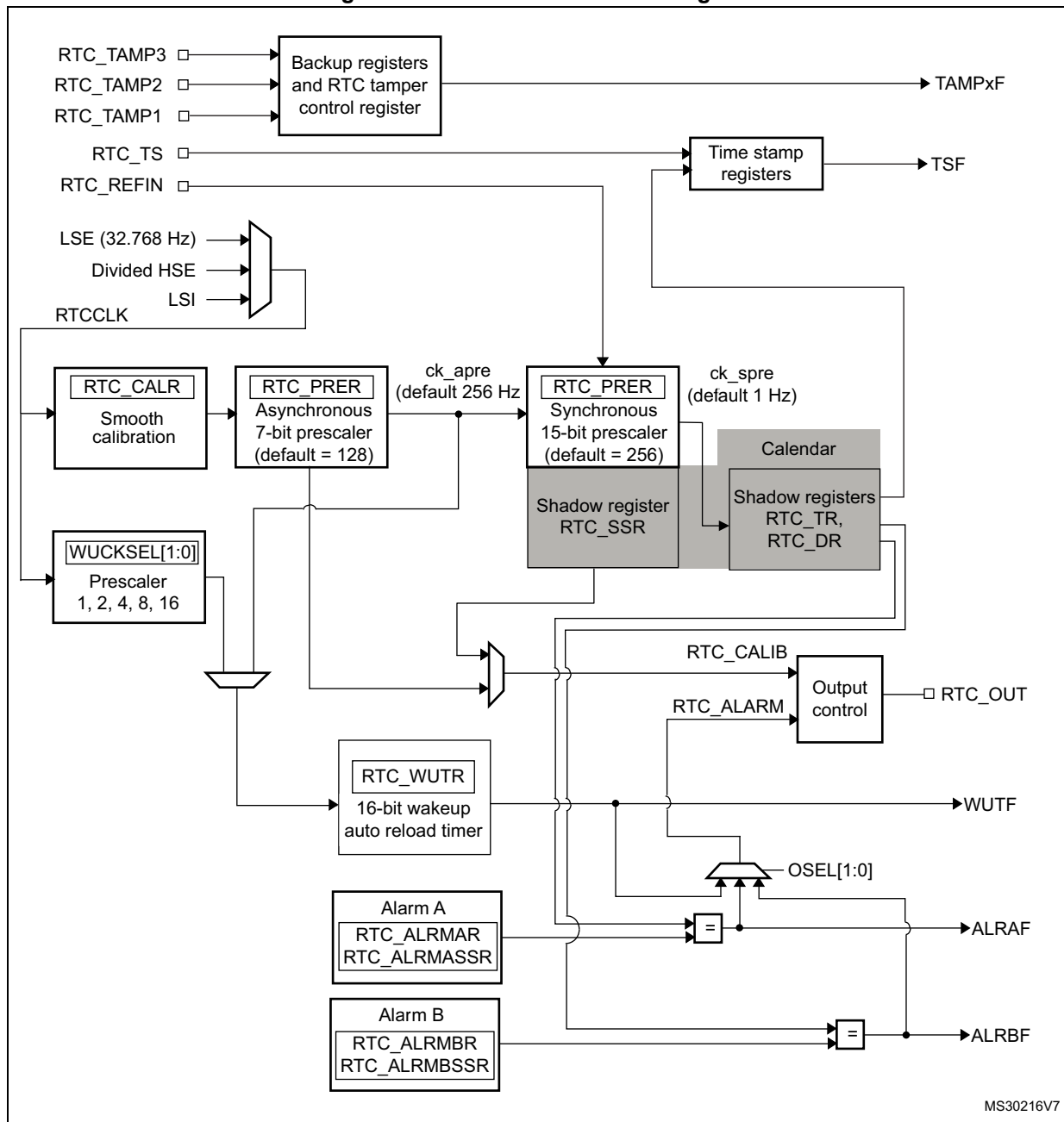
Figure 581. Detailed RTC block diagram
