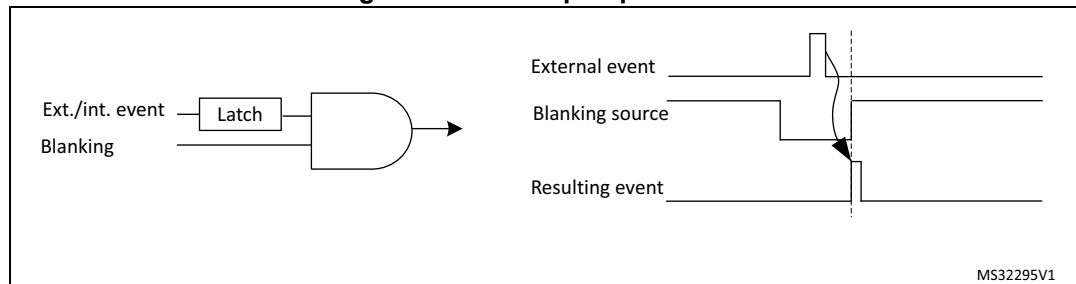
Figure 350. Event postpone mode
