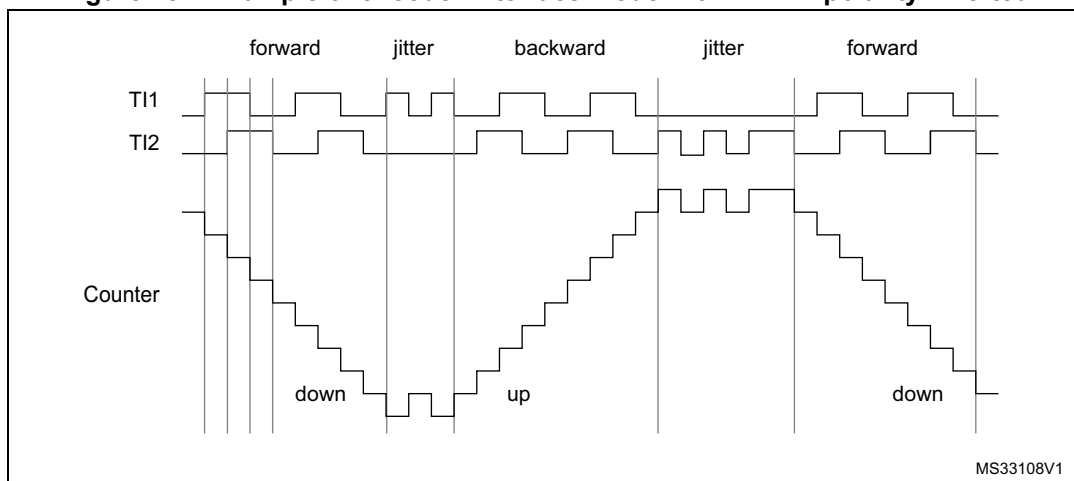
Figure 487. Example of encoder interface mode with TI1FP1 polarity inverted
