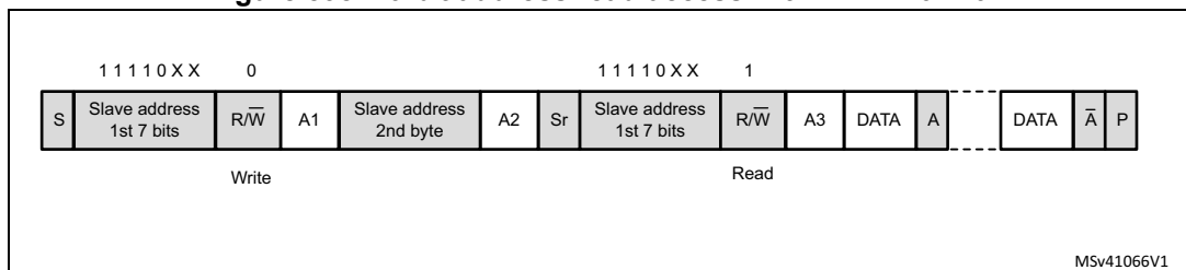
Figure 598. 10-bit address read access with HEAD10R=0
