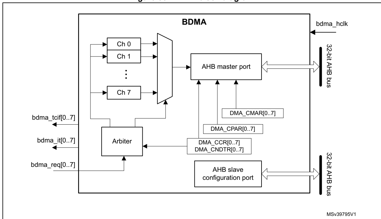
Figure 88. BDMA block diagram
