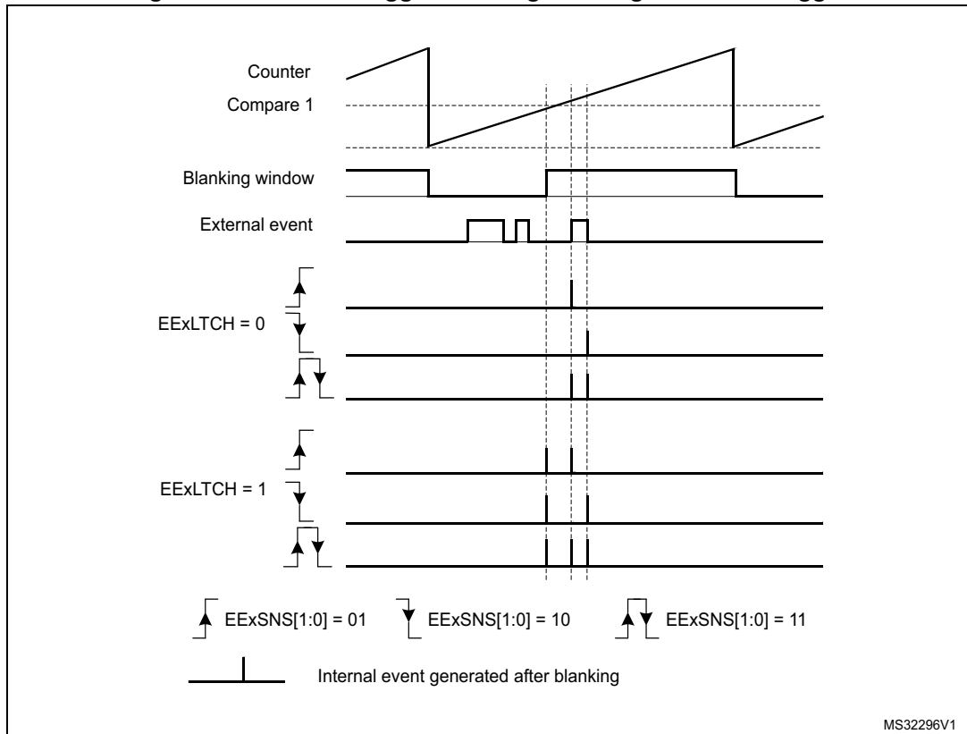
Figure 351. External trigger blanking with edge-sensitive trigger
