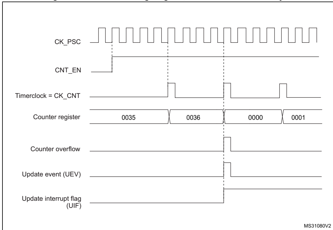
Figure 531. Counter timing diagram, internal clock divided by N
