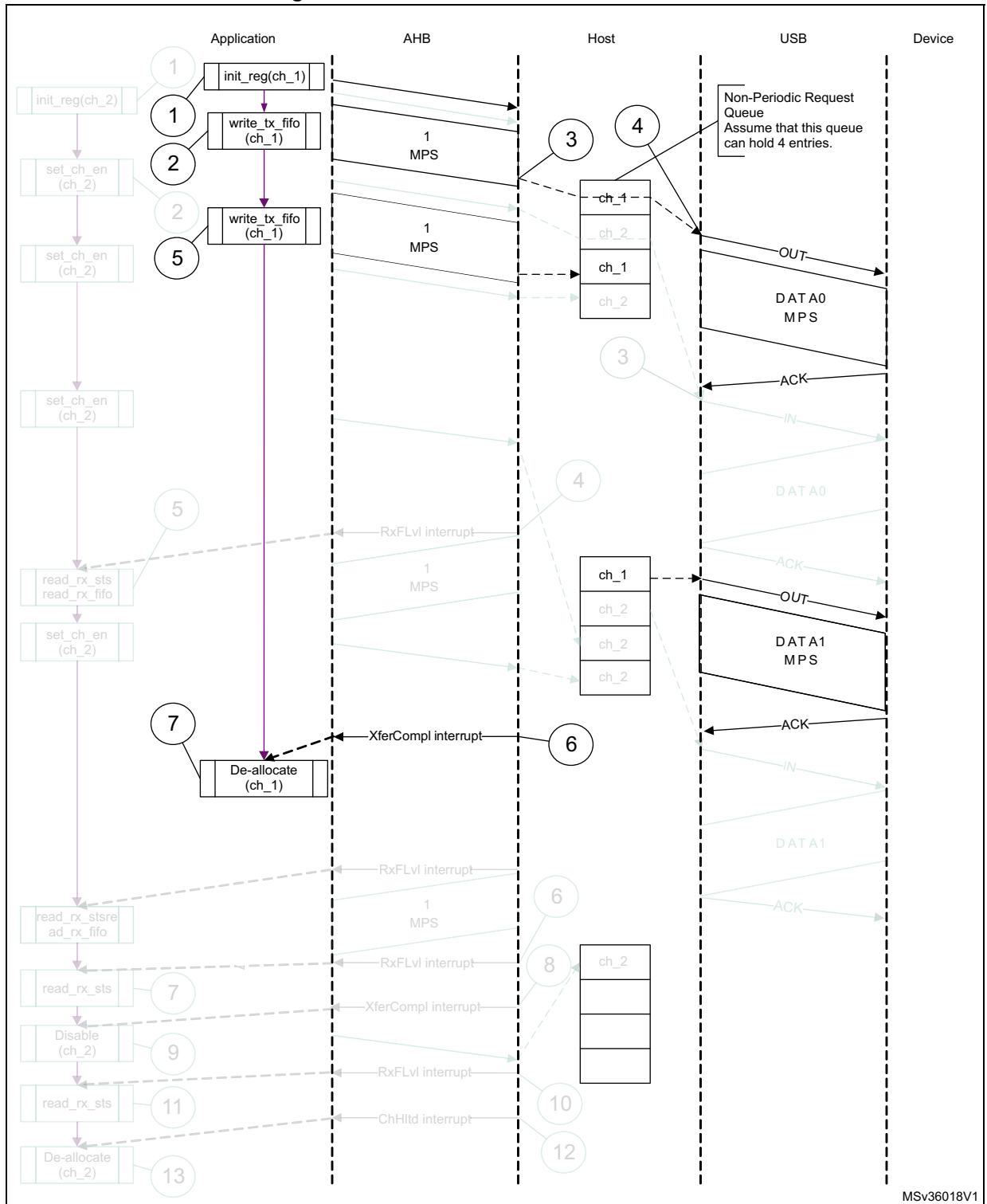
Figure 802. Normal bulk/control OUT/SETUP
