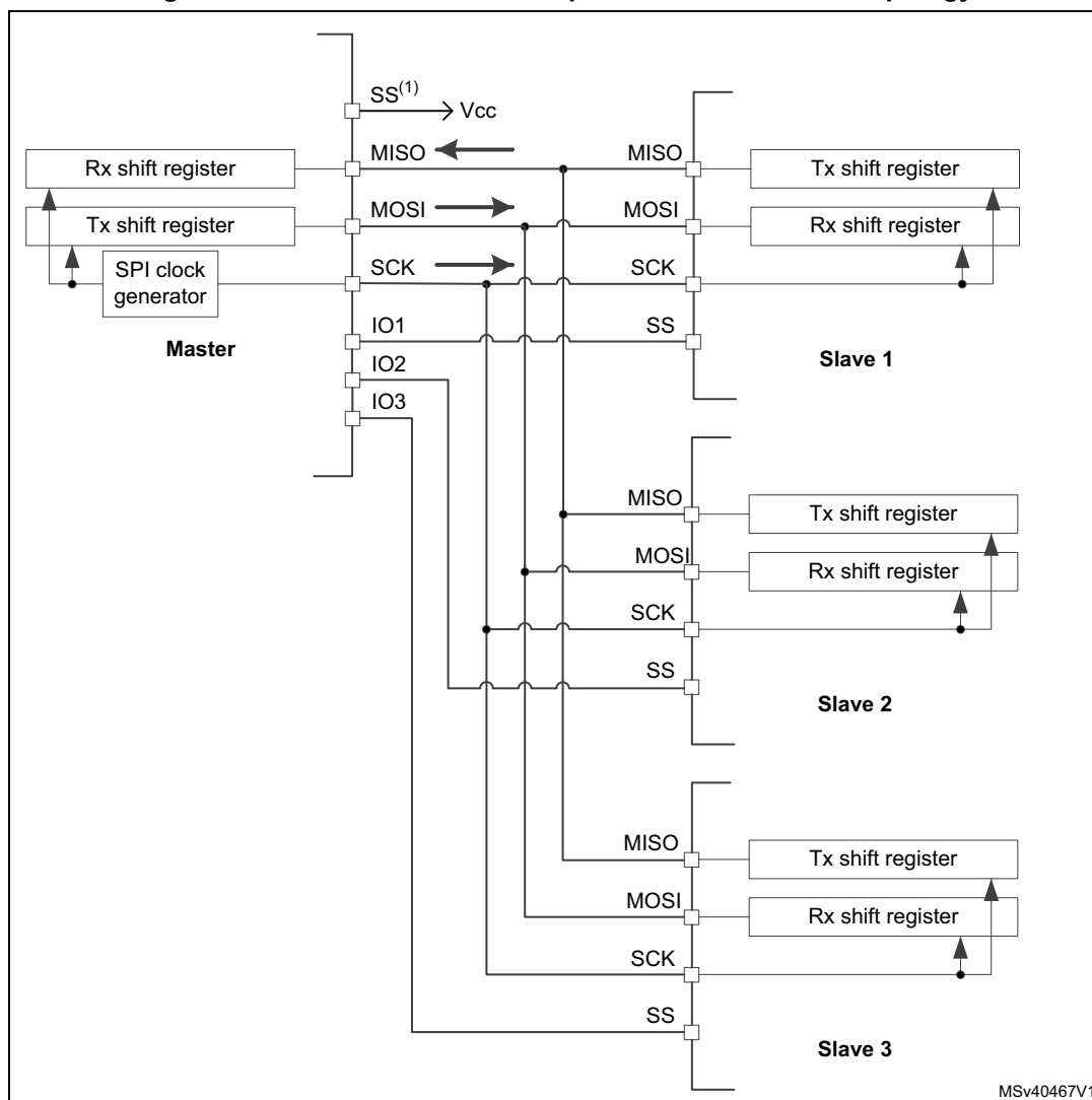
Figure 659. Master and three independent slaves at star topology
