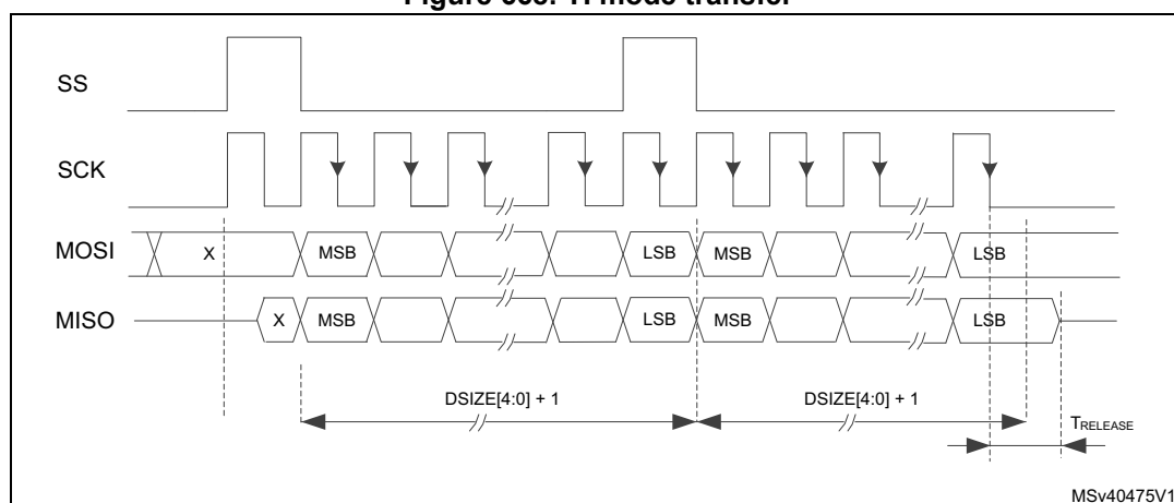
Figure 668. TI mode transfer
