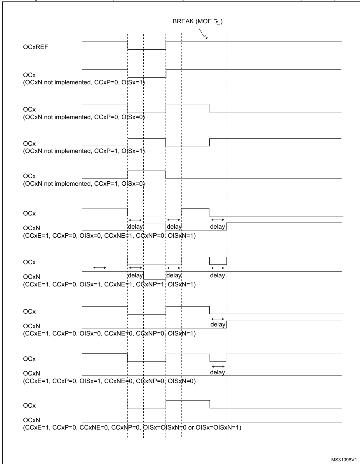
Figure 433. Various output behavior in response to a break event on BRK (OSS1 = 1)
