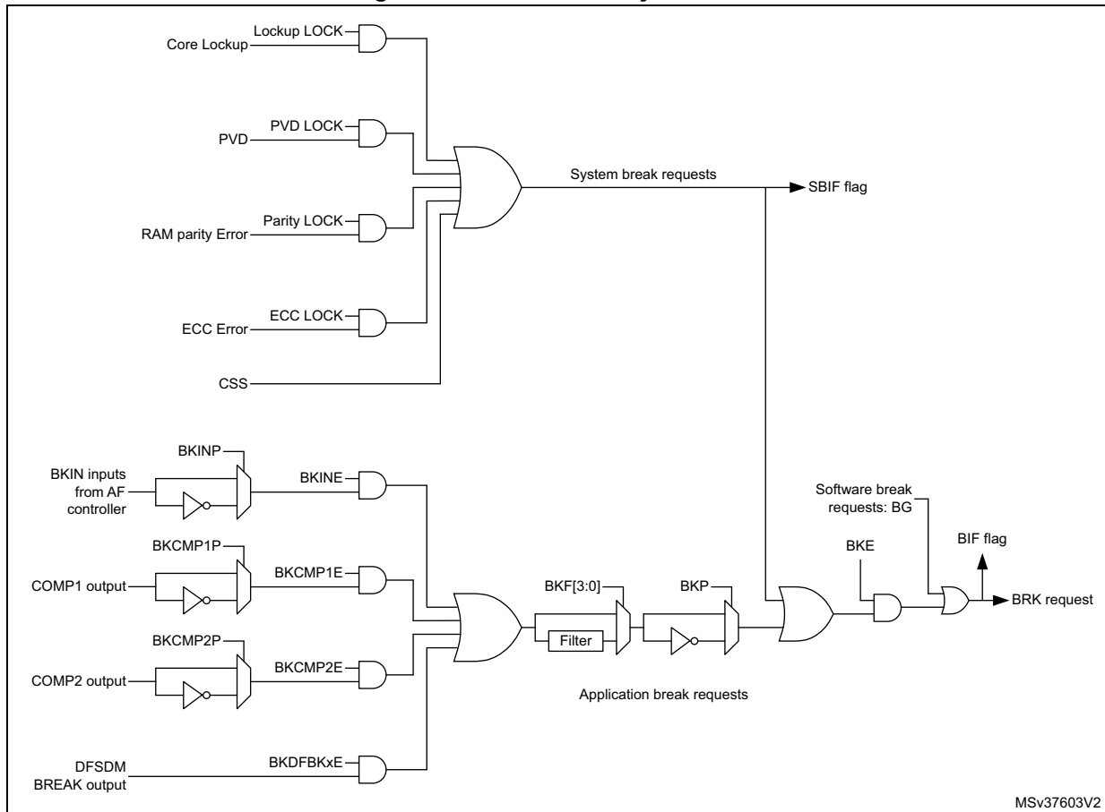
Figure 549. Break circuitry overview
