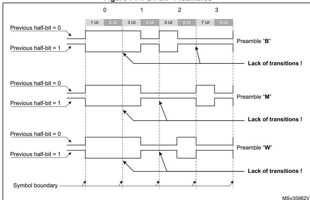
Figure 714. S/PDIF Preambles
