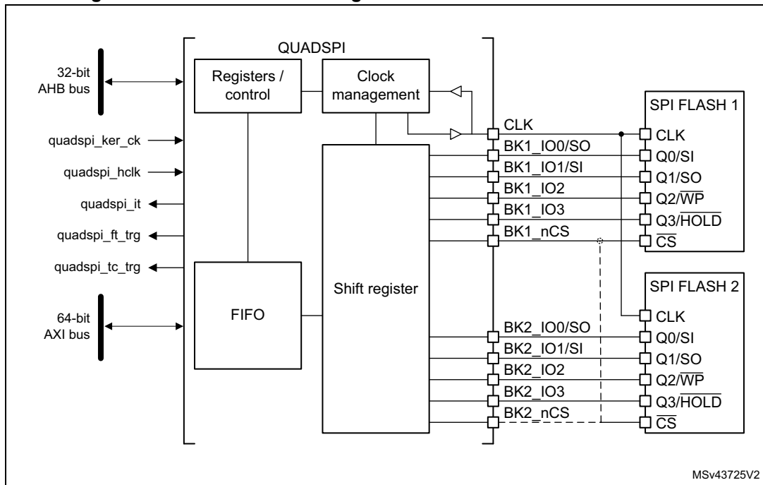
Figure 132. QUADSPI block diagram when dual-flash mode is enabled
