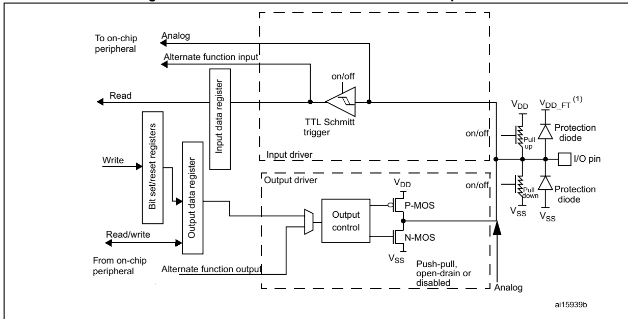
Figure 76. Basic structure of a 5-Volt tolerant I/O port bit
