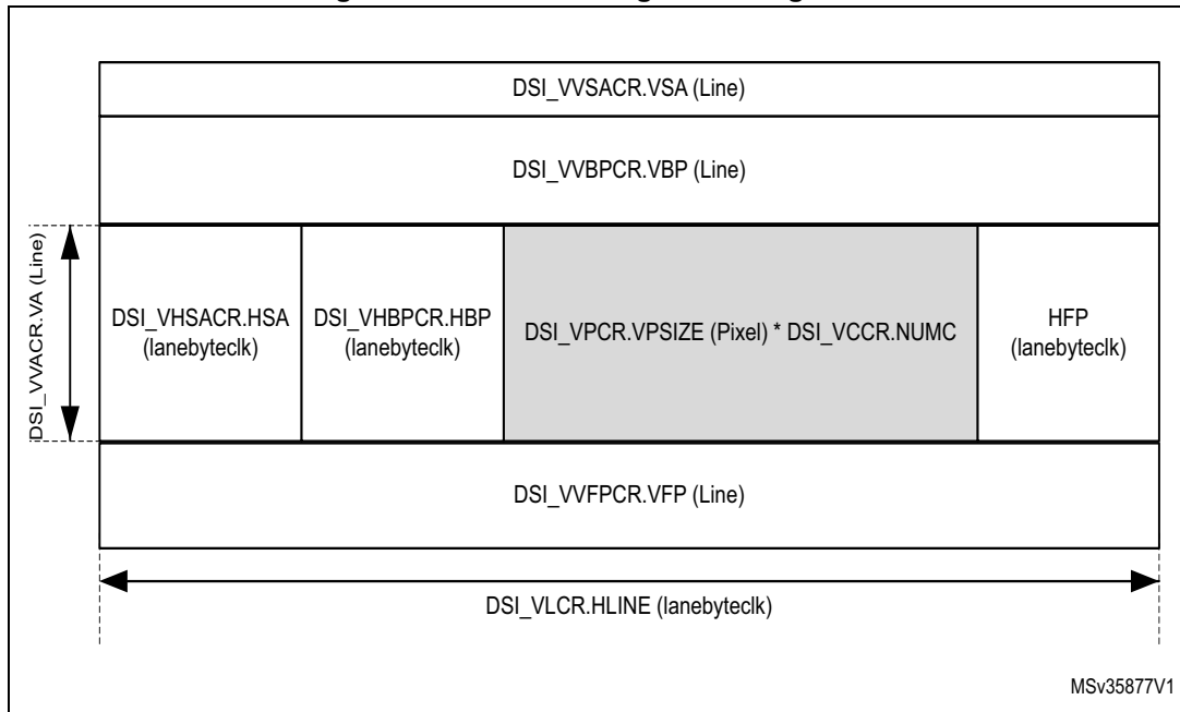
Figure 290. Frame configuration registers
