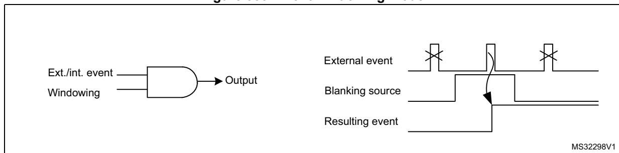
Figure 353. Event windowing mode
