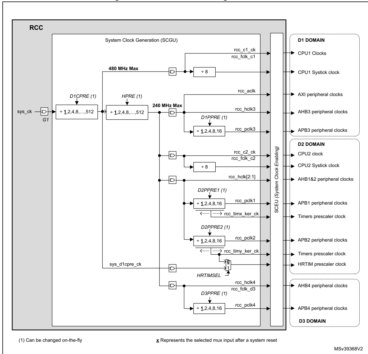
Figure 54. Core and bus clock generation
