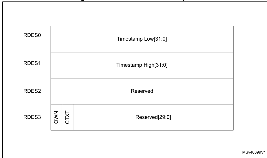
Figure 850. Receive context descriptor
