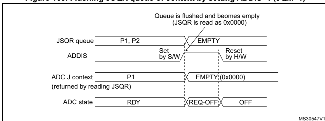
Figure 165. Flushing JSQR queue of context by setting ADDIS=1 (JQM=1)
