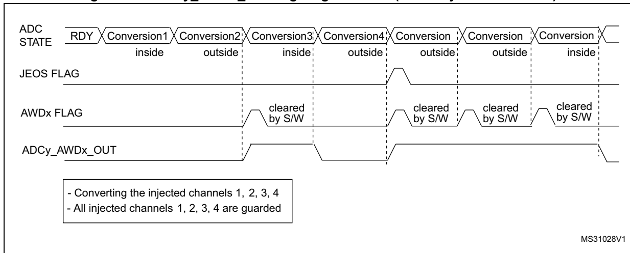
Figure 184. ADCy_AWDx_OUT signal generation (on all injected channels)
