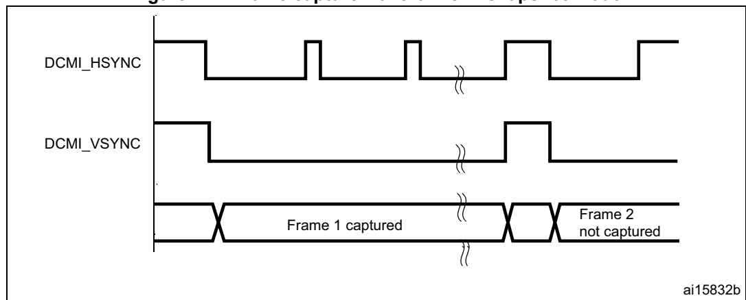
Figure 244. Frame capture waveforms in snapshot mode
