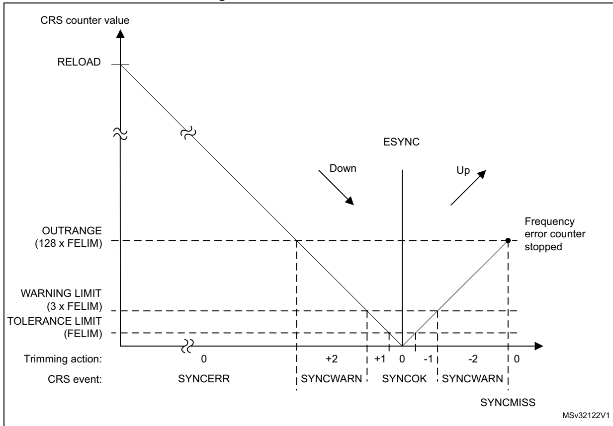
Figure 71. CRS counter behavior
