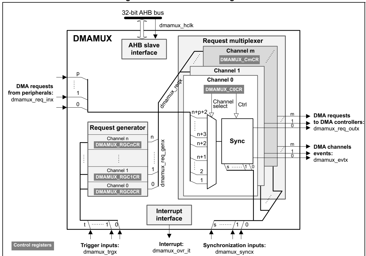
Figure 89. DMAMUX block diagram
