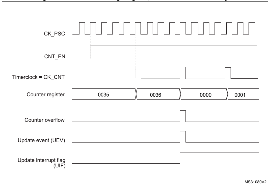
Figure 562. Counter timing diagram, internal clock divided by 4
