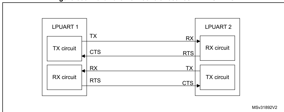
Figure 650. Hardware flow control between 2 LPUARTs
