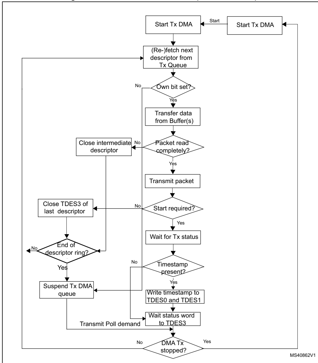
Figure 823. DMA transmission flow (standard mode)
