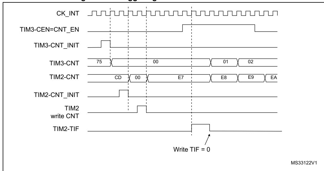
Figure 496. Triggering TIM2 with Enable of TIM3
