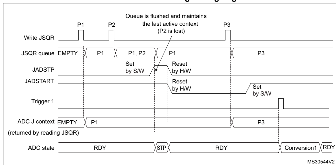
Figure 160. Flushing JSQR queue of context by setting JADSTP=1 (JQM=0). Case when JADSTP occurs during an ongoing conversion.
