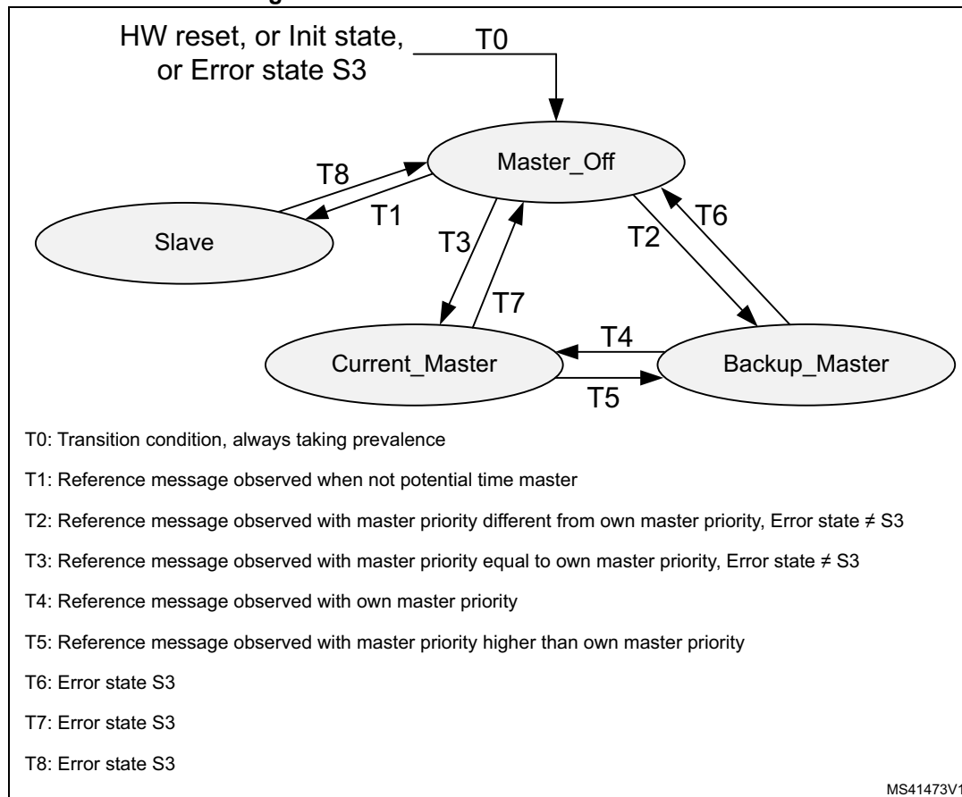
Figure 792. Level 0 master to slave relation
