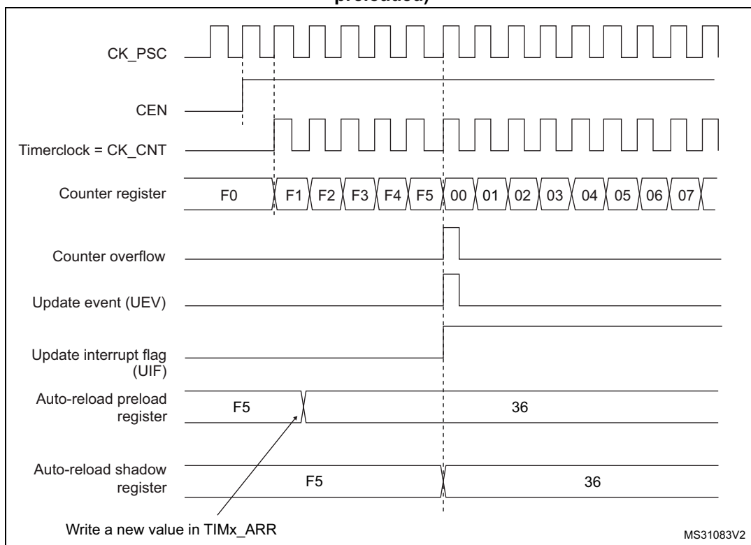
Figure 565. Counter timing diagram, update event when ARPE=1 (TIMx_ARR preloaded)
