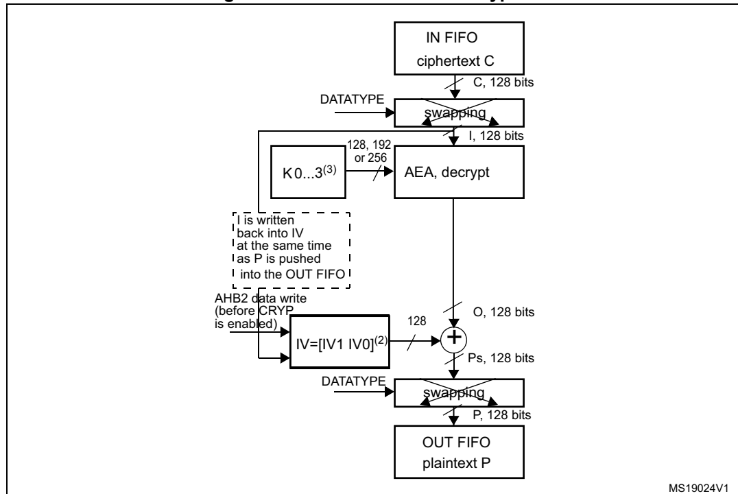
Figure 312. AES-CBC mode decryption
