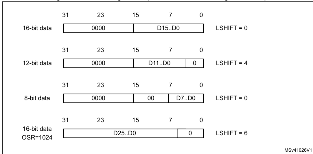
Figure 173. Left alignment (offset enabled, signed value)
