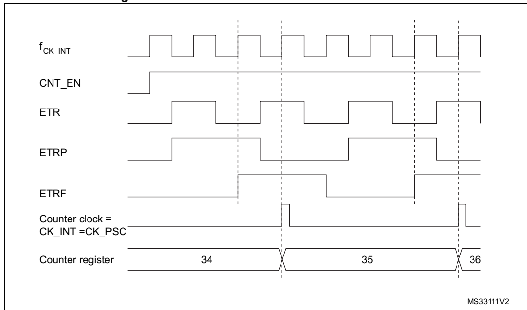
Figure 416. Control circuit in external clock mode 2
