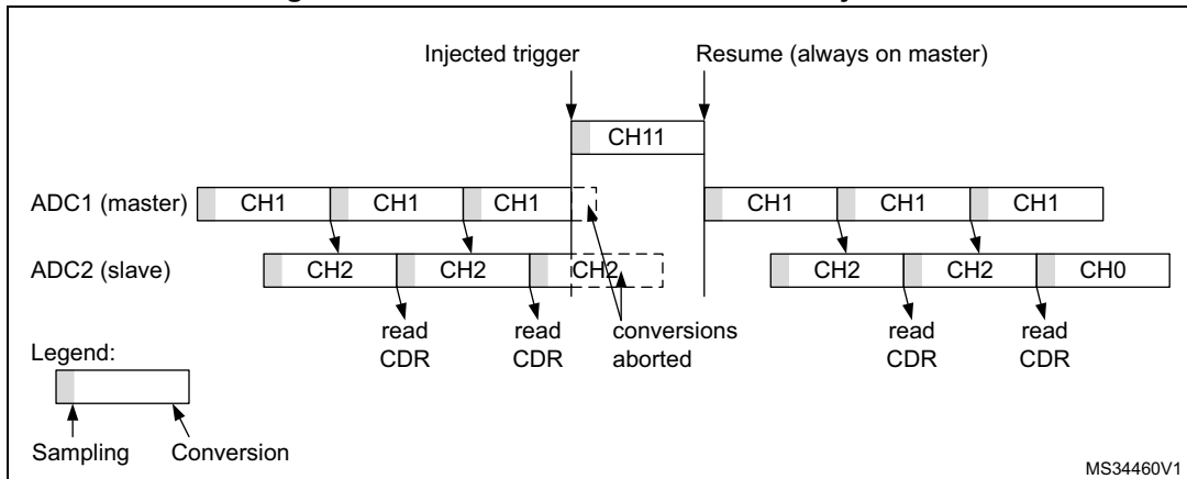
Figure 196. Interleaved conversion with injection
