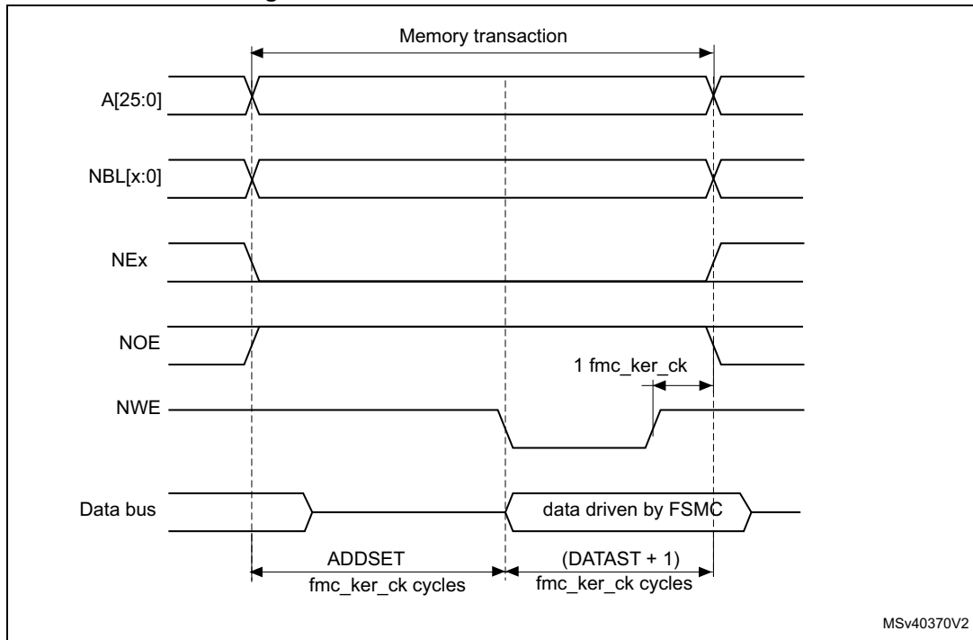
Figure 105. Mode 1 write access waveforms
