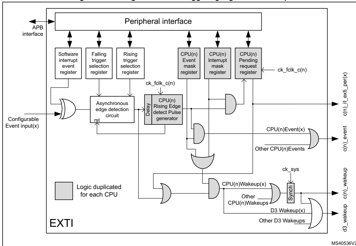
Figure 96. Configurable event triggering logic CPU wakeup
