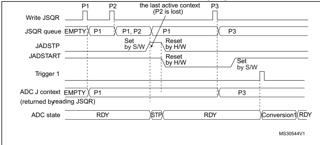
Figure 162. Flushing JSQR queue of context by setting JADSTP=1 (JQM=0). Case when JADSTP occurs outside an ongoing conversion
