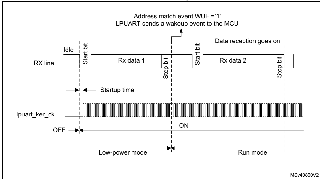
Figure 653. Wakeup event verified (wakeup event = address match, FIFO disabled)
