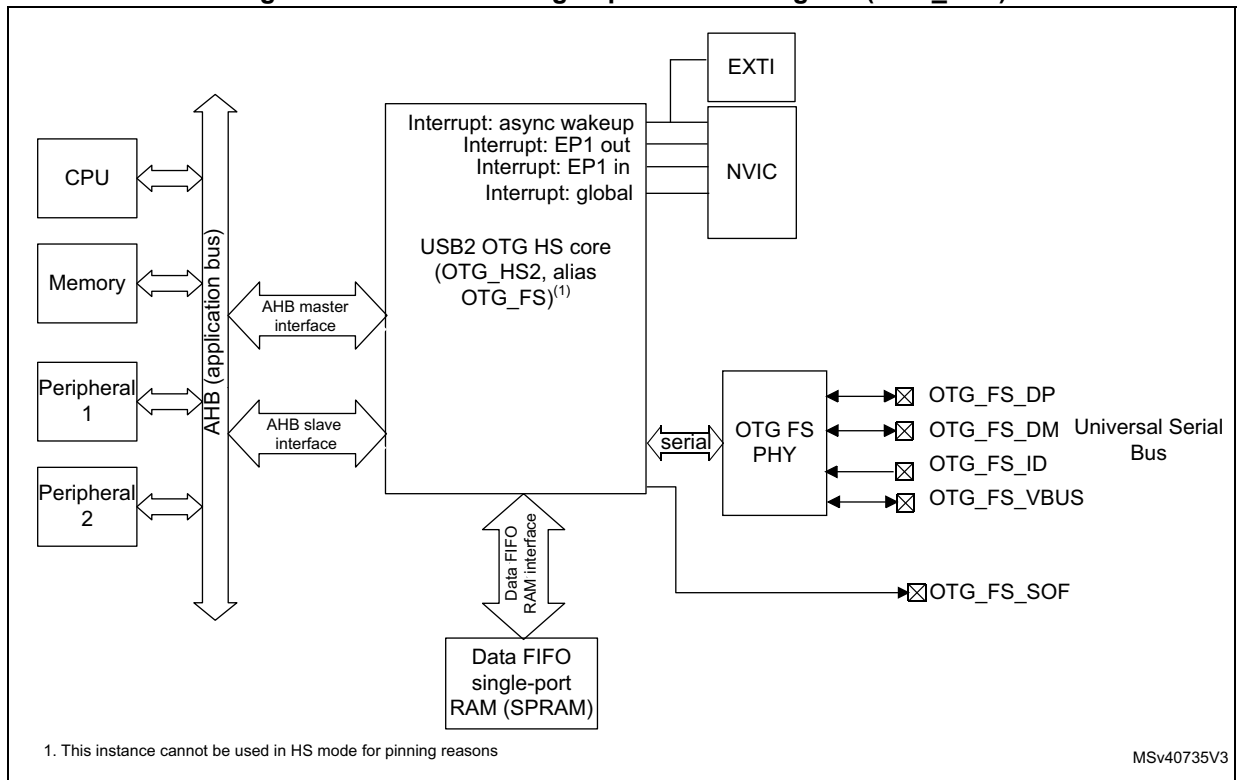
Figure 794. USB2 OTG high-speed block diagram (OTG_HS2)
