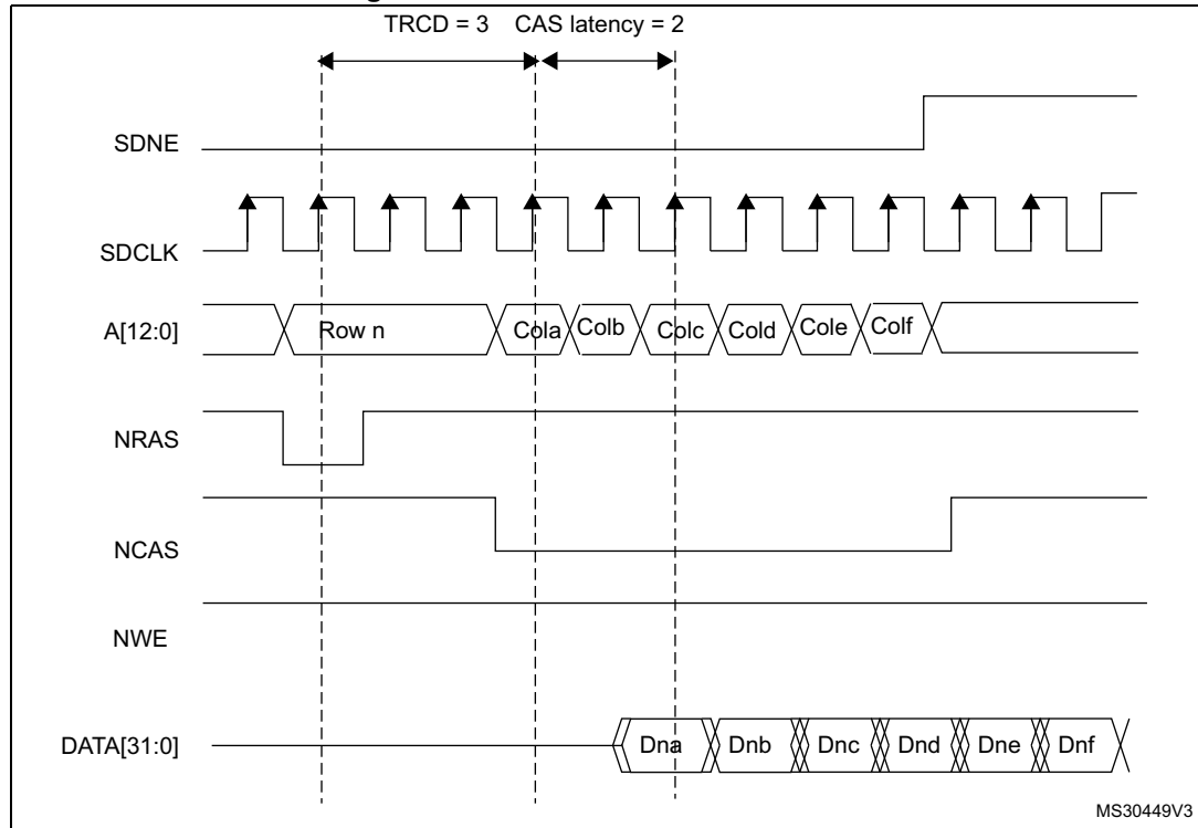
Figure 125. Burst read SDRAM access
