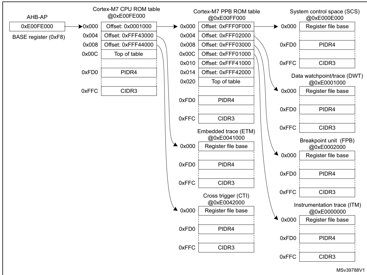
Figure 874. Cortex-M7 CoreSight Topology
