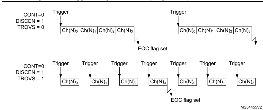
Figure 186. Triggered regular oversampling mode (TROVS bit = 1)
