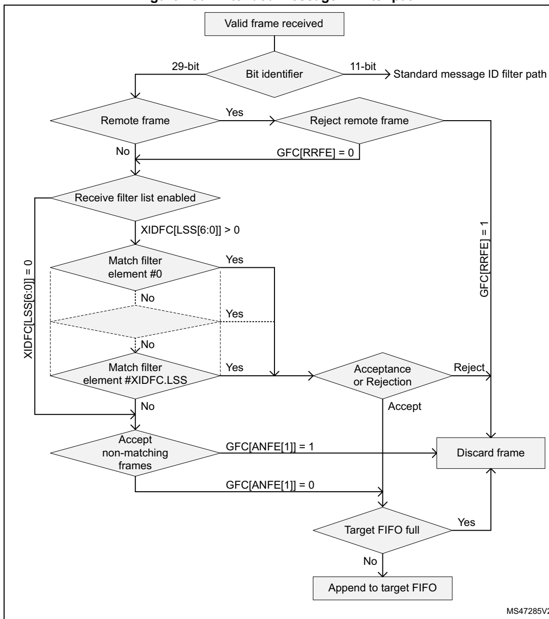
Figure 783. Extended message ID filter path
