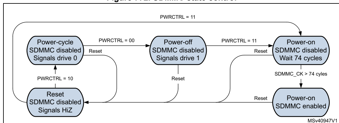
Figure 772. SDMMC state control
