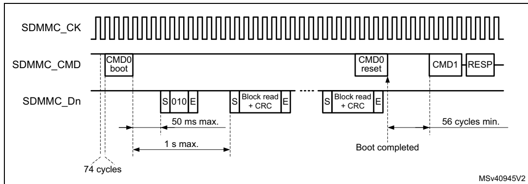
Figure 770. Alternative boot mode operation
