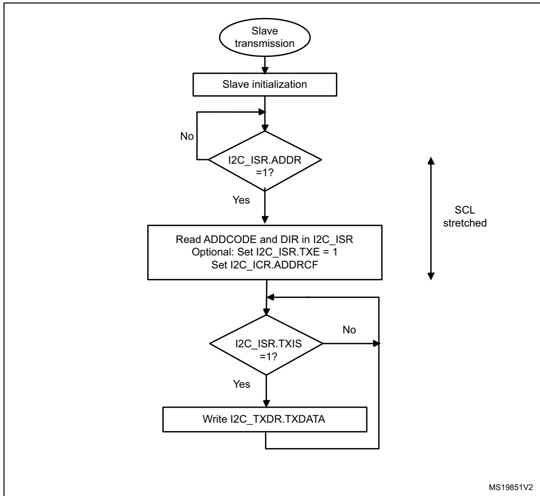
Figure 590. Transfer sequence flowchart for I2C slave transmitter, NOSTRETCH= 0
