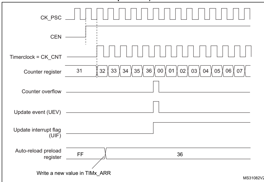
Figure 532. Counter timing diagram, update event when ARPE=0 (TIMx_ARR not preloaded)
