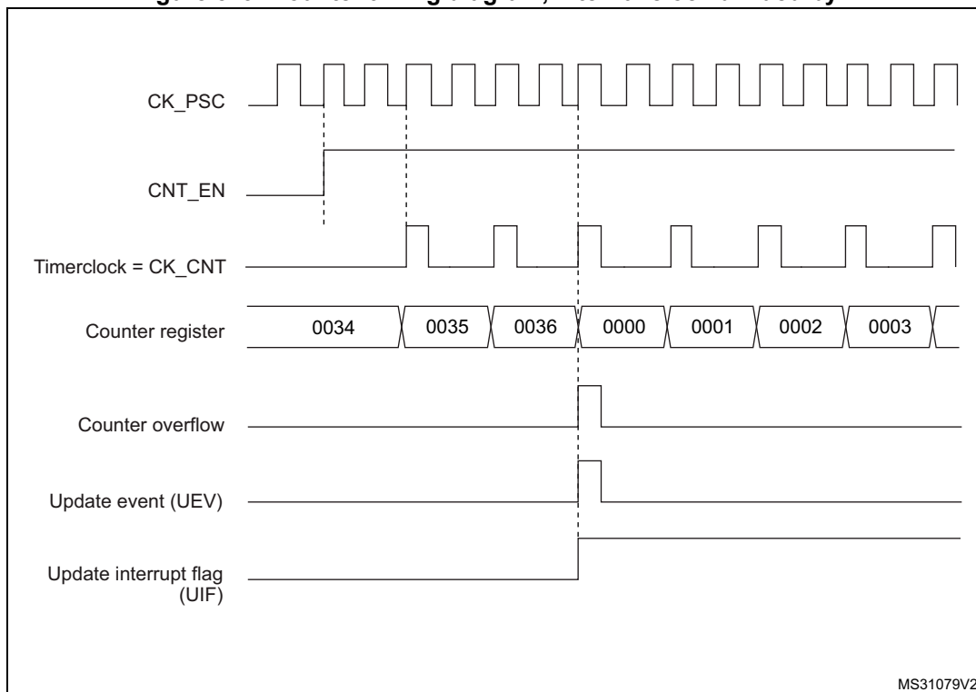
Figure 529. Counter timing diagram, internal clock divided by 2
