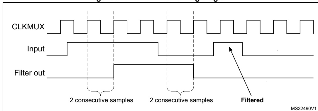
Figure 570. Glitch filter timing diagram
