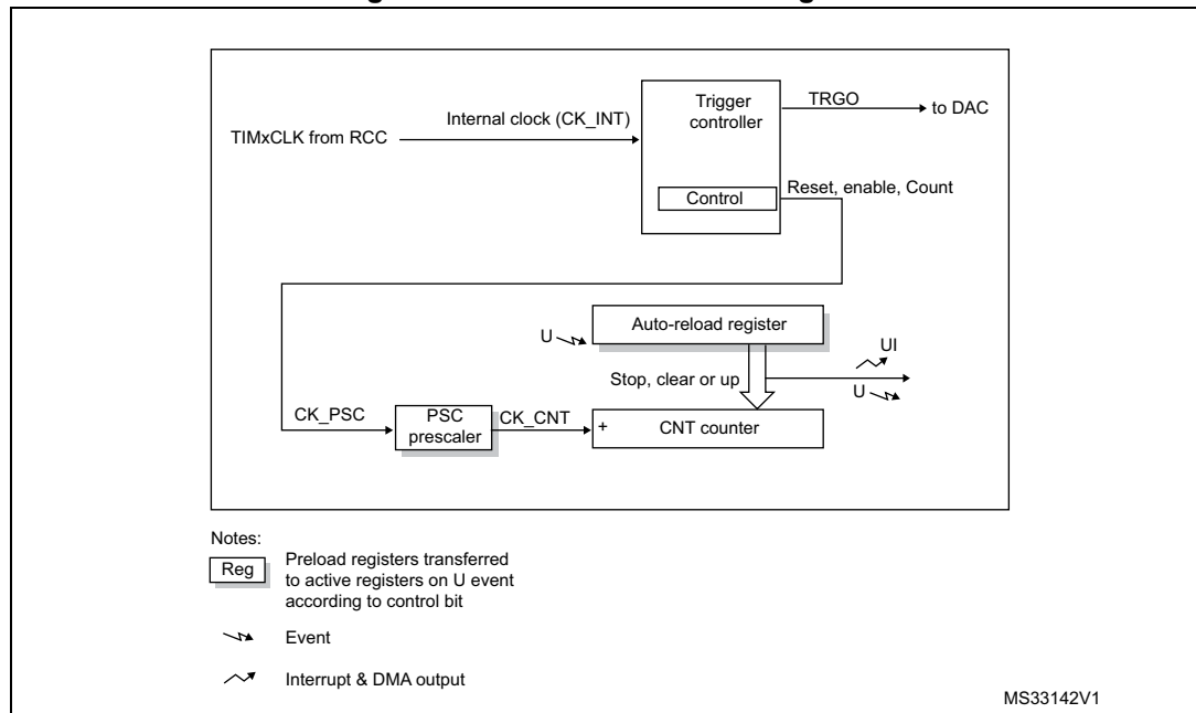
Figure 557. Basic timer block diagram
