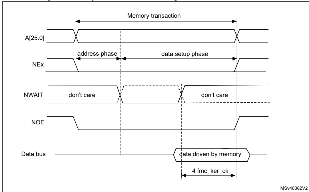
Figure 117. Asynchronous wait during a read access waveforms
