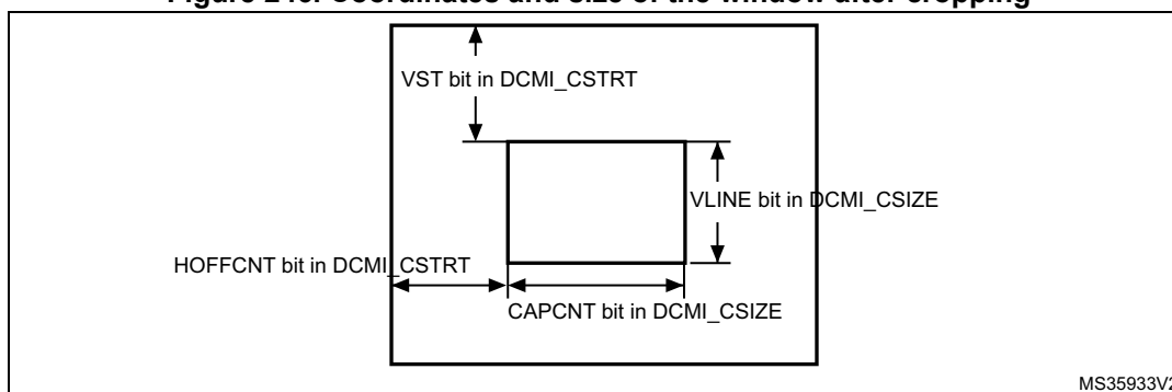
Figure 246. Coordinates and size of the window after cropping
