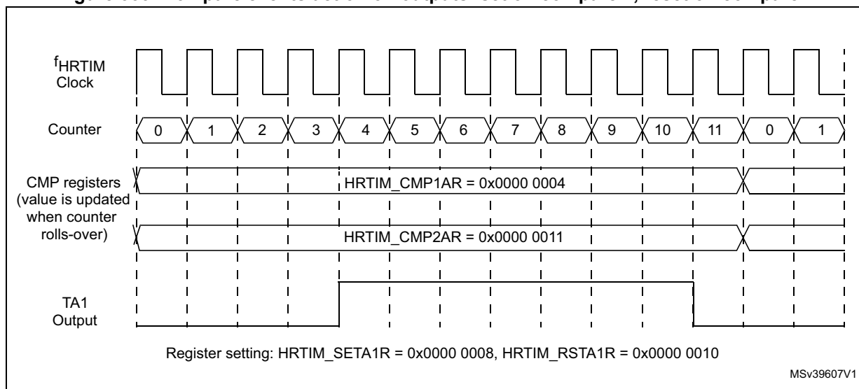
Figure 333. Compare events action on outputs: set on compare 1, reset on compare 2
