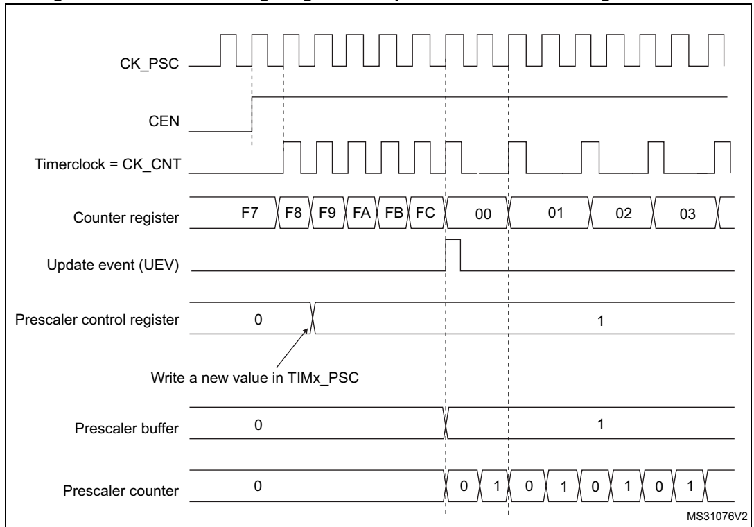
Figure 526. Counter timing diagram with prescaler division change from 1 to 2
