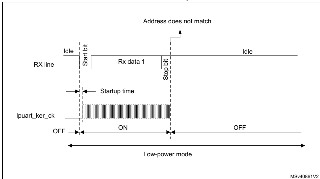
Figure 654. Wakeup event not verified (wakeup event = address match, FIFO disabled)
