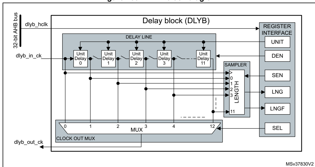
Figure 139. DLYB block diagram
