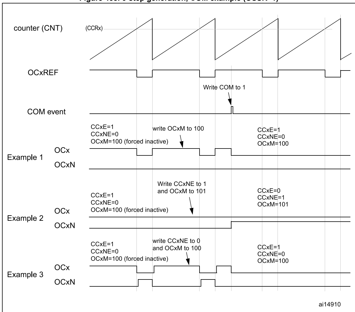
Figure 438. 6-step generation, COM example (OSSR=1)
