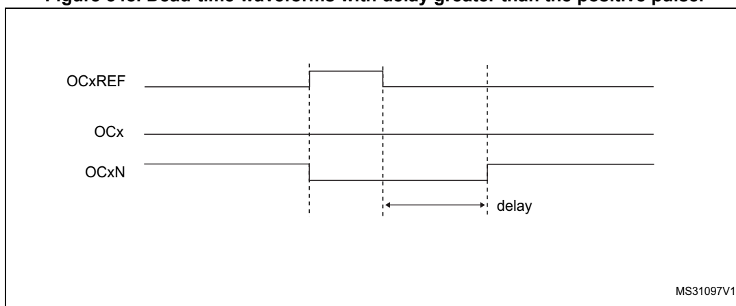
Figure 548. Dead-time waveforms with delay greater than the positive pulse.
