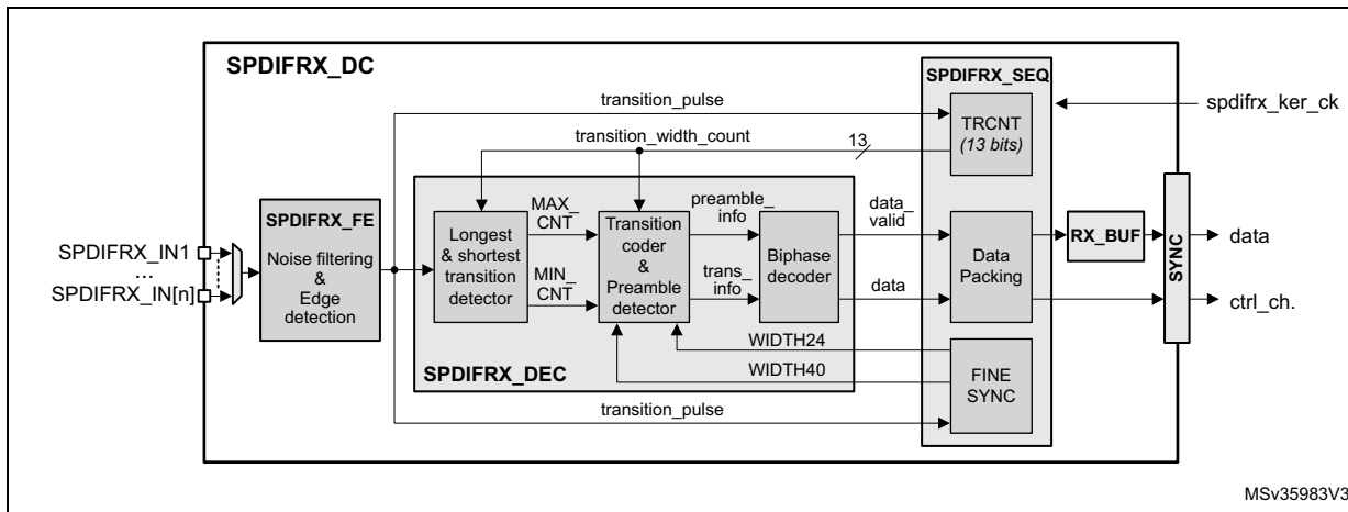
Figure 716. SPDIFRX decoder
