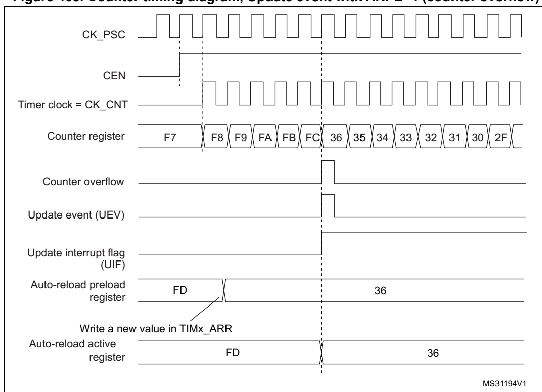
Figure 408. Counter timing diagram, Update event with ARPE=1 (counter overflow)
