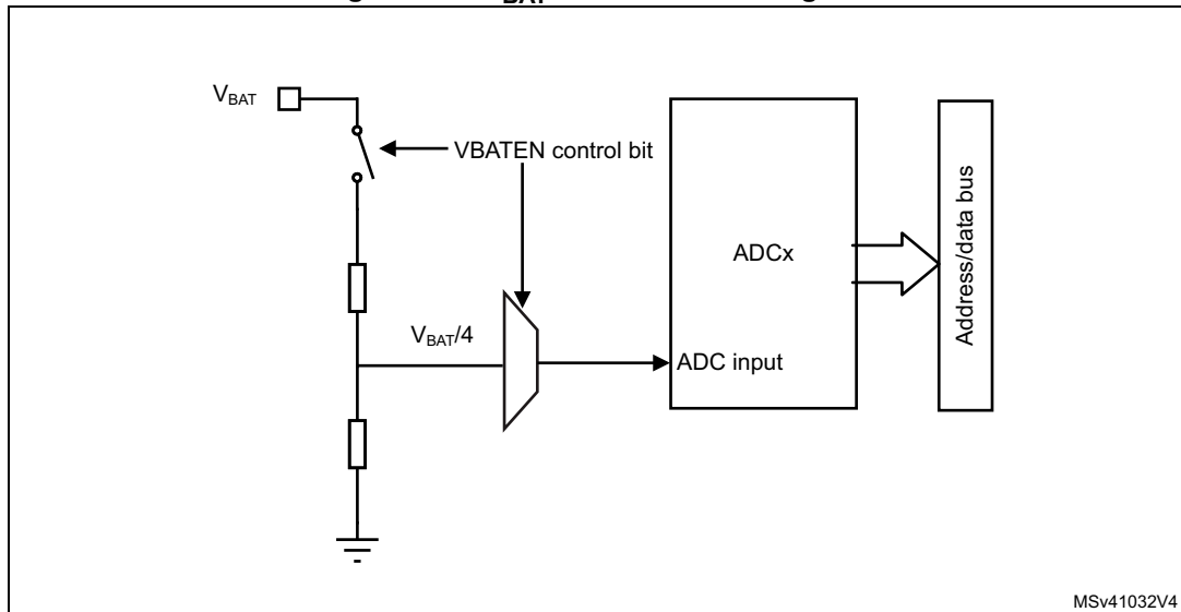
Figure 208. V_{BAT} channel block diagram
