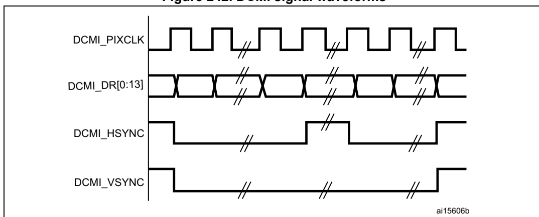
Figure 242. DCMI signal waveforms
