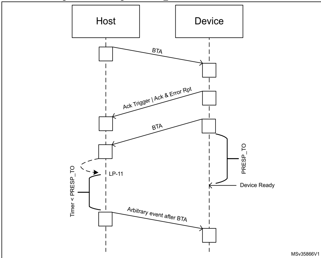
Figure 265. Timing of PRESP_TO after a bus-turn-around
