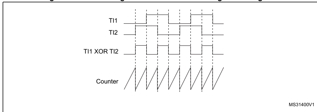
Figure 520. Measuring time interval between edges on 2 signals
