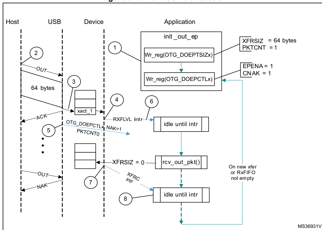
Figure 816. Bulk OUT transaction
