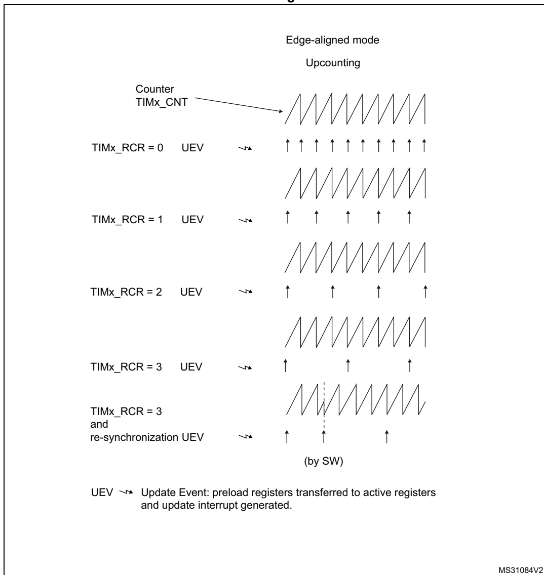
Figure 534. Update rate examples depending on mode and TIMx_RCR register settings
