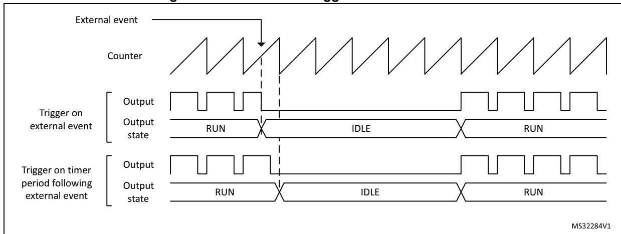
Figure 363. Burst mode trigger on external event
