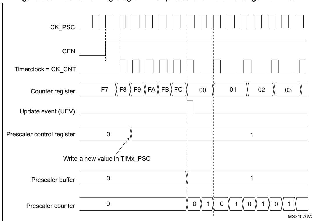
Figure 390. Counter timing diagram with prescaler division change from 1 to 2
