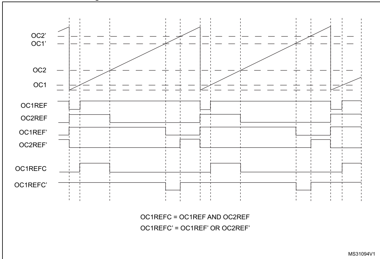
Figure 427. Combined PWM mode on channel 1 and 3
