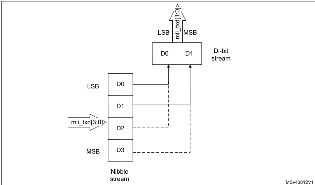
Figure 841. Transmission bit order
