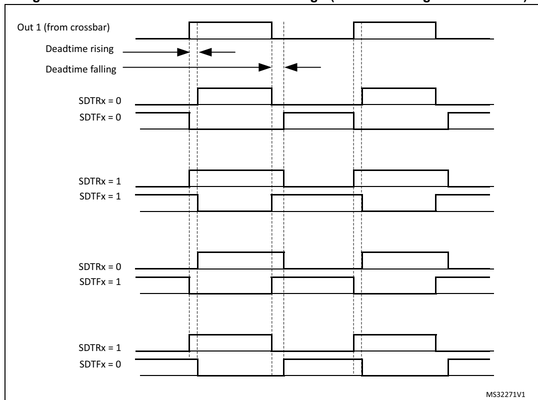
Figure 340. Deadtime insertion vs deadtime sign (1 indicates negative deadtime)
