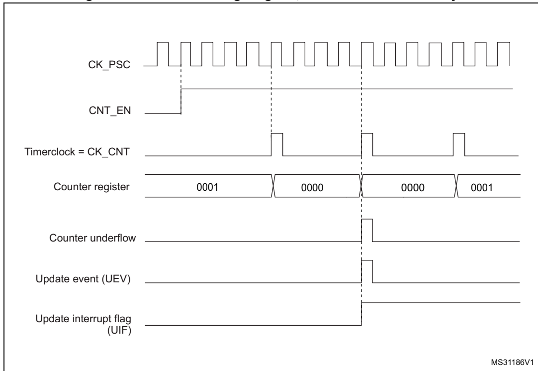
Figure 401. Counter timing diagram, internal clock divided by N
