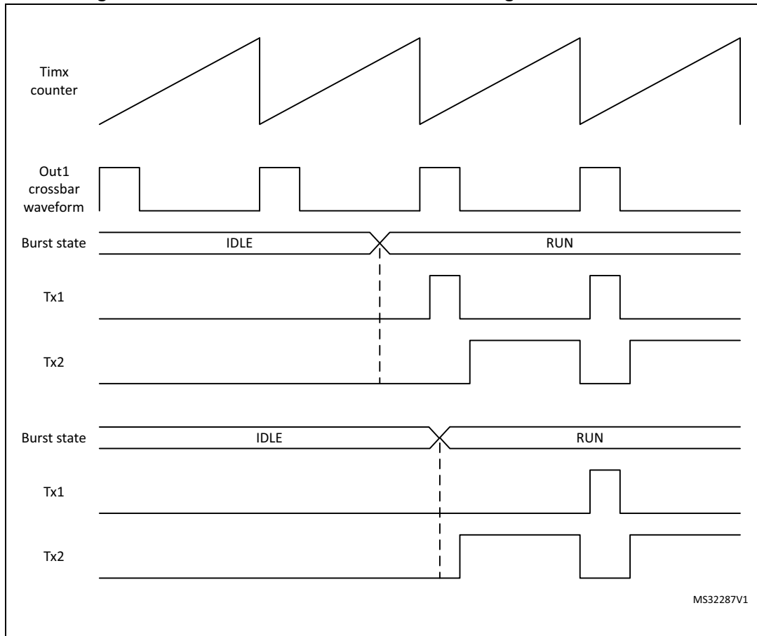
Figure 366. Burst mode exit when the deadtime generator is enabled
