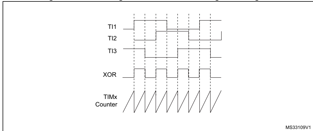
Figure 443. Measuring time interval between edges on 3 signals
