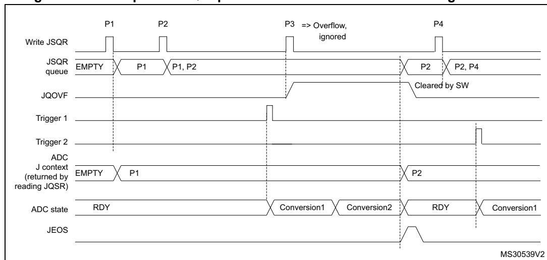
Figure 157. Example of JSQR queue of context with overflow during conversion
