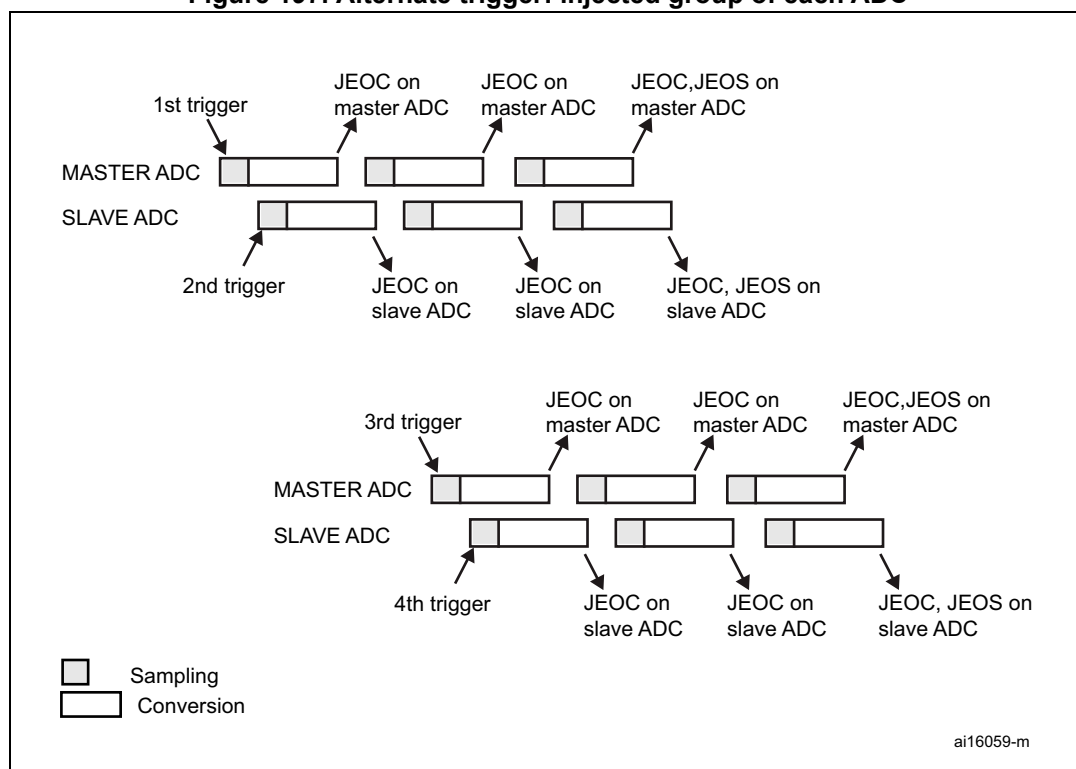
Figure 197. Alternate trigger: injected group of each ADC
