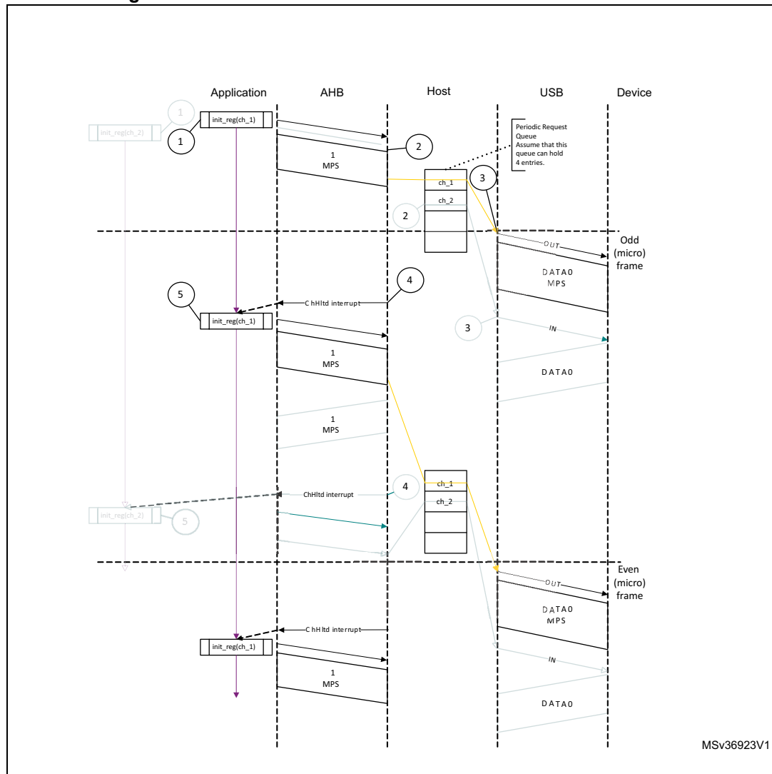
Figure 812. Normal isochronous OUT transaction - DMA mode
