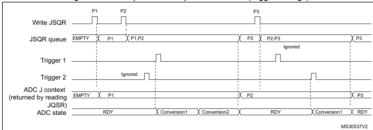
Figure 155. Example of JSQR queue of context (trigger change)
