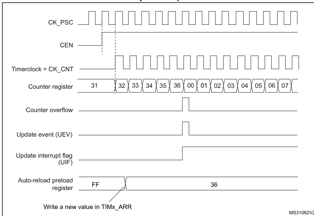
Figure 456. Counter timing diagram, Update event when ARPE=0 (TIMx_ARR not preloaded)
