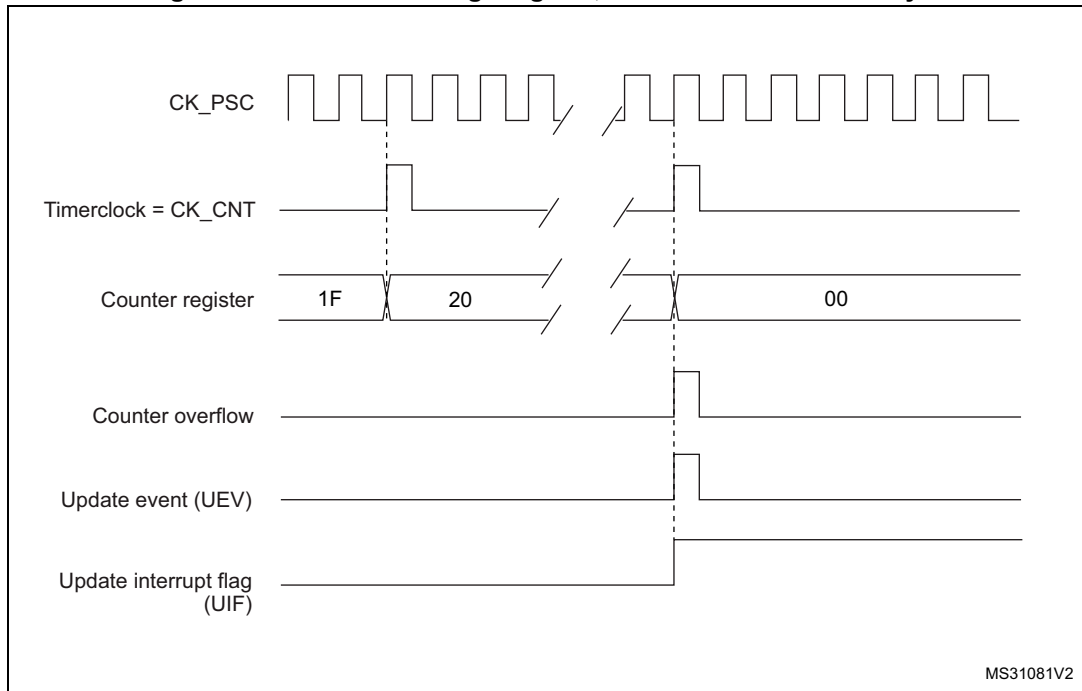
Figure 564. Counter timing diagram, update event when ARPE = 0 (TIMx_ARR not preloaded)
