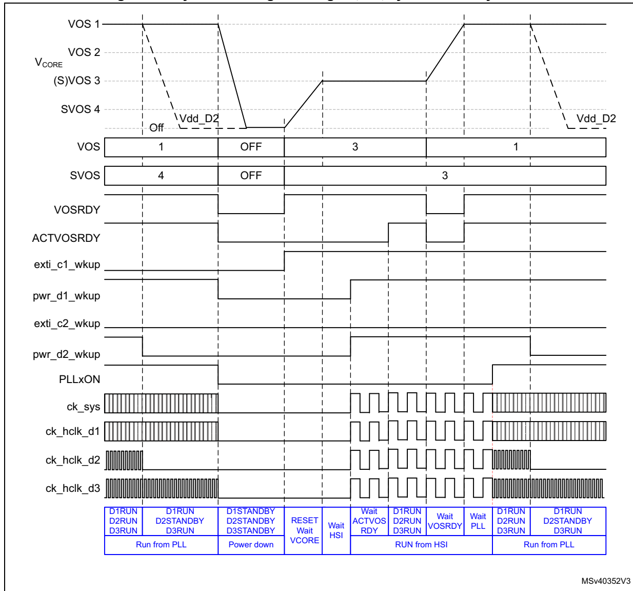
Figure 40. Dynamic Voltage Scaling D1, D2, system Standby mode
