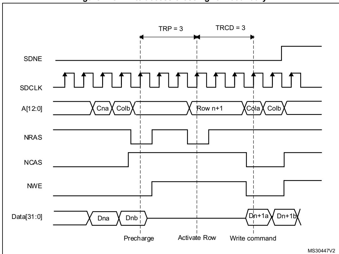
Figure 128. Write access crossing row boundary
