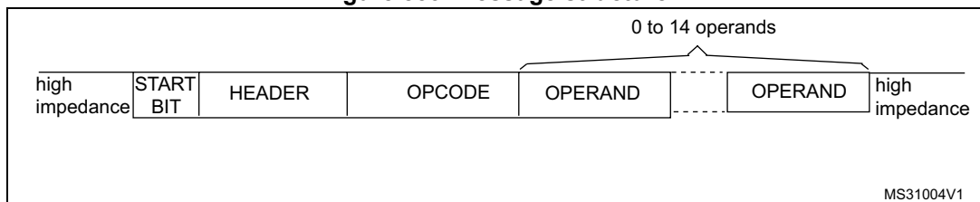
Figure 853. Message structure
