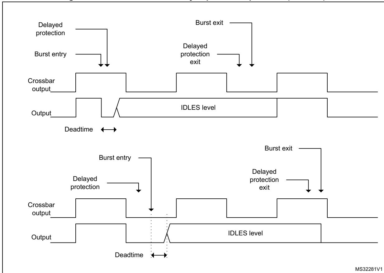
Figure 358. Burst mode and delayed protection priorities (DIDL = 1)
