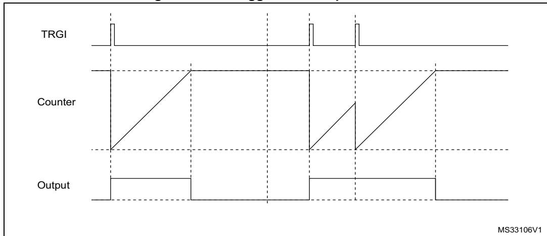
Figure 440. Retriggerable one pulse mode
