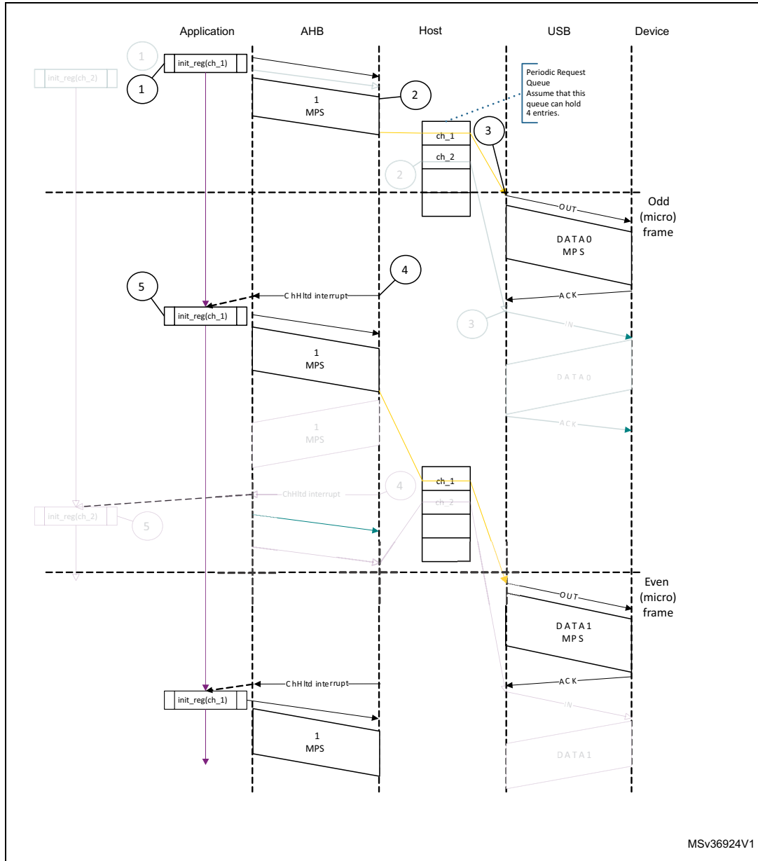
Figure 810. Normal interrupt OUT transactions - DMA mode
