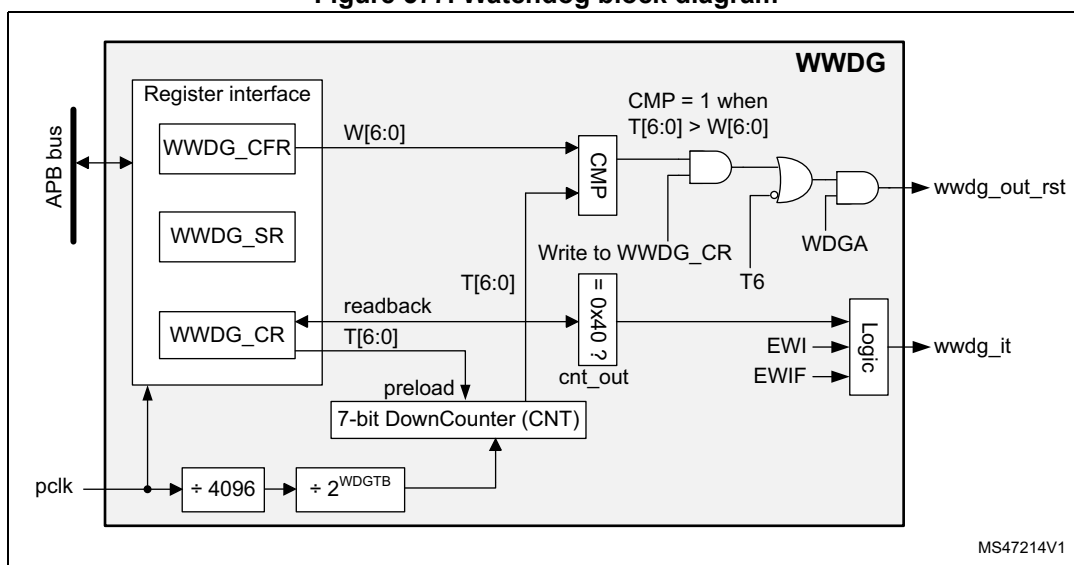
Figure 577. Watchdog block diagram
