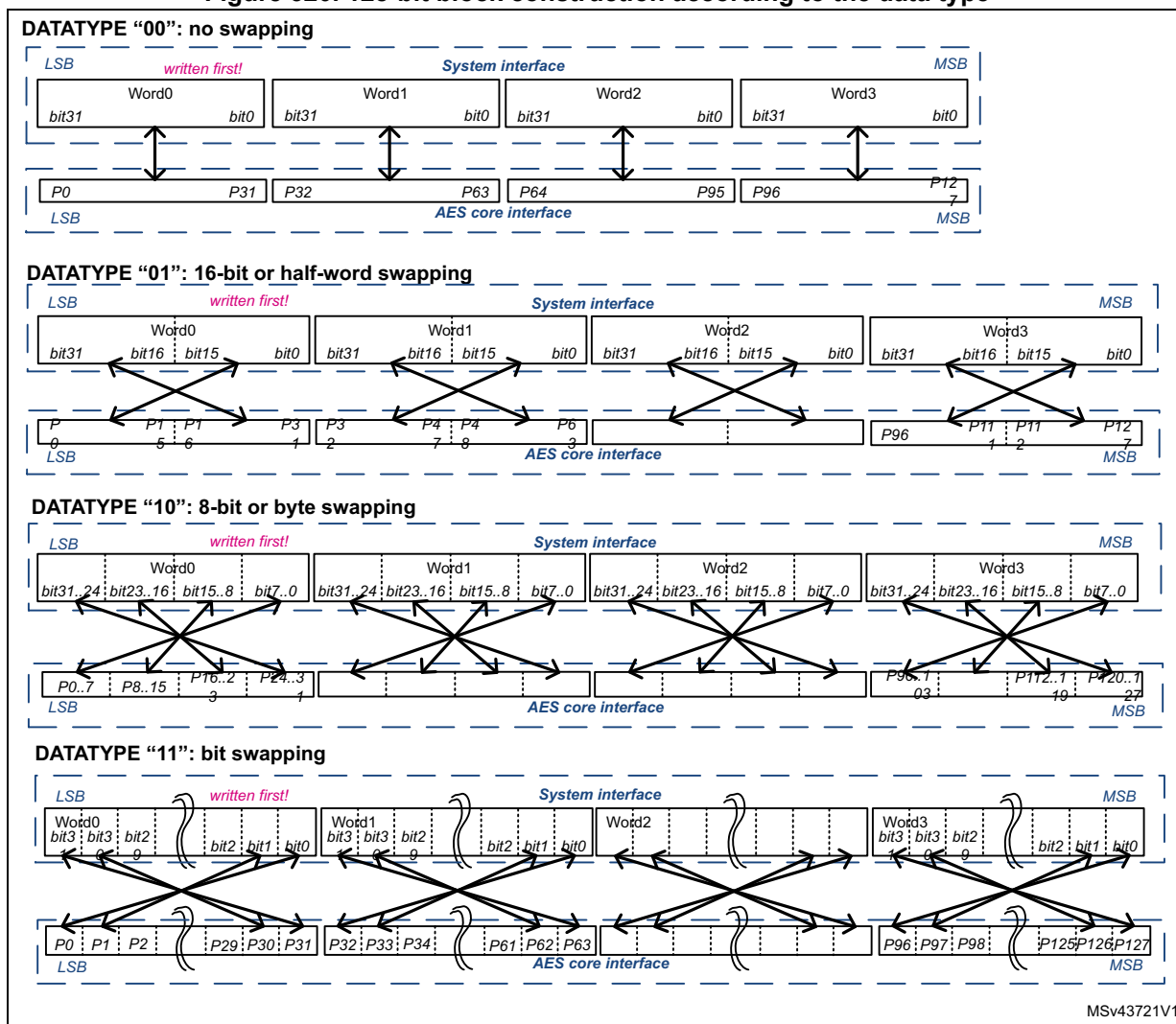
Figure 320. 128-bit block construction according to the data type
