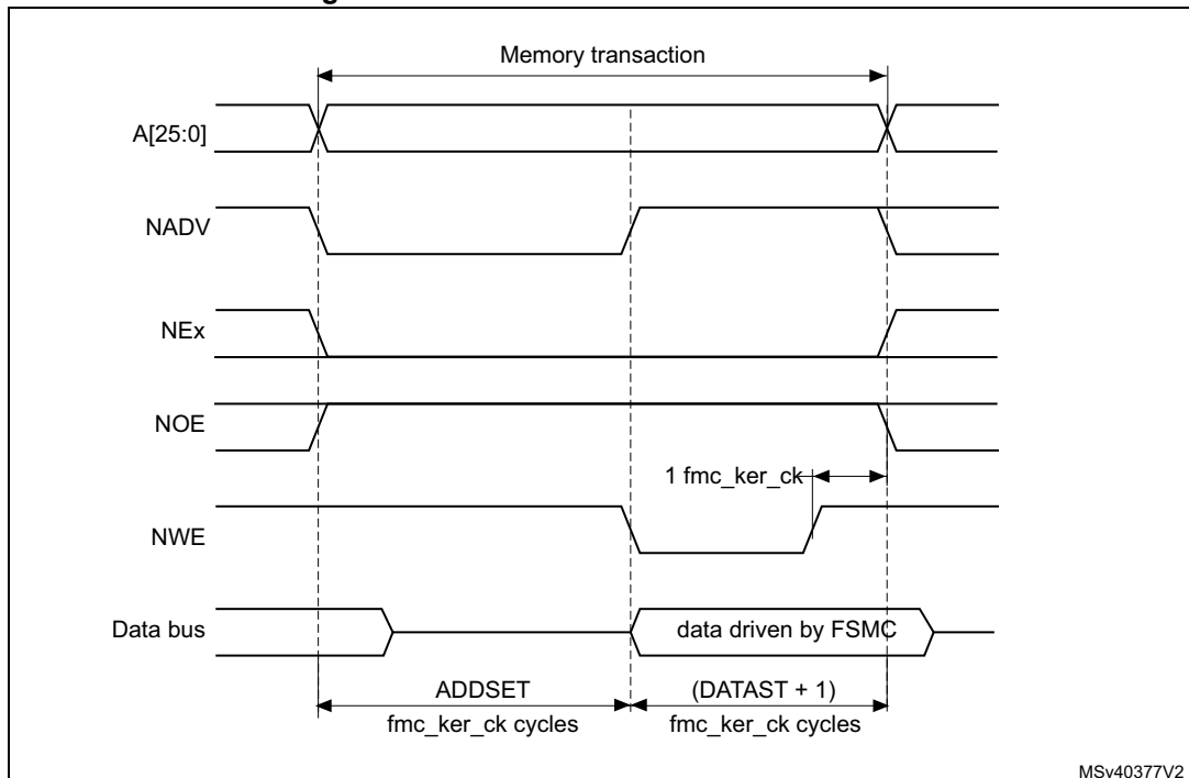
Figure 112. Mode C write access waveforms
