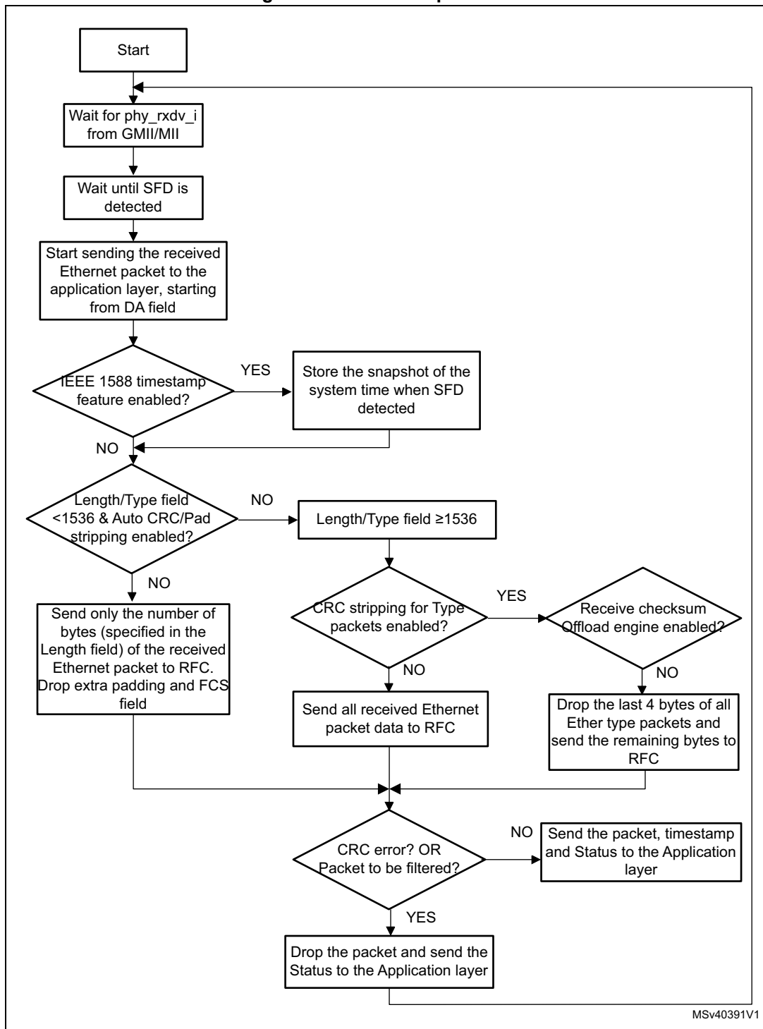
Figure 827. MAC reception flow
