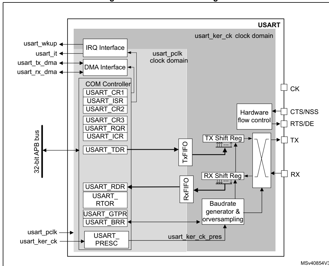
Figure 614. USART block diagram
