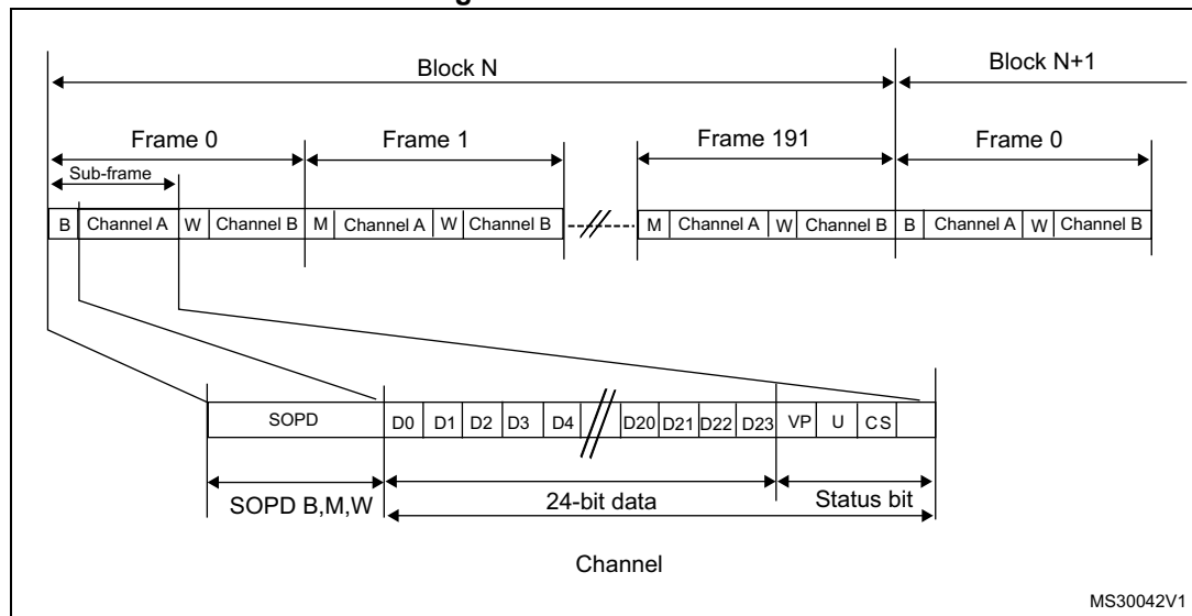
Figure 704. SPDIF format
