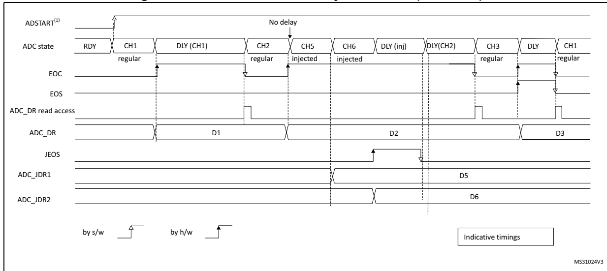
Figure 179. AUTDLY=1 in auto-injected mode (JAUTO=1)
