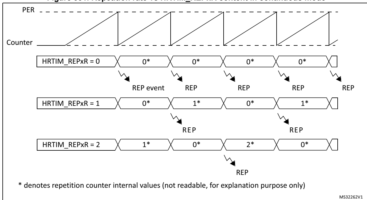
Figure 331. Repetition rate vs HRTIM_REPxR content in continuous mode
