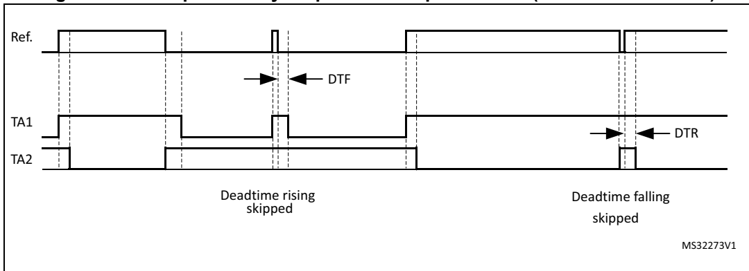
Figure 343. Complementary outputs for low pulse width (SDTRx = 0, SDTFx = 1)
