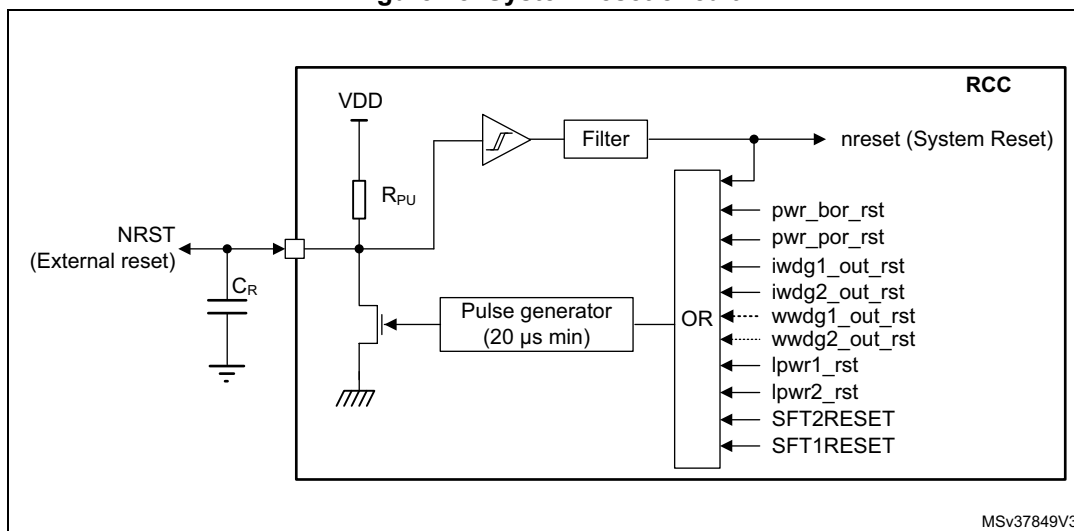
Figure 48. System reset circuit
