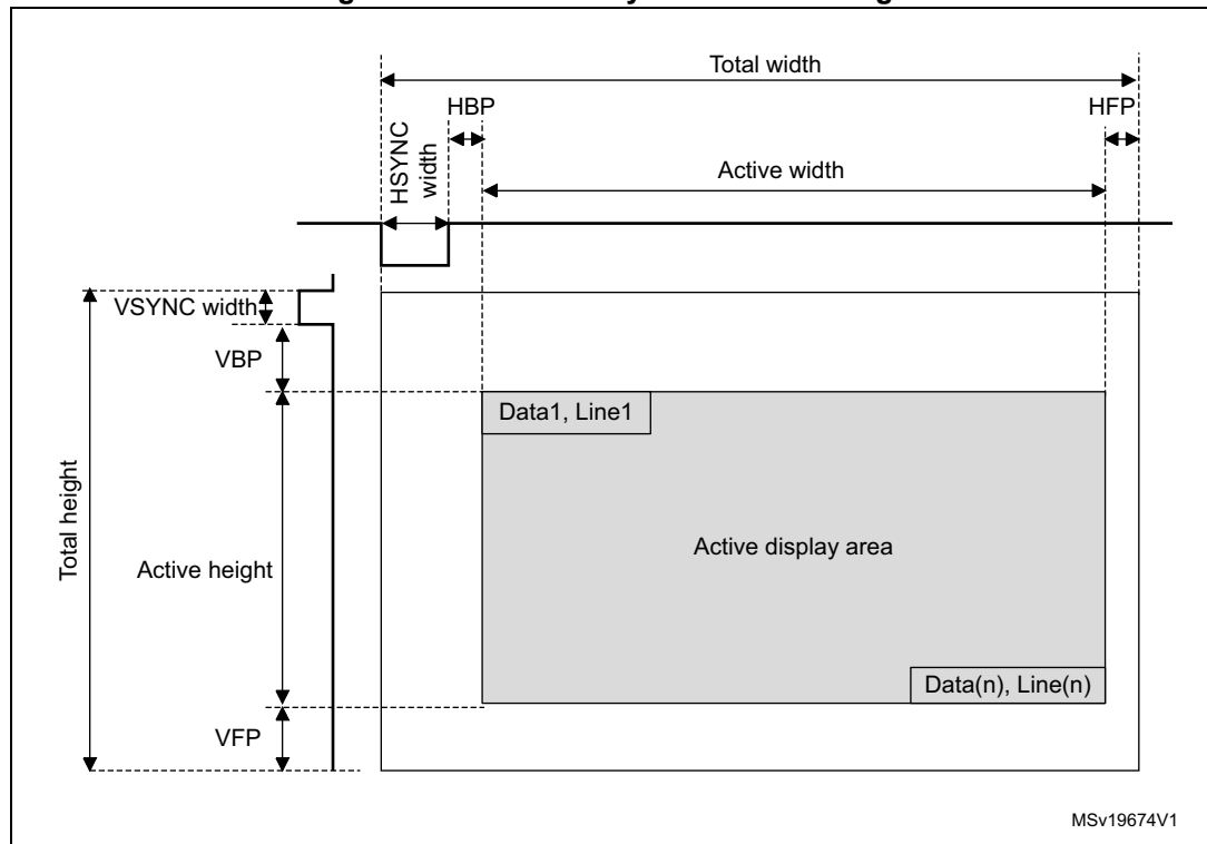
Figure 250. LCD-TFT synchronous timings
