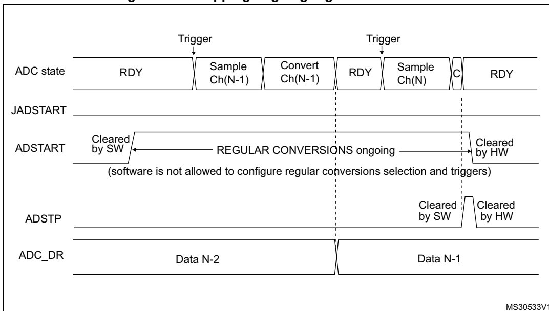
Figure 150. Stopping ongoing regular conversions
