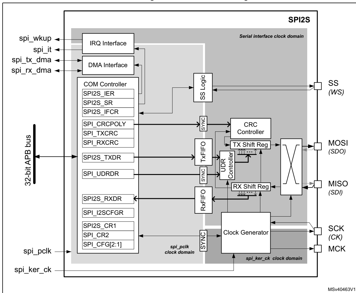
Figure 655. SPI2S block diagram
