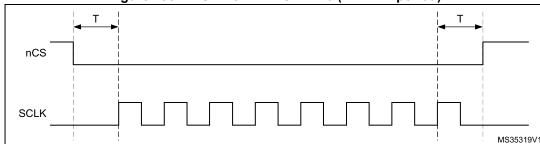
Figure 135. nCS when CKMODE = 0 (T = CLK period)
