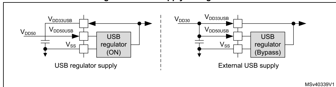
Figure 27. USB supply configurations
