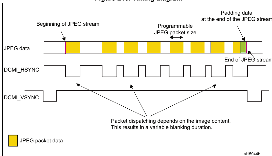
Figure 243. Timing diagram
