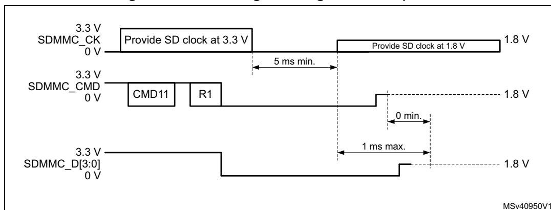
Figure 774. CMD11 signal voltage switch sequence
