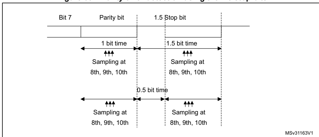
Figure 631. Parity error detection using the 1.5 stop bits
