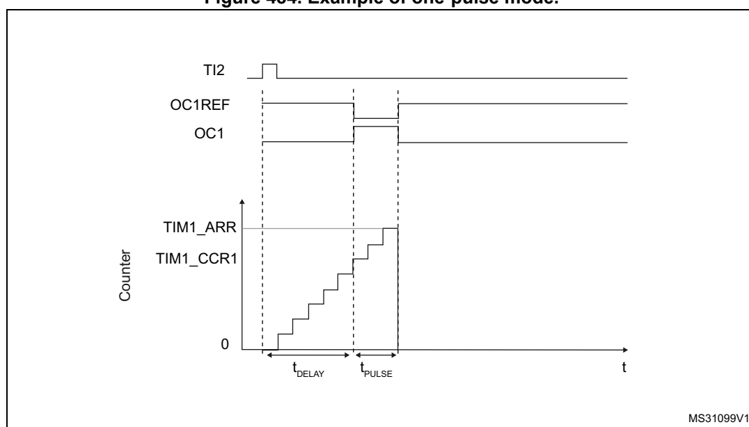
Figure 484. Example of one-pulse mode.
