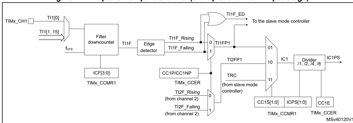
Figure 474. Capture/Compare channel (example: channel 1 input stage)
