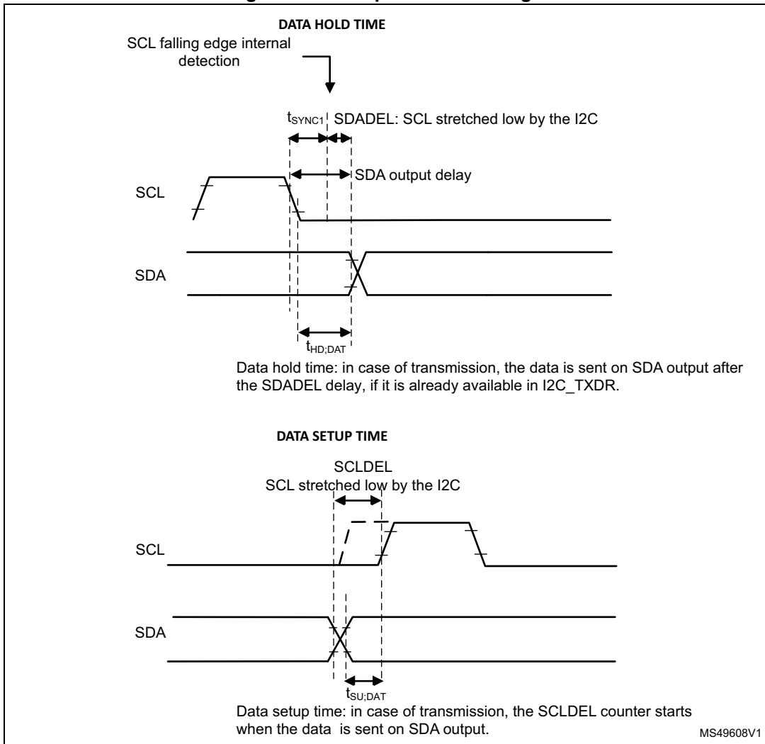
Figure 585. Setup and hold timings
