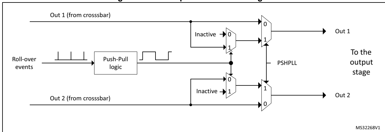
Figure 337. Push-pull mode block diagram
