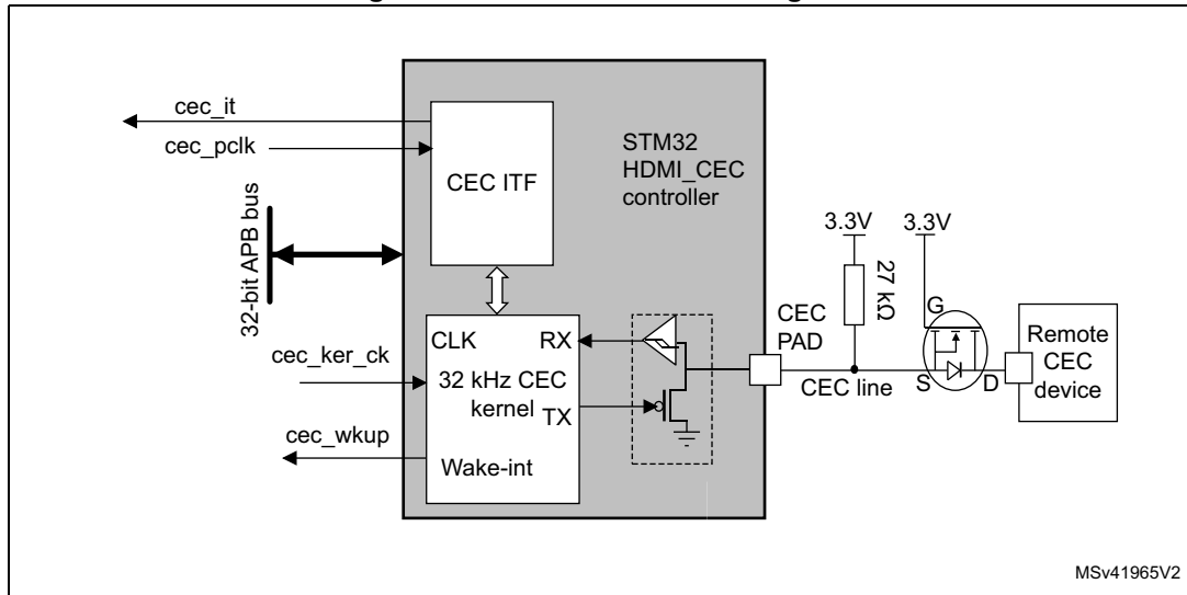
Figure 852. HDMI-CEC block diagram
