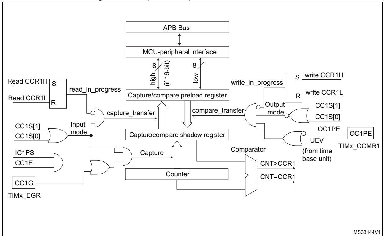
Figure 475. Capture/Compare channel 1 main circuit
