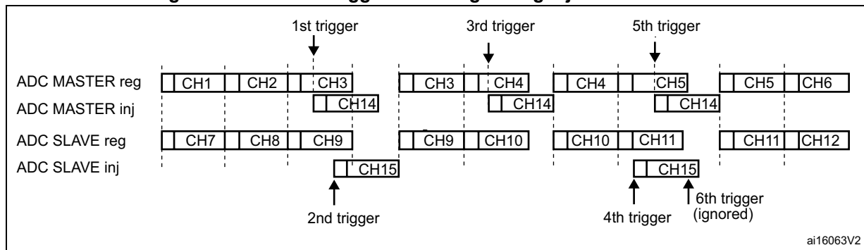
Figure 200. Case of trigger occurring during injected conversion
