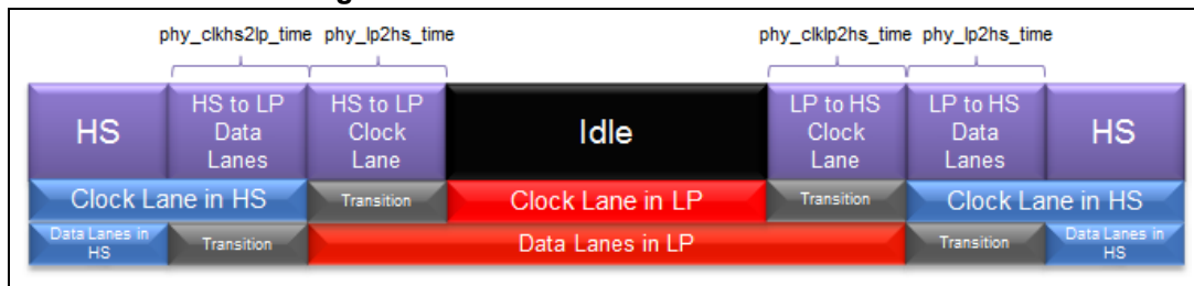
Figure 279. Clock lane and data lane in LP
