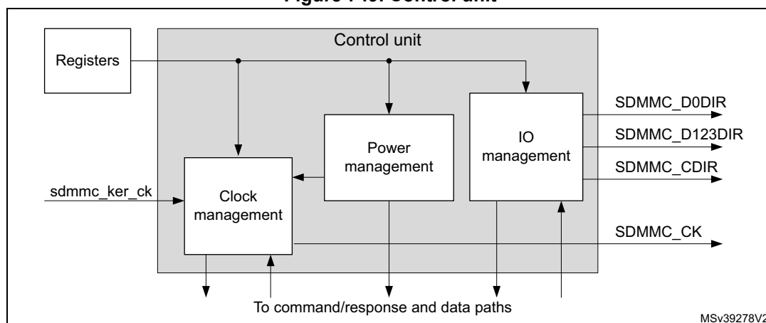
Figure 749. Control unit
