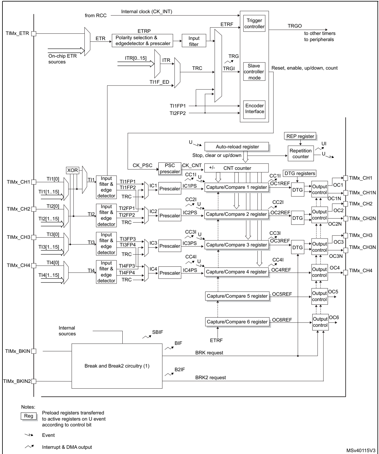
Figure 389. Advanced-control timer block diagram
