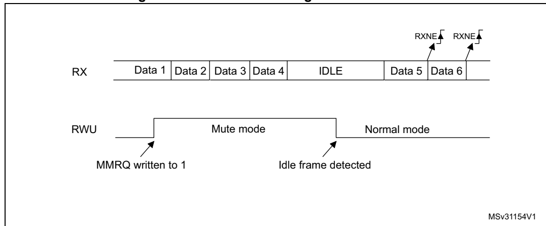
Figure 646. Mute mode using Idle line detection
