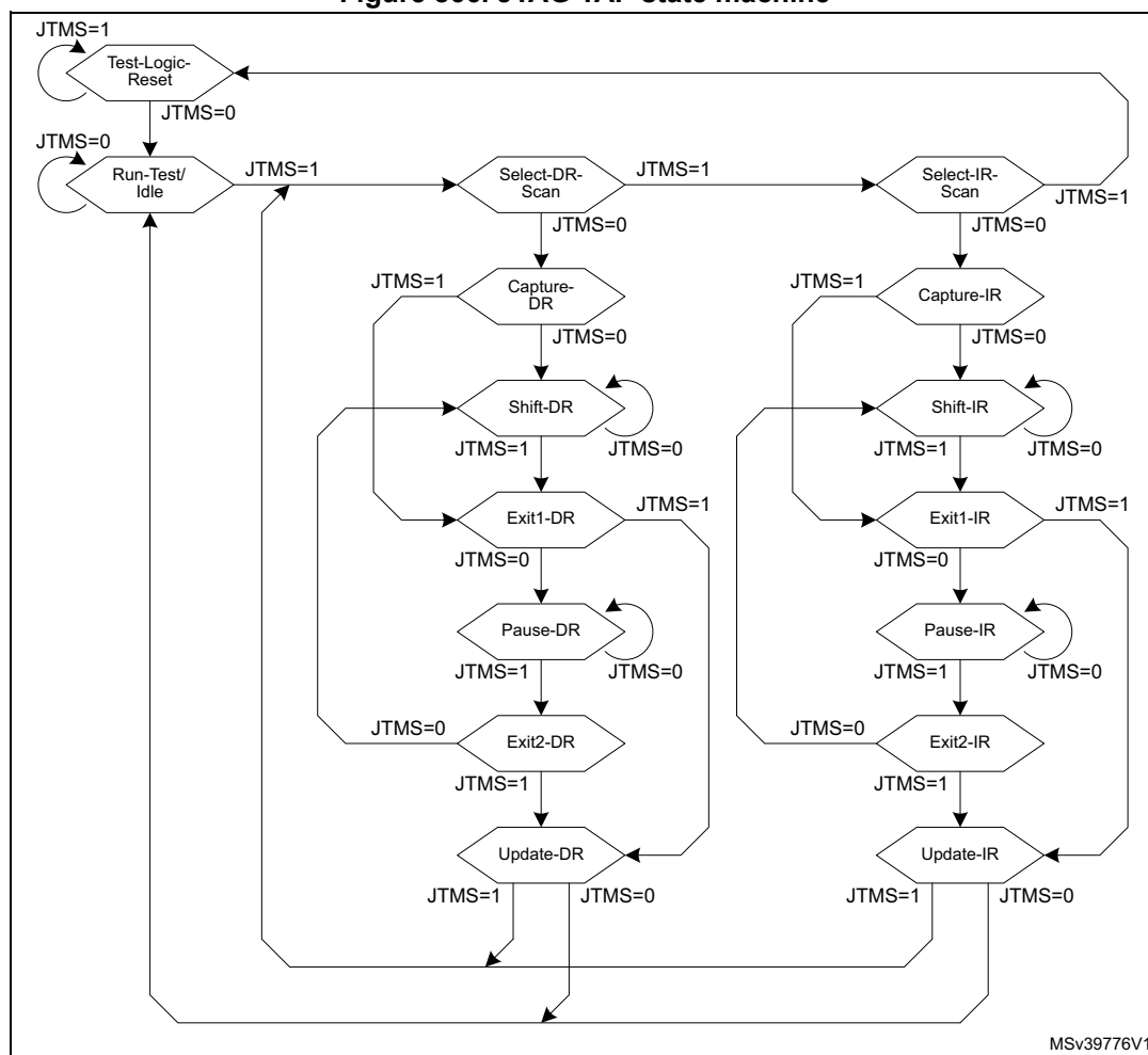
Figure 866. JTAG TAP state machine
