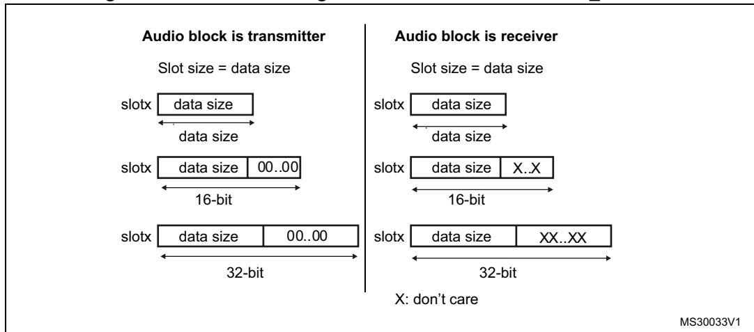
Figure 693. Slot size configuration with FBOFF = 0 in SAI_xSLOTR
