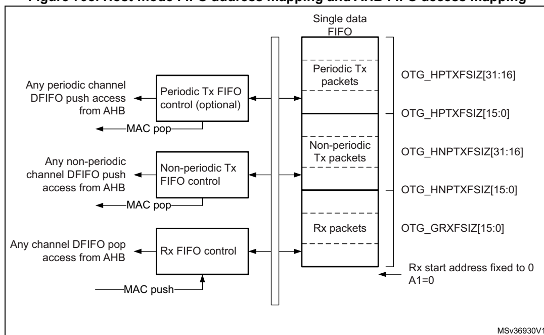
Figure 798. Host-mode FIFO address mapping and AHB FIFO access mapping
