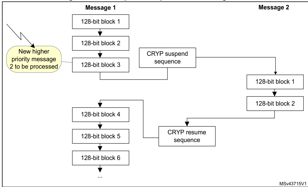
Figure 304. Example of suspend mode management
