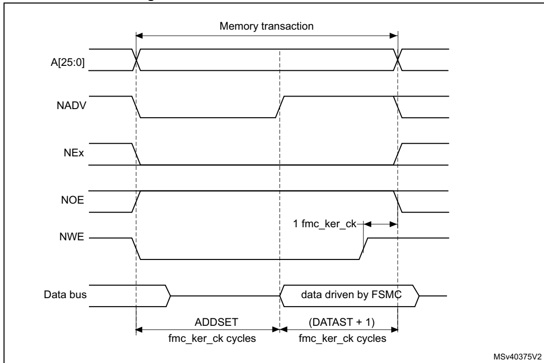
Figure 110. Mode B write access waveforms
