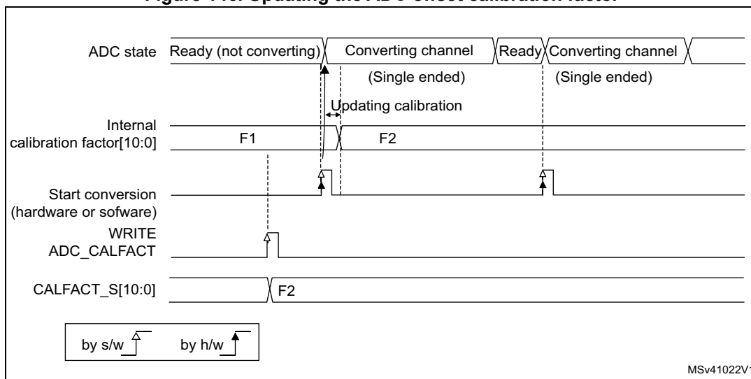
Figure 146. Updating the ADC offset calibration factor
