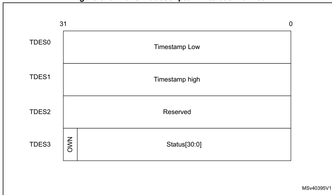
Figure 846. Transmit descriptor write-back format
