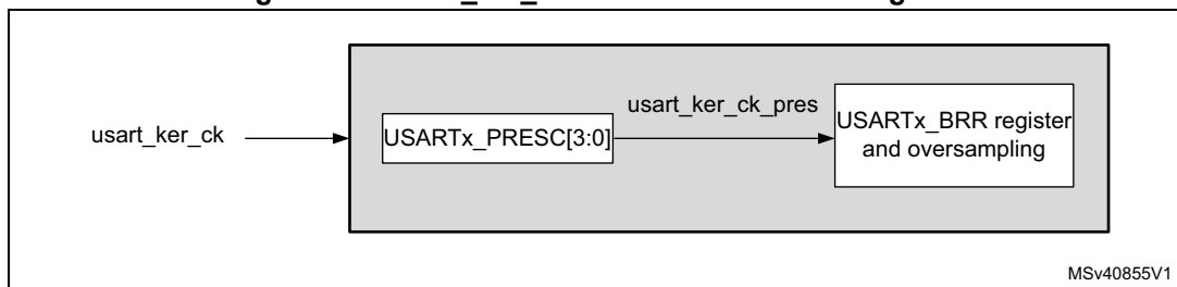
Figure 619. usart_ker_ck clock divider block diagram
