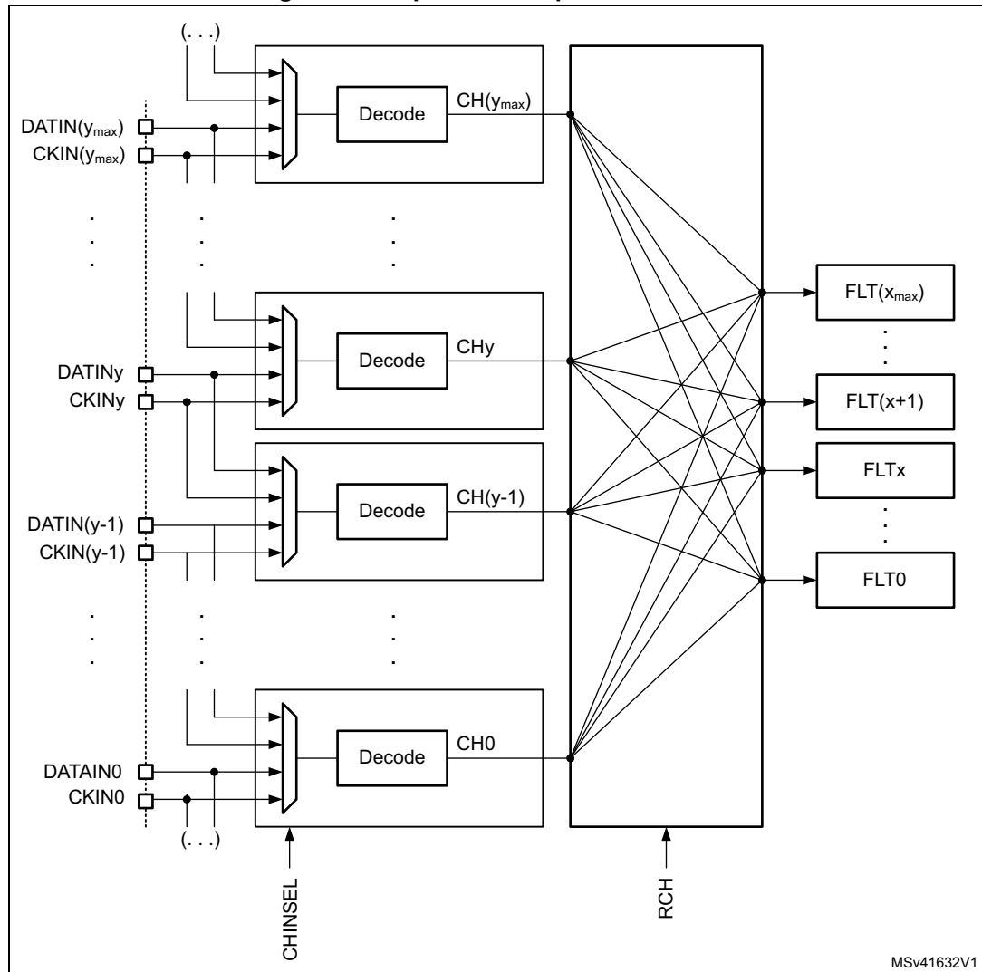
Figure 233. Input channel pins redirection
