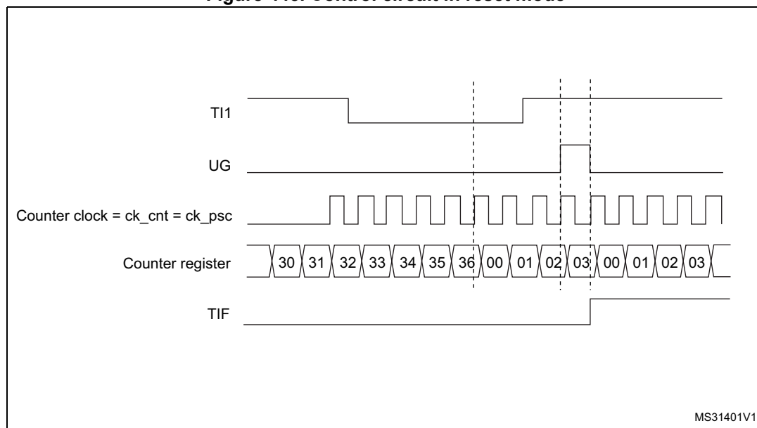
Figure 445. Control circuit in reset mode
