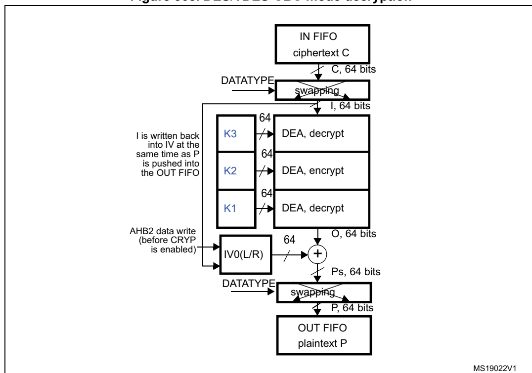
Figure 308. DES/TDES-CBC mode decryption
