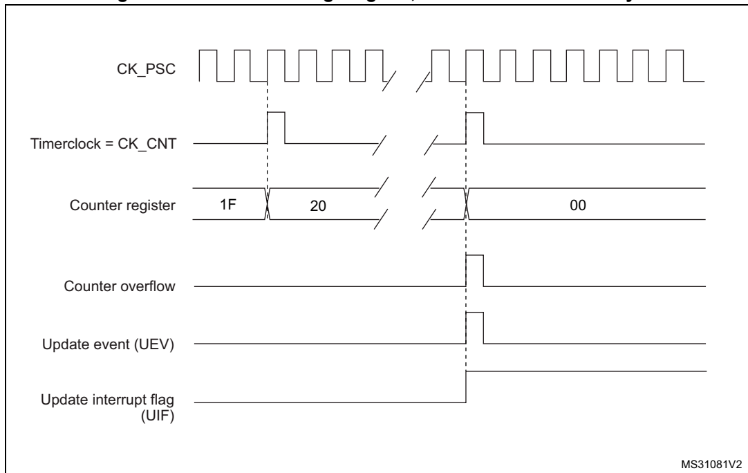
Figure 395. Counter timing diagram, internal clock divided by N
