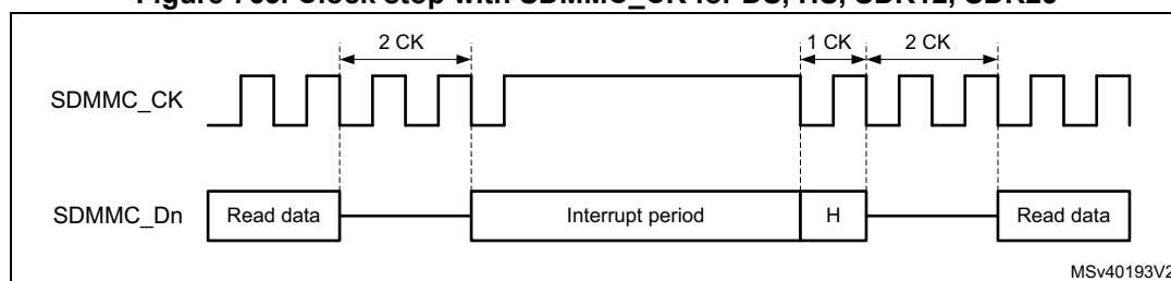
Figure 763. Clock stop with SDMMC_CK for DS, HS, SDR12, SDR25
