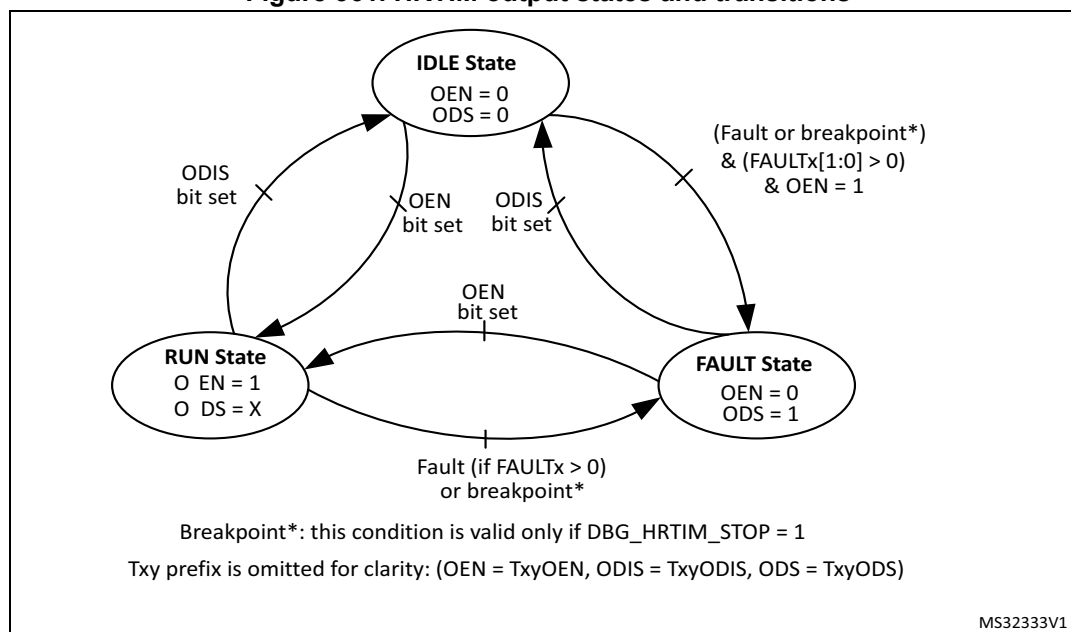
Figure 361. HRTIM output states and transitions
