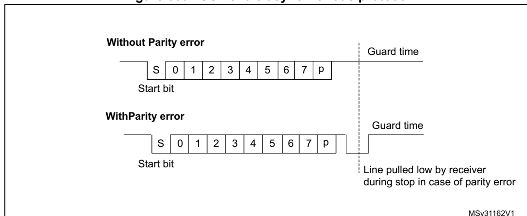
Figure 630. ISO 7816-3 asynchronous protocol
