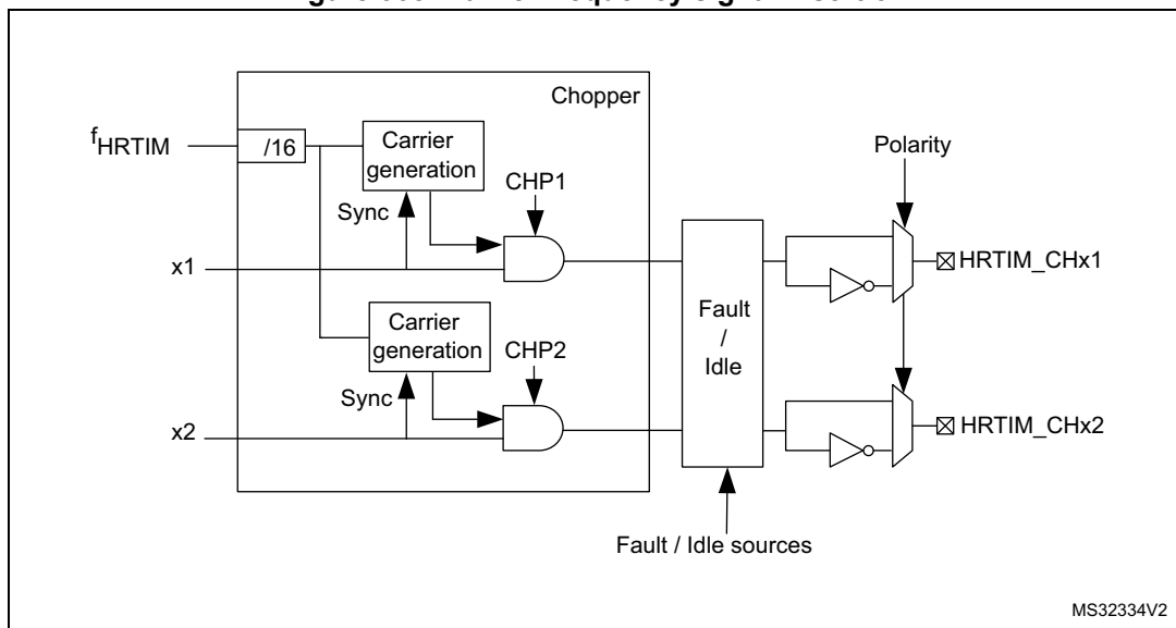
Figure 368. Carrier frequency signal insertion
