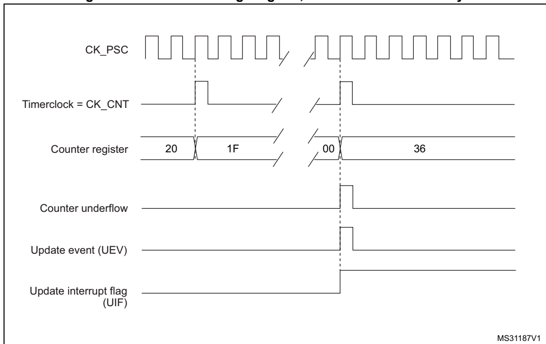
Figure 461. Counter timing diagram, internal clock divided by N
