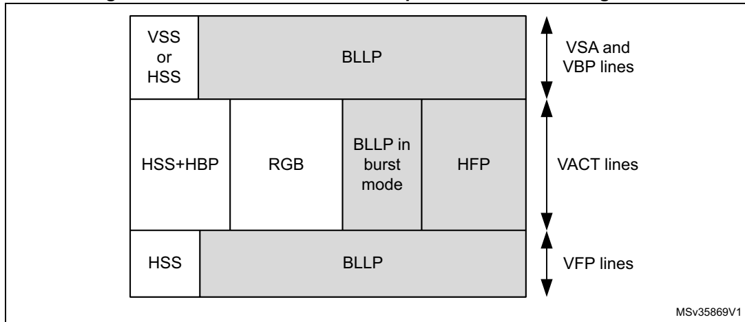
Figure 269. Command transmission periods within the image area
