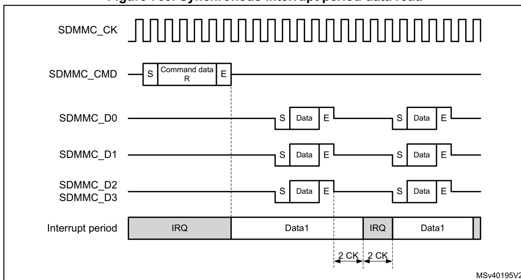
Figure 759. Synchronous interrupt period data read
