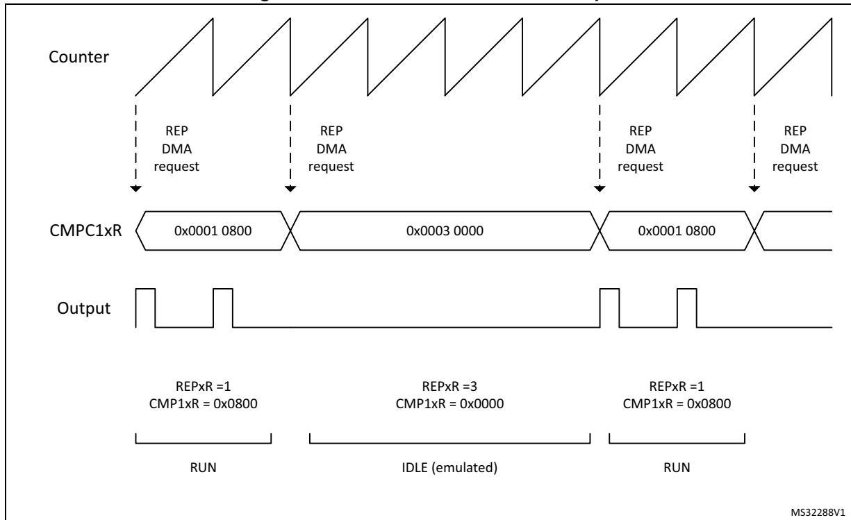
Figure 367. Burst mode emulation example
