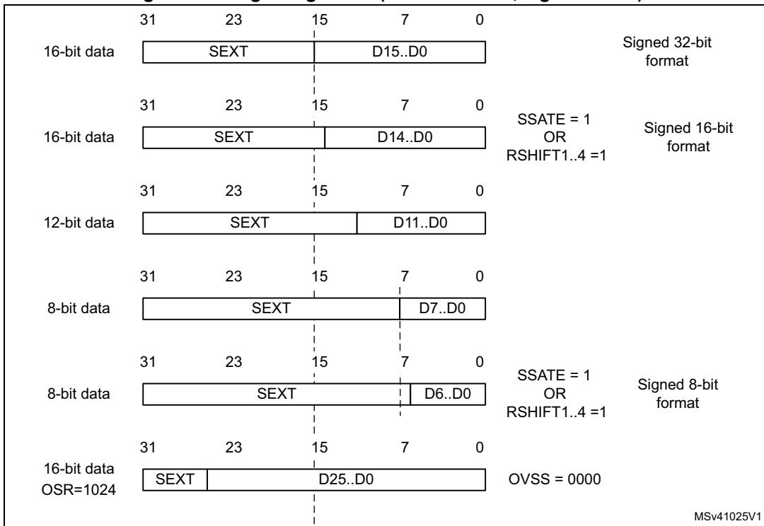
Figure 171. Right alignment (offset enabled, signed value)
