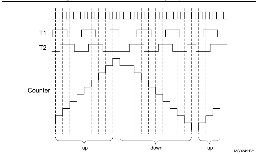
Figure 575. Encoder mode counting sequence
