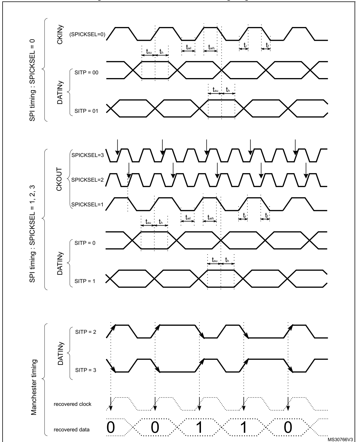
Figure 234. Channel transceiver timing diagrams
