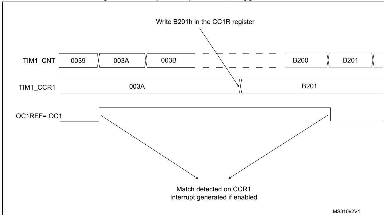
Figure 423. Output compare mode, toggle on OC1
