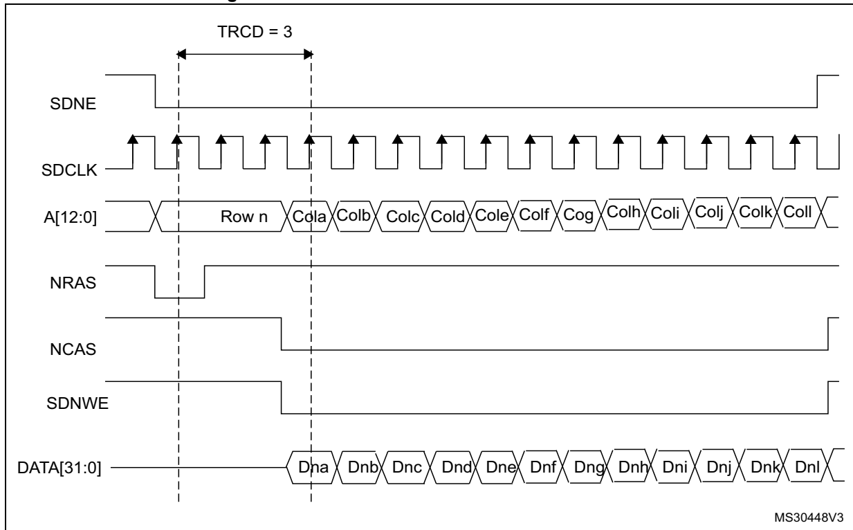
Figure 124. Burst write SDRAM access waveforms
