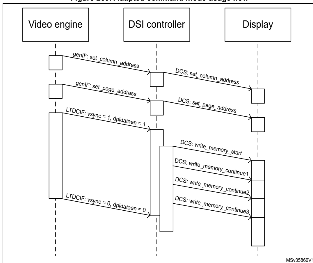
Figure 259. Adapted command mode usage flow
