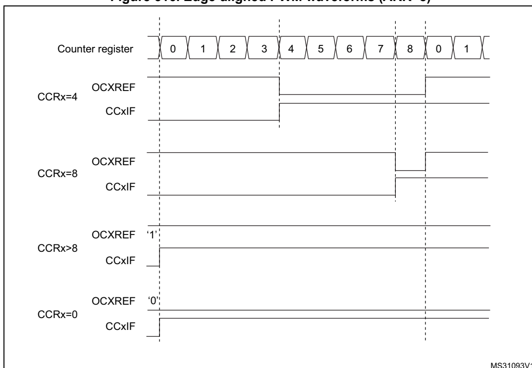
Figure 516. Edge-aligned PWM waveforms (ARR=8)
