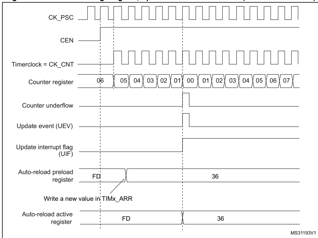
Figure 407. Counter timing diagram, update event with ARPE=1 (counter underflow)
