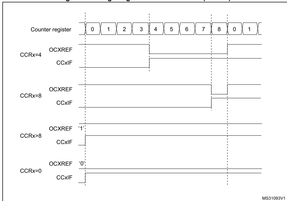
Figure 424. Edge-aligned PWM waveforms (ARR=8)
