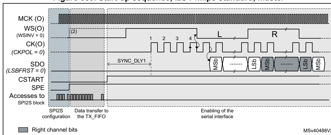
Figure 680. Start-up sequence, I2S Philips standard, master
