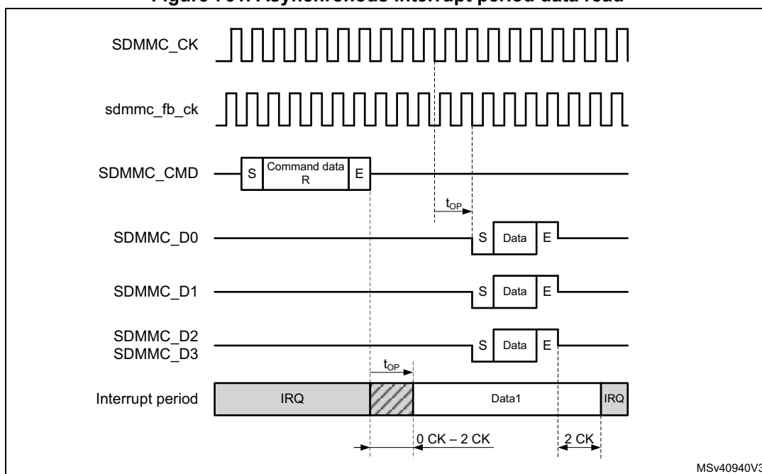
Figure 761. Asynchronous interrupt period data read
