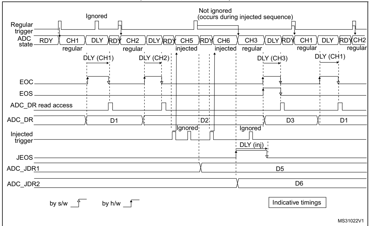
Figure 177. AUTDLY=1, regular HW conversions interrupted by injected conversions (DISCEN=1, JDISCEN=1)
