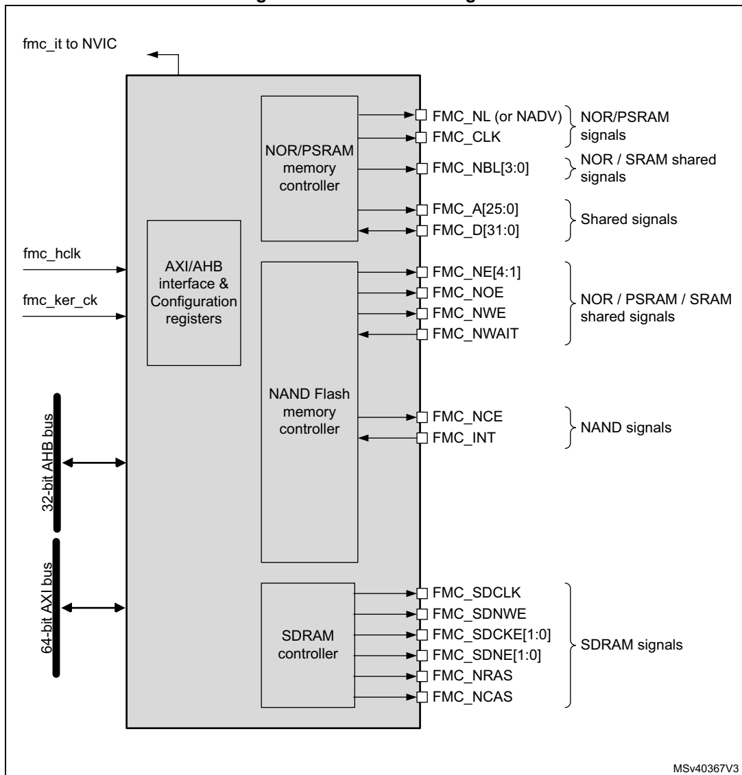
Figure 102. FMC block diagram
