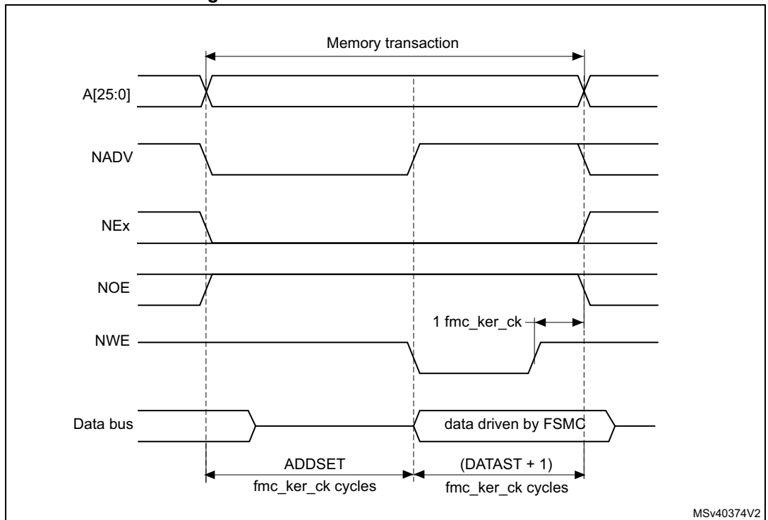
Figure 109. Mode 2 write access waveforms
