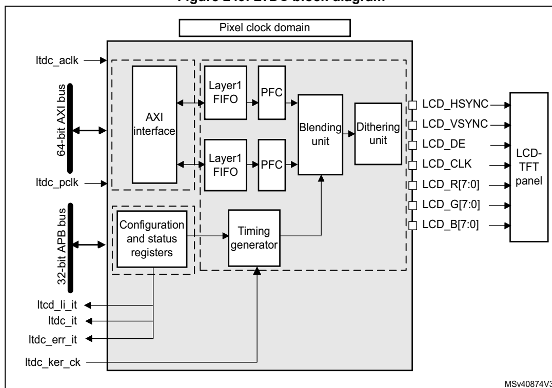
Figure 249. LTDC block diagram
