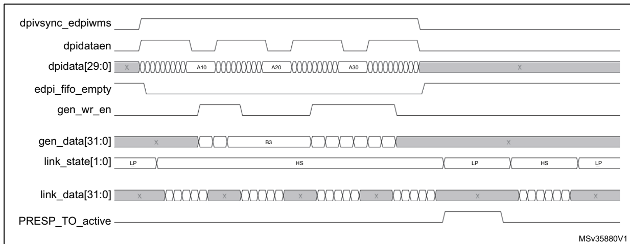
Figure 268. Effect of prep mode at 1
