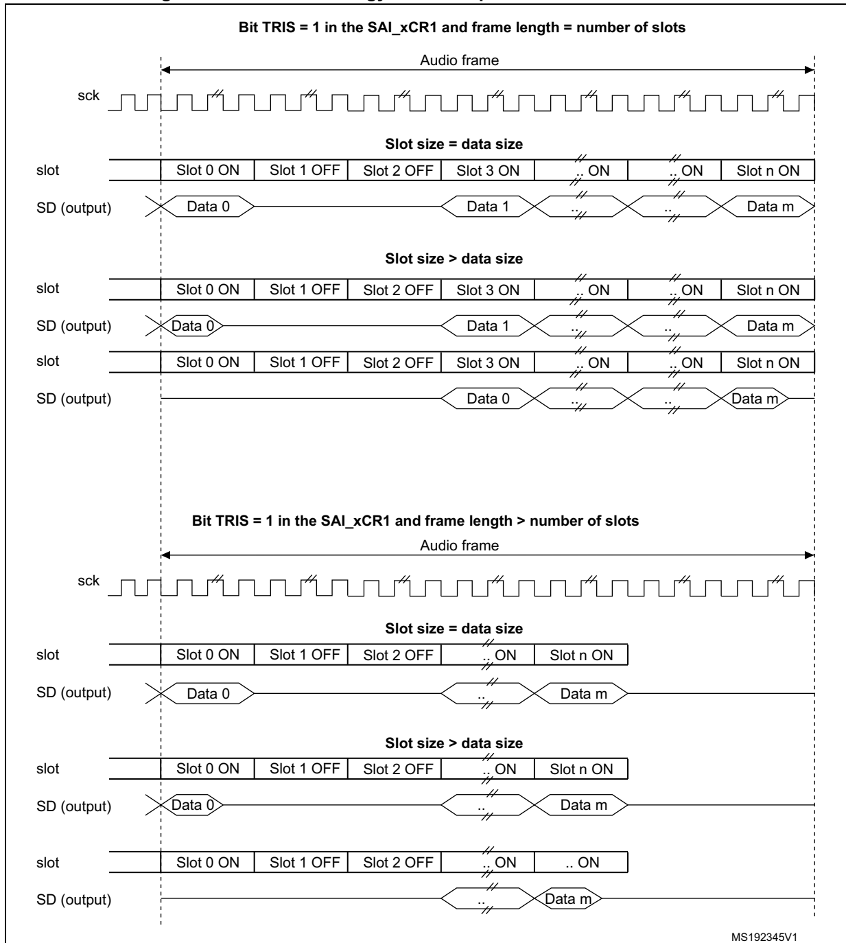
Figure 707. Tristate strategy on SD output line on an inactive slot
