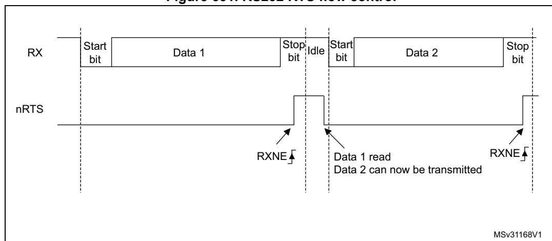
Figure 651. RS232 RTS flow control
