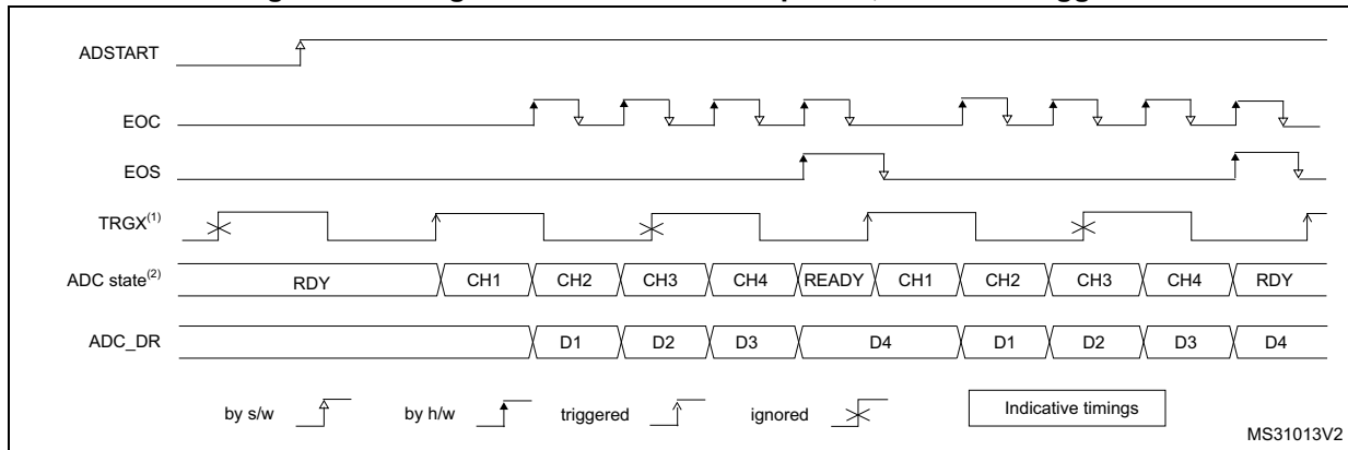
Figure 168. Single conversions of a sequence, hardware trigger
