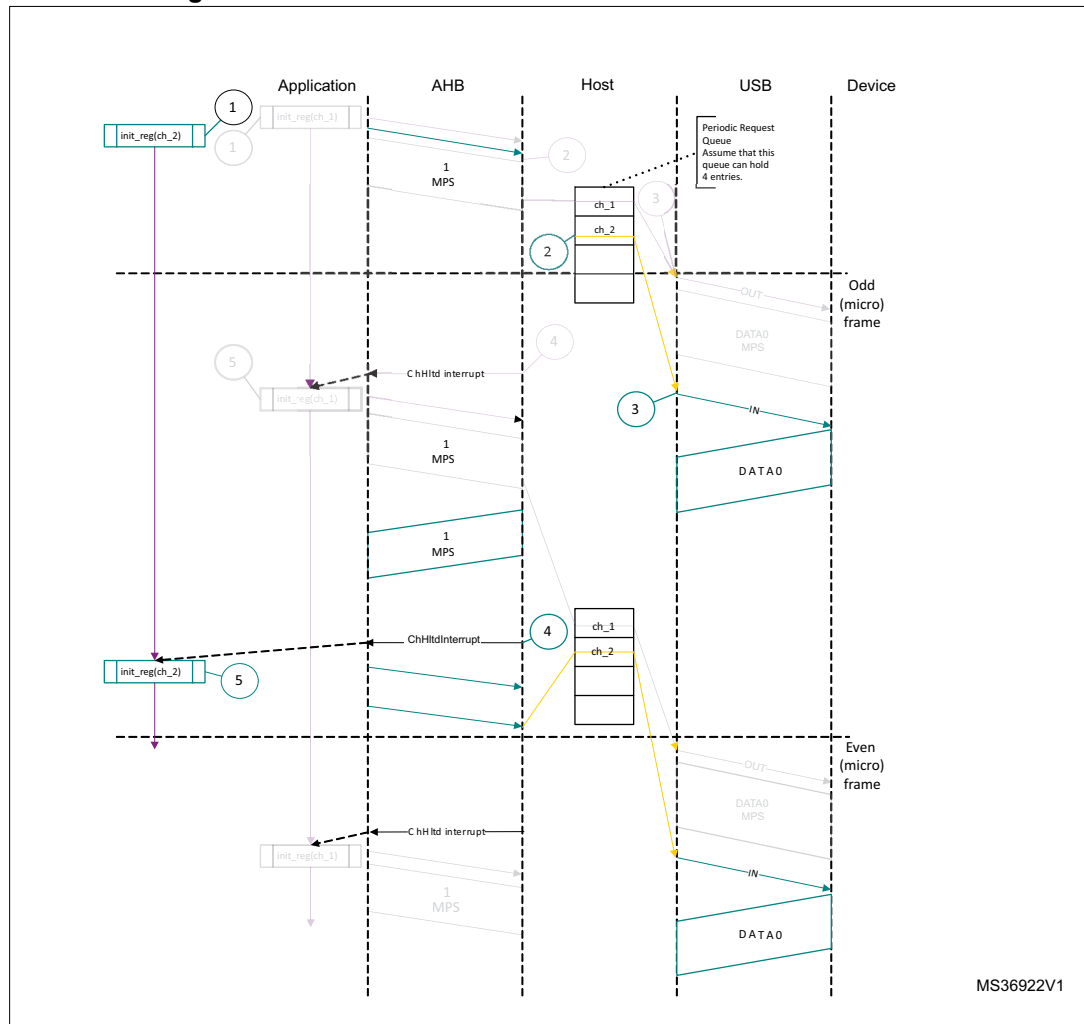
Figure 813. Normal isochronous IN transactions - DMA mode
