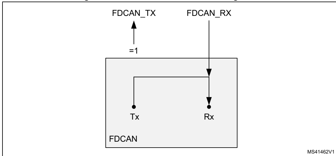
Figure 779. Pin control in bus monitoring mode
