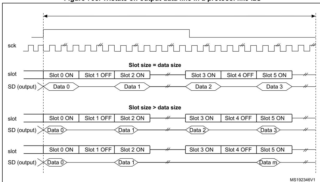
Figure 708. Tristate on output data line in a protocol like I2S
