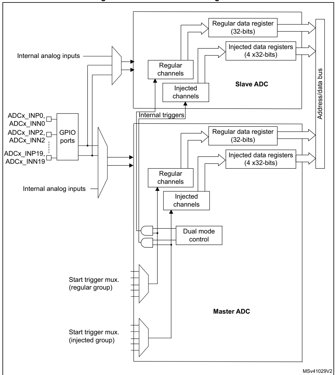
Figure 191. Dual ADC block diagram (1)
