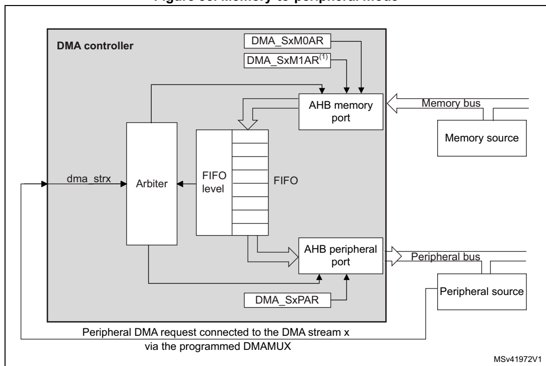
Figure 85. Memory-to-peripheral mode
