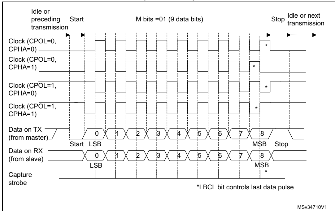
Figure 628. USART data clock timing diagram in synchronous master mode (M bits = '01')
