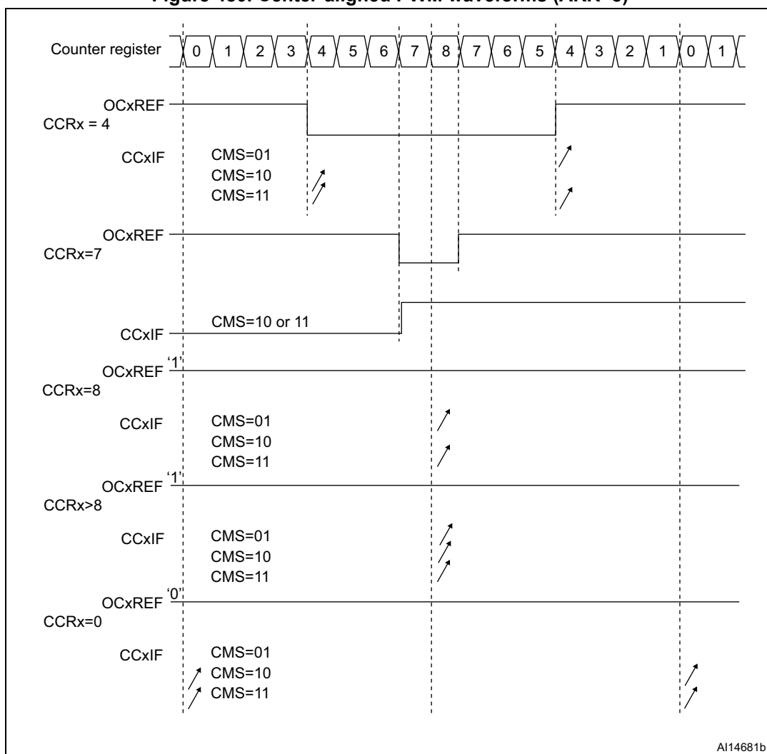
Figure 480. Center-aligned PWM waveforms (ARR=8)
