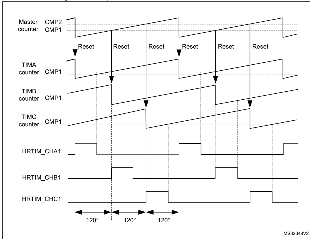
Figure 386. 3-phase interleaved buck converter control
