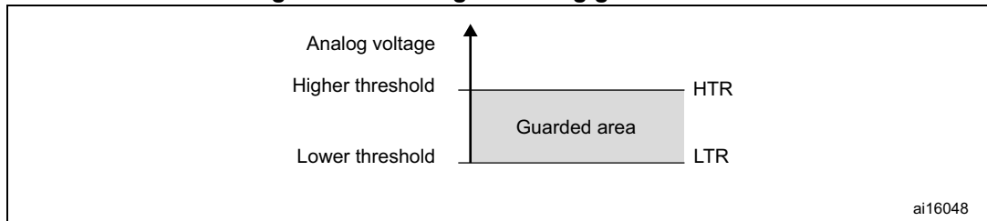
Figure 180. Analog watchdog guarded area
