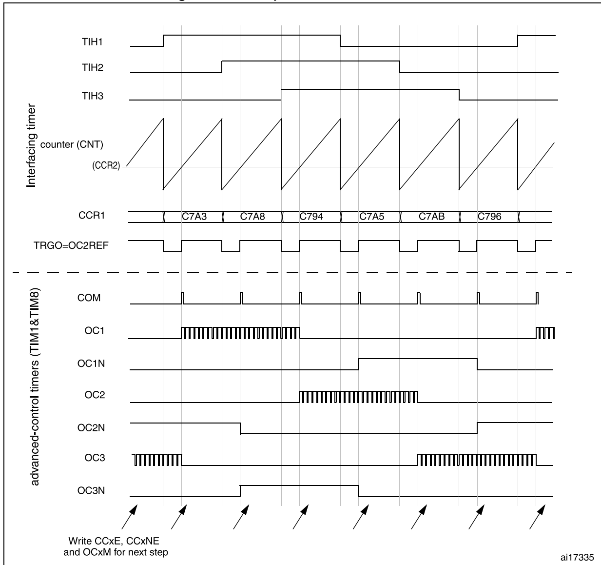
Figure 444. Example of Hall sensor interface
