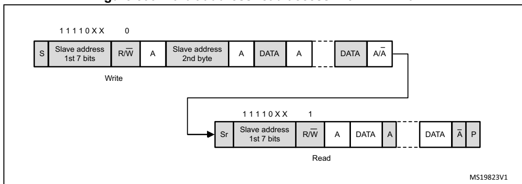
Figure 599. 10-bit address read access with HEAD10R=1
