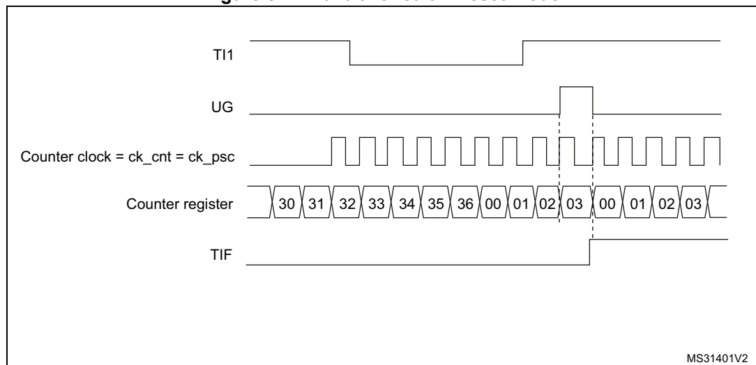
Figure 521. Control circuit in reset mode
