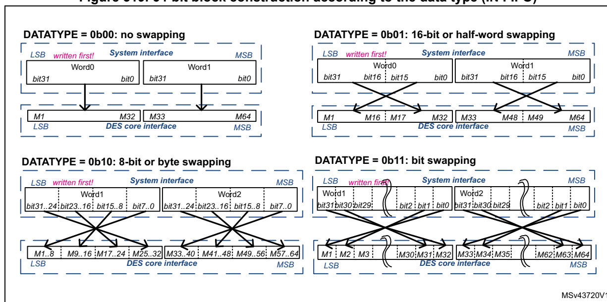
Figure 319. 64-bit block construction according to the data type (IN FIFO)
