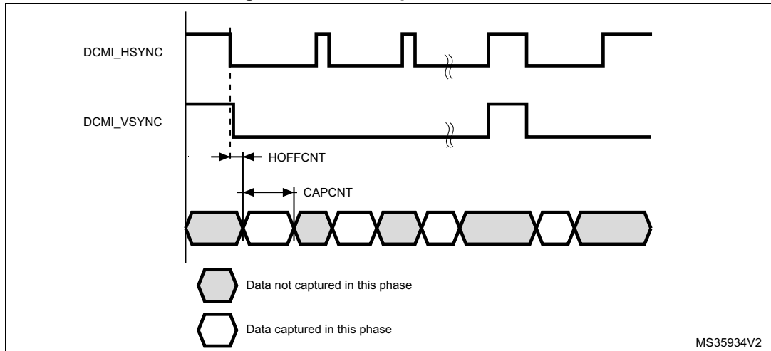
Figure 247. Data capture waveforms
