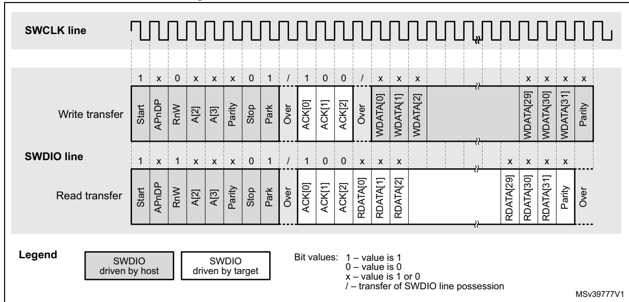
Figure 865. SWD successful data transfer
