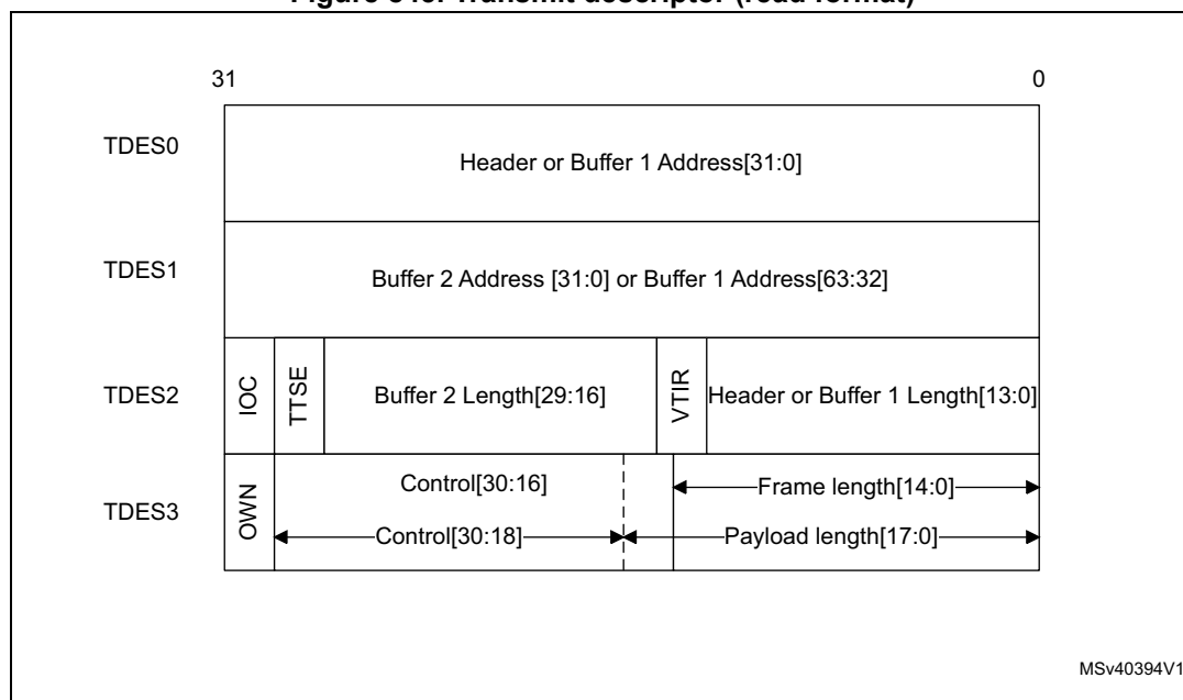
Figure 845. Transmit descriptor (read format)
