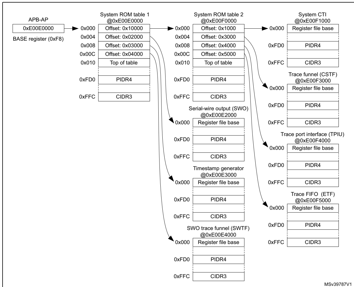
Figure 868. APB-D CoreSight component topology
