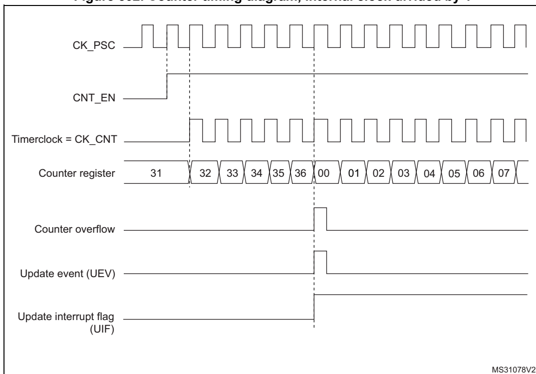
Figure 502. Counter timing diagram, internal clock divided by 1
