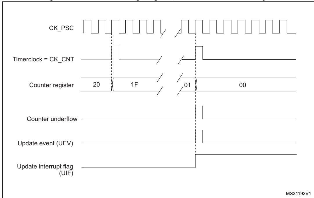
Figure 467. Counter timing diagram, Update event with ARPE=1 (counter underflow)
