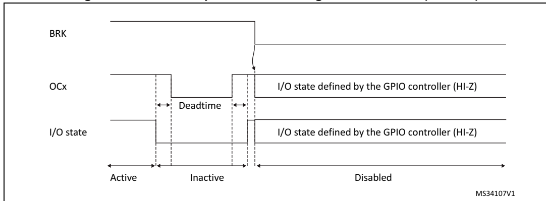
Figure 435. PWM output state following BRK assertion (OSS1=0)
