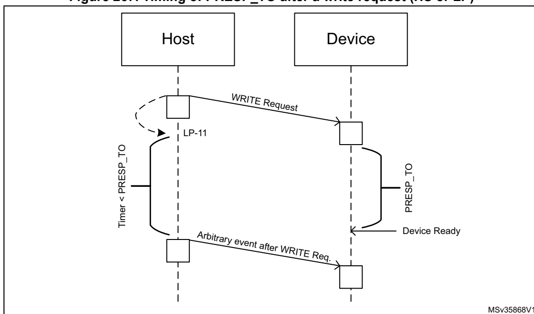
Figure 267. Timing of PRESP_TO after a write request (HS or LP)
