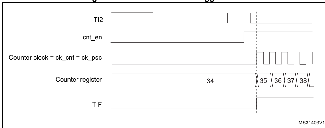
Figure 556. Control circuit in trigger mode
