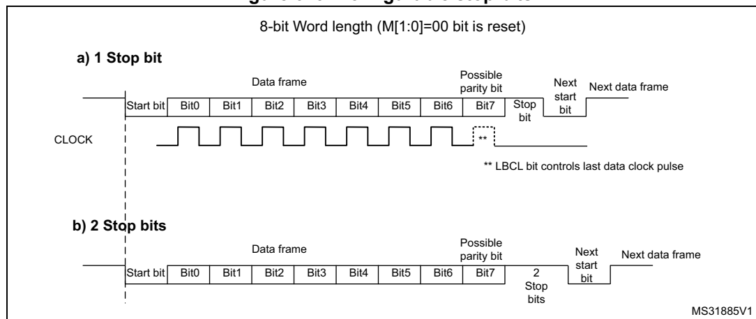
Figure 643. Configurable stop bits
