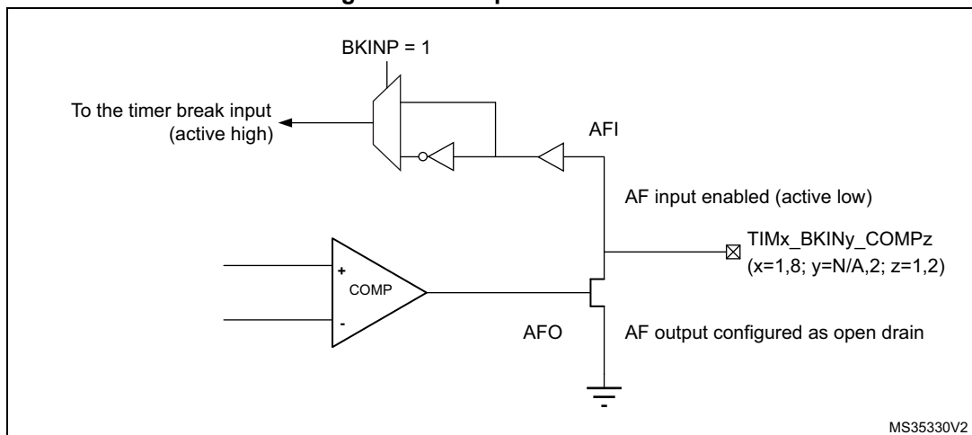
Figure 436. Output redirection
