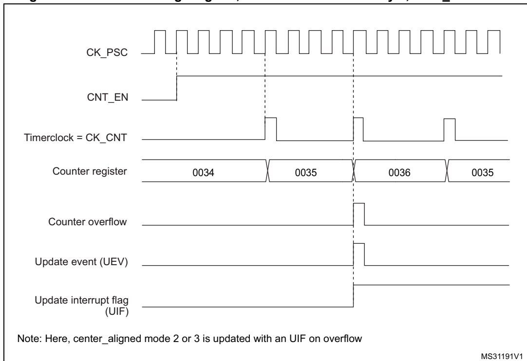
Figure 465. Counter timing diagram, internal clock divided by 4, TIMx_ARR=0x36
