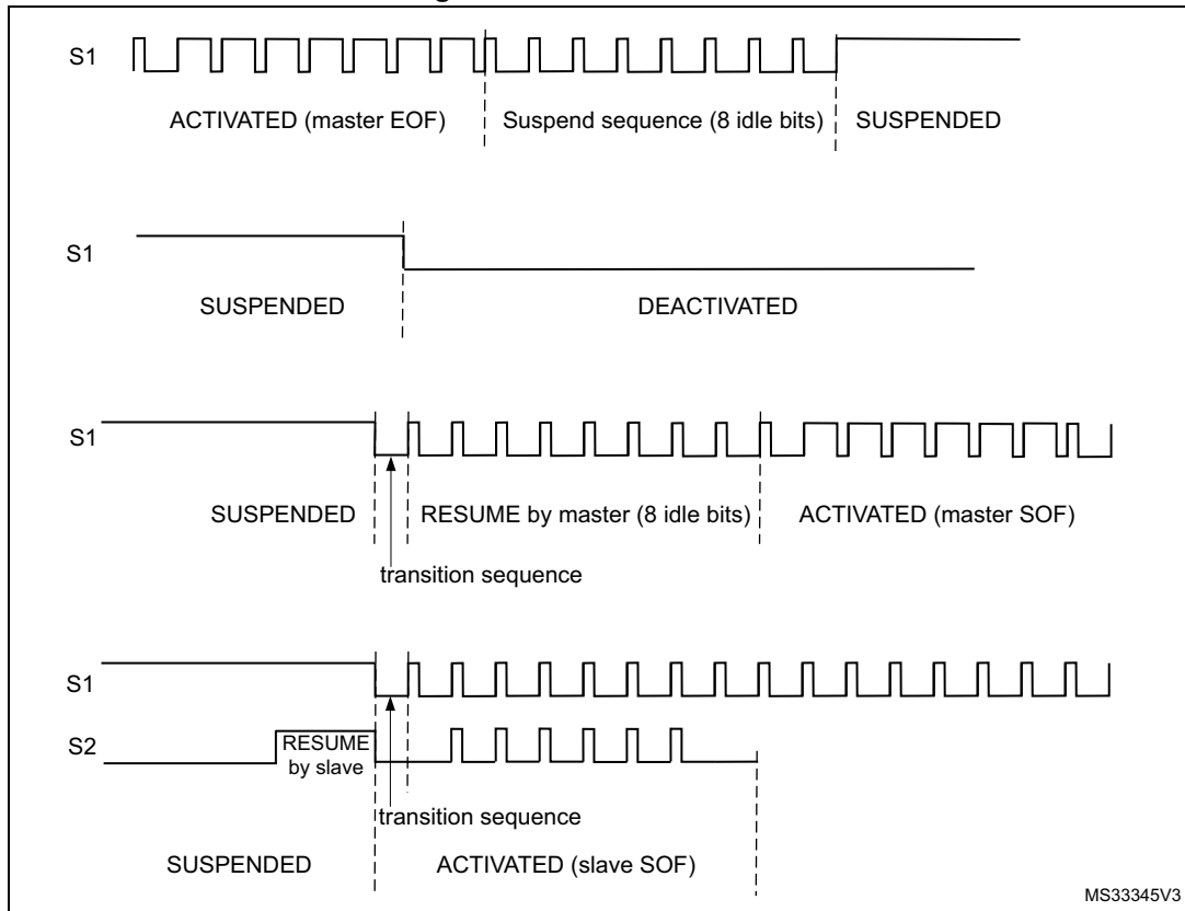
Figure 730. SWP bus states
