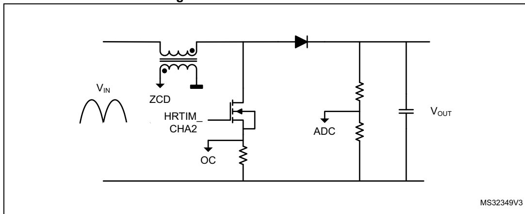
Figure 387. Transition mode PFC
