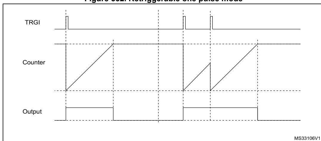
Figure 552. Retriggerable one pulse mode
