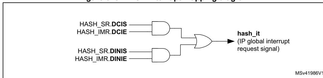
Figure 325. HASH interrupt mapping diagram
