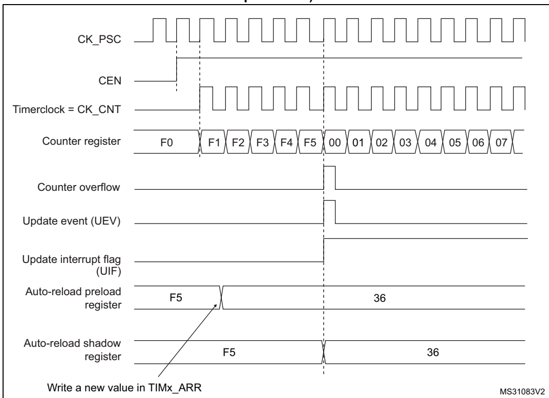
Figure 397. Counter timing diagram, update event when ARPE=1 (TIMx_ARR preloaded)
