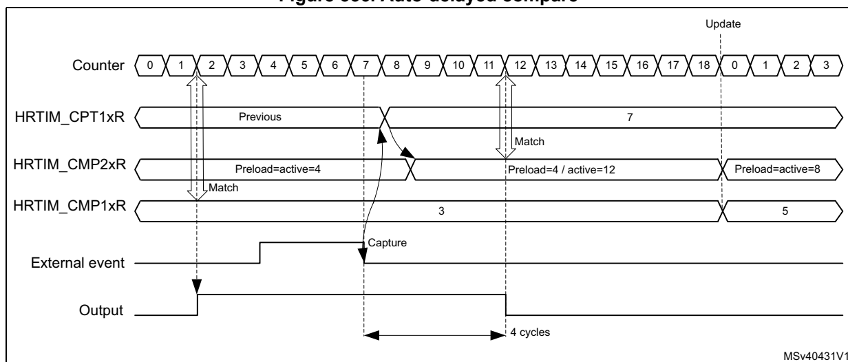
Figure 336. Auto-delayed compare
