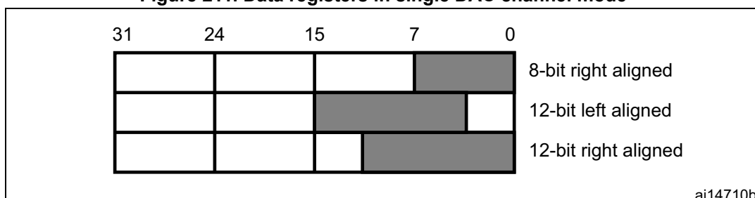
Figure 211. Data registers in single DAC channel mode
