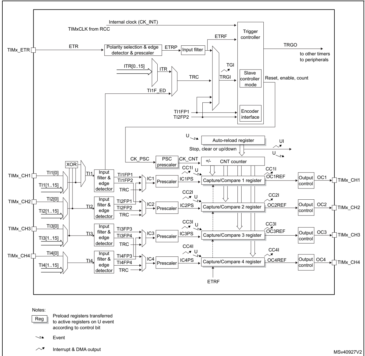
Figure 449. General-purpose timer block diagram
