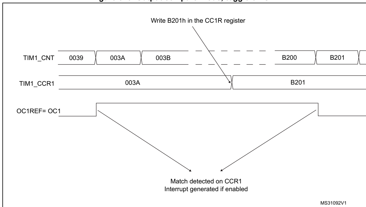
Figure 543. Output compare mode, toggle on OC1
