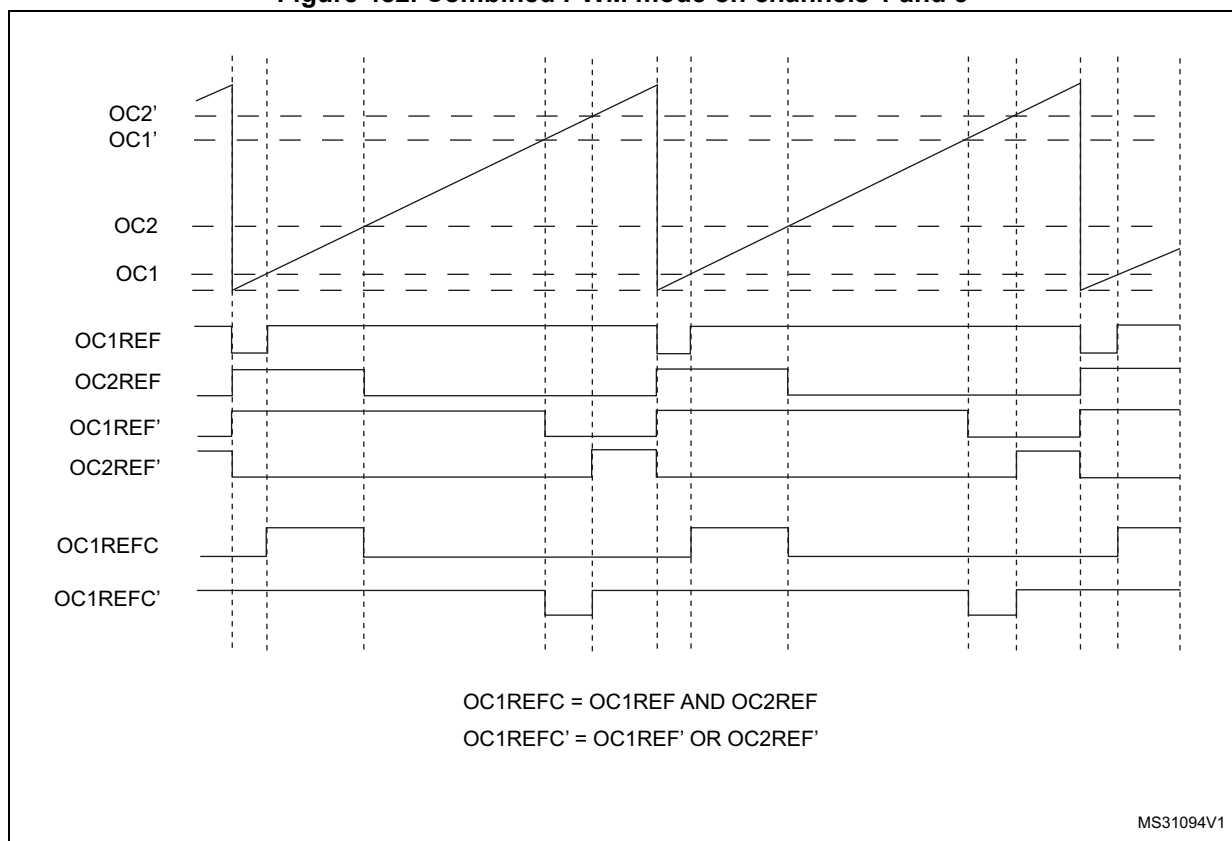
Figure 482. Combined PWM mode on channels 1 and 3
