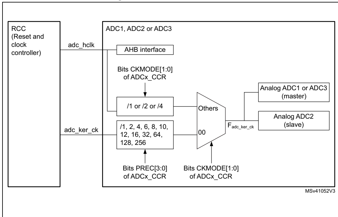
Figure 141. ADC clock scheme
