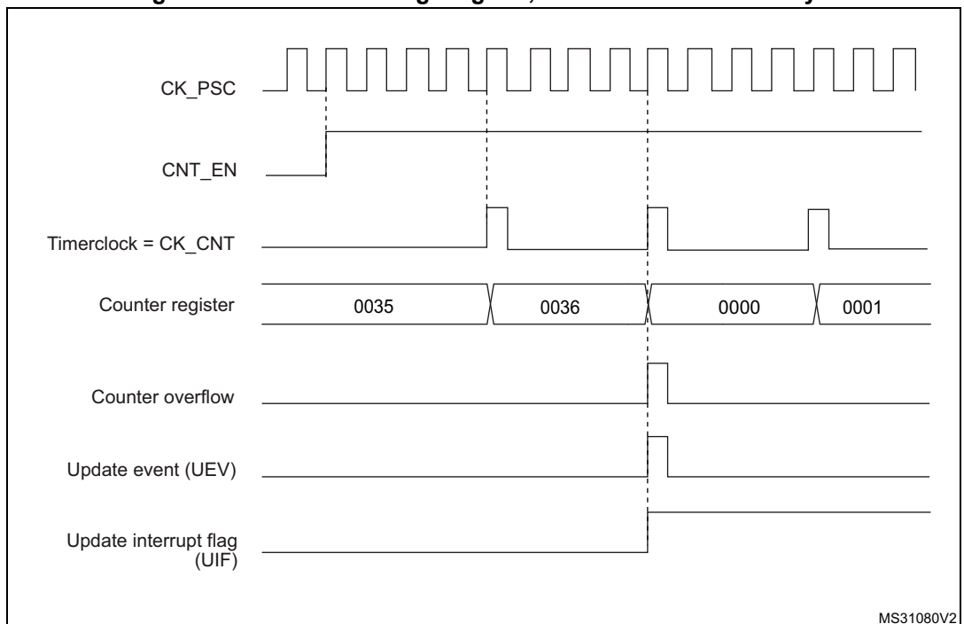
Figure 504. Counter timing diagram, internal clock divided by 4
