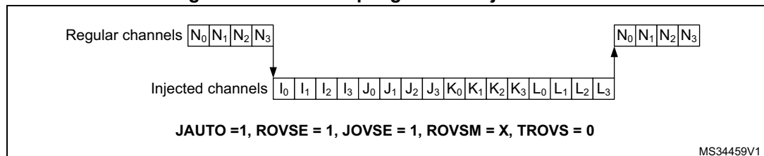
Figure 190. Oversampling in auto-injected mode
