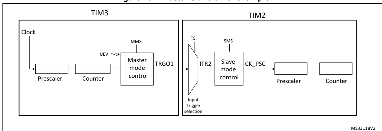
Figure 492. Master/Slave timer example
