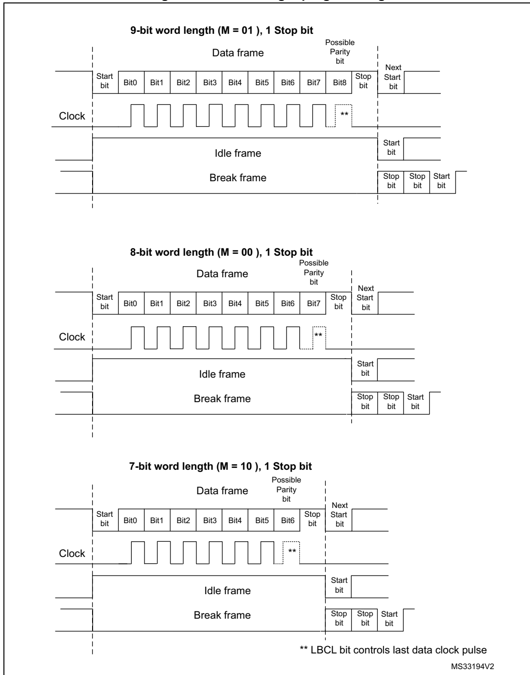
Figure 615. Word length programming
