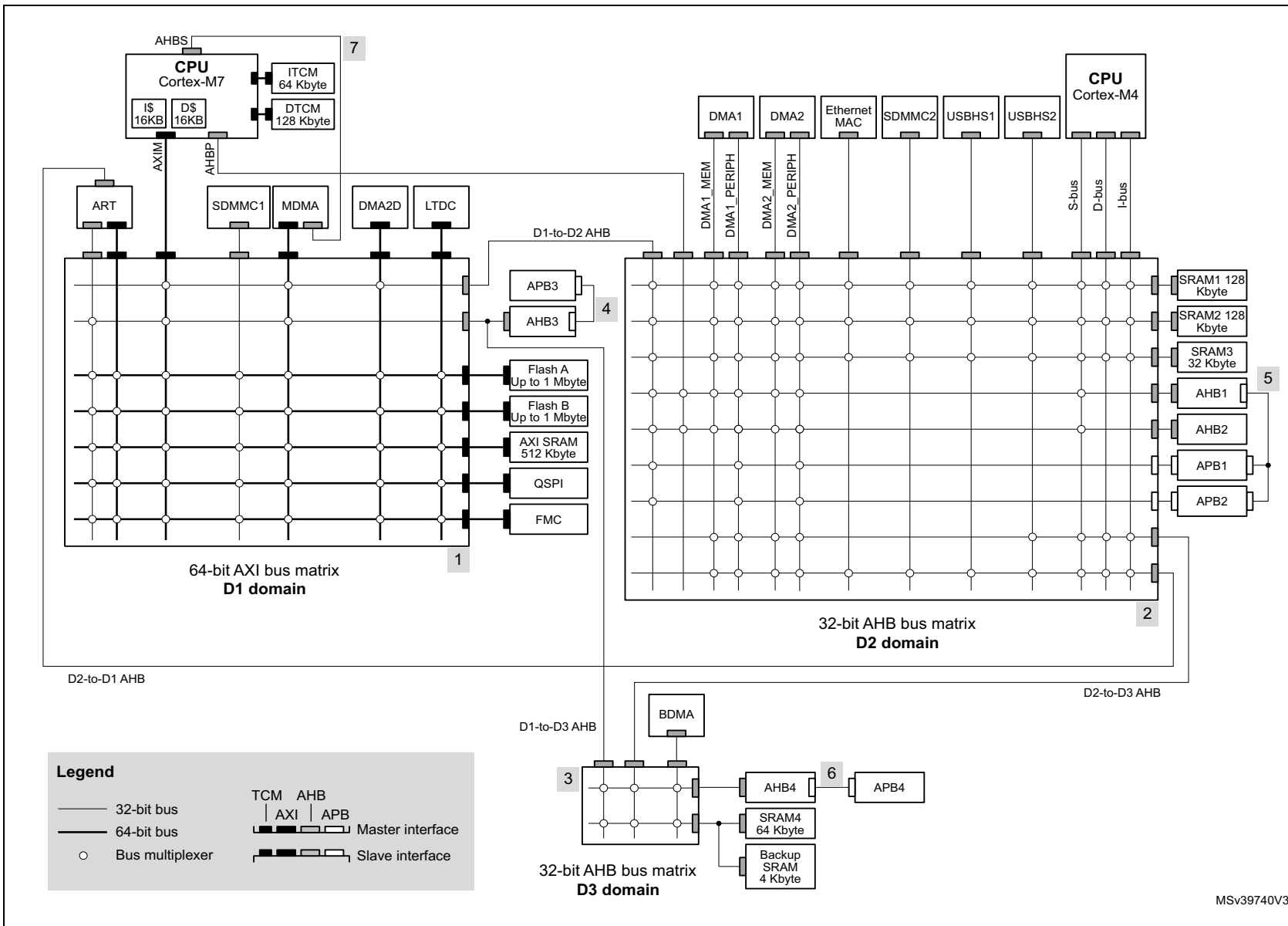
Figure 1. System architecture for STM32H745/55/47/57xx devices
