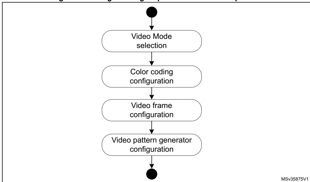
Figure 289. Programming sequence to send a test pattern
