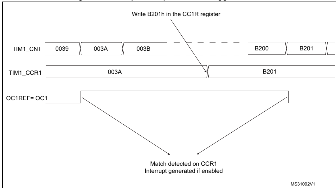
Figure 515. Output compare mode, toggle on OC1.
