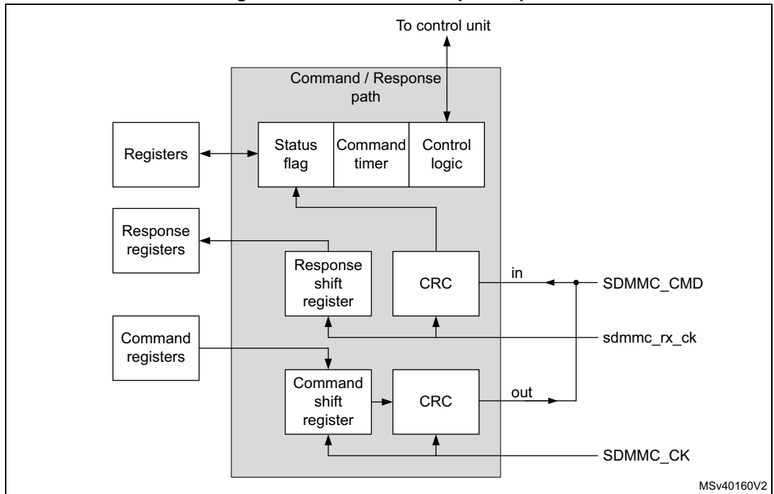
Figure 750. Command/Response path
