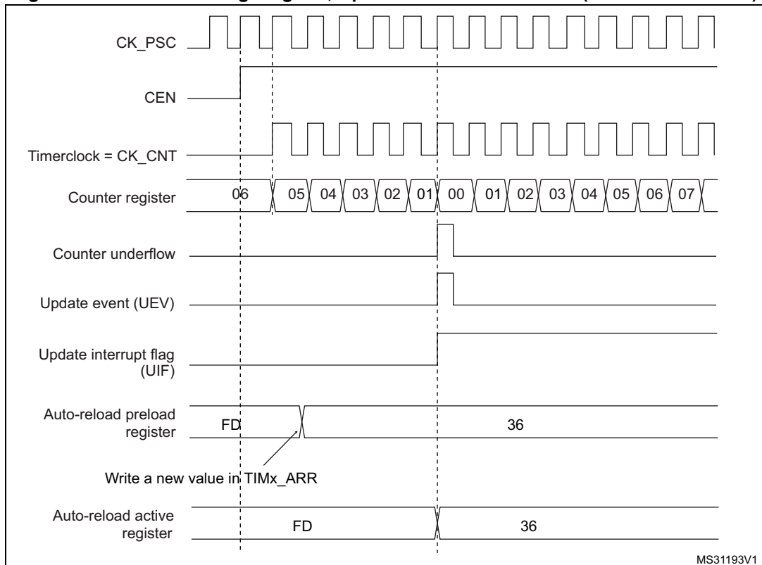
Figure 467. Counter timing diagram, Update event with ARPE=1 (counter underflow)
