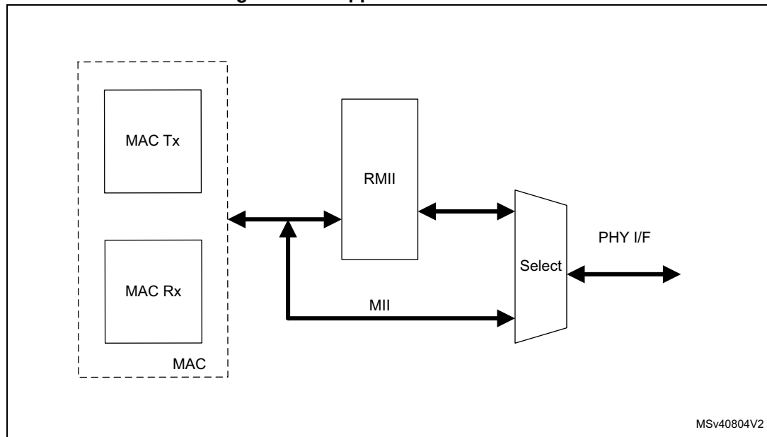
Figure 834. Supported PHY interfaces
