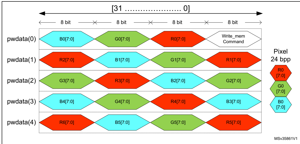
Figure 260. 24 bpp APB pixel to byte organization
