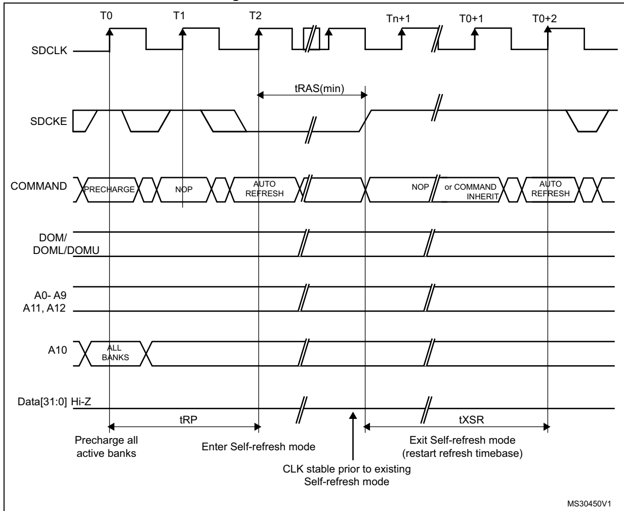
Figure 129. Self-refresh mode
