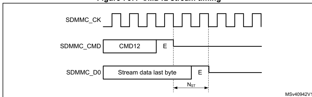
Figure 767. CMD12 stream timing
