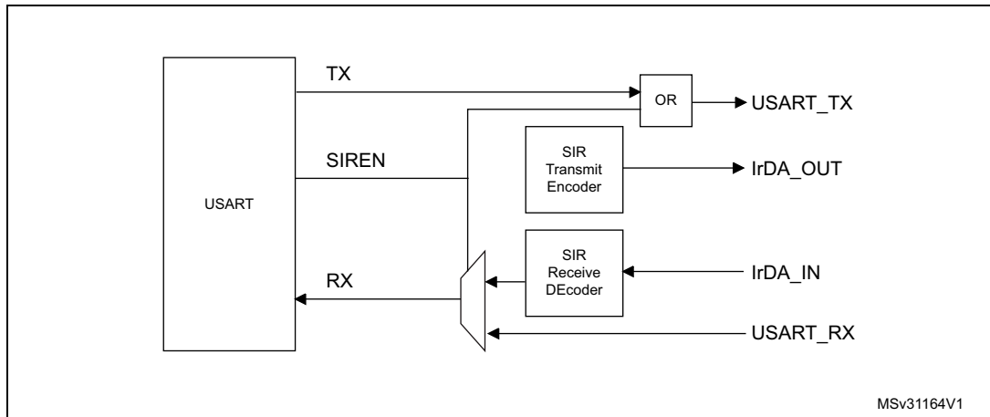
Figure 632. IrDA SIR ENDEC block diagram
