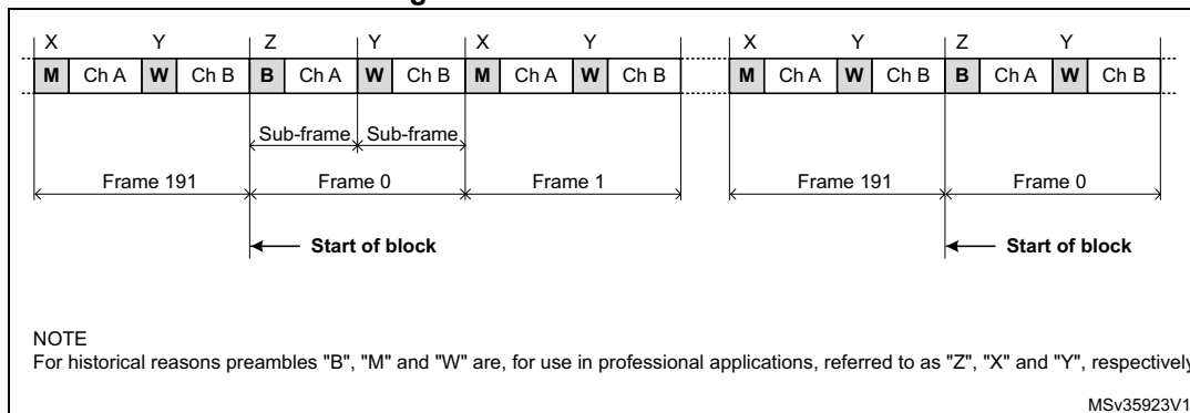
Figure 713. S/PDIF block format
