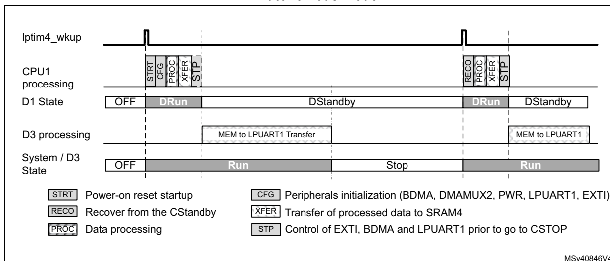
Figure 44. Timing diagram of SRAM4-to-LPUART1 transfer with BDMA and D3 domain in Autonomous mode
