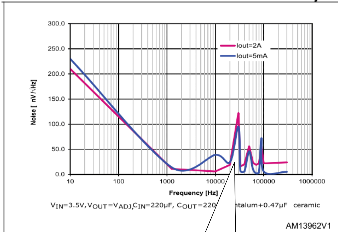
Figure 37. Output noise spectrum ( V_{out}=V_{adj} )
