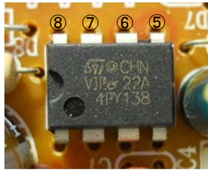
"VIPer22A" implemented in SMPS
