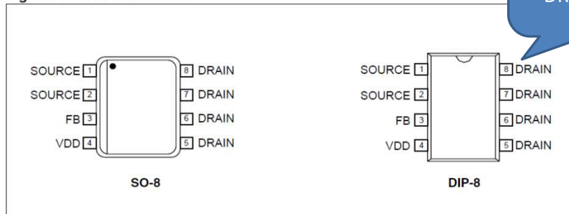
Figure 2. Pin connection
