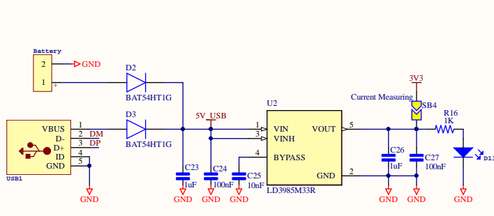
Power Supply
