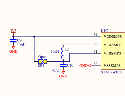
MCU Power Supply
