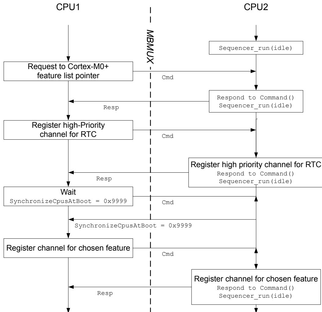
Figure 16. MBMUX initialization
