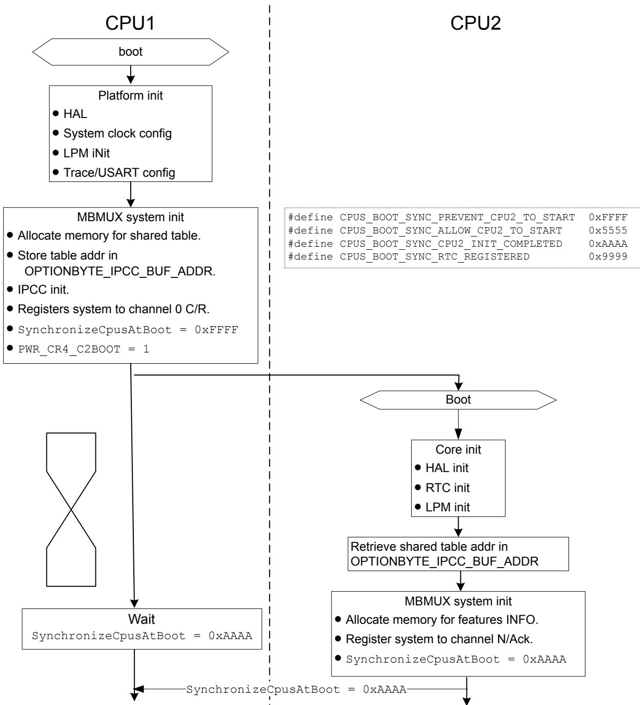
Figure 15. Startup sequence
