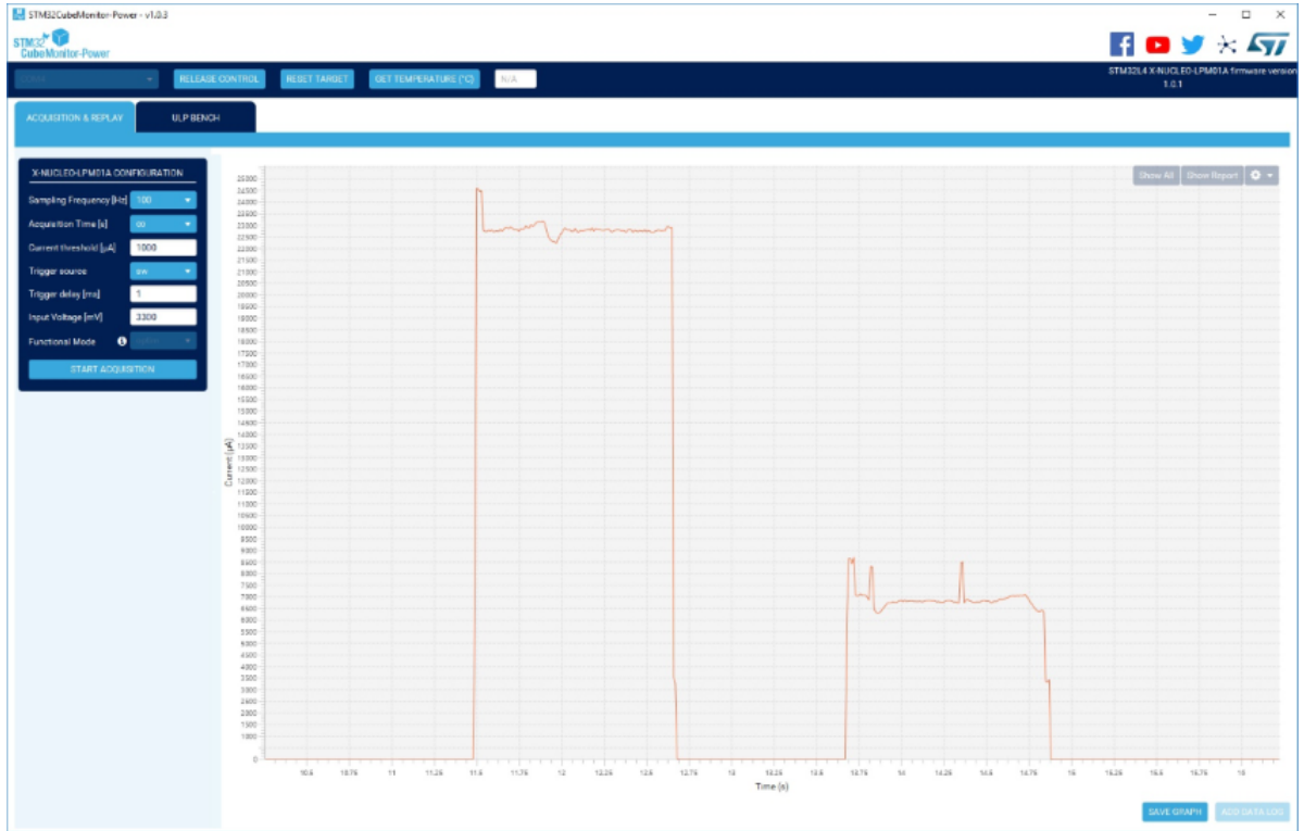
Figure 21. NUCLEO-WL55JC1 current consumption versus time
