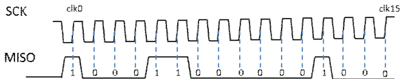
Figure 20 SPI Bit Order (transmission of 0x8C08)
