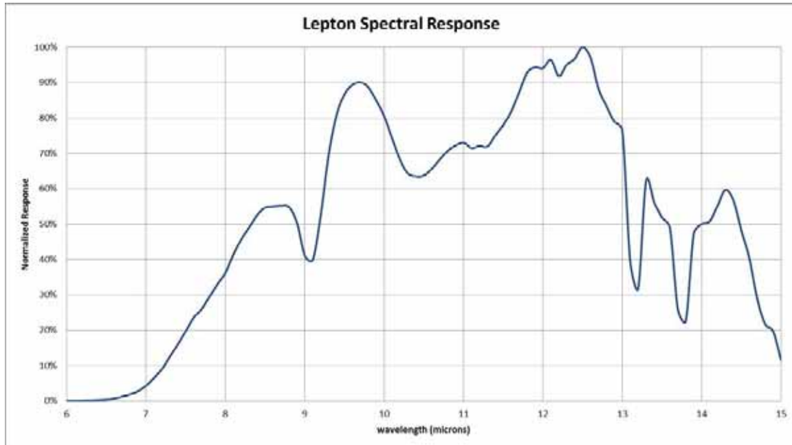
Figure 40 Normalized Response as a Function of Signal Wavelength
