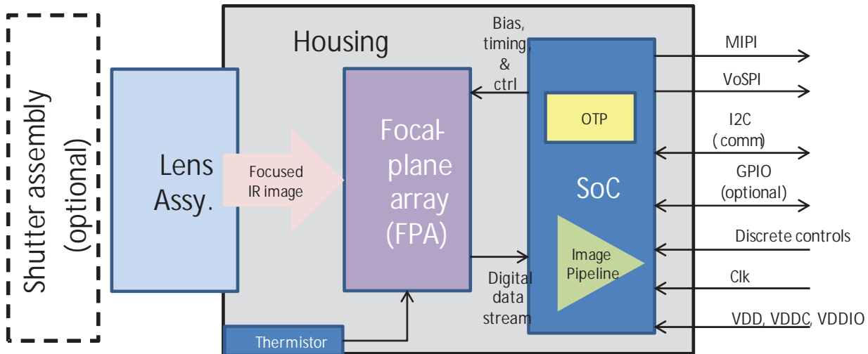
Figure 4 Lepton 3 Architecture
