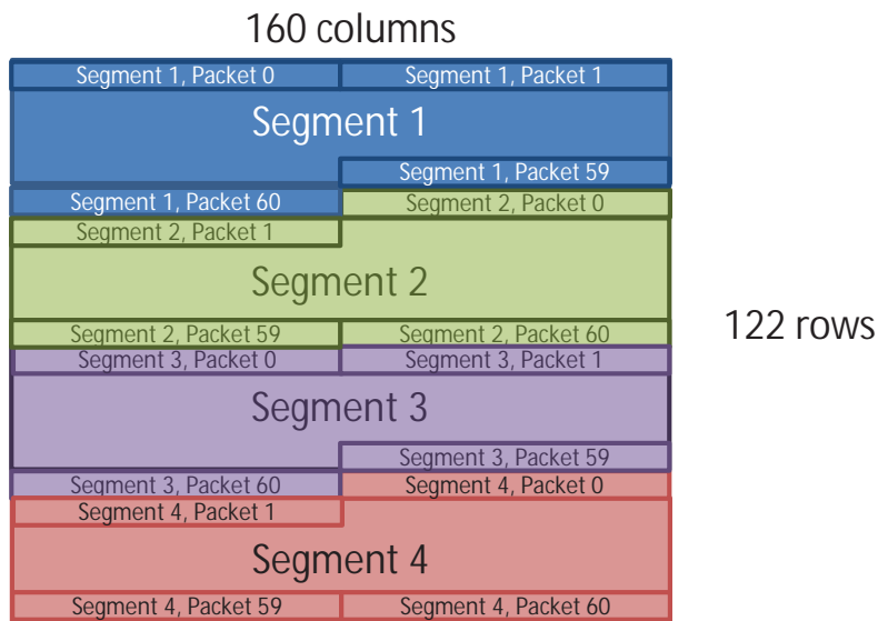
(b) Frame contents with telemetry enabled
