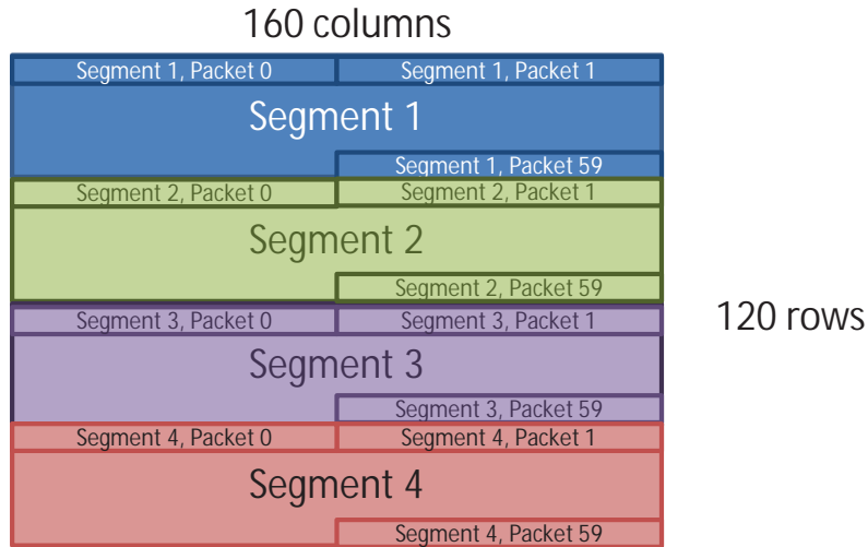
(a) Frame contents with telemetry disabled
