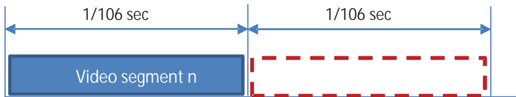
Figure 32 Failure to Read Out an Available Frame
