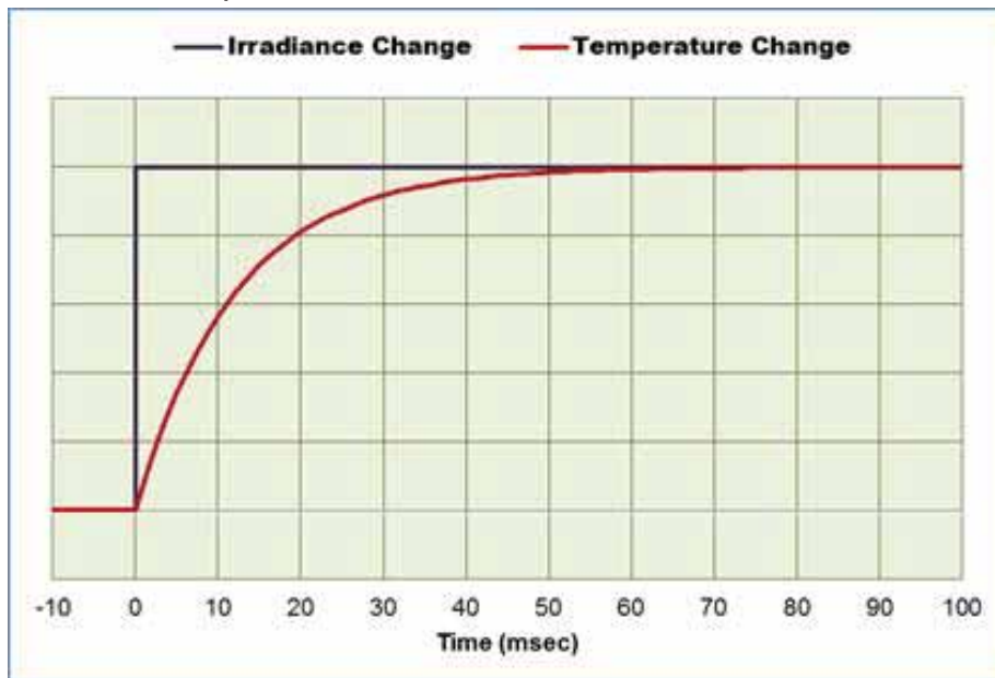
Figure 33 Illustration of Lepton 3 Detector Time Constant
