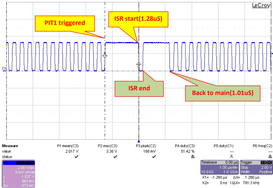
Output of PC9 (Pin-2) of SPC560D4x
